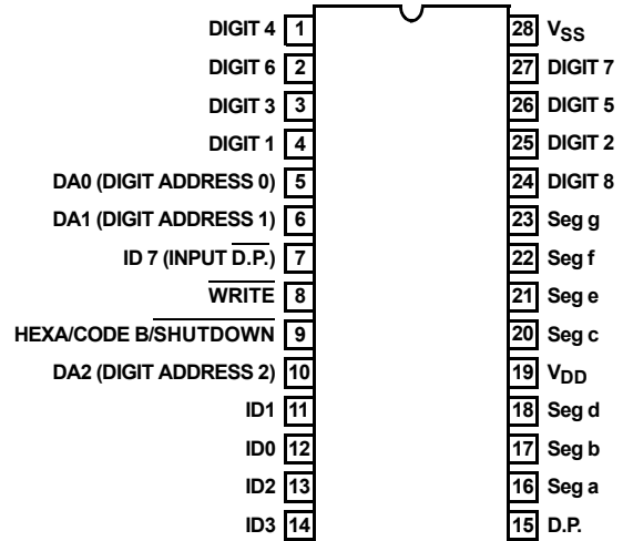
ICM7218B (28 LD CERDIP) TOP VIEW
