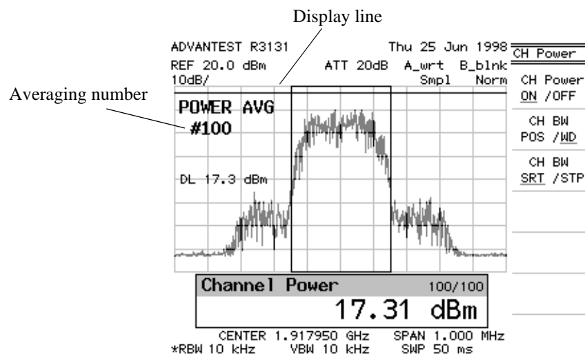
Figure 2-55 Measuring the Channel Power
