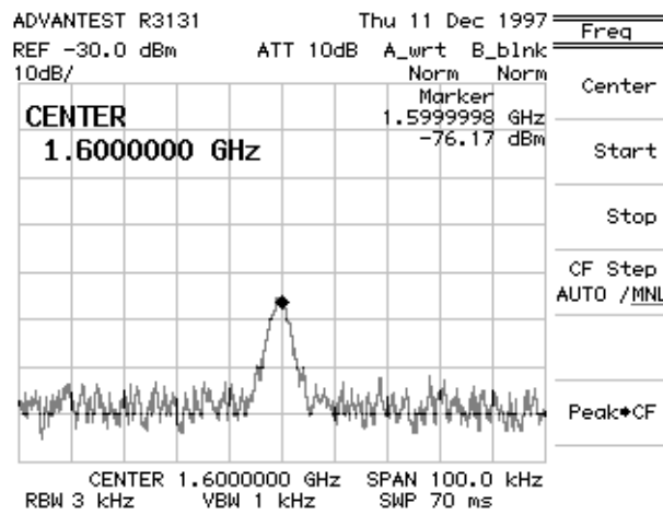
Figure 2-76 Measuring the Harmonic Distortion
