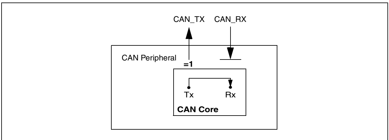
Figure 46. CAN Core in Silent Mode
