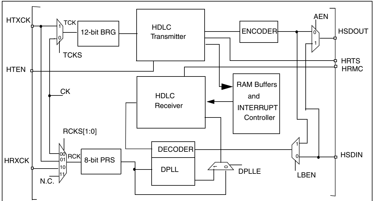
Figure 73. HDLC functional block
