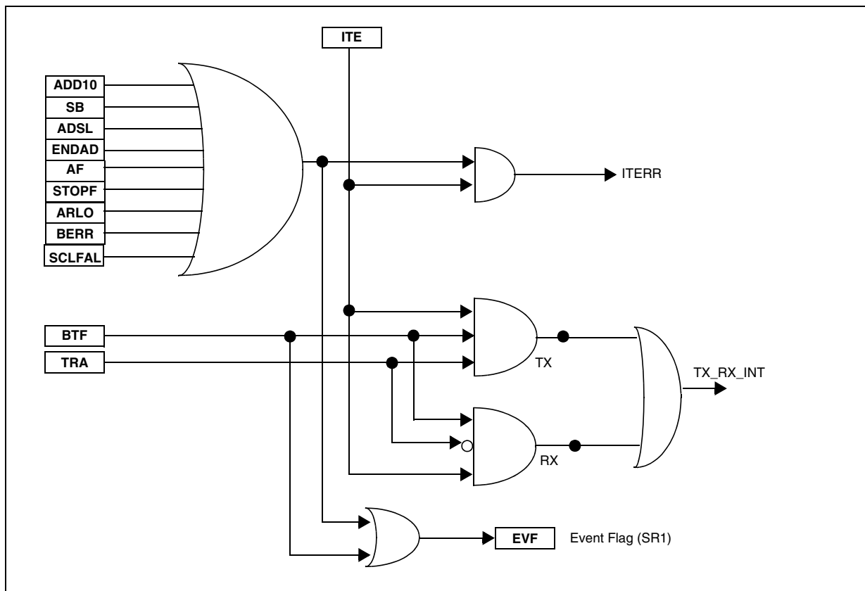
Figure 59. Event Flags and Interrupt Generation
