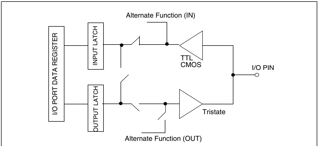
Figure 21. Input Configuration
