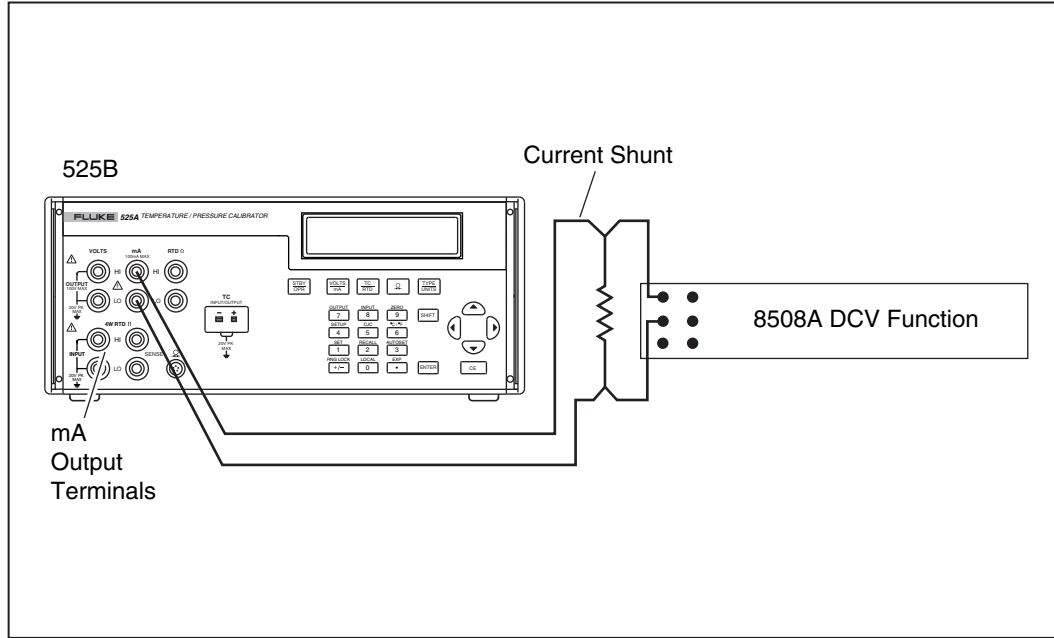
Figure 6-2. Output DC Current
