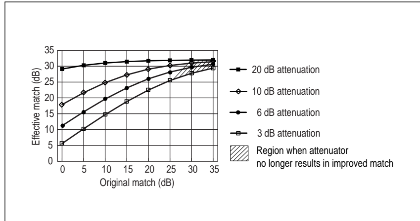
Figure 12. Effective Match as a Function of Attenuation (Attenuator Match = 32 dB)
