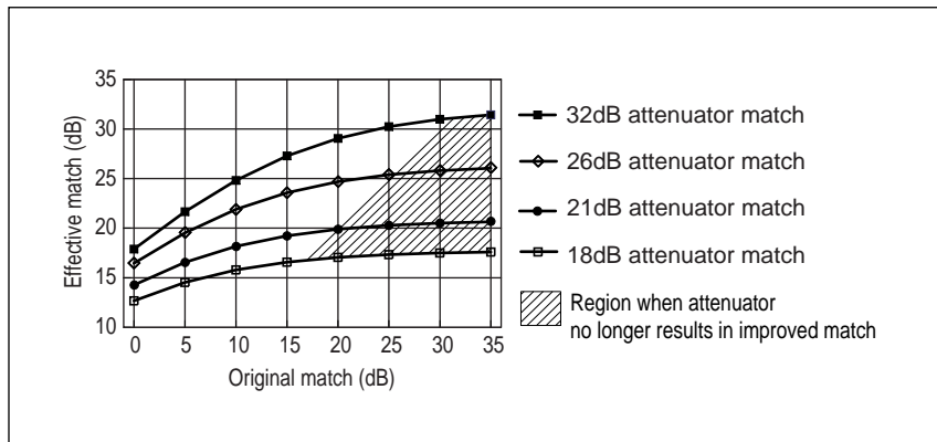
Figure 11. Effective Match as a Function of Attenuator's Match (Fixed 10 dB Attenuator).
