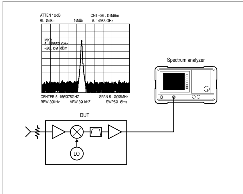
Figure 34. Feedthrough of Tuners and Converters
