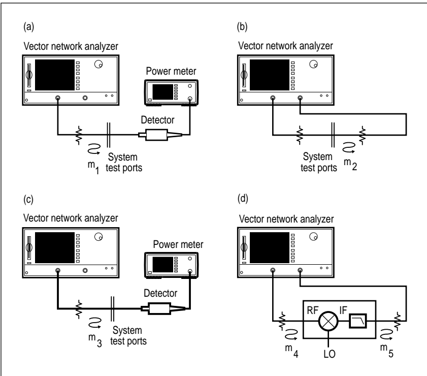
Figure 22. (a) Power Meter Calibration over the IF Range. (b) Normalization Calibration over the IF Range. (c) Power Meter Calibration over the RF Range. (d) DUT is Measured.
