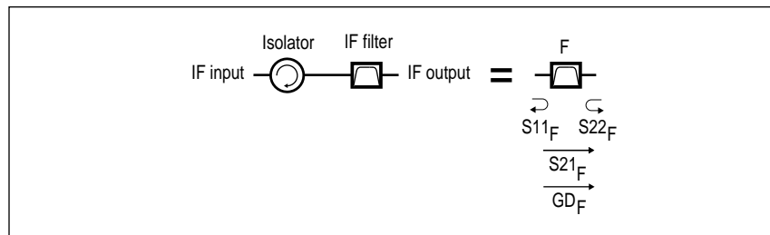
Figure 37. Diagram of the Filter Assembly
