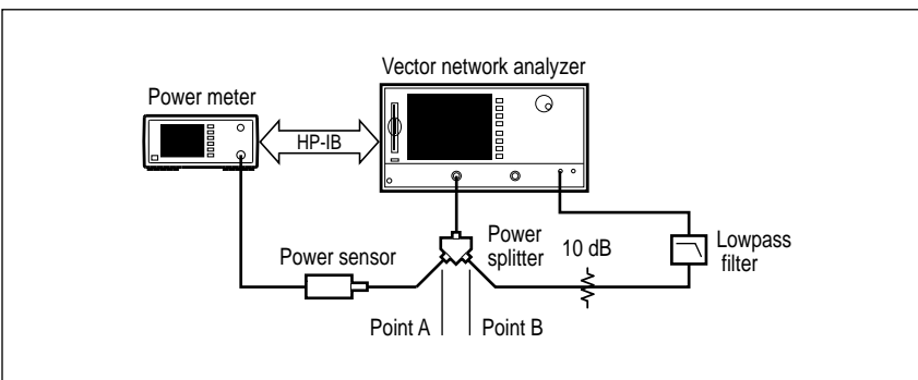
Figure 17. Configuration for Power Meter Calibration over the IF Range
