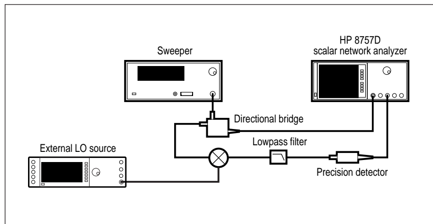
Figure 2. HP 8757D Scalar Network Analyzer Configuration
