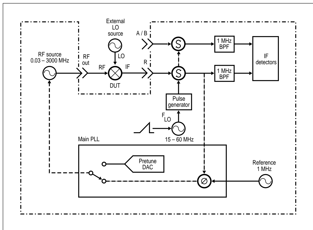
Figure 16. HP 8753E Block Diagram of Frequency Offset Mode
