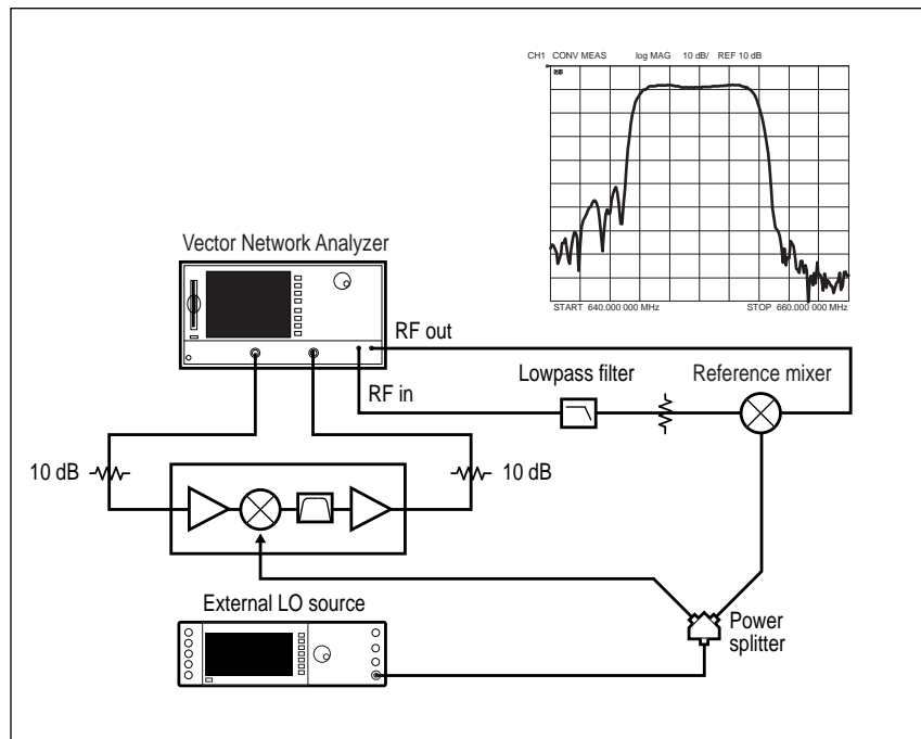
Figure 4. Vector Network Analyzer, High Dynamic Range Configuration
