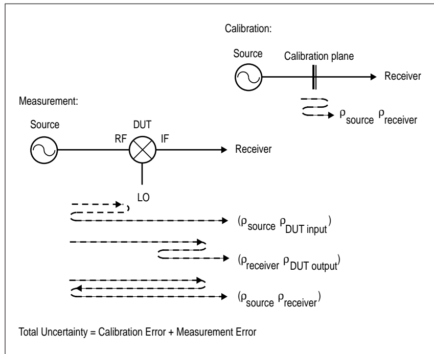
Figure 9. Mismatch Effects
