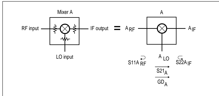
Figure 36. Diagram of the Mixer Assembly
