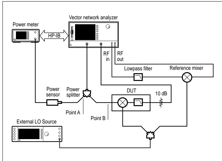
Figure 20. Power Meter Calibration over the RF Range, High- Dynamic-Range Configuration
