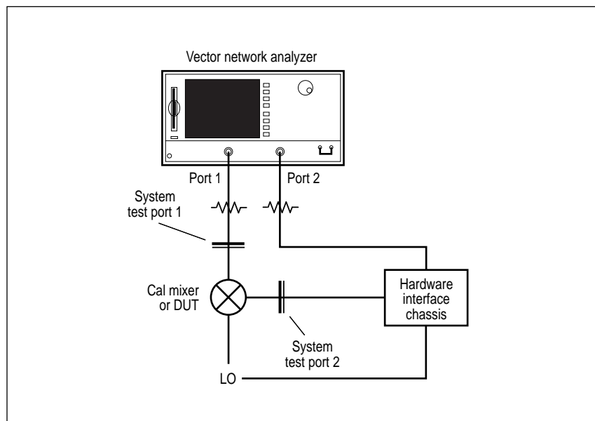
Figure 42. Typical Configuration of Test System
