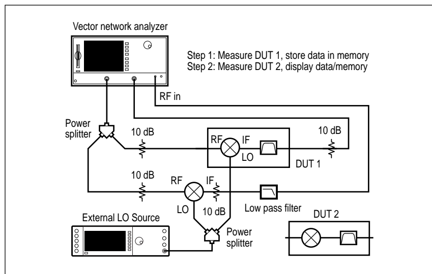
Figure 24. Mixer Matching — Magnitude and Group Delay
