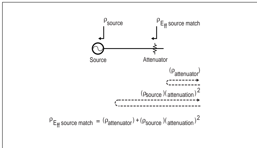
Figure 10. Effective Match as a function of Attenuator's Match.
