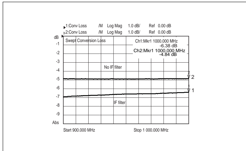
Figure 13. Conversion Loss Response with and without an IF Filter
