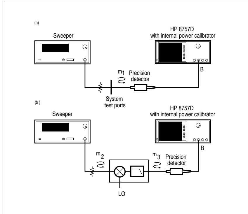
Figure 21. (a) Absolute Power Measurement over the RF Range (b) Absolute Power Measurement over the IF Range.
