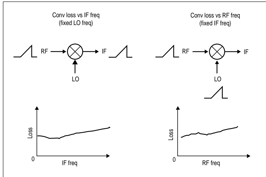
Figure 7. Two Types of Conversion Loss Measurements
