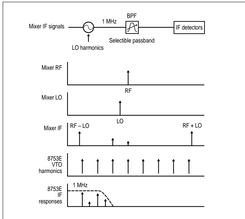
Figure 15. Effects of IF BW on Spurious Measurement Responses
