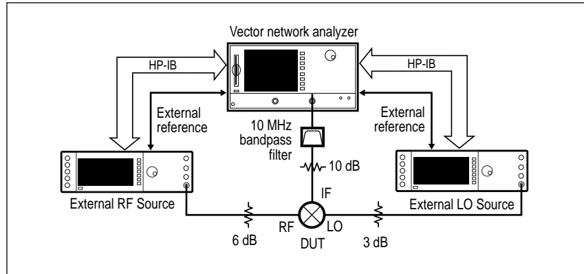
Figure 23. Fixed IF Configuration
