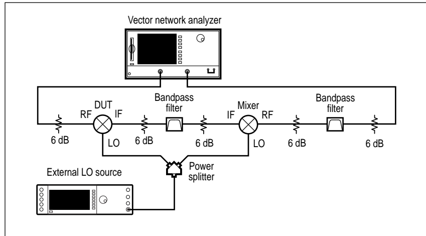
Figure 5. Upconversion/ Downconversion Configuration
