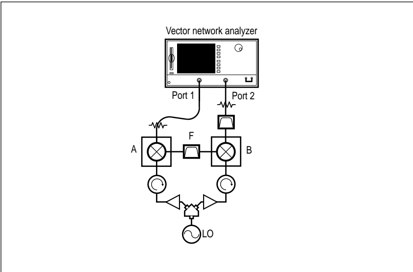
Figure 41. Typical Configuration for Measuring the Mixer-Pairs
