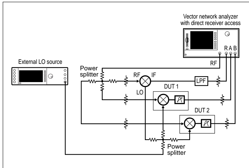
Figure 26. Simultaneous Tuning and High- Dynamic Range Configuration
