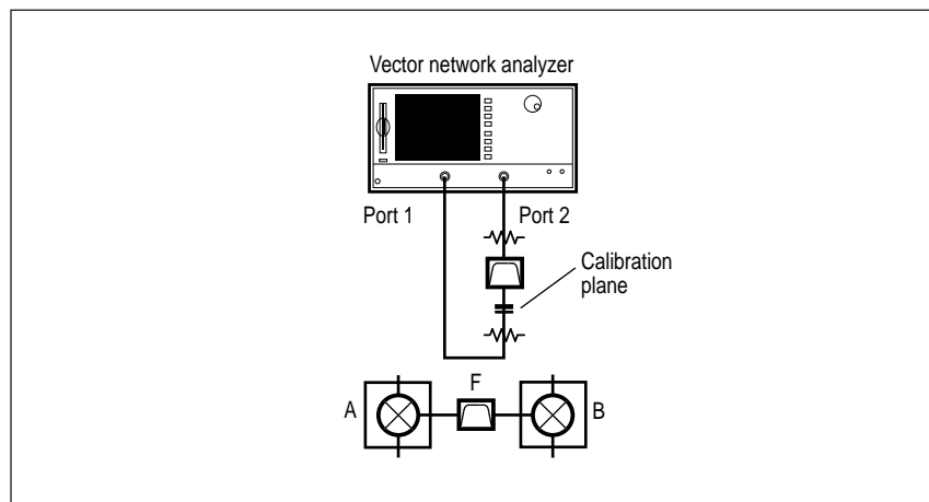
Figure 40. Typical Configuration for Calibrating the Test System
