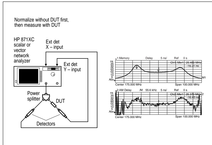
Figure 30. AM Delay Measurements using the HP 8711 Series
