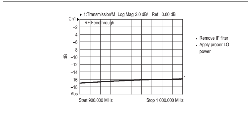
Figure 33. RF Feedthrough
