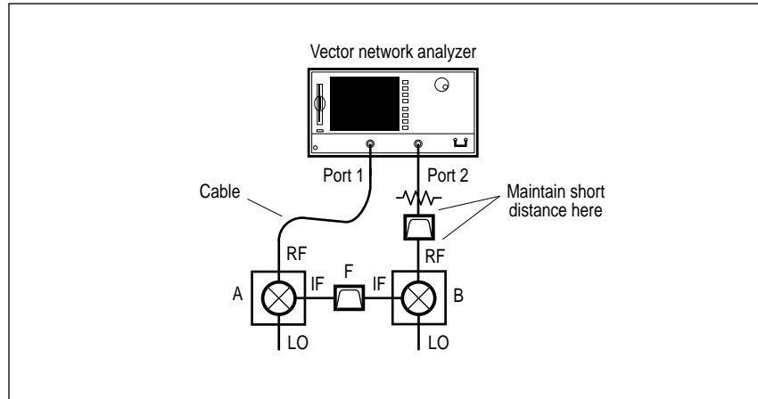
Figure 38. Diagram of the Suggested Component Connections
