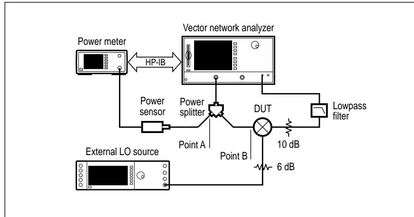
Figure 18. Configuration for Power-Meter Calibration over the RF Range.
