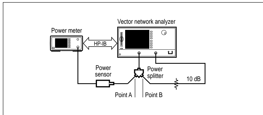
Figure 19. Power Meter Calibration over the IF Range, High-Dynamic- Range Configuration.
