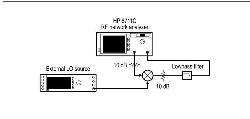
Figure 1. HP 8711C Scalar Network Analyzer Configuration
