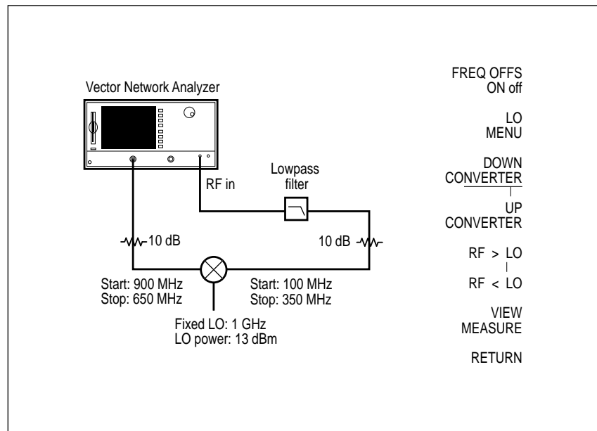
Figure 3. Vector Network Analyzer in Frequency Offset Mode
