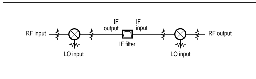
Figure 35. Typical Configuration for a Mixer Pair
