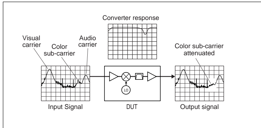
Figure 8. TV Tuner Conversion Loss Example
