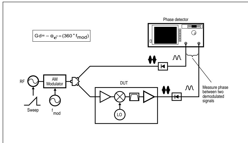
Figure 29. Modulation Delay Method for Measuring Group Delay
