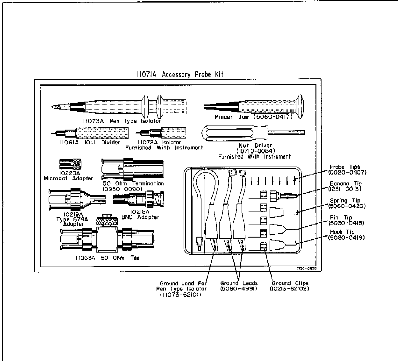
Figure 1-3. 11071A Complete Probe Kit
