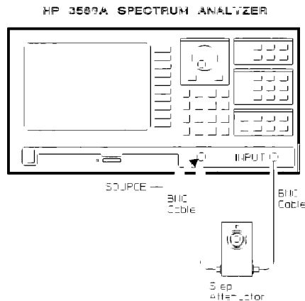
Figure 3 15 Source Dynamic Accuracy Setup
