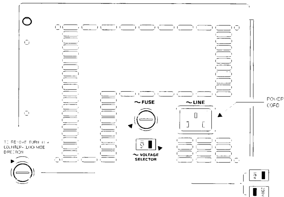
Figure 2-1. Voltage Selection and Fuse Replacement
