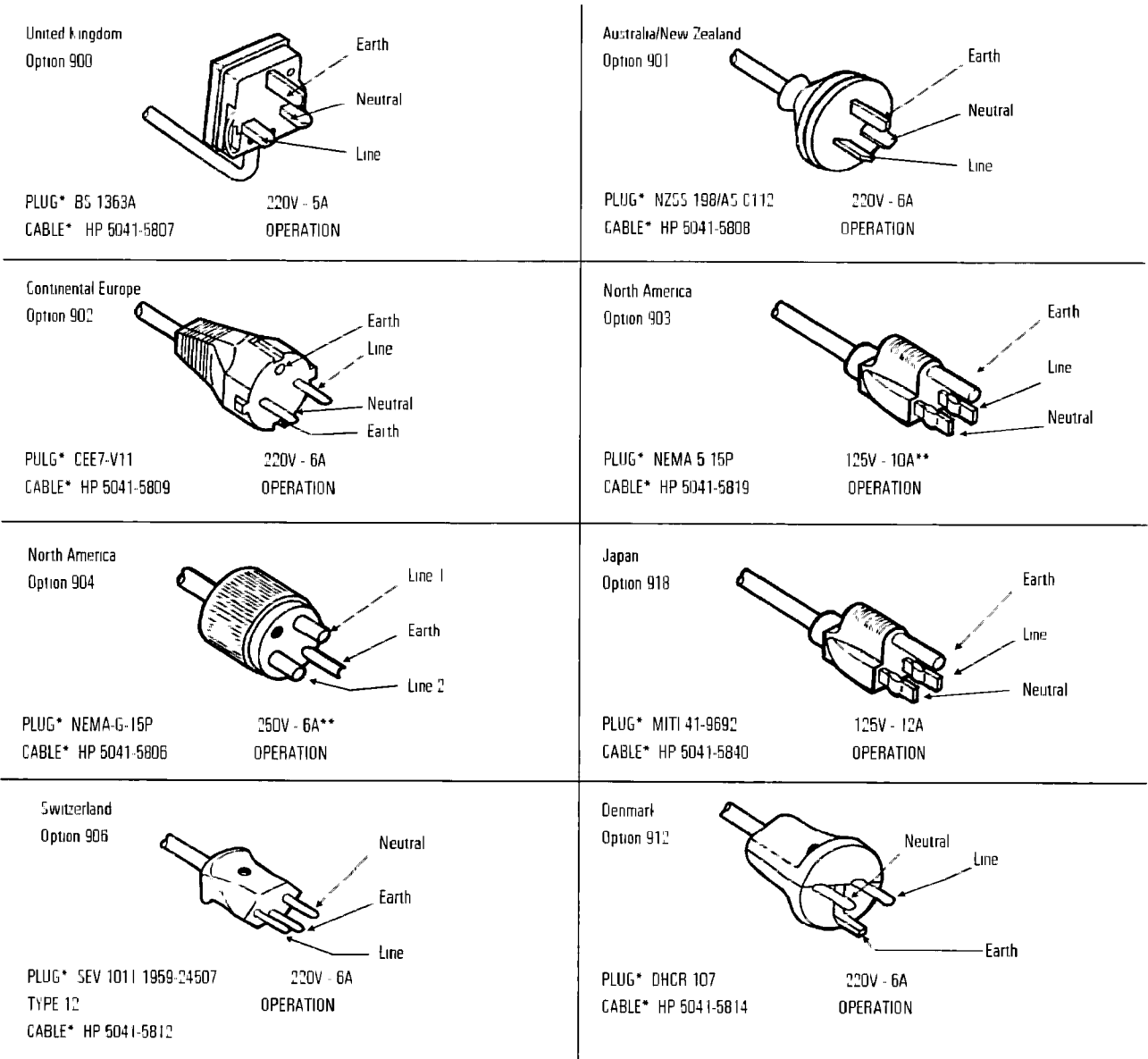
Figure 2-2. Power Cables
