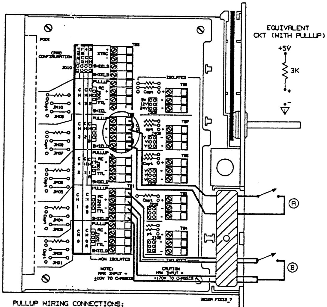
Figure 12-7. Using Pullup Resistors
