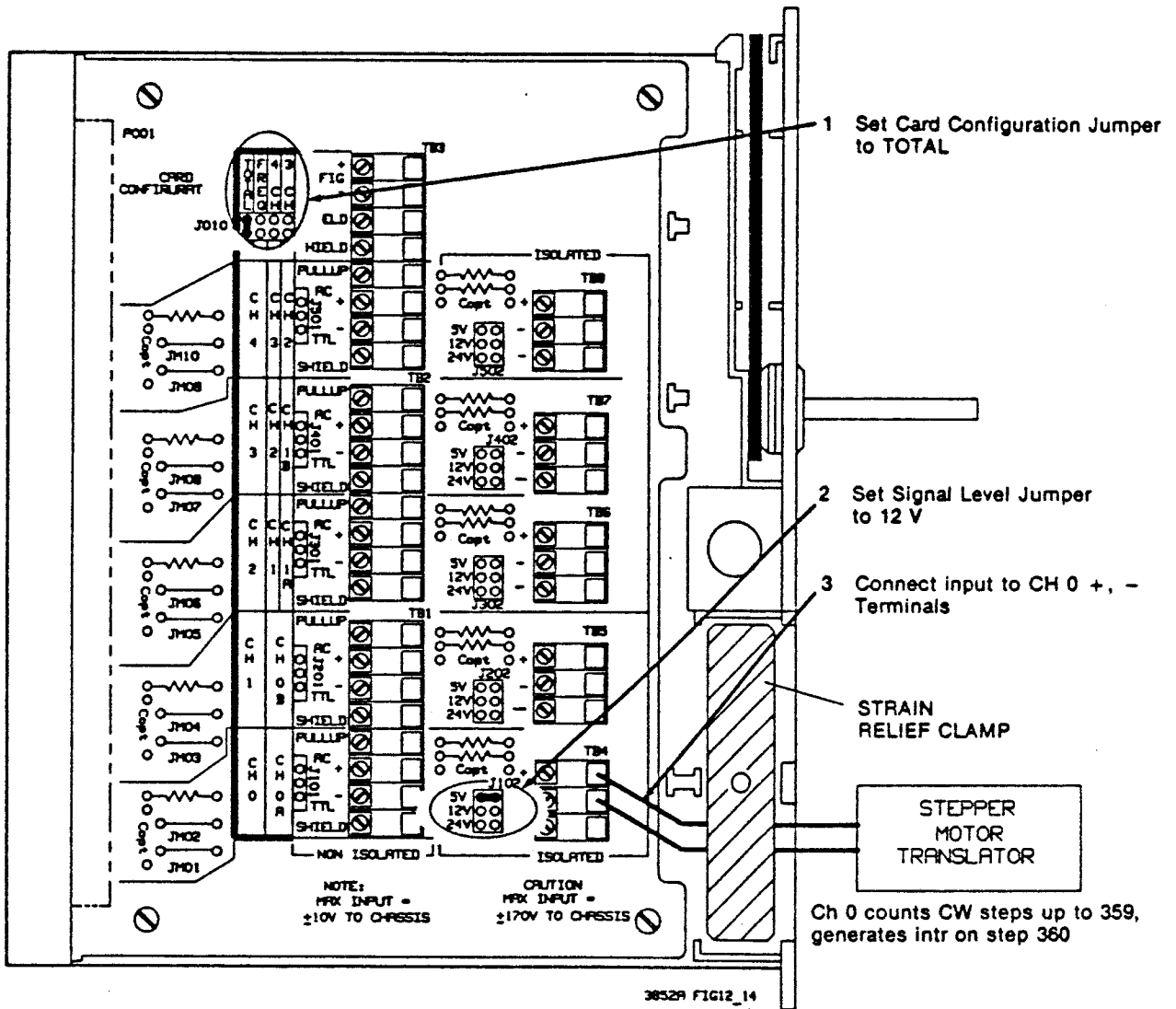
Figure 12-14. Example: Totalize Stepper Motor Steps
