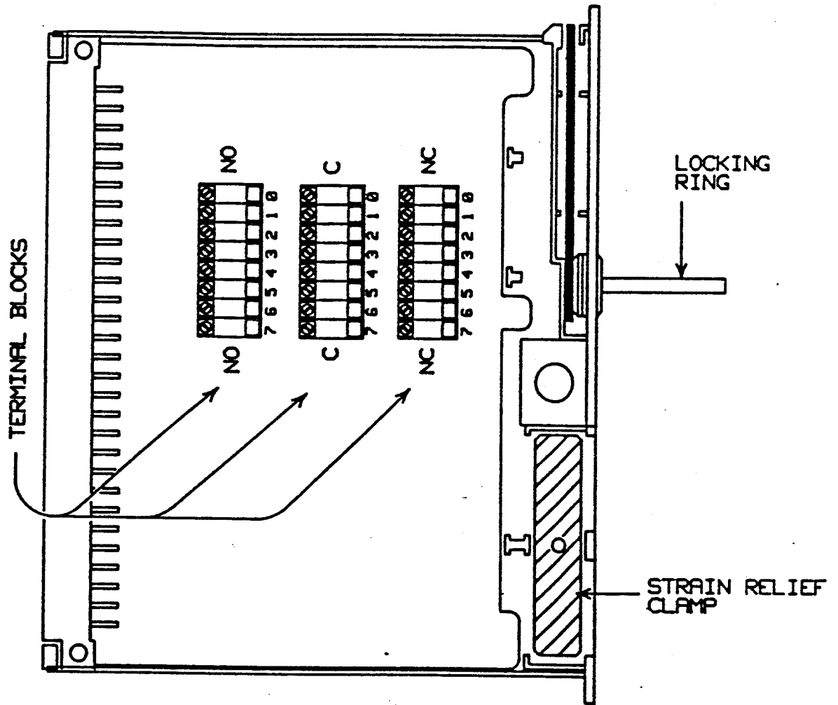
Figure 17-1. Terminal Block Wiring Layout
