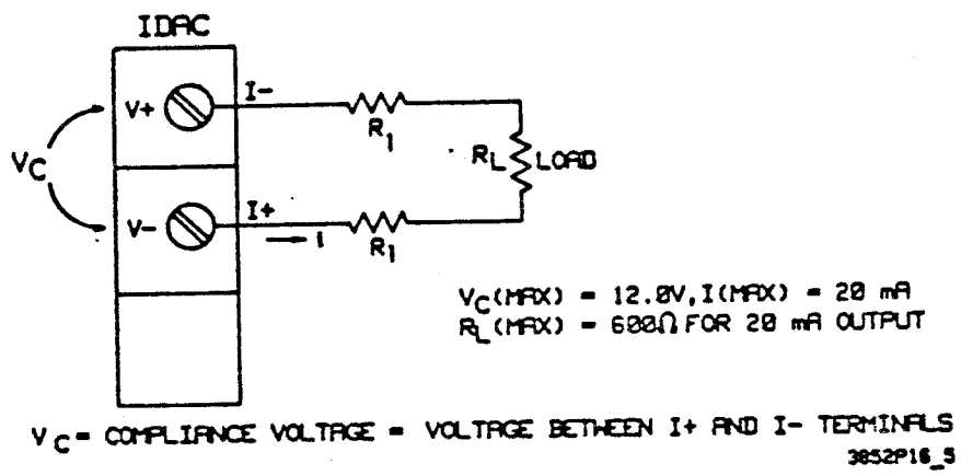
Figure 16-5. Compliance Voltage
