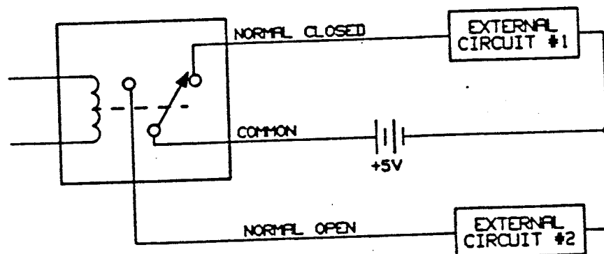
VOLTAGE SWITCHING
