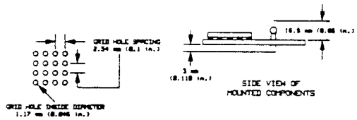
Figure 19-1. Dimensions and Component Height/Protrusion Restrictions
