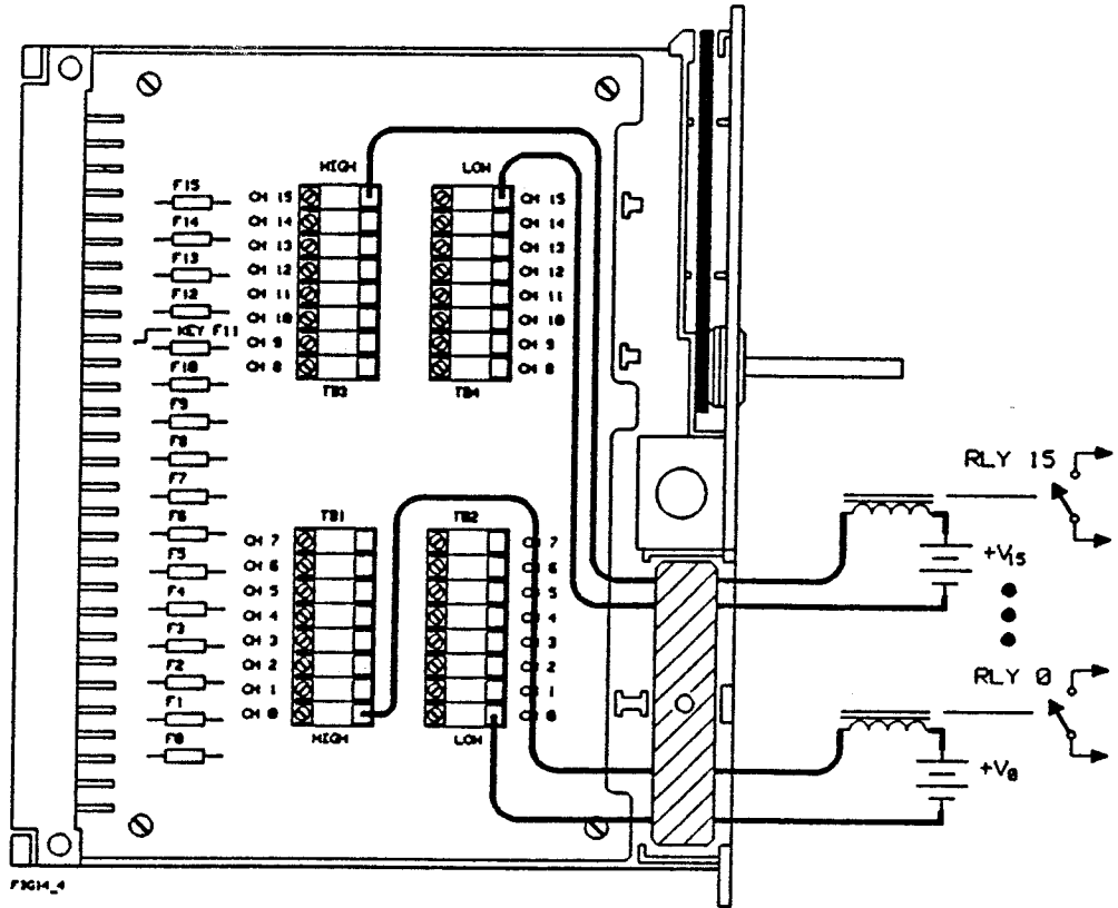
Figure 14-4. Opening/Closing Relays
