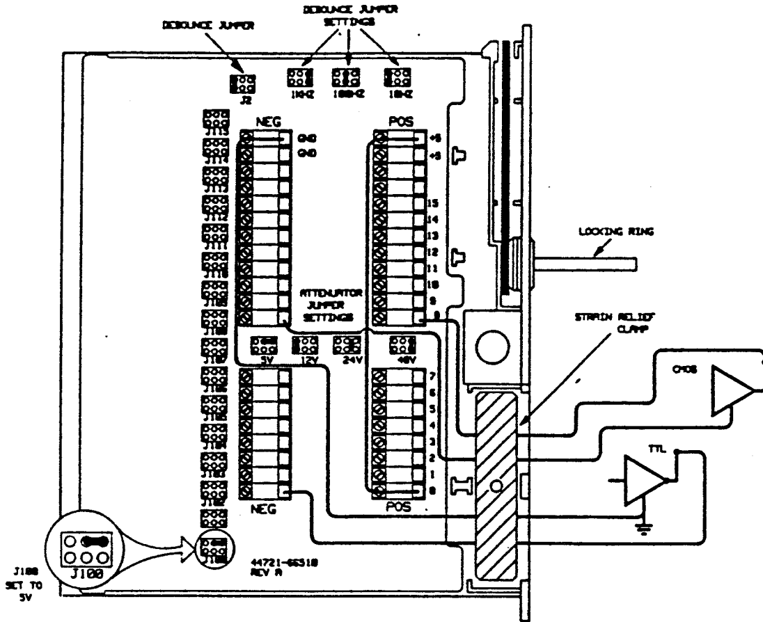
Figure 13-10. Connecting TTL/CMOS to 16-Channel Digital Input
