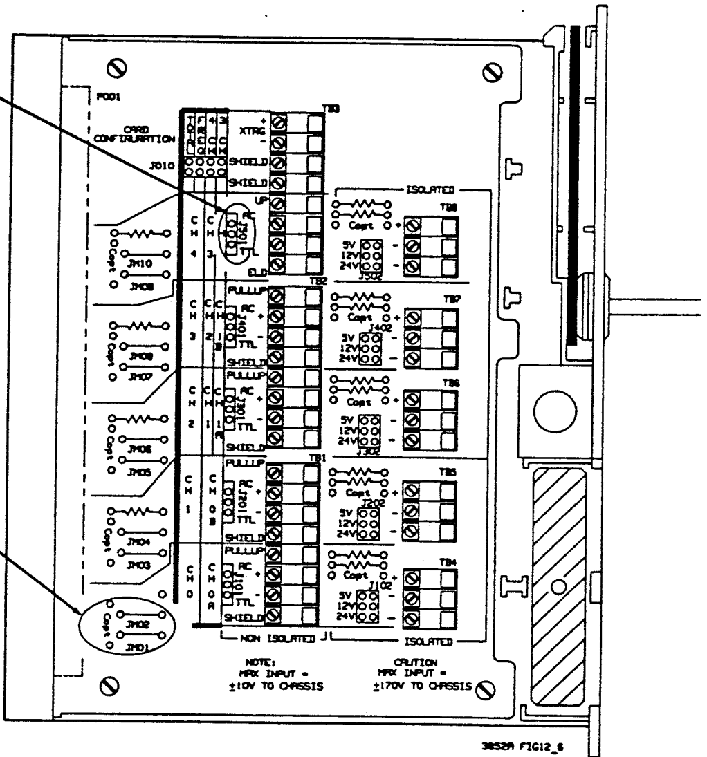
Figure 12-6. Signal Conditioning - Non-Isolated Channels
