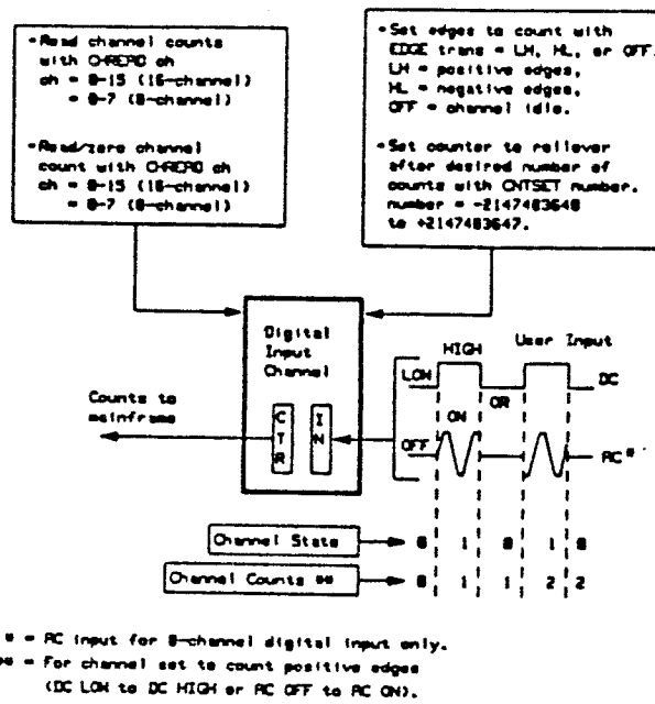
Figure 13-19. Counting Input Events
