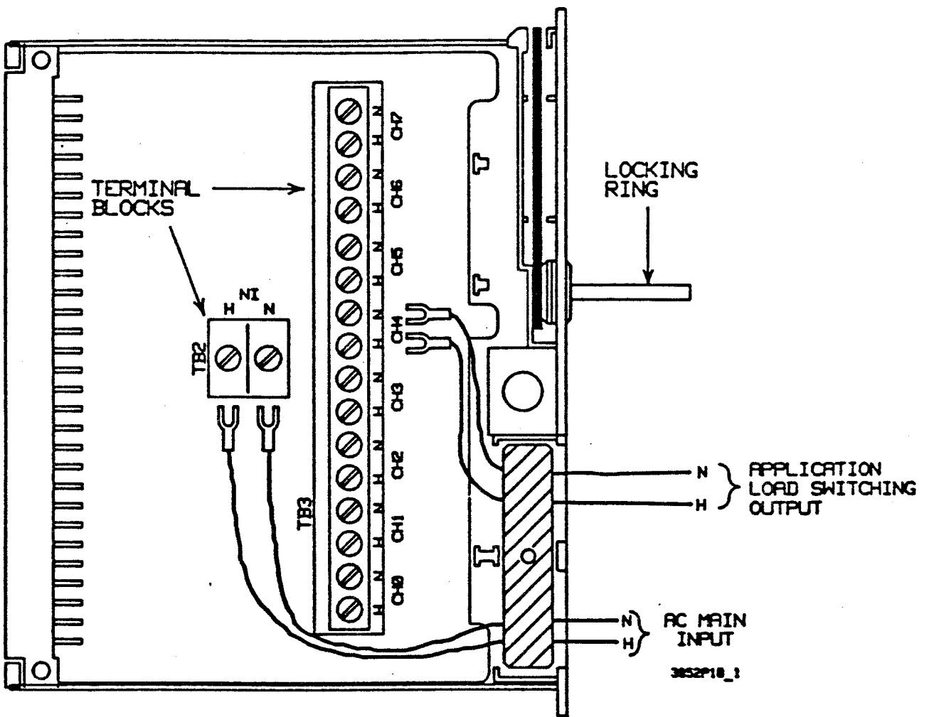
Figure 18-1. Field Wiring Interconnect Diagram
