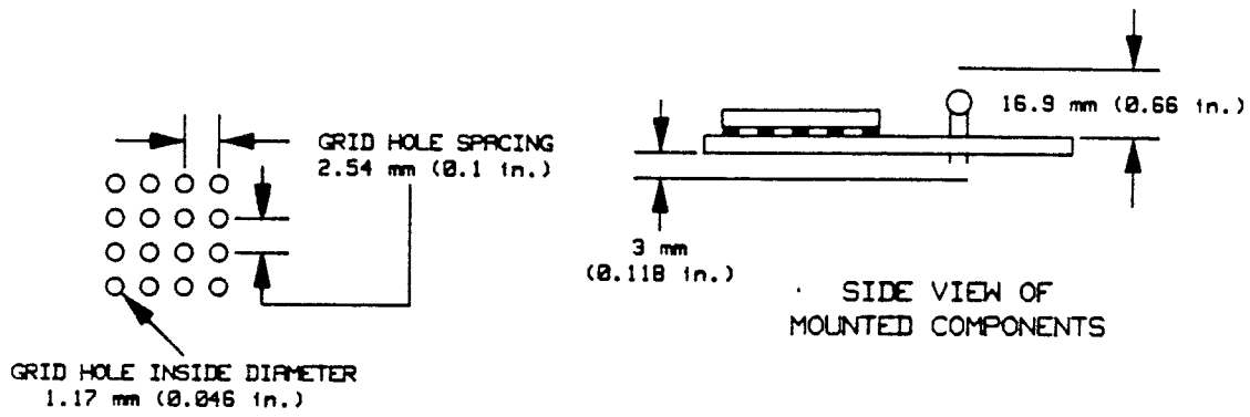
Figure 19-14. Component Height/Protrusion Restrictions
