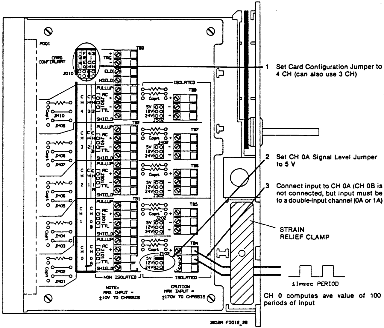
Figure 12-28. Example: Measure Average Period
