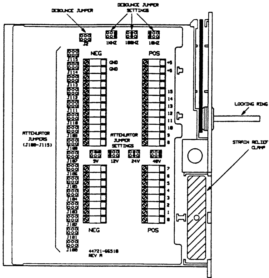
Figure 13-2. 16-Channel Terminal Module
