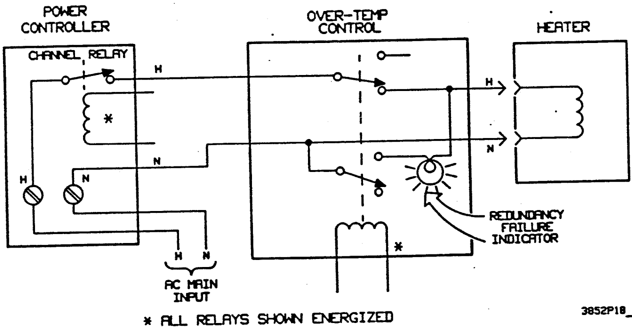
Figure 18-2. Redundant Switching Control, Simplified Block Diagram
