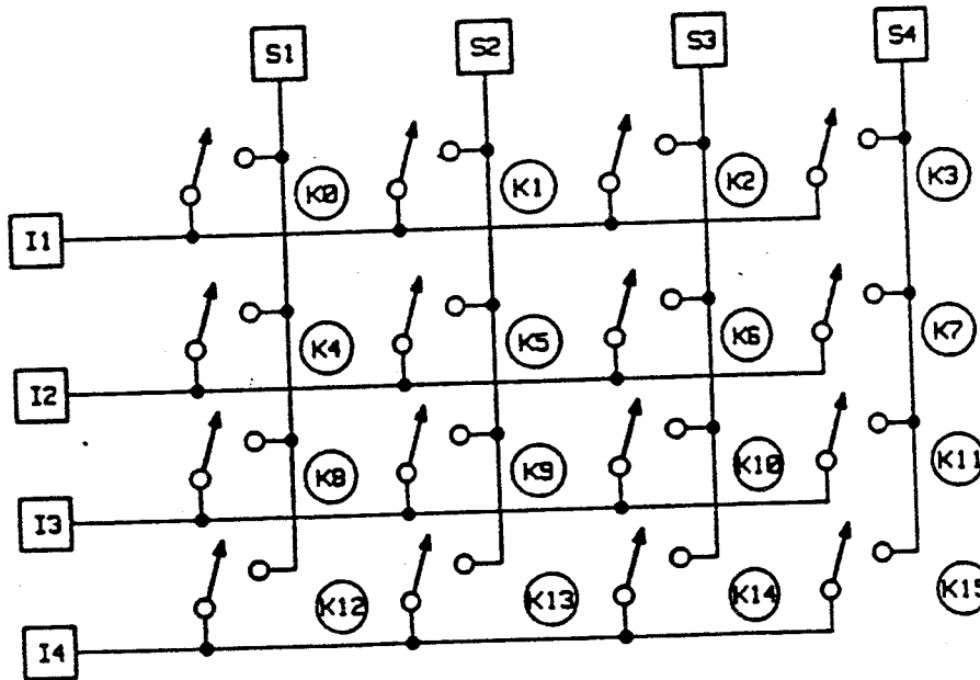
MATRIX SWITCHING
