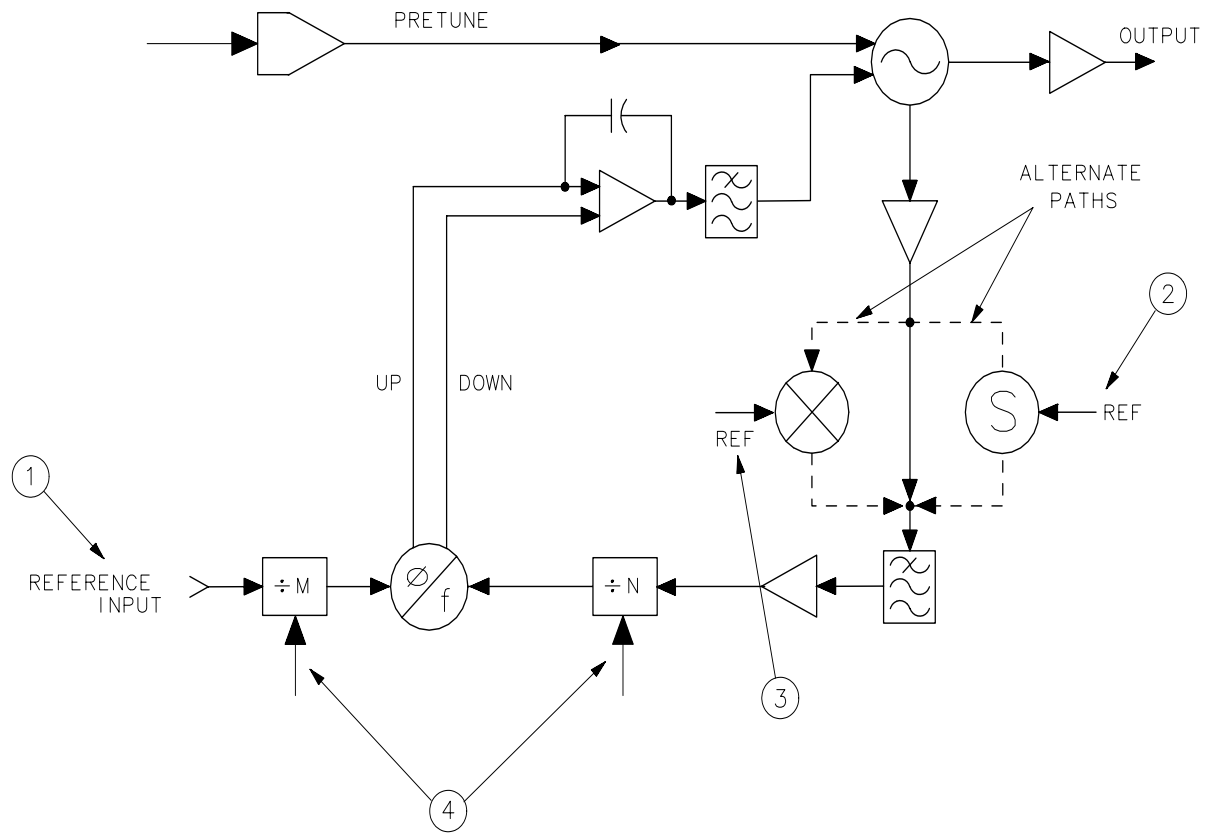
Figure 10-5 PLL Locked at Wrong Frequency
