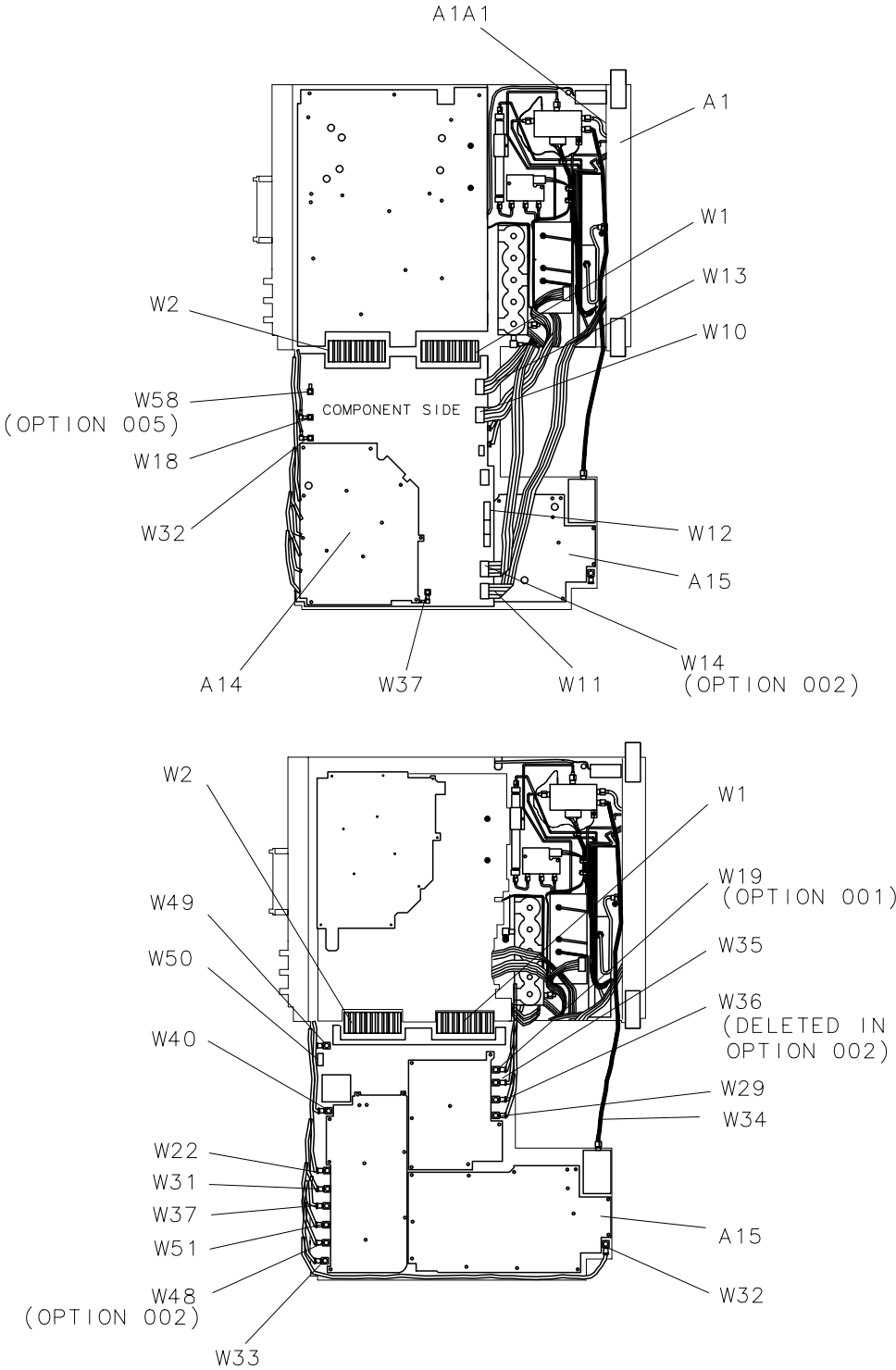
Figure 3-26 A14 and A15 Assembly Cables
