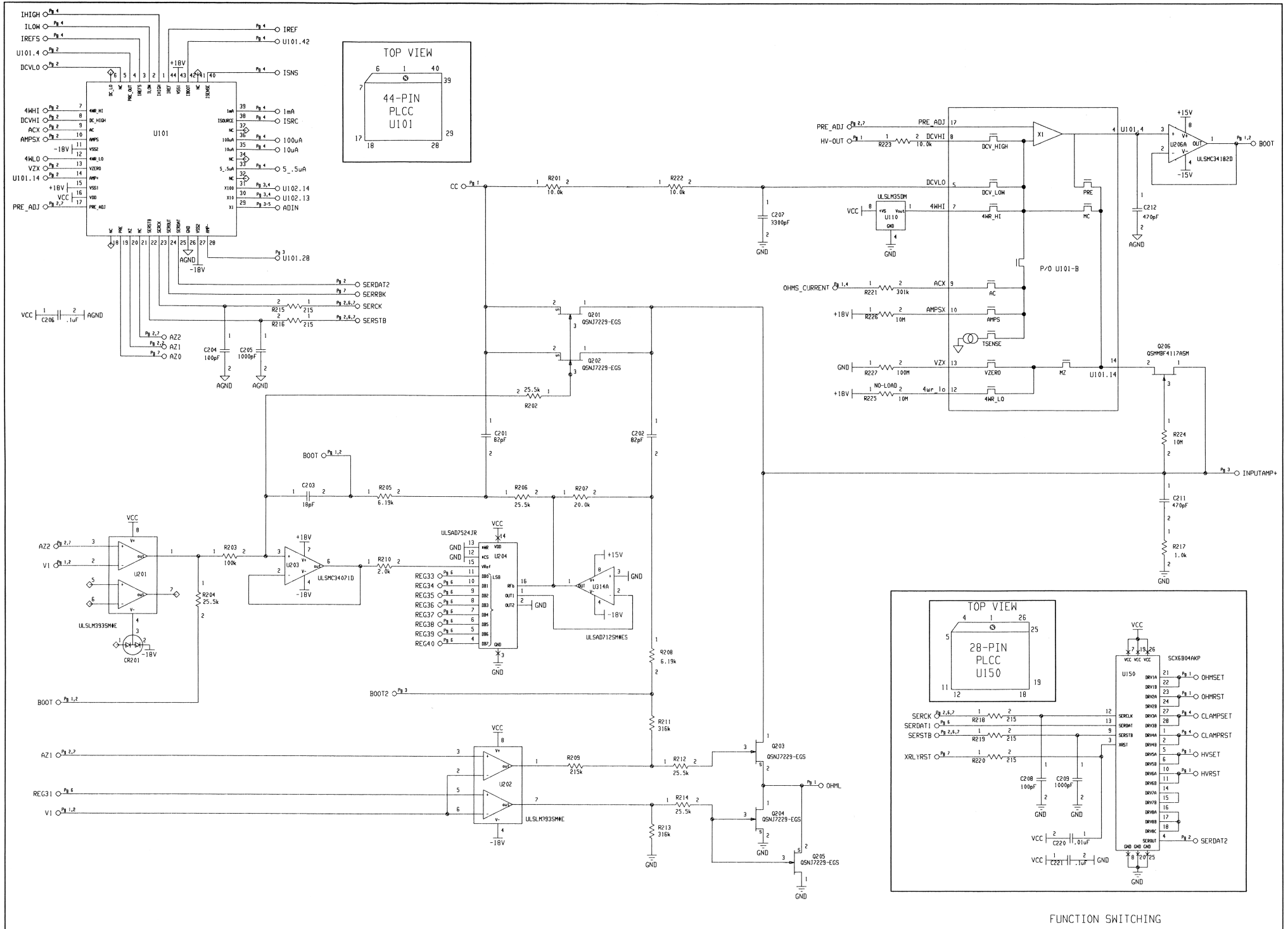
Function Switching Schematic
