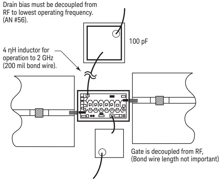
Figure 3. Assembly diagram
