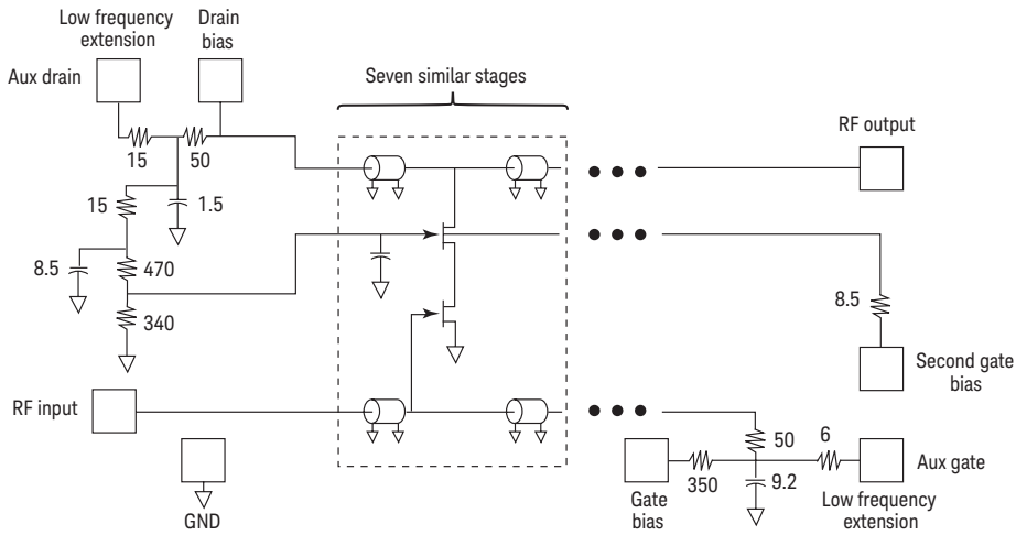
Figure 1. Schematic
