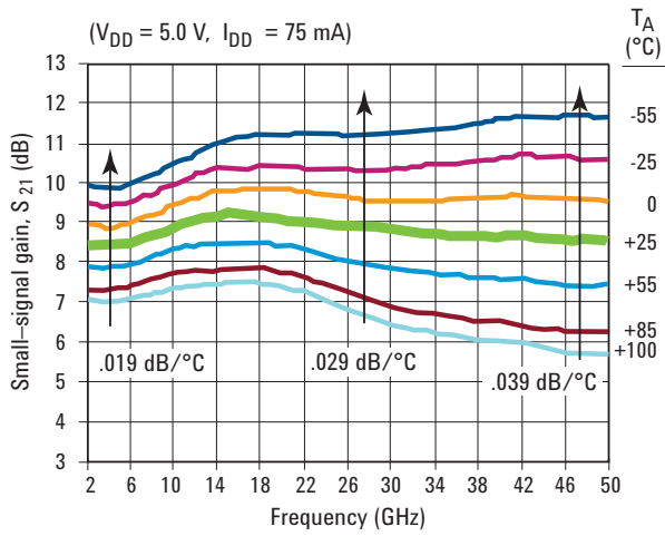
Figure 6. Typical Small-signal gain vs. Temperature
