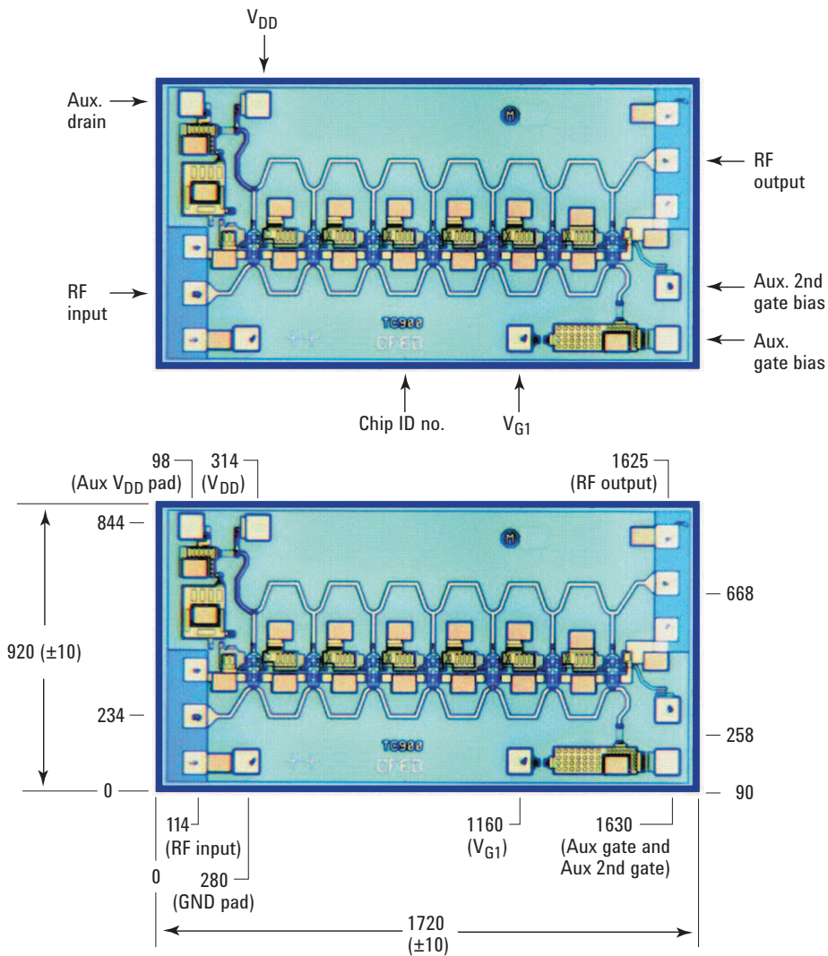
Figure 2. Bond pad locations
