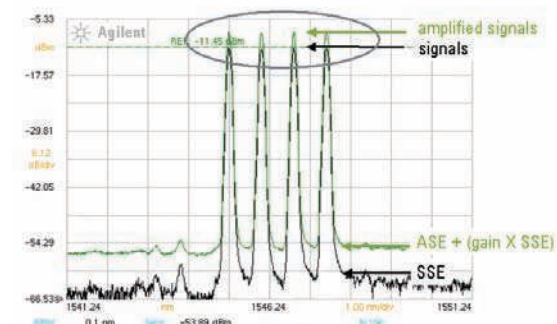
Wavelength flatness preserves multichannel signal flatness for EDFA test.
