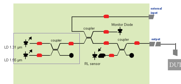
Return Loss Module, Optical Assembly
