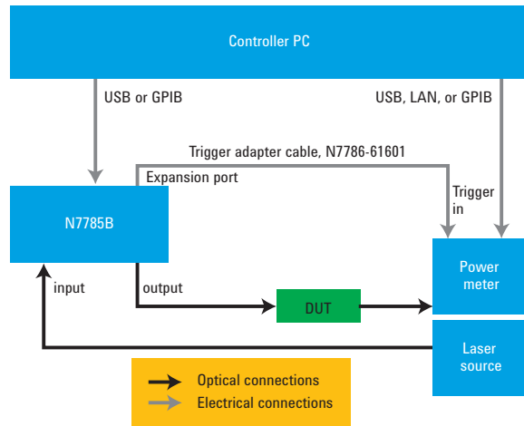
Figure 4: A typical setup for synchronized all-states measurement.
