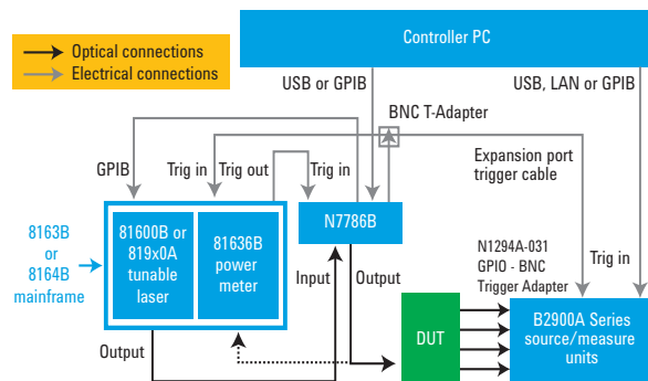
Figure 1: Setup example for measuring optoelectrical devices with the B2900A.
