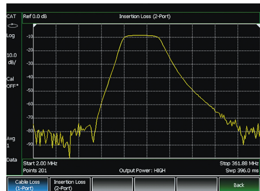
Insertion loss display
