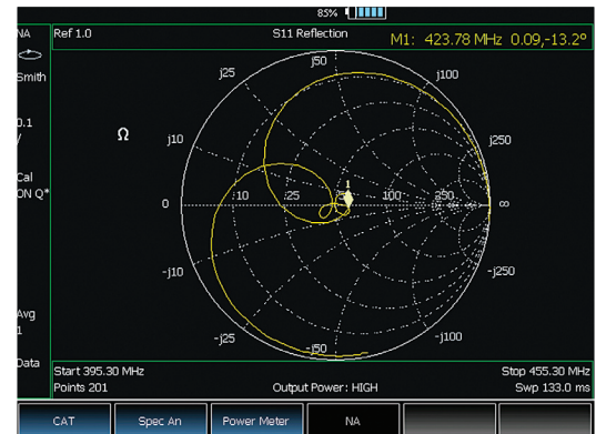
Smith chart display
