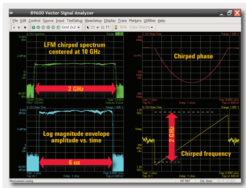
FIGURE 3: Shown here is a wide-bandwidth LFM chirped Radar measurement using the VSA software on the 90000X oscilloscope.
