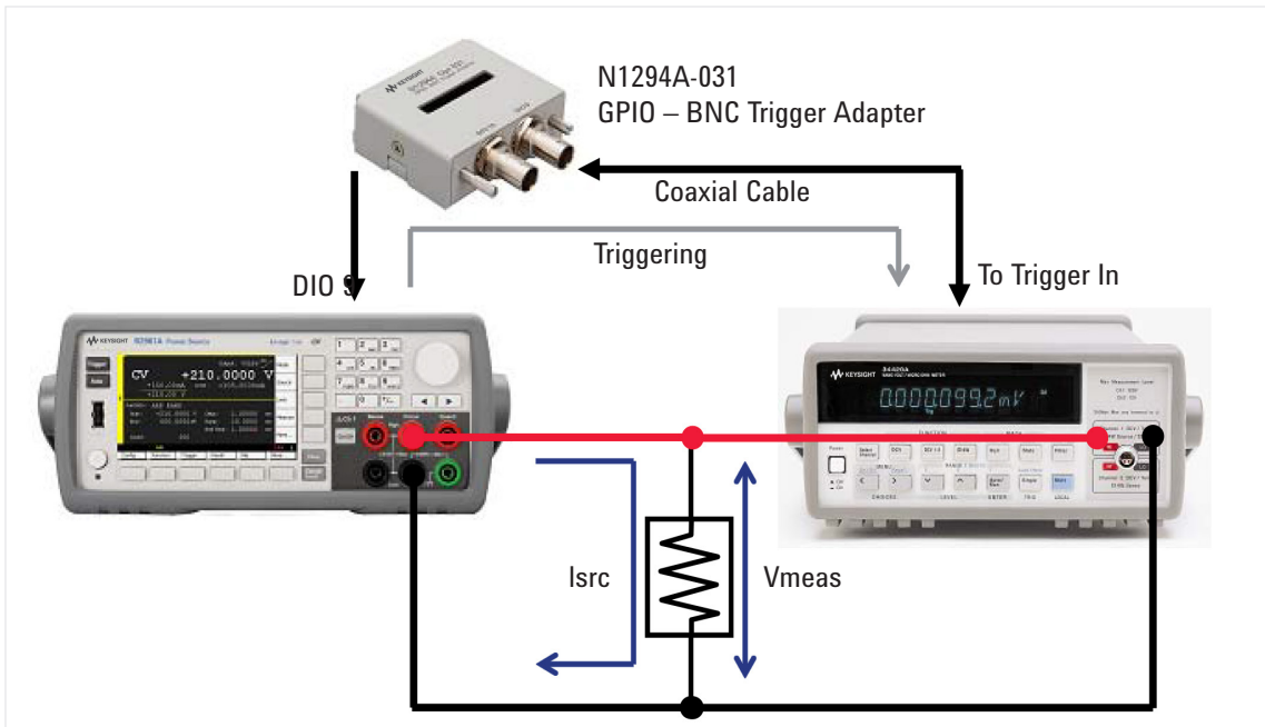
Figure 3. Diagram of the B2961A and 34420A low resistance measurement solution
