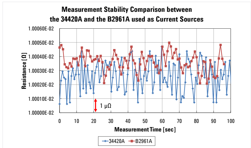
Figure 6. Measurement stability comparison between the 34420A and the B2961A used as current sources
