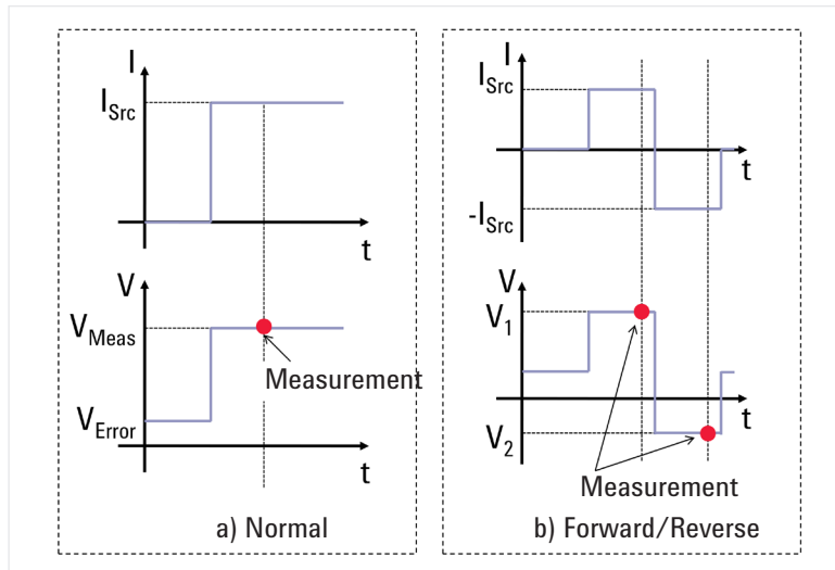
Figure 4. Technique to eliminate the measurement error caused by electro motive force
