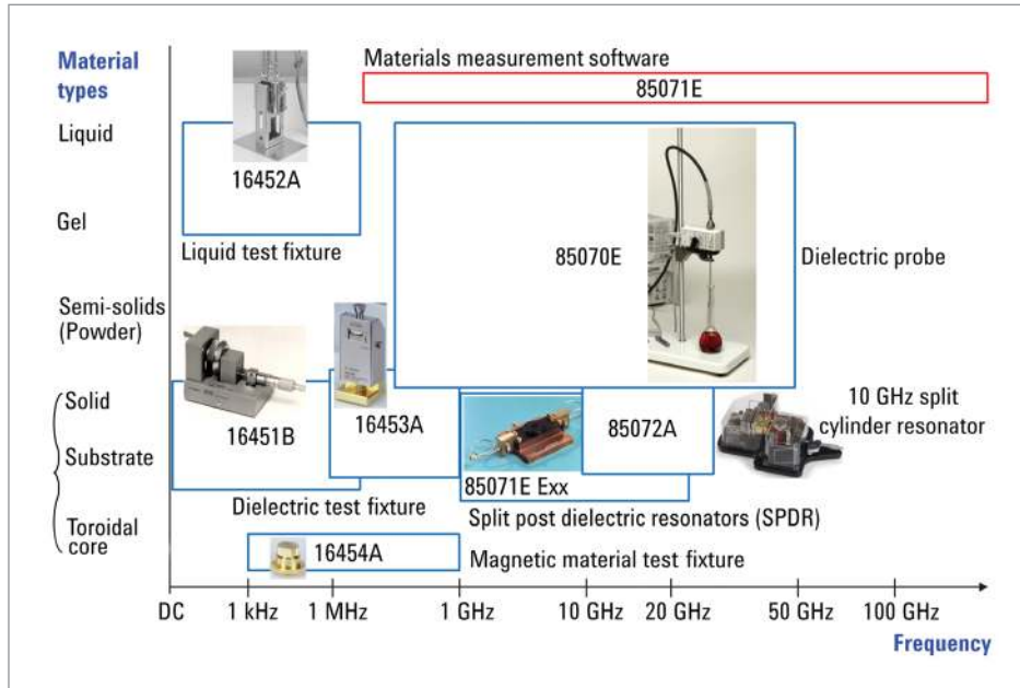
Figure 2. Keysight materials measurement fixtures
