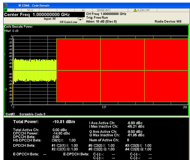
Figure 1. M9073A W-CDMA/HSPA+ X-Series measurement application for modular instruments.
