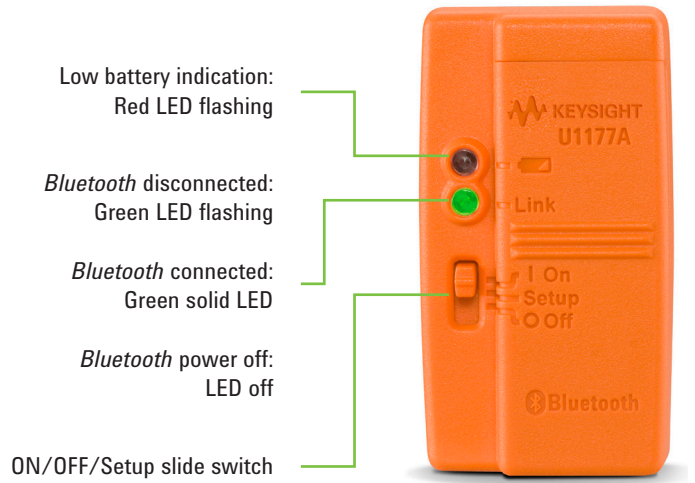
Figure 5. The U1177A as illustrated
