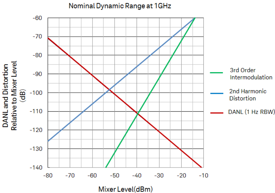
Figure 1. Nominal dynamic range for Band 0, for second and third order distortion, 10 MHz to 3 GHz
