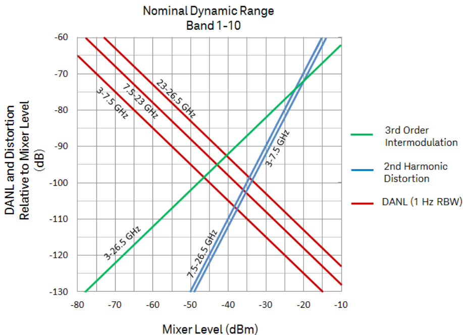
Figure 2. Nominal dynamic range, for second and third order distortion, 3 GHz to 26.5 GHz
