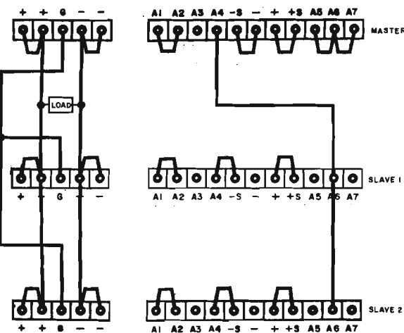
B. THREE POWER SUPPLIES
