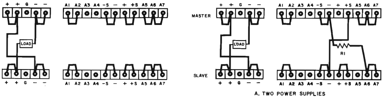
FIGURE 3-9. NORMAL SERIES STRAPPING PATTERN
