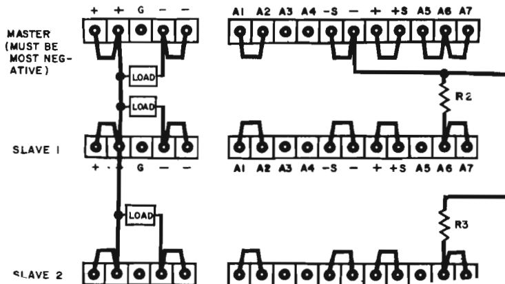
FIGURE 3-12. AUTO-TRACKING STRAPPING PATTERN
