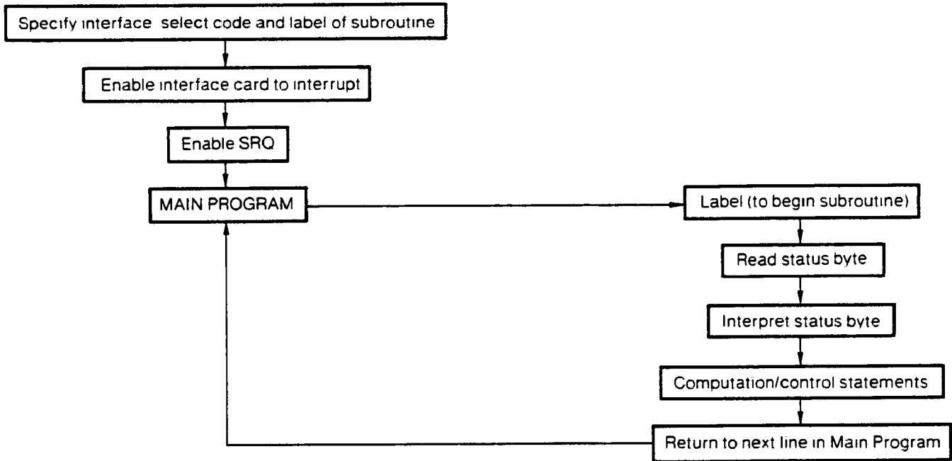
FIGURE 4-5. INTERRUPT SETUP
