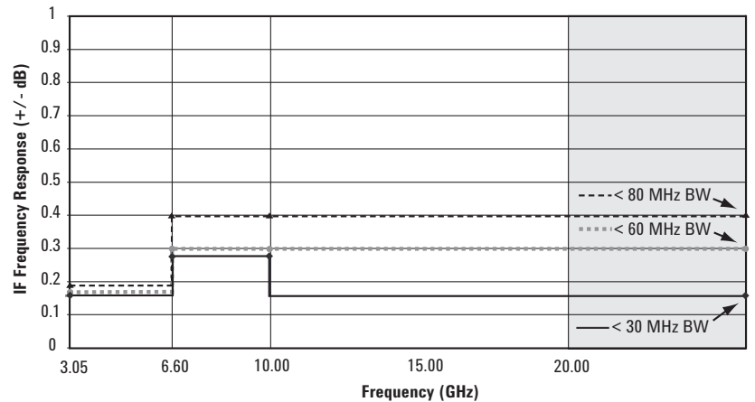
Figure 3: 40/80 MHz BW digitizers typical IF frequency response > 3 GHz (with Option 123).
