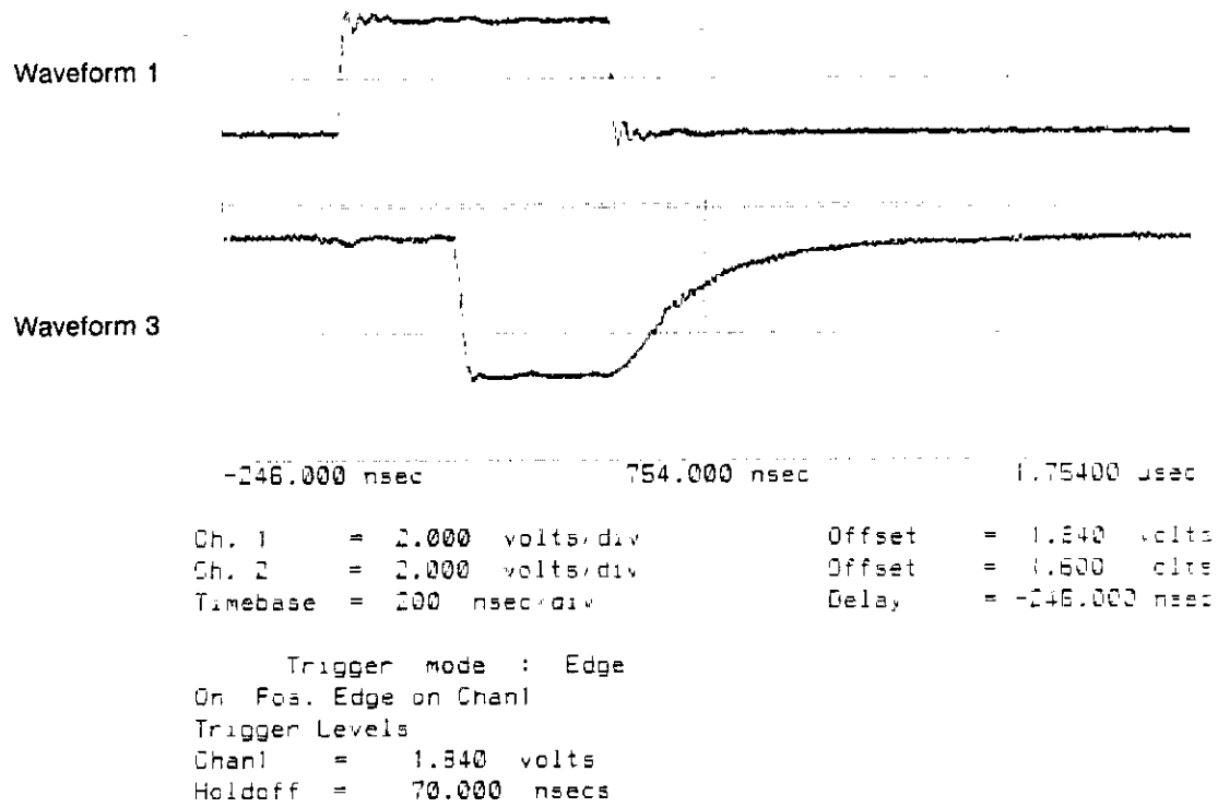
Figure 6D-2. Waveform Numbers 1 and 3.
