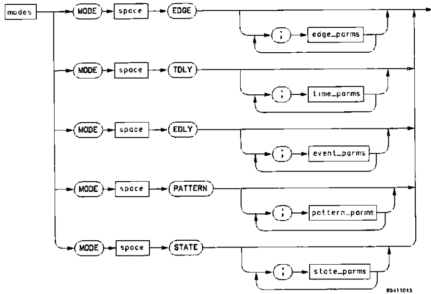
Figure 10-12 Trigger Subsystem Commands
