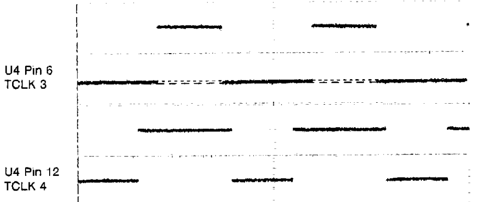
Figure 6E-96 Loop 59 Troubleshooting Waveforms at U4 Pins 1 and 17.
