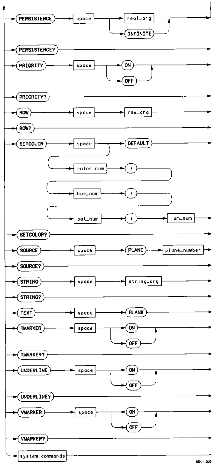
Figure 10-5. Display Subsystem Commands
