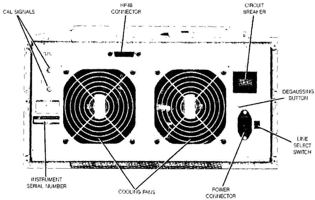
Figure 4-1 HP 54110D Rear Panel
