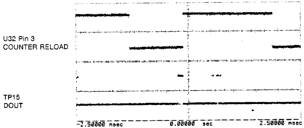
Figure 6E-59. Loop 51 Troubleshooting Waveforms at U4 Pin 8 and U6 Pin 2.
