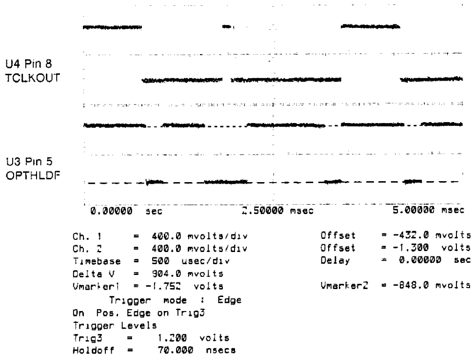
Figure 6E-37 Loop 45 Troubleshooting Waveforms at U4 Pin 8 and U3 Pin 5.
