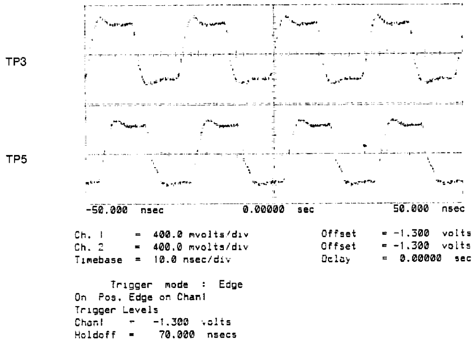
Figure 6E-3. Timebase Troubleshooting Waveforms at TP3 and TP5.
