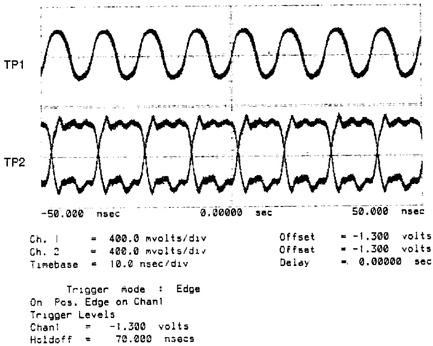
Figure 6E-1. Timebase Troubleshooting Waveforms at TP1 and TP2.
