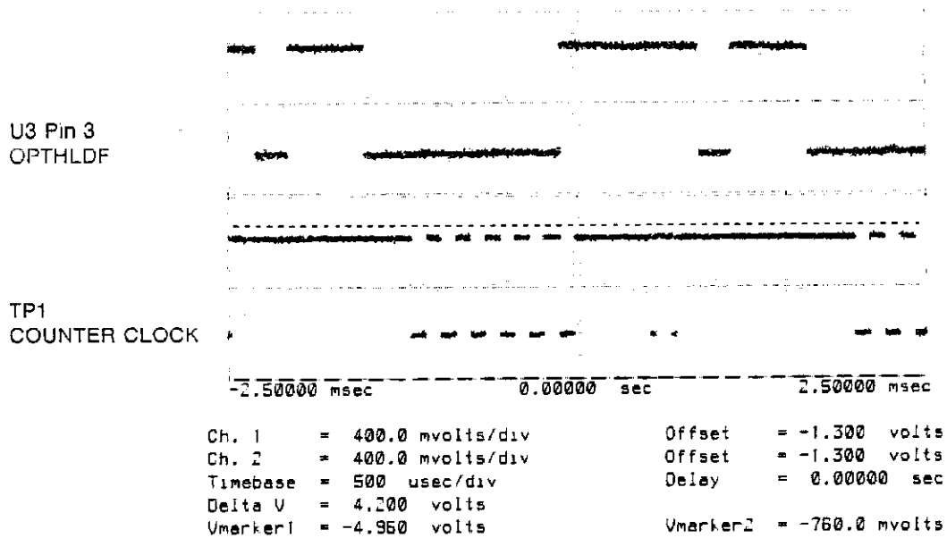
Trigger mode : Edge On Pos. Edge on Trig3 Trigger Levels Trig3 = 1.200 volts Holdoff = 70.000 nsecs Figure 6E-61. Loop 51 Troubleshooting Waveforms at U3 Pin 3 and TP1.
