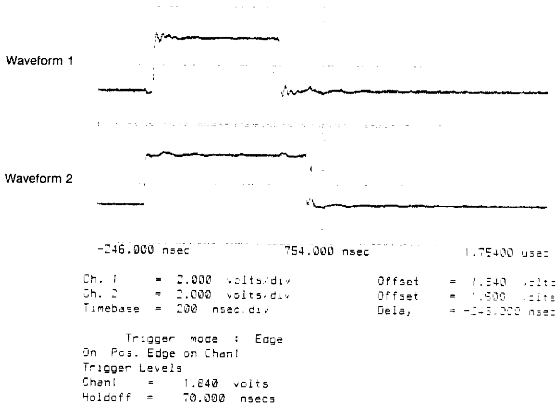
Figure 6D-1. Waveform Numbers 1 and 2.
