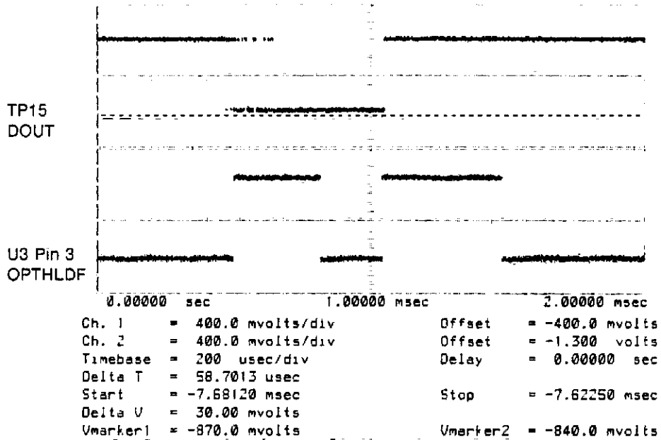
Figure 6E-67 Loop 57 Troubleshooting Waveforms at TP1 and U4 Pin 8.
