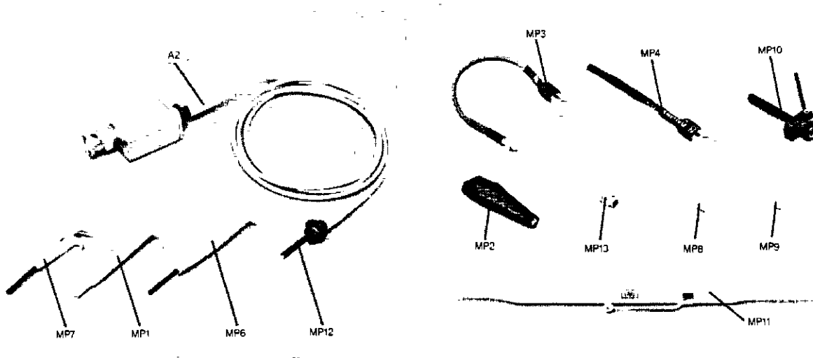
Figure 7C-1. HP 54003A Active Probe Parts, 54001-69501.
