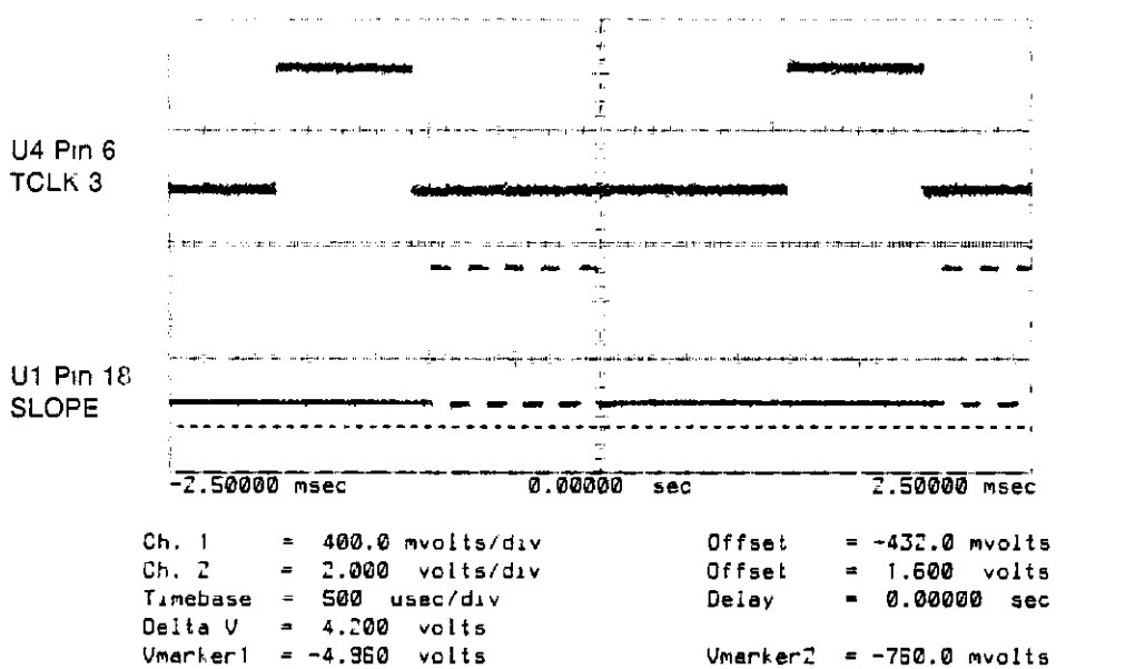
Figure 6E-57. Loop 50 Troubleshooting Waveforms at U3 Pin 3 and TP1.
