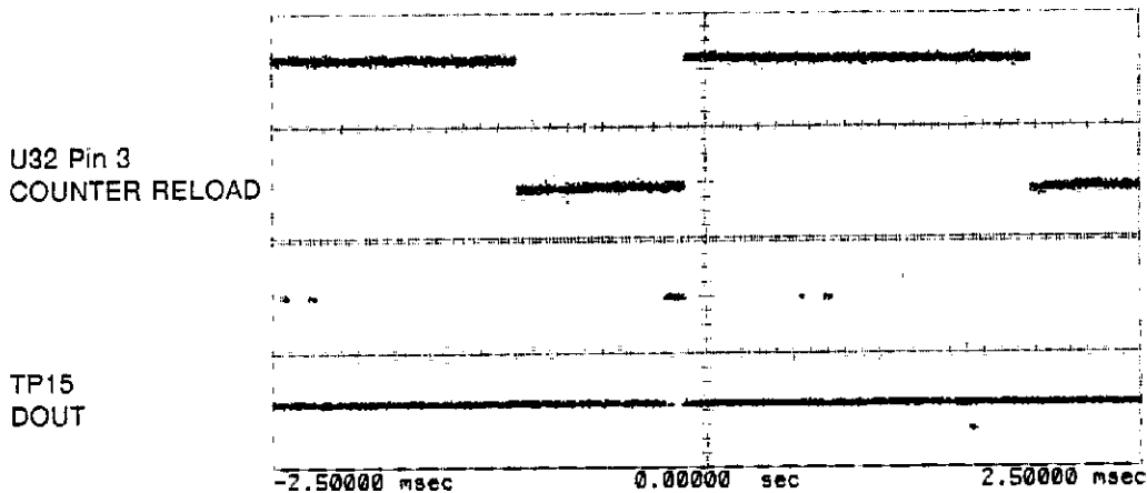
Figure 6E-55. Loop 50 Troubleshooting Waveforms at U4 Pin 8 and U6 Pin 2.
