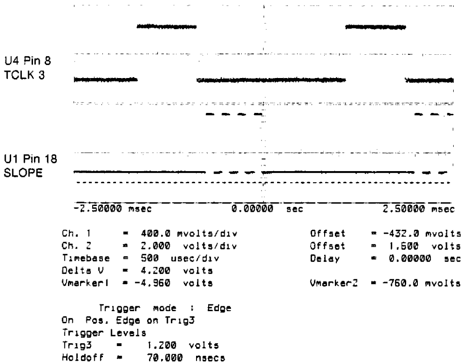
Figure 6E-54. Loop 49 Troubleshooting Waveforms at U4 Pin 8 and U1 Pin 18.
