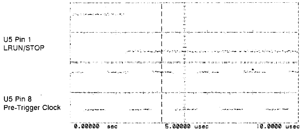
Figure 6E-15. Loop 18 Troubleshooting Waveforms at U5 Pin 1 and TP9.
