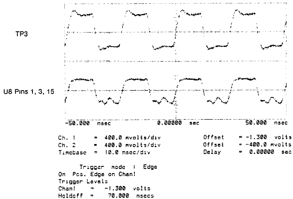
Figure 6E-4. Timebase Troubleshooting Waveforms at TP3 and U8 Pins 1, 3, 15.
