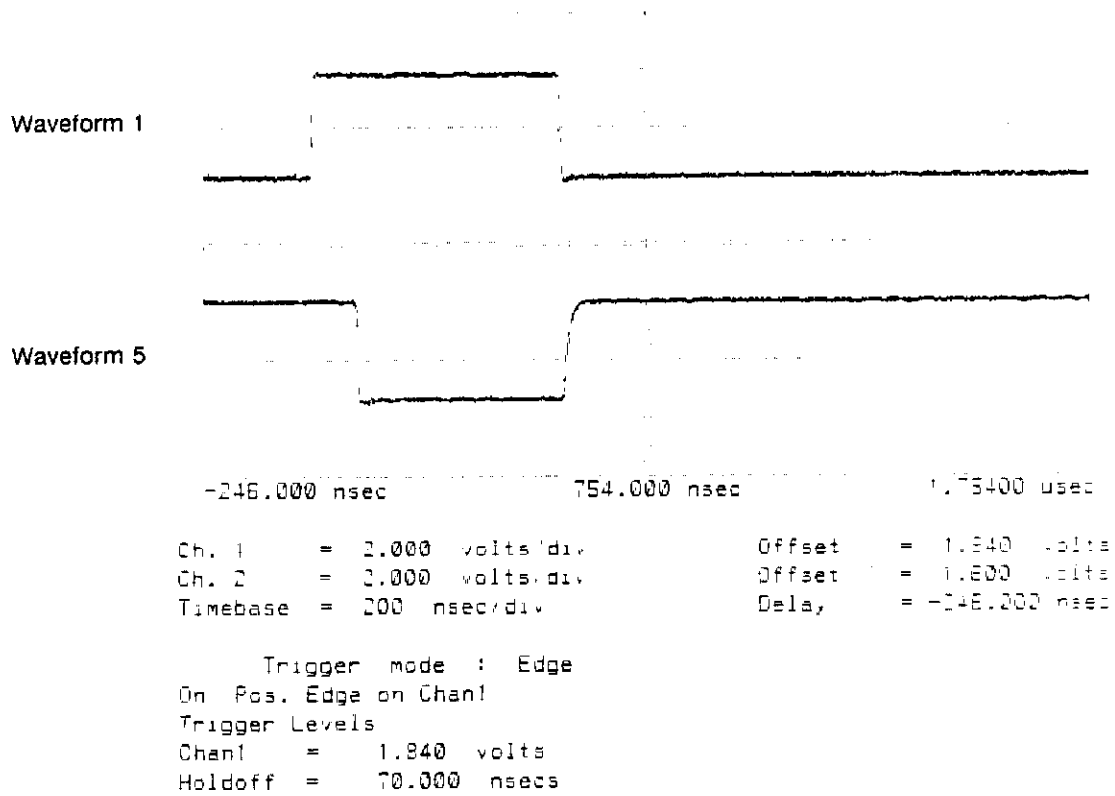
Figure 6D-4. Waveform Numbers 1 and 5.
