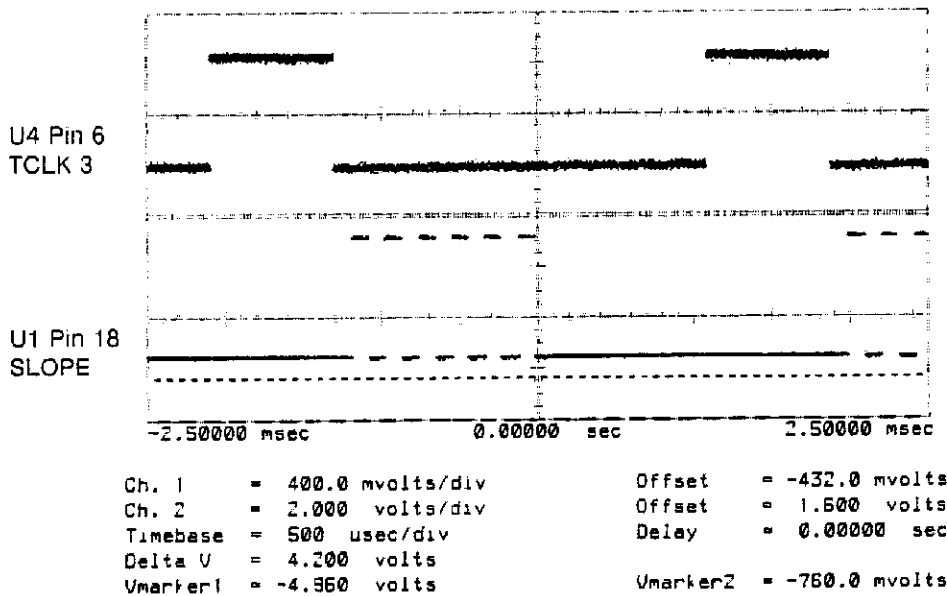
Trigger mode : Edge On Pos. Edge on Trig3 Trigger Levels Trig3 = 1.200 volts Holdoff = 70.000 nsecs Figure 6E-62. Loop 51 Troubleshooting Waveforms at U4 Pin 6 and U1 Pin 18.
