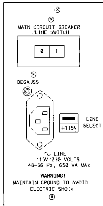
Figure 4-2. Power Module
