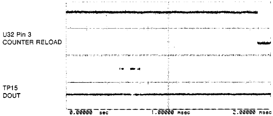
Figure 6E-67. Loop 53 Troubleshooting Waveforms at U4 Pin 8 and U6 Pin 2.
