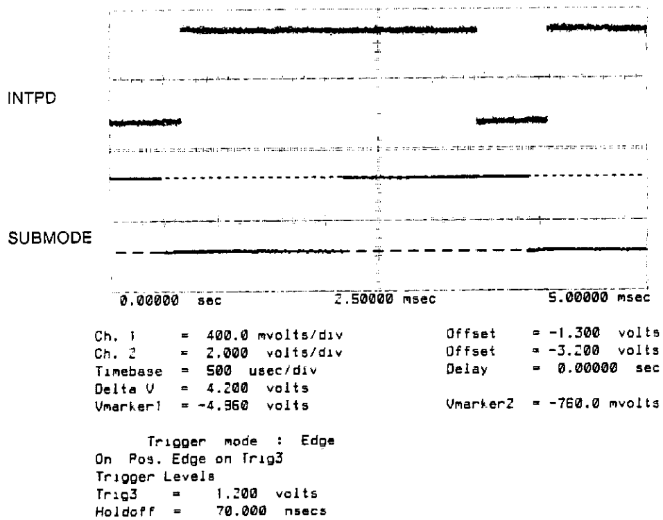
Figure 6E-38. Loop 45 Troubleshooting Waveforms at INTPD and SUBMODE.
