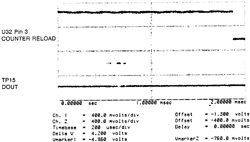
Trigger mode : Edge On Pos. Edge on Trig3 Trigger Levels Trig3 = 1.200 volts Holdoff = 70.000 nsecs Figure 6E-72. Loop 54 Troubleshooting Waveforms at U32 Pin 3 and TP15.
