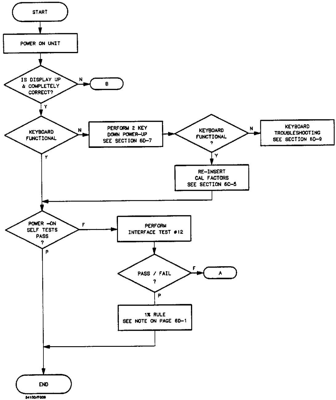
Figure 6D-11. Troubleshooting Tree Number 1.
