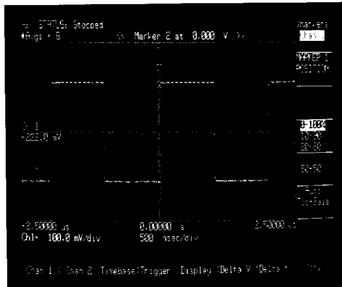
Figure 7-4. Auto Top-Base Voltage Measurement
