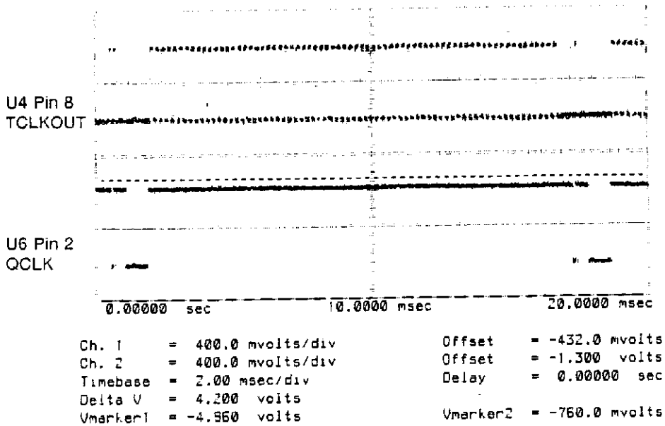
Trigger mode : Edge On Pos. Edge on Trig3 Trigger Levels Trig3 = 1.200 volts Holdoff = 70.000 nsecs Figure 6E-71. Loop 54 Troubleshooting Waveforms at U4 Pin 8 and U6 Pin 2.
