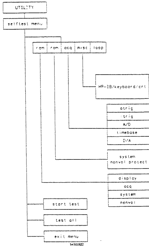
Figure 12-3. Self-Test Menu
