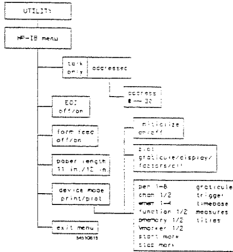
Figure 12-2. HP-IB Menu
