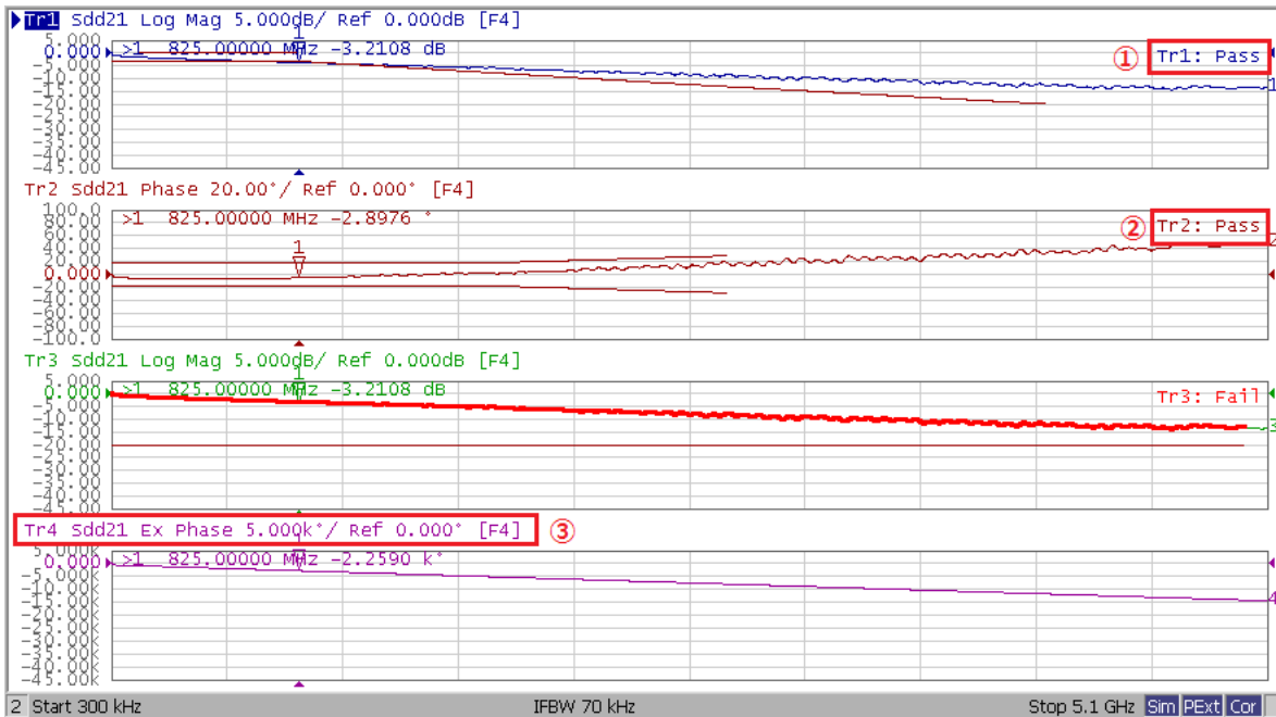
Figure 5-9 Attenuation and Phase Measurement Example
