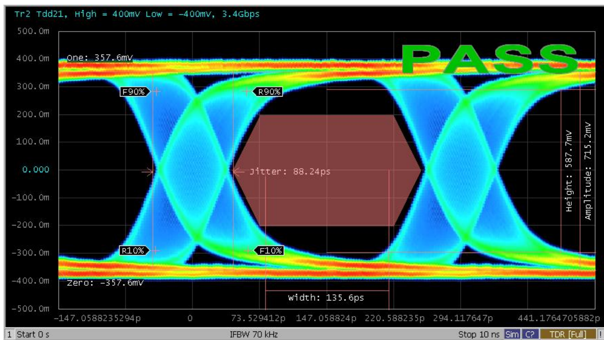
Figure 5-5 The eye diagram of cable input signal with adjusted jitter.
