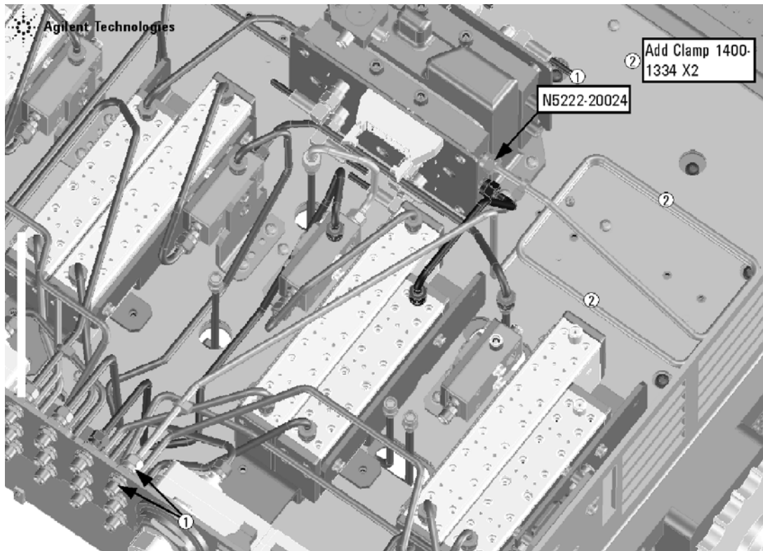
Figure 5 Location of Cable Clamps to Secure W49
