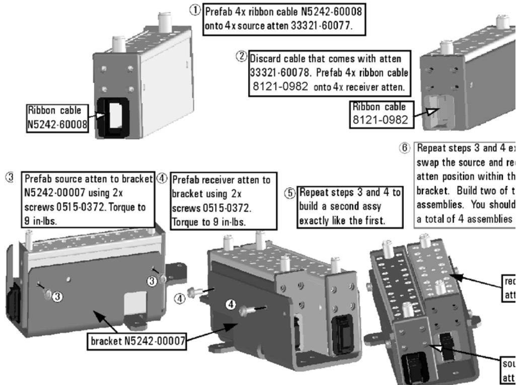
Figure 1 Attenuator Assembly
