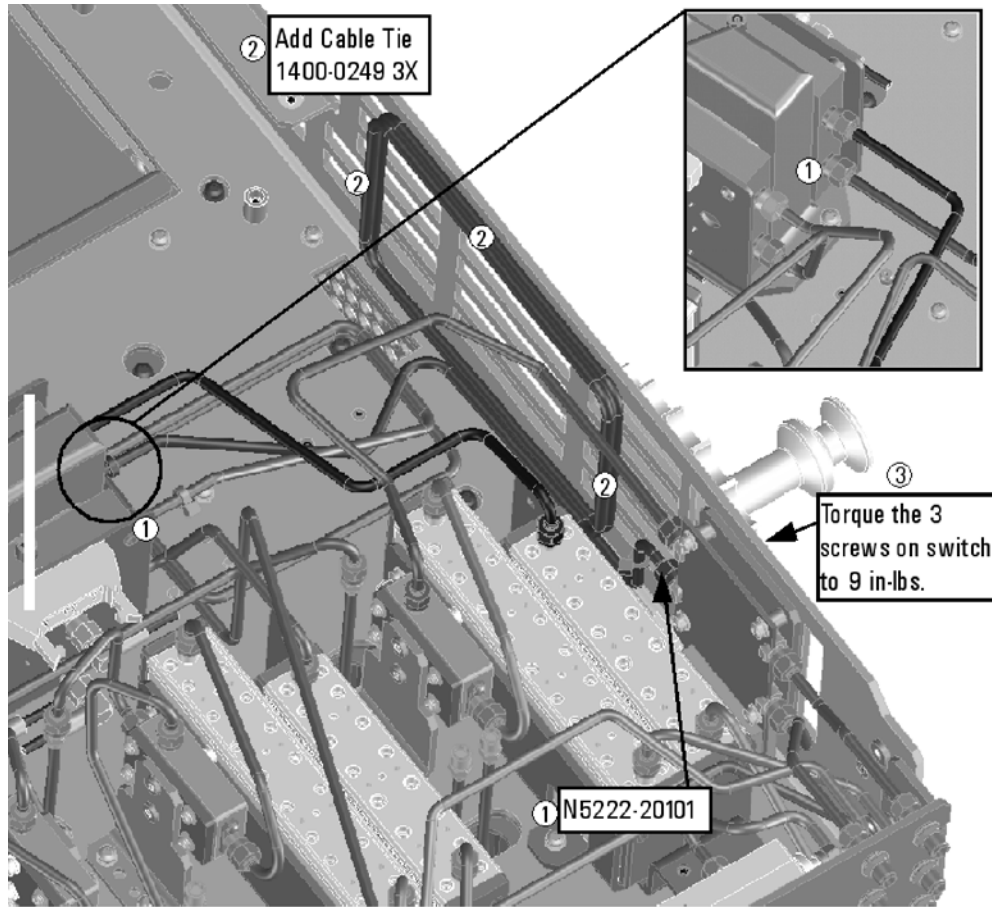
Figure 6 Location of Cable Ties to Secure W48
