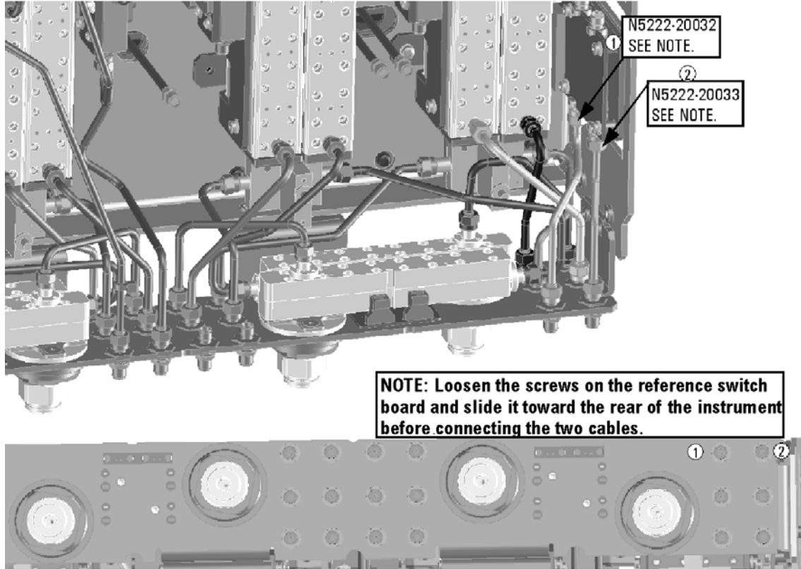
Figure 4 Information to Secure W35 and W36
