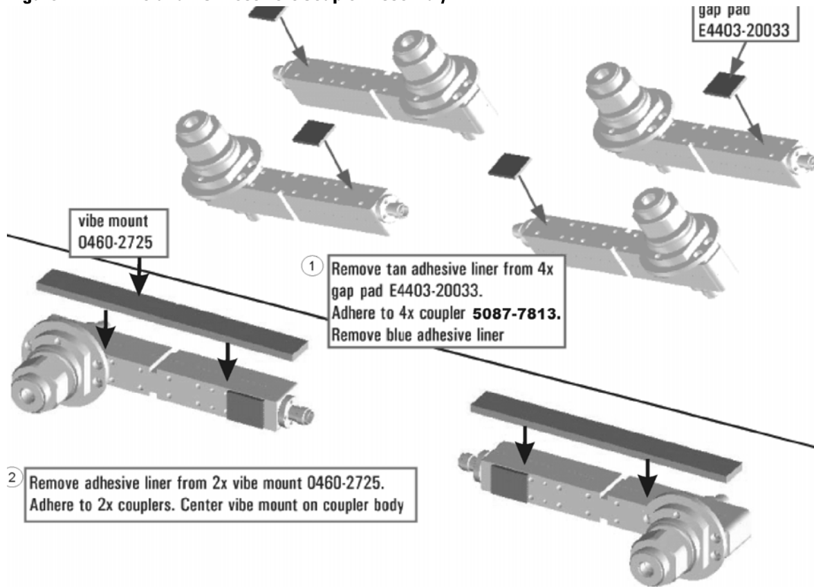
Figure 7 A29 and A32 Test Port Coupler Assembly
