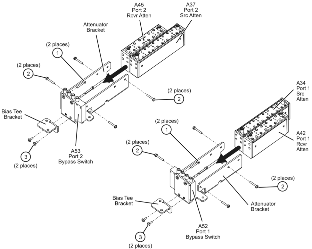
Figure 5 Attenuators and Bypass Switches Assembly
