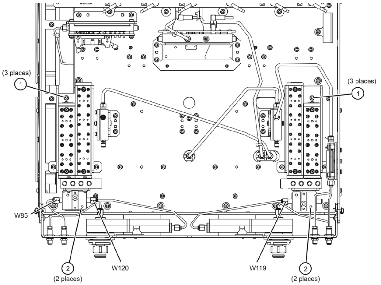
Figure 6 New Brackets Installation into the Analyzer
