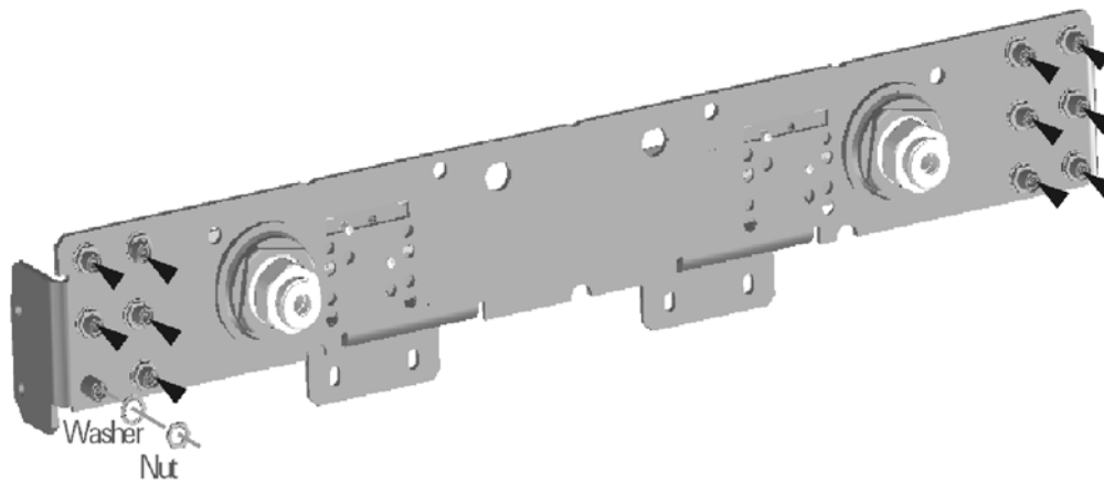
Figure 11 Bulkhead Connectors Installation
