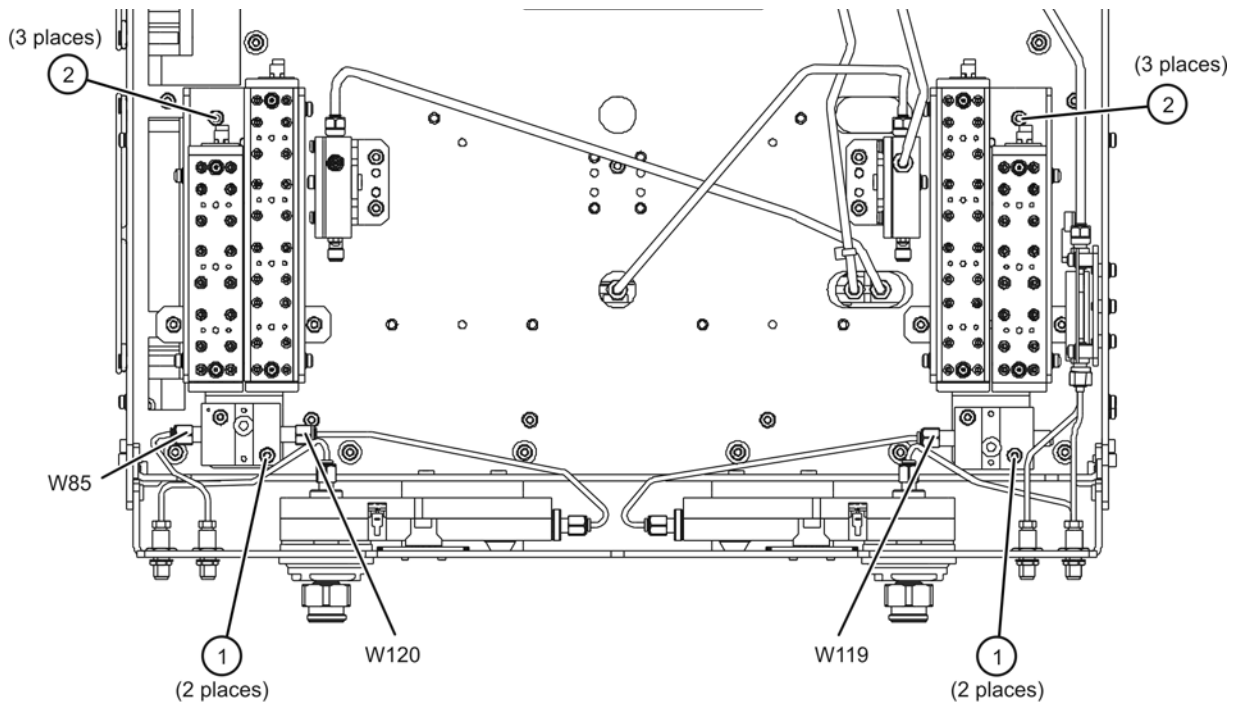
Figure 4 Existing Attenuators and Brackets Removal
