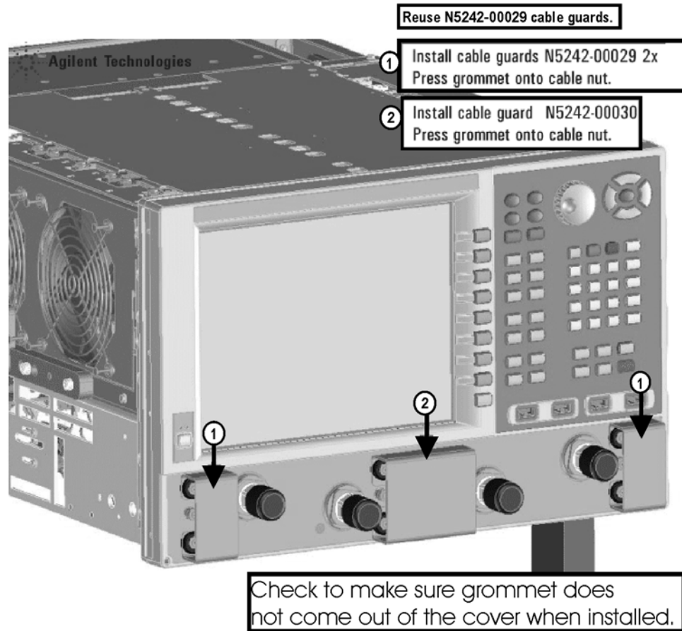
Figure 31 Install the Cable Guards Over the Front Panel Jumpers
