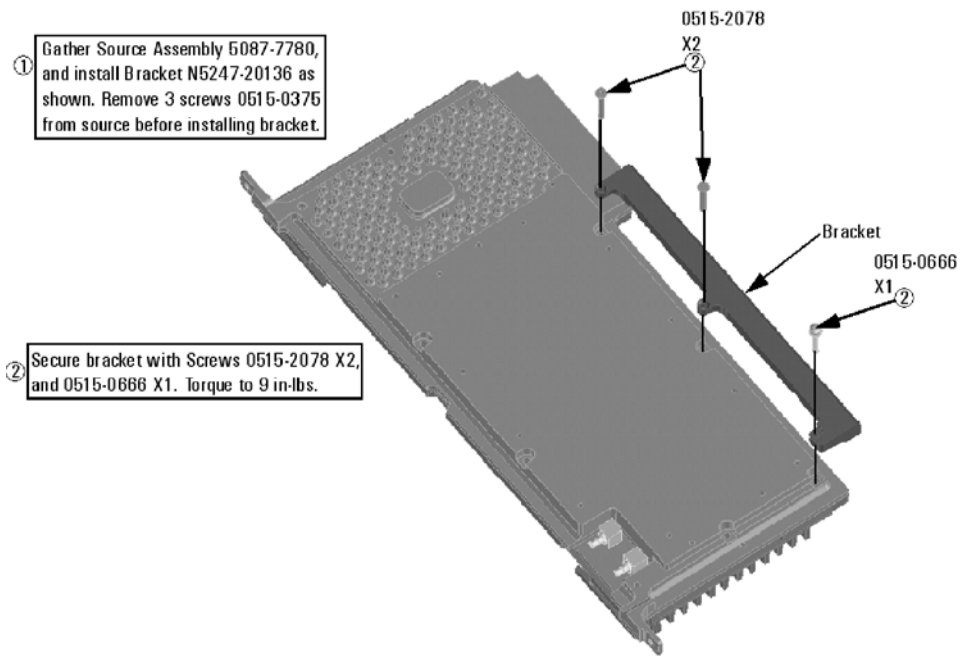
Figure 7 A10 Source 2 Assembly Bracket Installation
