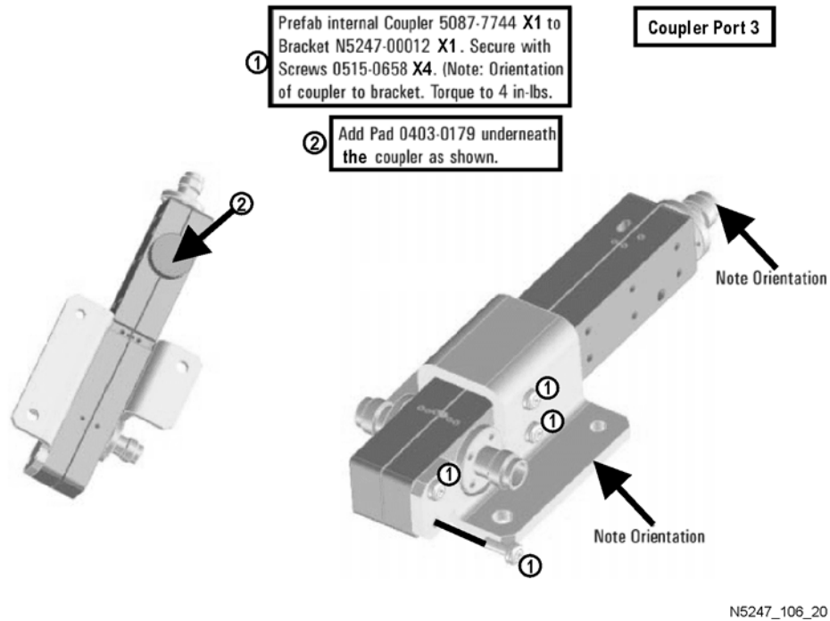
Figure 20 A31 Reference Coupler Assembly
