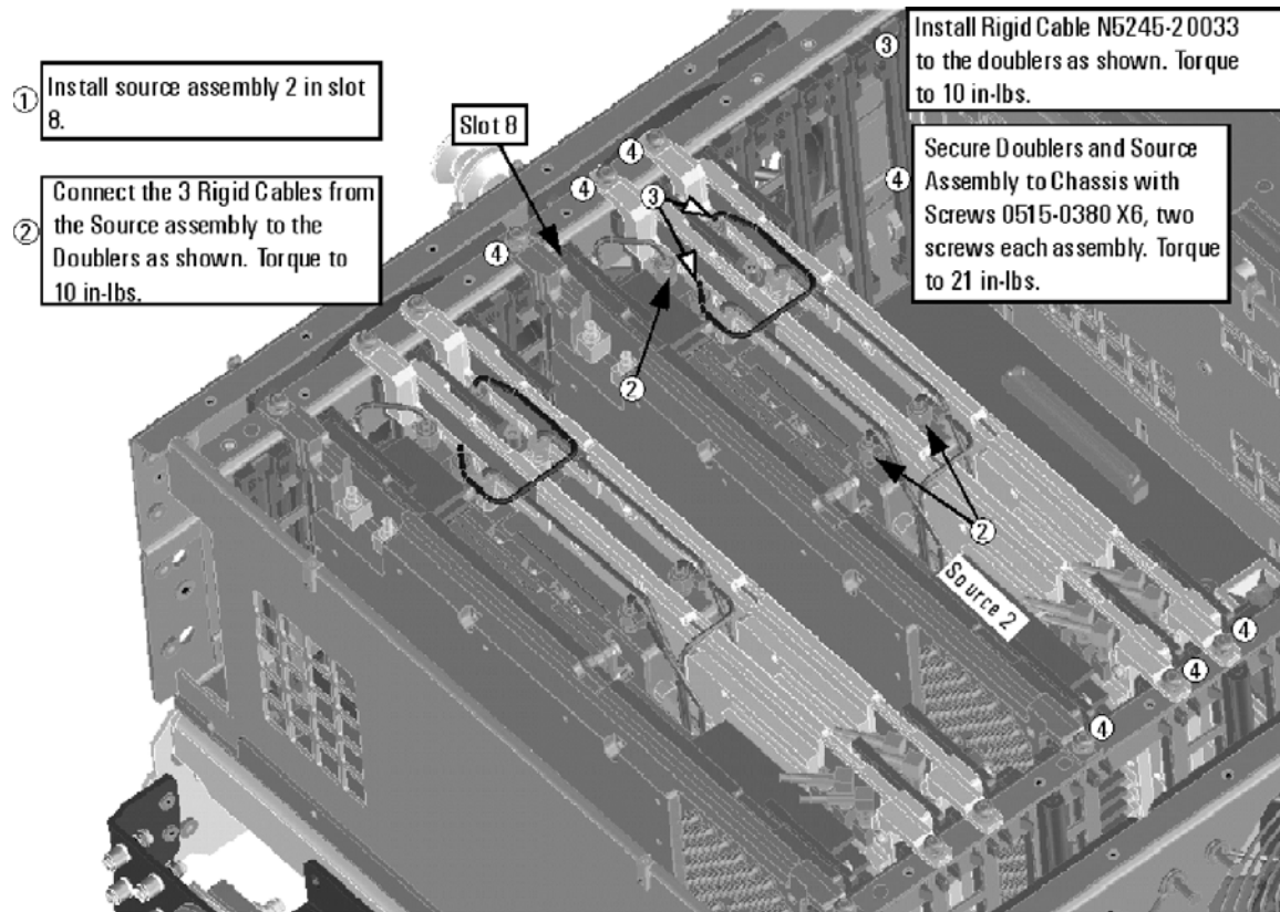
Figure 13 A10 Source 2 Assembly Installation
