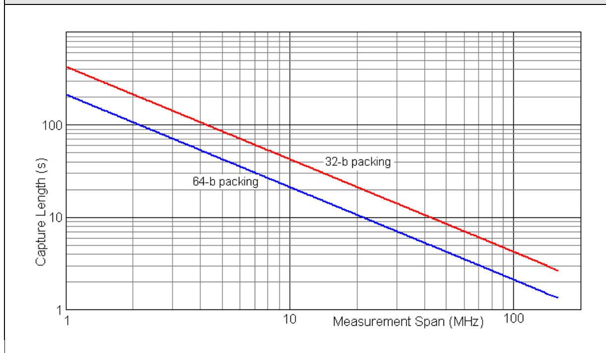
Capture Time [Plot]
