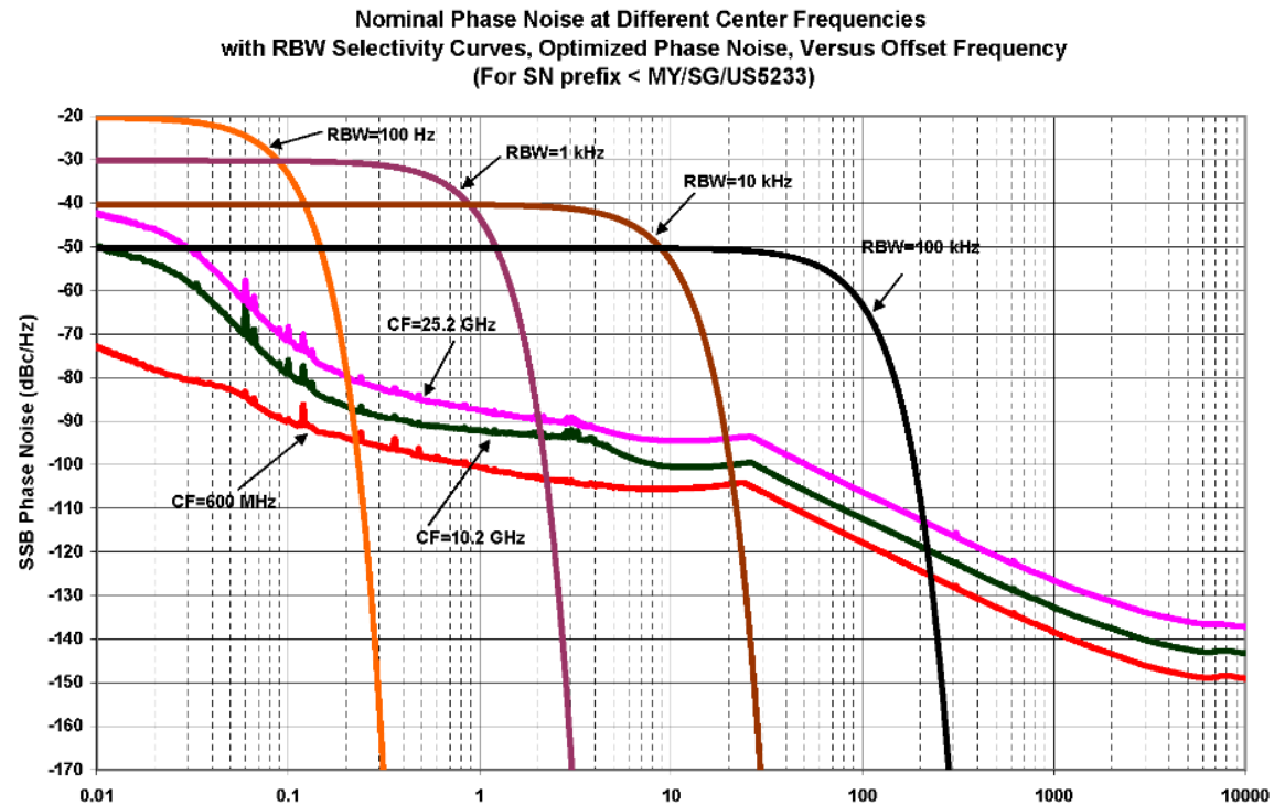
Nominal Phase Noise at Different Center Frequencies [Plot] (SN prefix <MY/SG/US5233)
