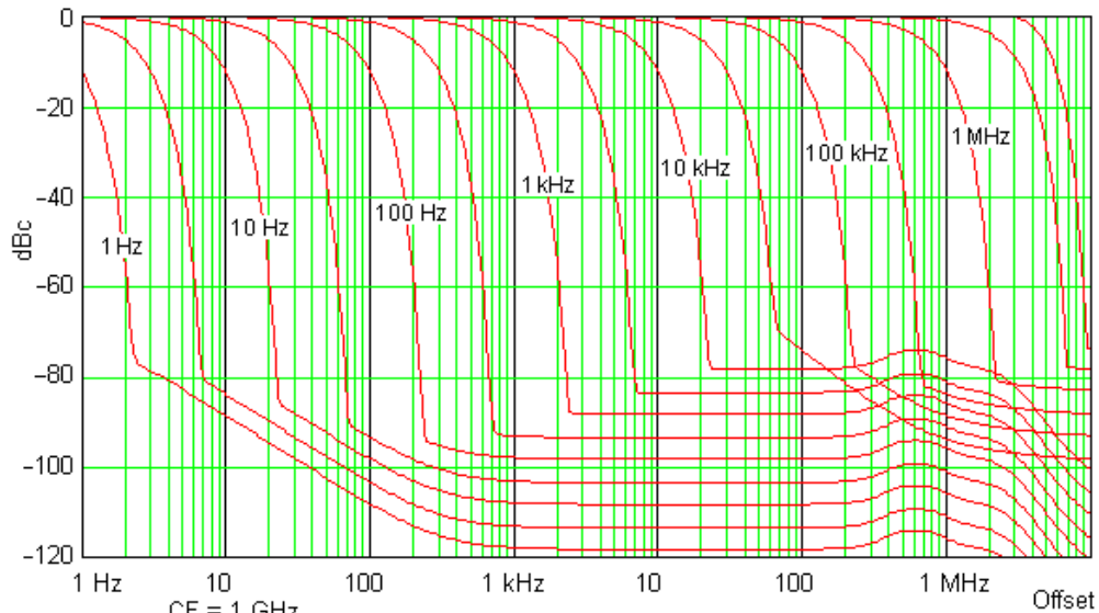
Nominal Dynamic Range vs. Offset Frequency vs. RBW [Plot] (SN prefix \geq MY/SG/US5233, ship standard with N9020A-EP2)
