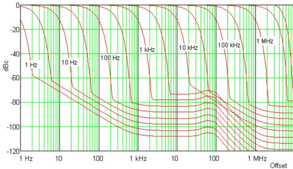
Nominal Dynamic Range vs. Offset Frequency vs. RBW [Plot] (SN prefix <MY/SG/US5233)
