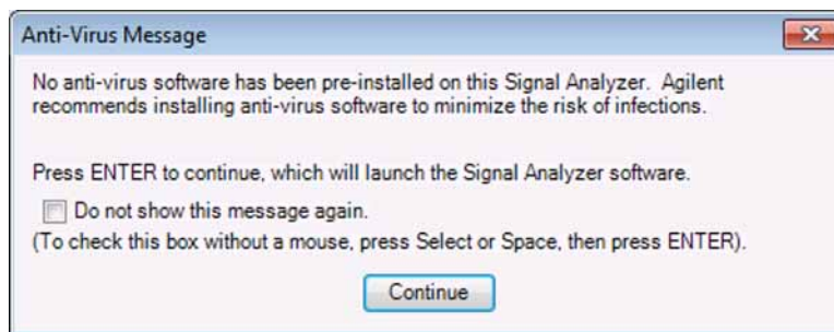
Figure 5 Anti-Virus Message
