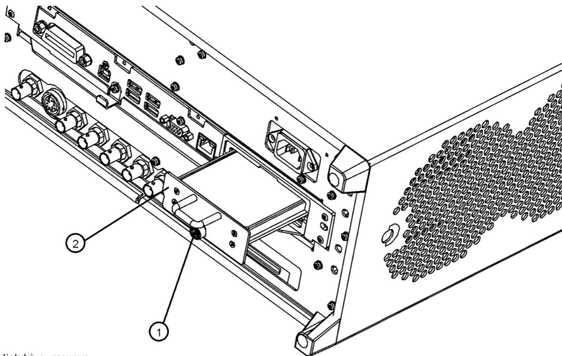
Figure 8 Replacing the Disk Drive Carrier Assembly
