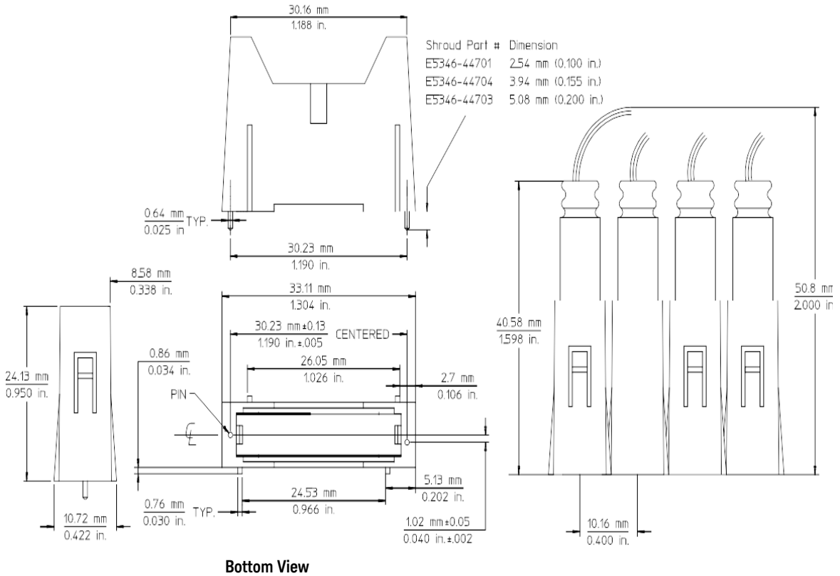
Figure 5 Support shroud dimensions for the MICTOR 38-pin connector
