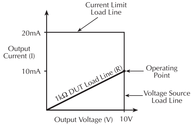
Figure 5-5 Loading effects
