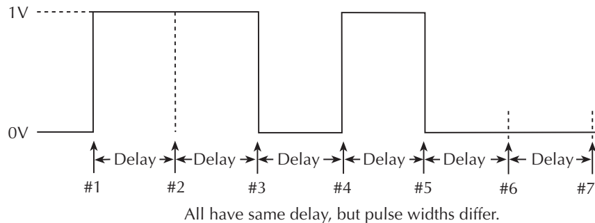
Figure 9-4 Custom sweep with different pulse widths
