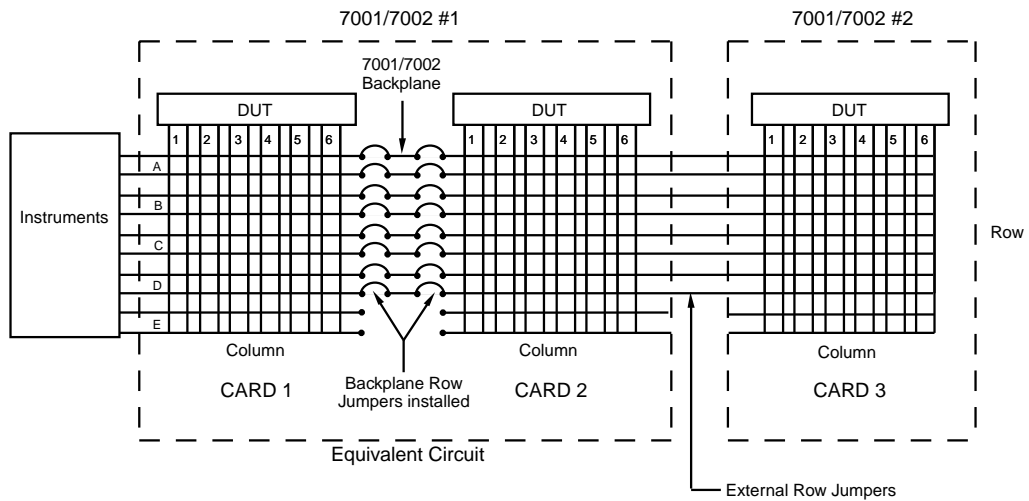
Figure 4-14 Two-mainframe system example
