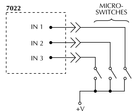
B. INPUT RESISTOR IS SET TO PULL DOWN.
