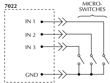
A. INPUT RESISTOR IS SET TO PULL UP.
