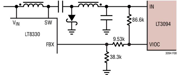
Figure 8. VIOC Connection Using LT8330 Delivers -3.3V When Operating, -5V When LT3094 is Disabled
