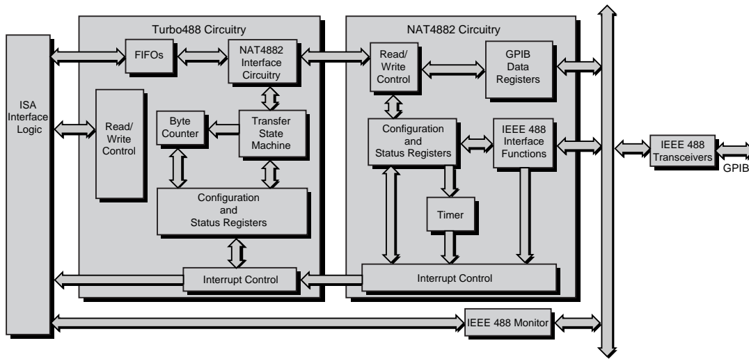
Figure 2. TNT4882 Two-Chip Mode
