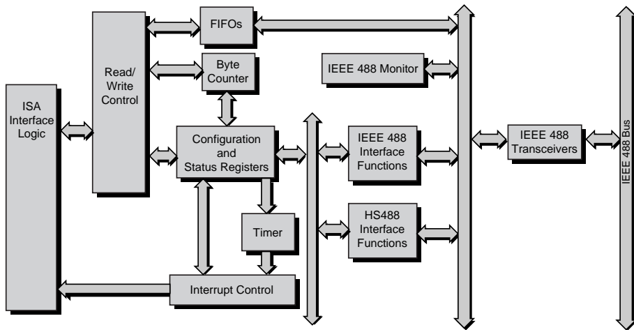
Figure 1. TNT4882 One-Chip Mode
