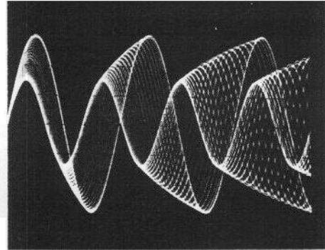
Modulation signal analysis using FAM: display of RF signal with simultaneous FM and AM
