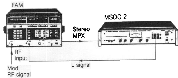
Measurement of stereo multiplex signals using Modulation Analyzer FAM
