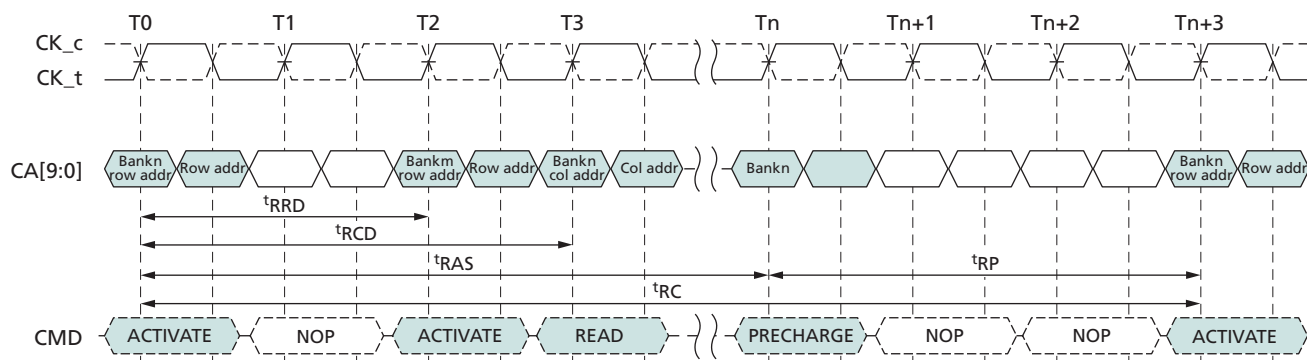
Figure 10: ACTIVATE Command
