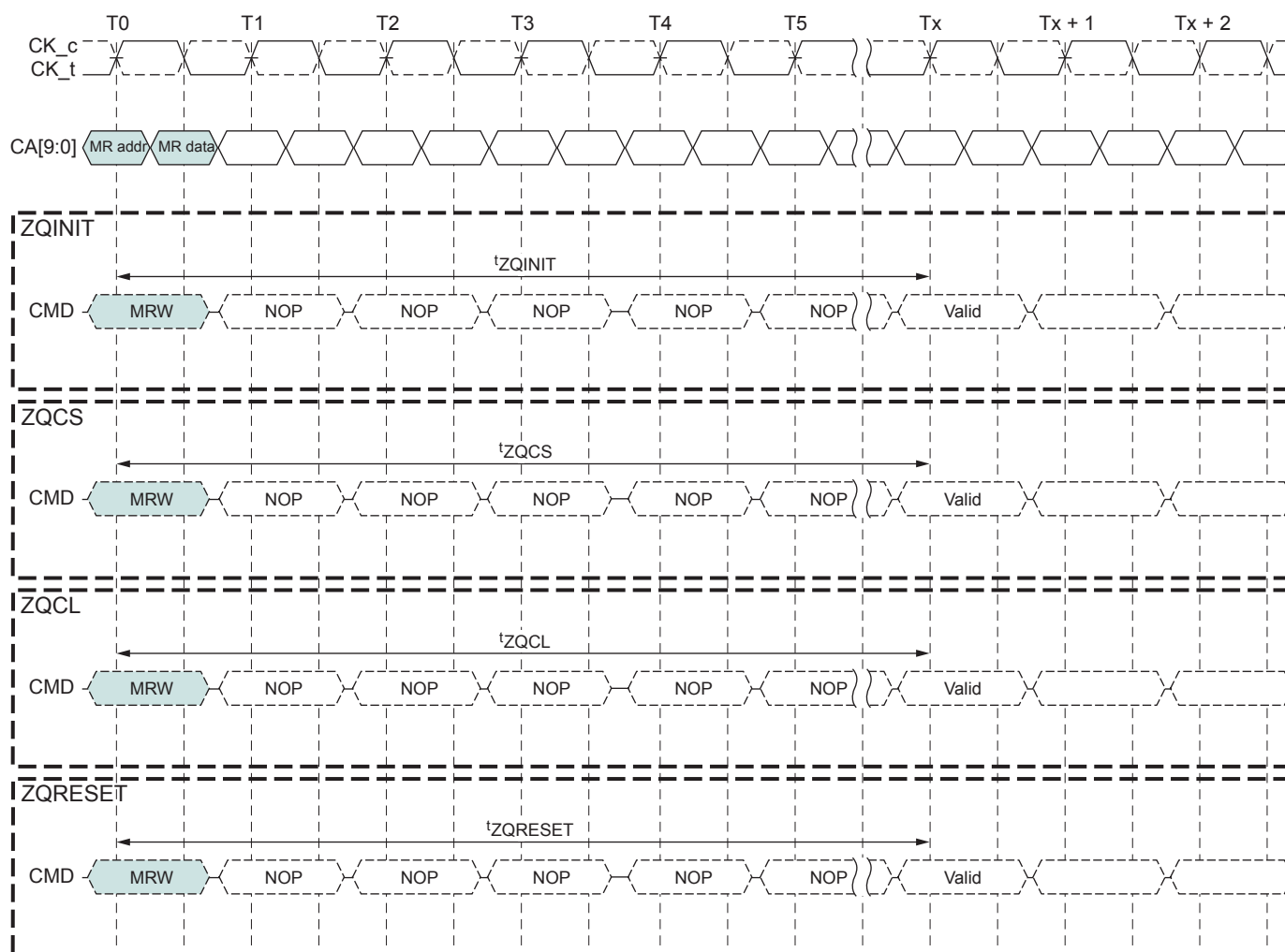
Figure 50: ZQ Timings
