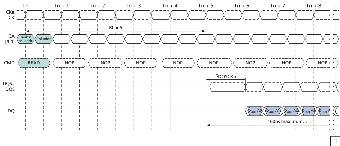
Figure 18: t_{DQCKDS} Timing
