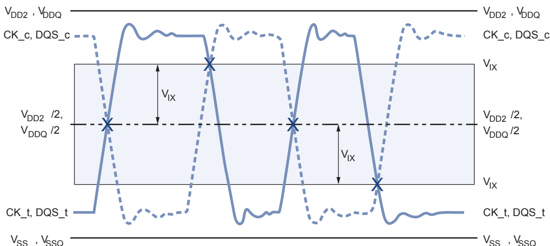
Figure 69: V_{IX} Definition
