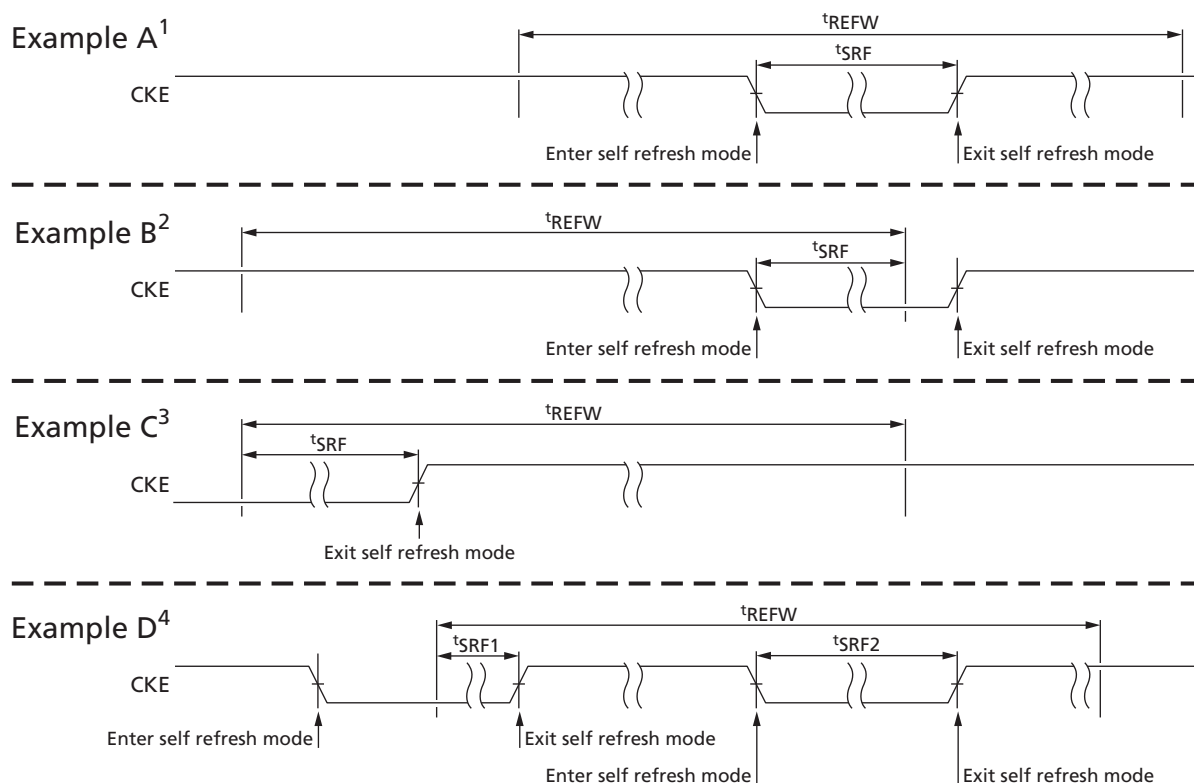
Figure 36: t_{SRF} Definition
