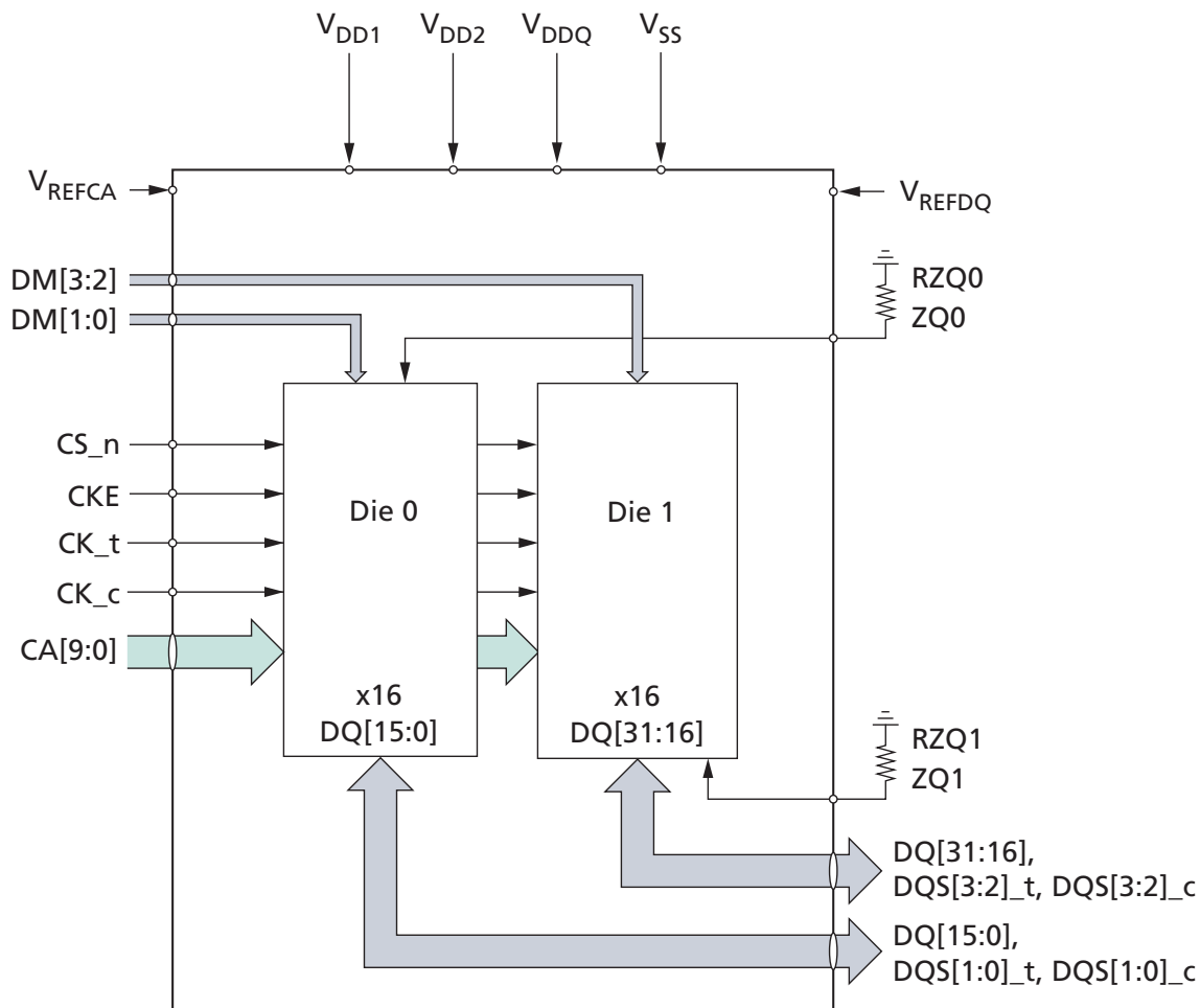
Figure 2: Single-Rank, Dual-Die, Single-Channel Package Block Diagram
