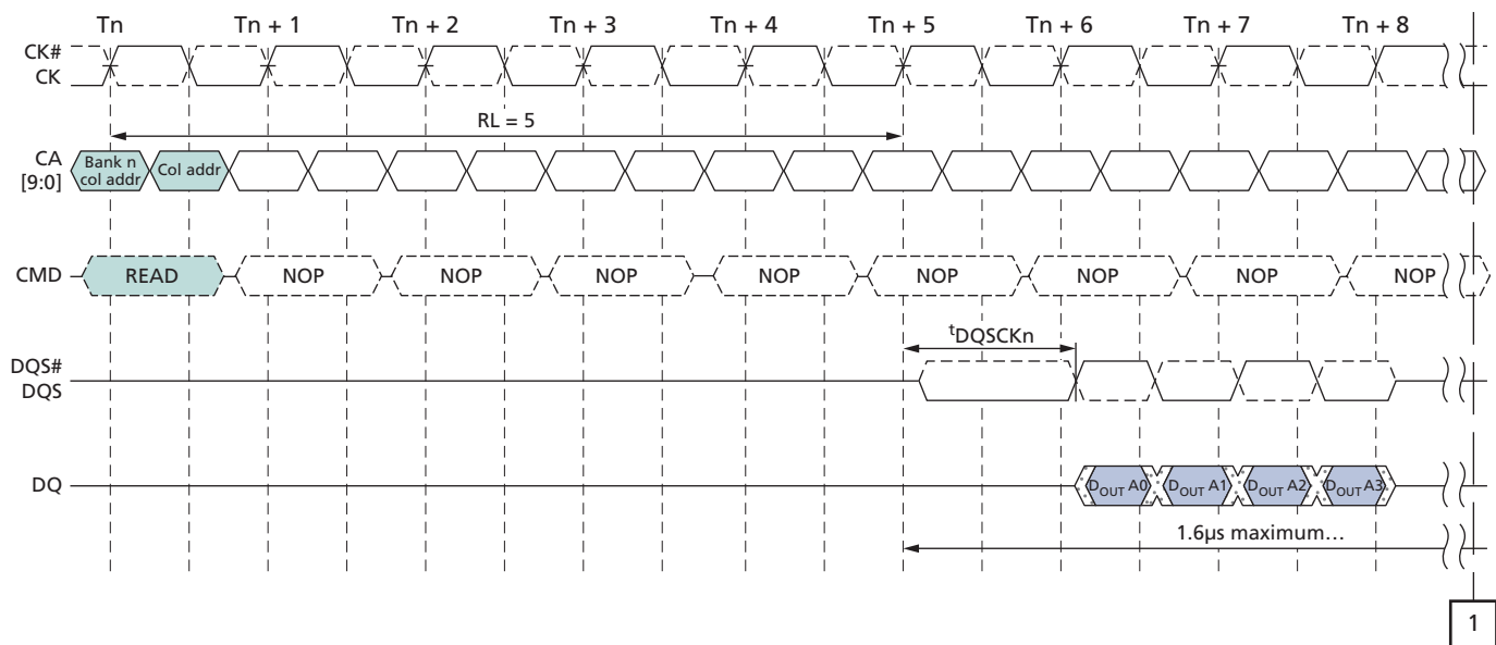
Figure 17: t_{DQSCDM} Timing
