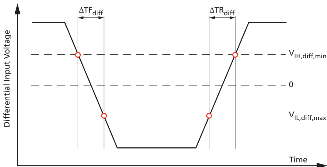
Figure 70: Differential Input Slew Rate Definition for CK_t, CK_c, DQS_t, and DQS_c
