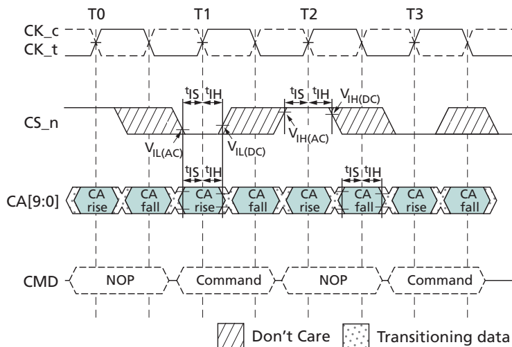
Figure 8: Command and Input Setup and Hold
