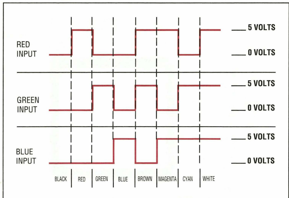
Fig. 1: Alternating TTL levels from 1's and 0's produce shades of gray or colors in digital computer monitors.
