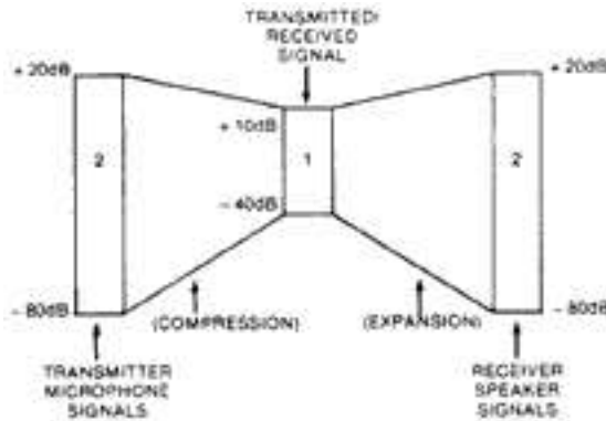
Fig. 11: Compression - Expansion response showing action from the transmitter to the receiver.
