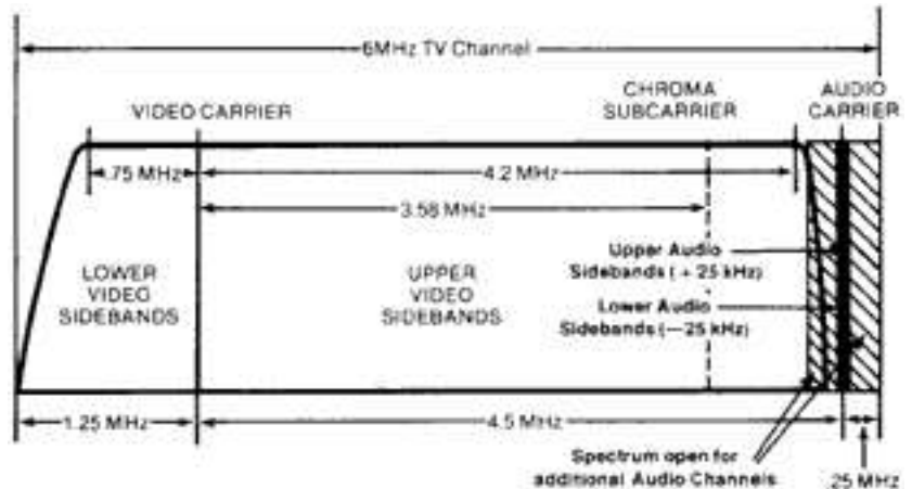
Fig. 2: Standard N channel. Note positioning of MTS Stereo audio signals.
