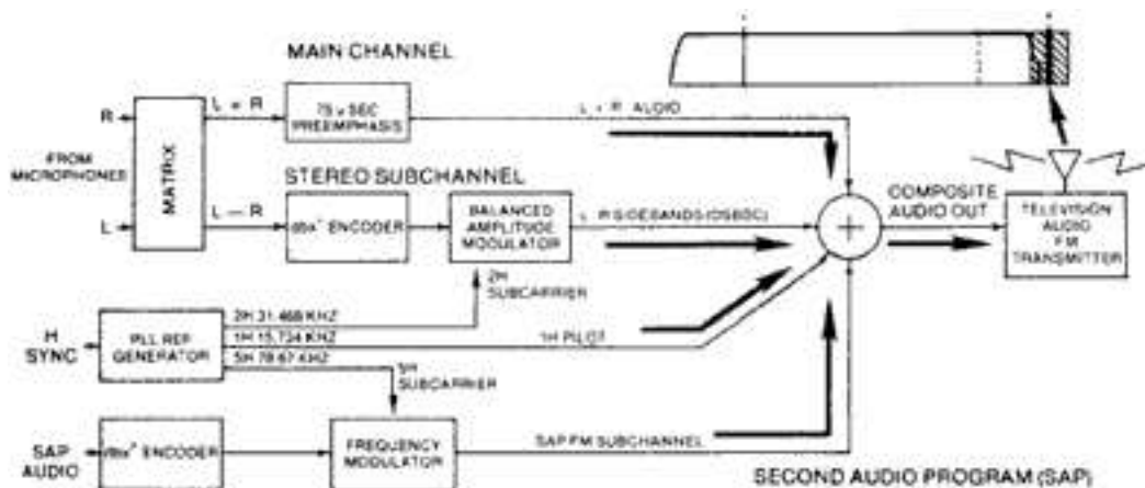
Fig. 4 : The composite MTS audio signal frequency modulates the TV channel's audio carrier.
