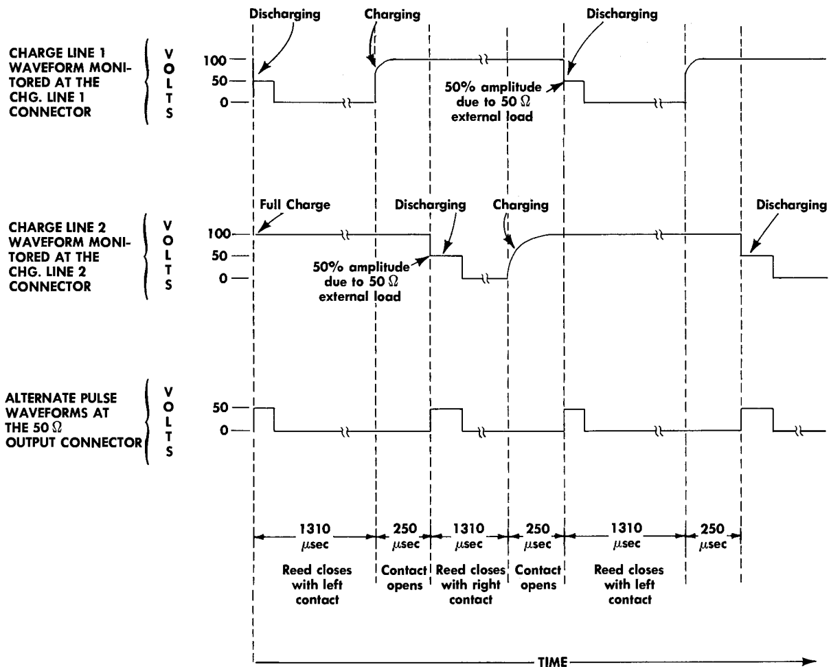
Fig. 4-3. Charge and discharge sequence using two separate different length charge lines. For this illustration CHARGE LINE 2 is twice as long as CHARGE LINE 1, the Type 109 output amplitude is +50 volts, and the nominal repetition rate of the pulses generated from each contact is 320 cps.
