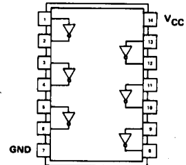
7416 156-0093-00 Hex Inverter
