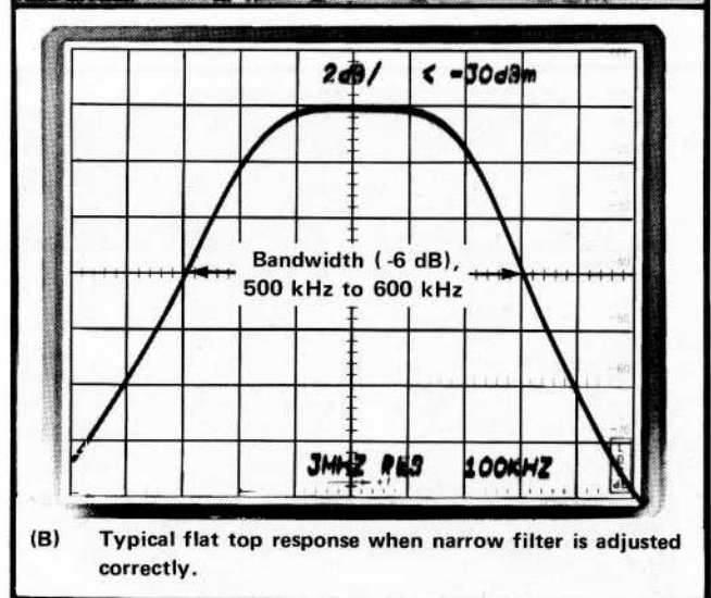
Fig. 4-16. Connections, adjustments, and typical response when adjusting the Narrow Post-Amplifier Filter.
