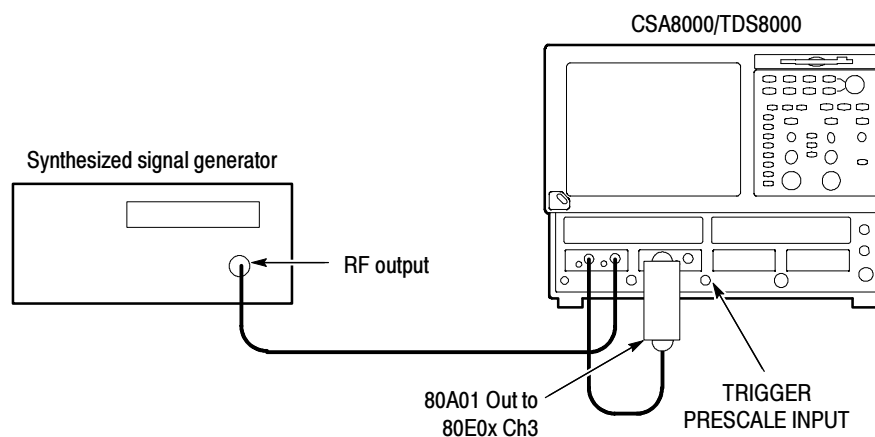
Figure 4-53: 80A00 test hookup
