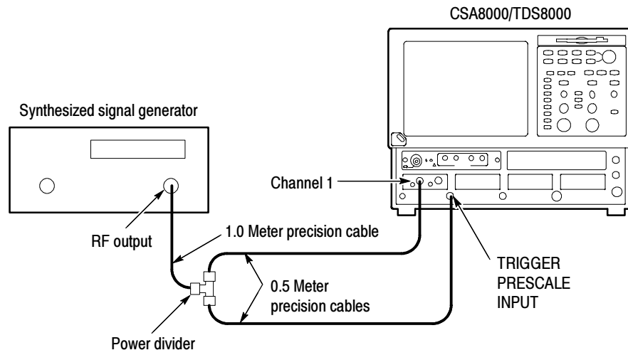
Figure 4-21: External prescaled trigger sensitivity test hookup
