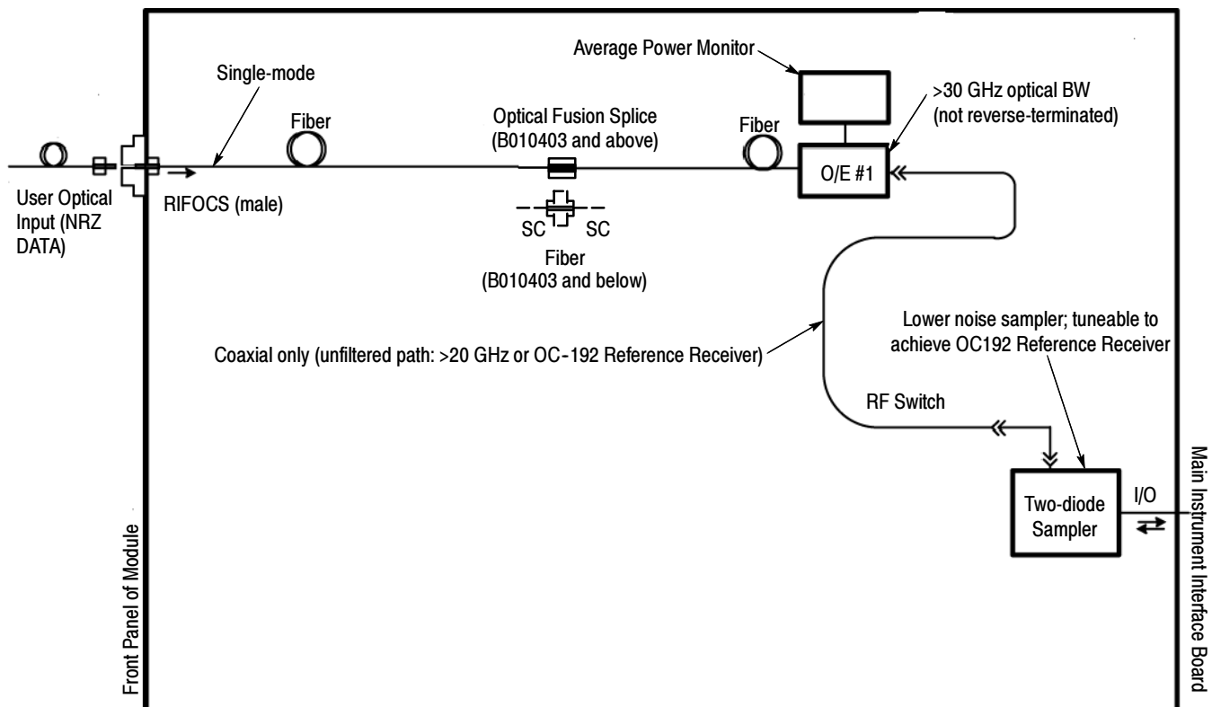
Figure 9-5: 80C02 Optical sampling block diagram
