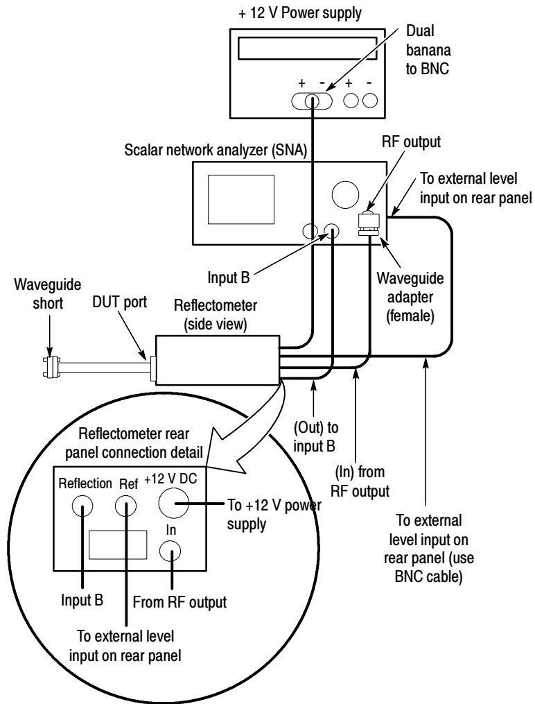
Figure 4-36: SNA/Waveguide Characterization
