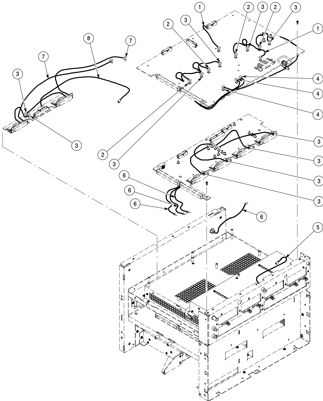
Figure 10-5: Coaxial cables
