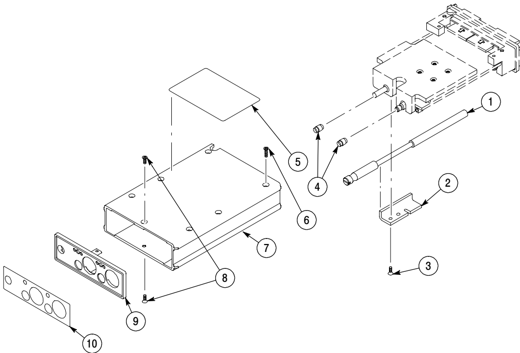
Figure 10-9: 80A01 module
