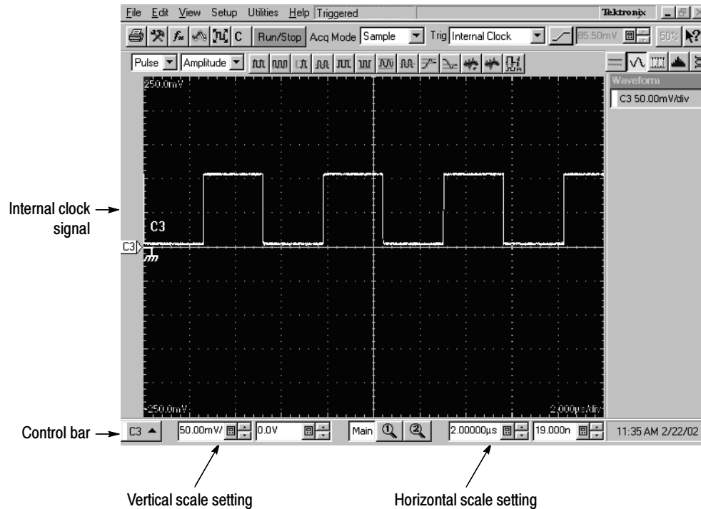
Figure 4-12: Signal triggered
