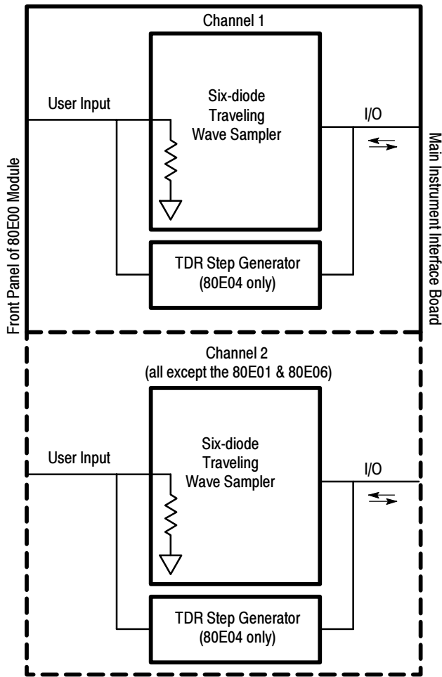
Figure 9-2: Block diagram for the 80E00 Series Electrical Sampling Modules
