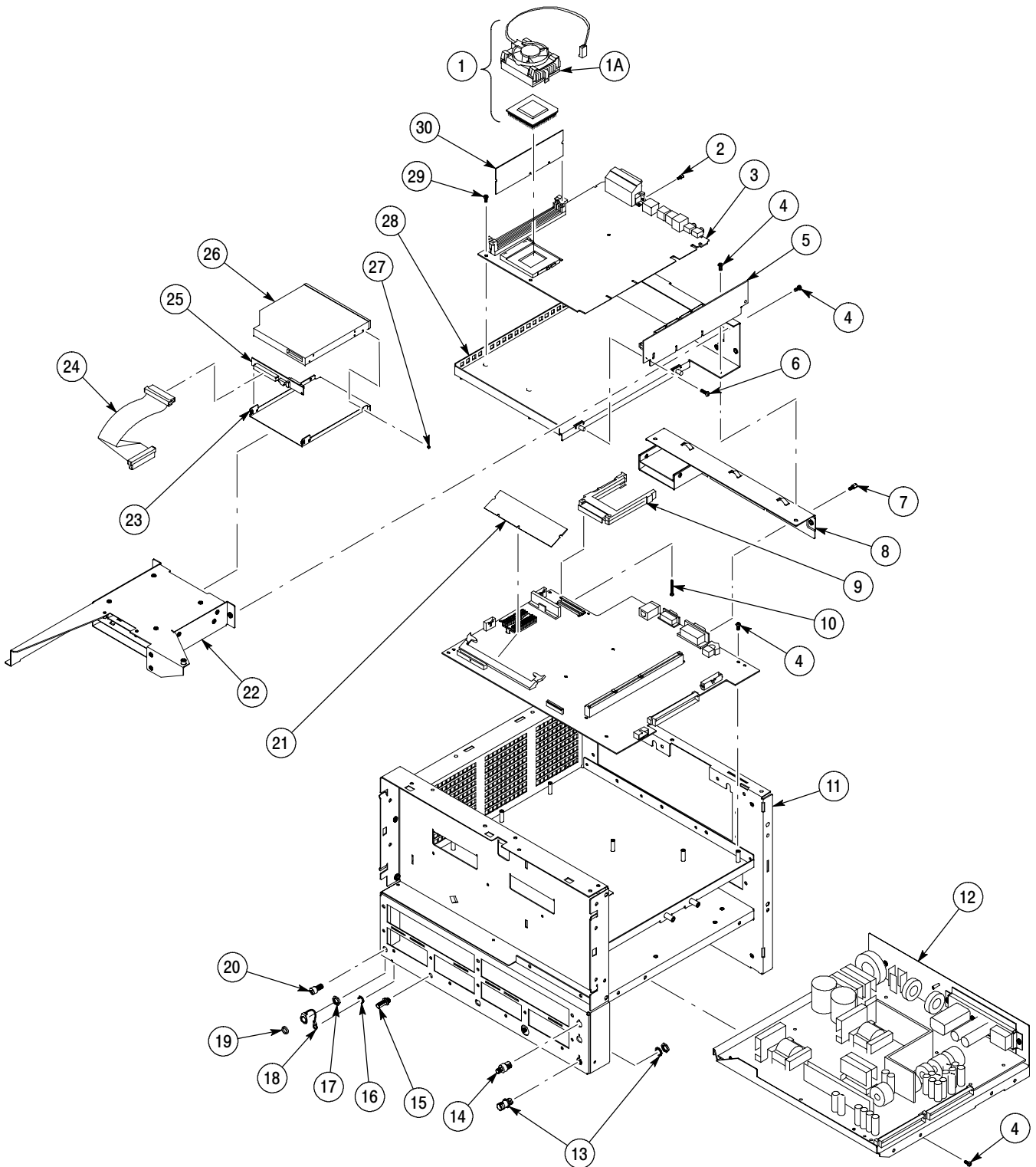
Figure 10-3: Power supply
