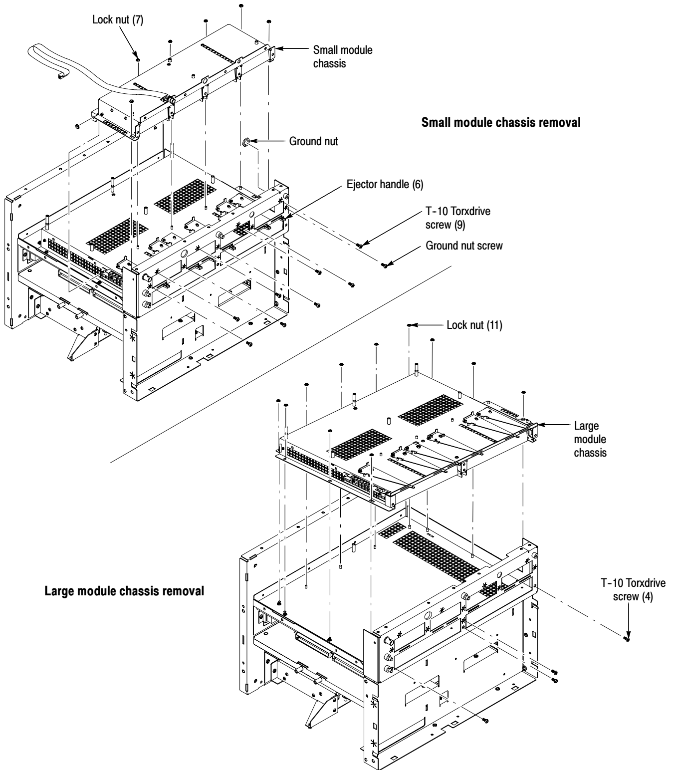
Figure 6-33: Small and Large module chassis removal
