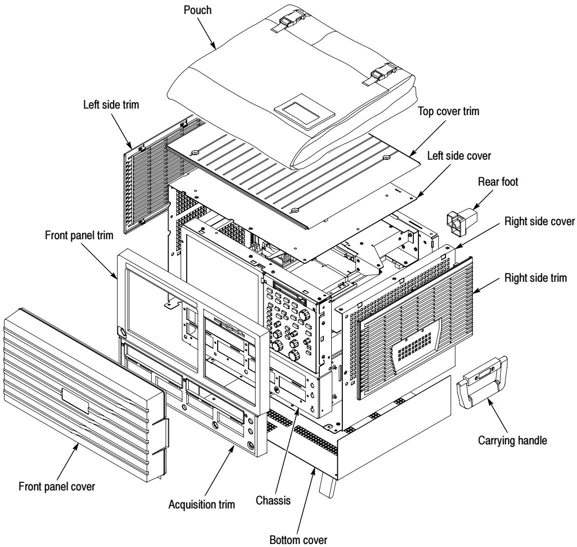
Figure 6-7: External modules
