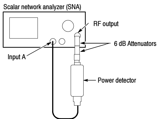
Figure 4-33: No Adapter hookup
