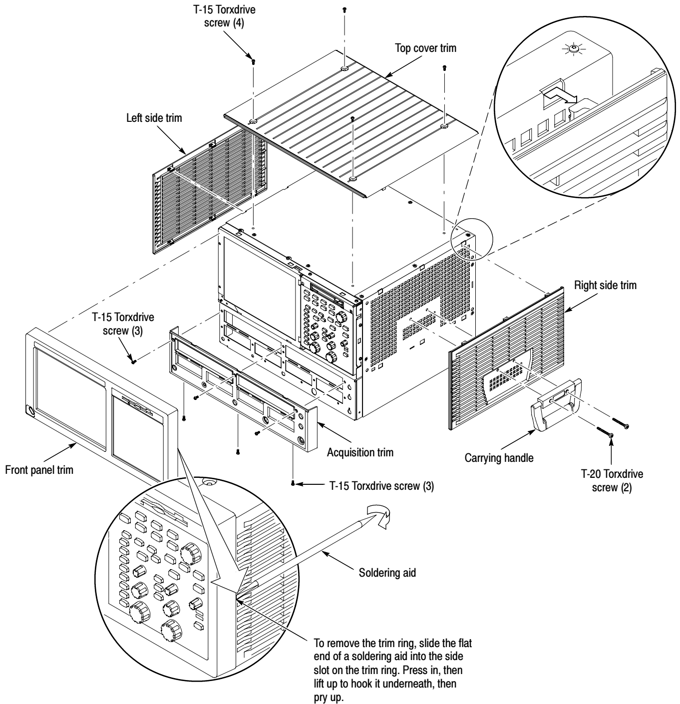
Figure 6-2: Trim removal
