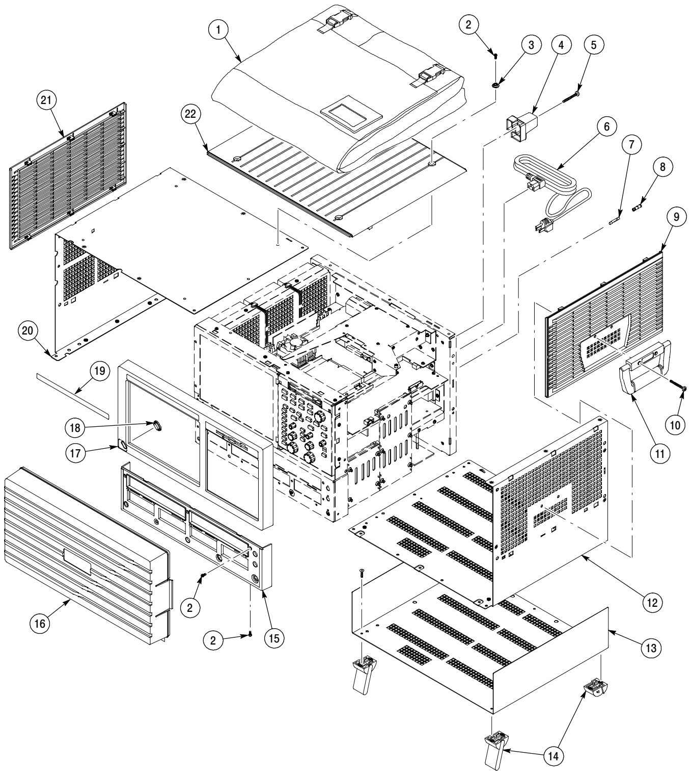
Figure 10-1: External parts
