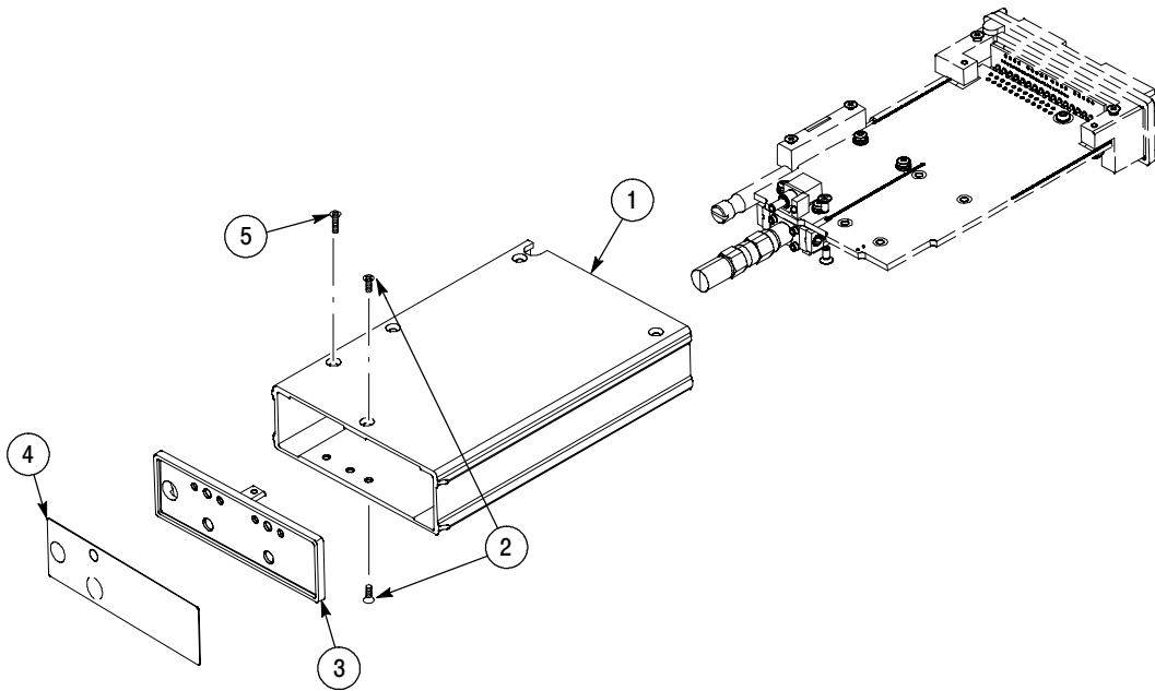
Figure 10-7: 80E06 module
