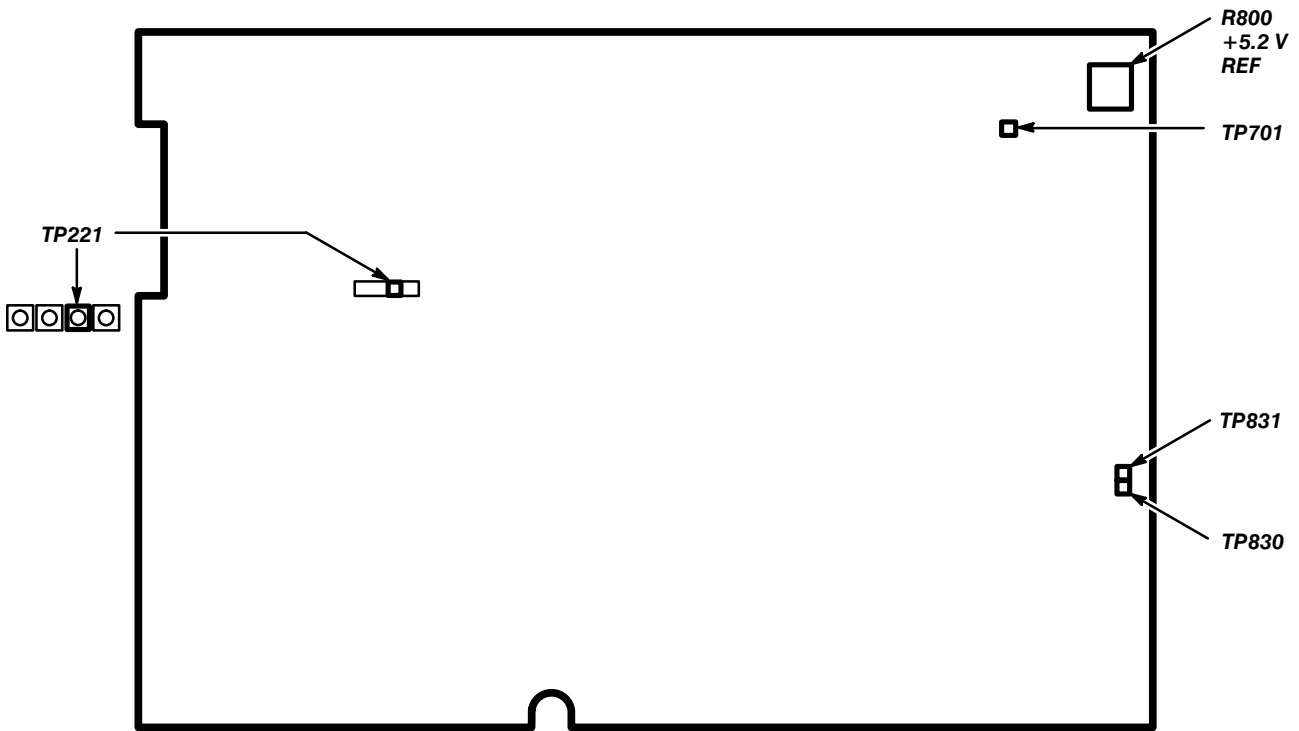
Figure 5-2: A2A2 Control Rectifier Board Test Point and Adjustment Locations
