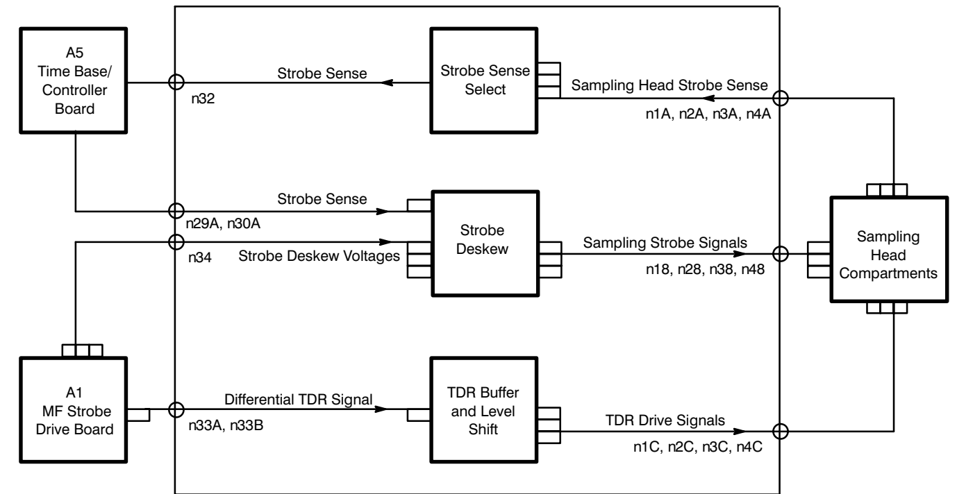
Figure 9- A: A. 9 Strobe/TDR Buffer Board Block Diagram
