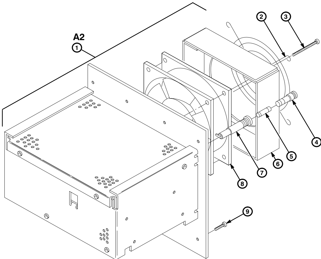
Figure 10-6: Power Supply
