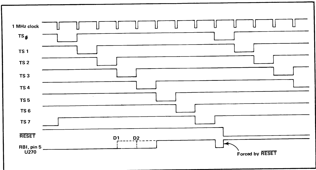
Fig. 2-3. Multiplexing circuit ladder diagram showing timing with an all-zero display.
