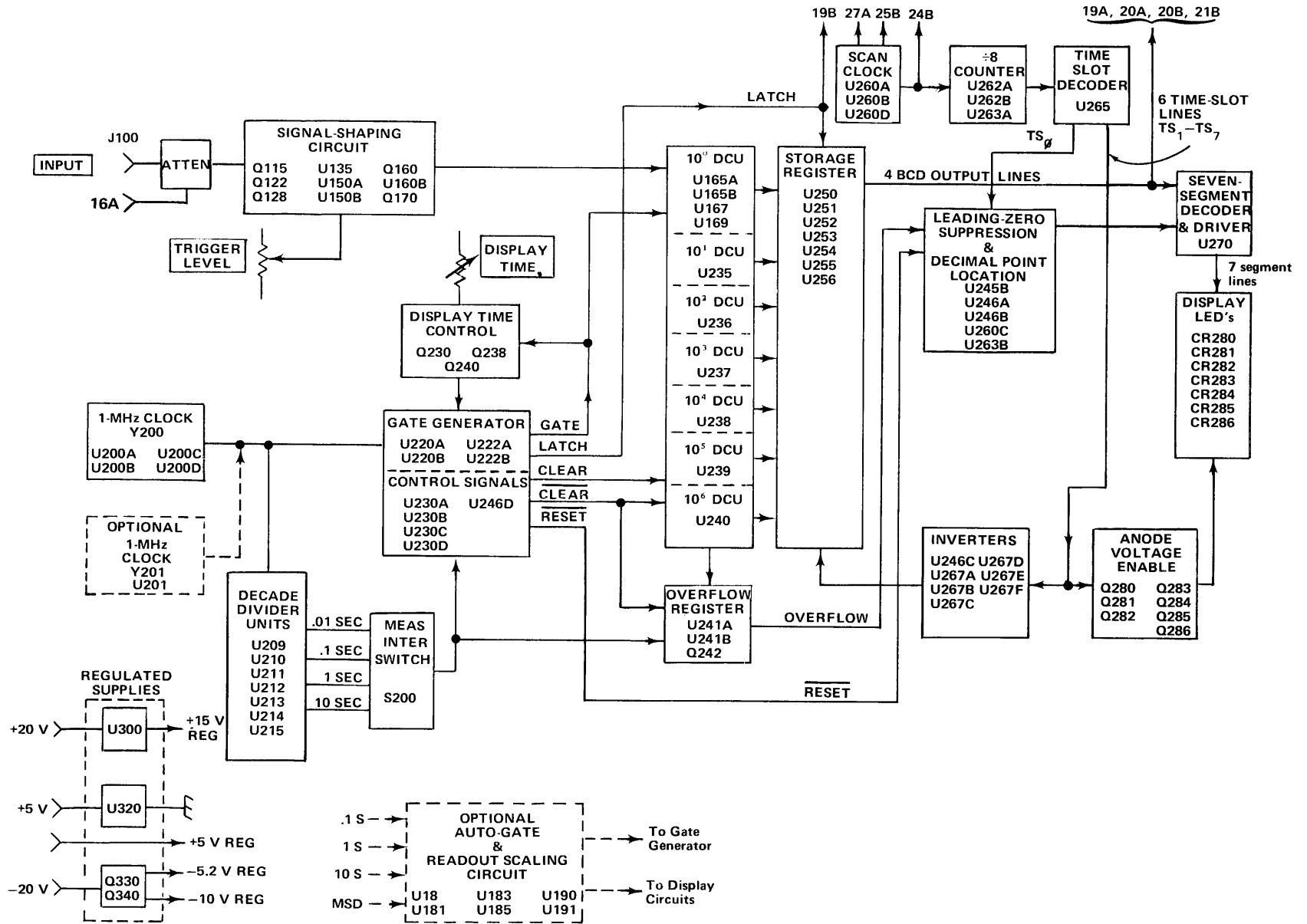
Fig. 2-1. DC 501 Block Diagram.
