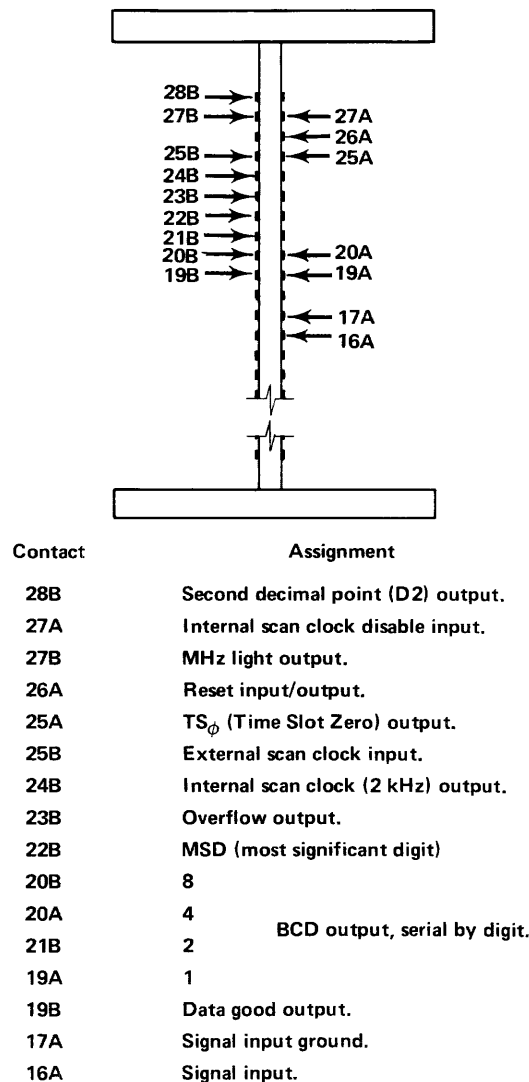
Fig. 1-1. Input/Output assignments of plug-in connector contacts.
