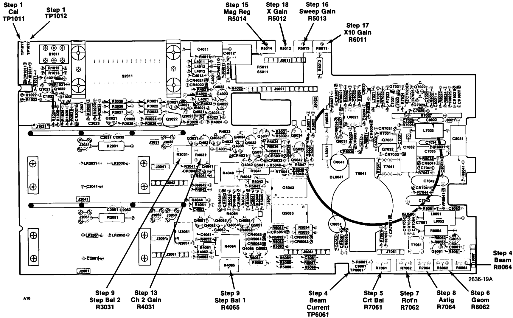
Fig. 8-13 Main Board.
