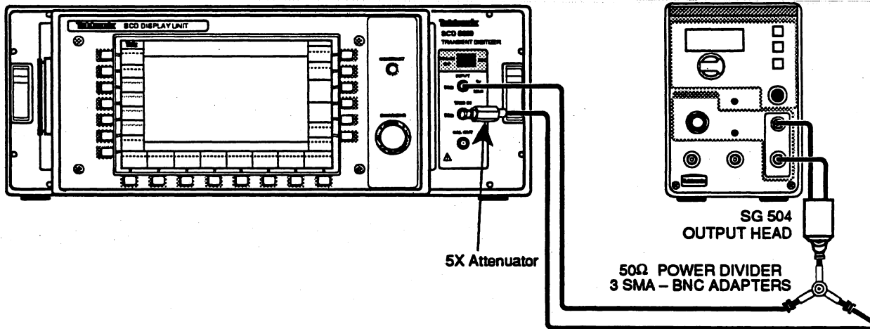
Figure 4-23: SCD5000 Trigger Sensitivity Setup Part 1
