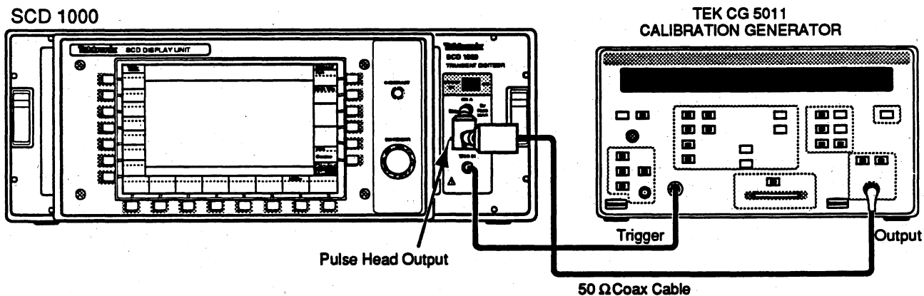
Figure 4-13: Step Response Setup
