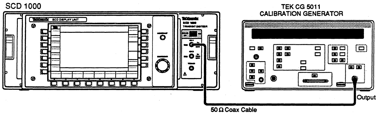
Figure 4-15: Low Frequency Linearity Setup
