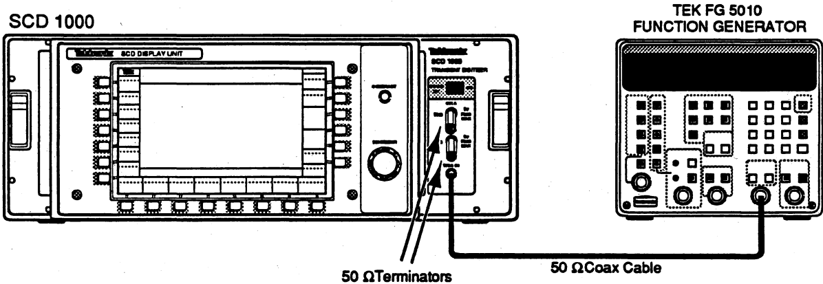
Figure 4-17: RMS Noise Setup
