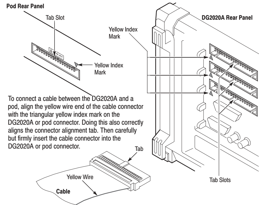
Figure 2: Yellow index mark and yellow wire for cable connection
