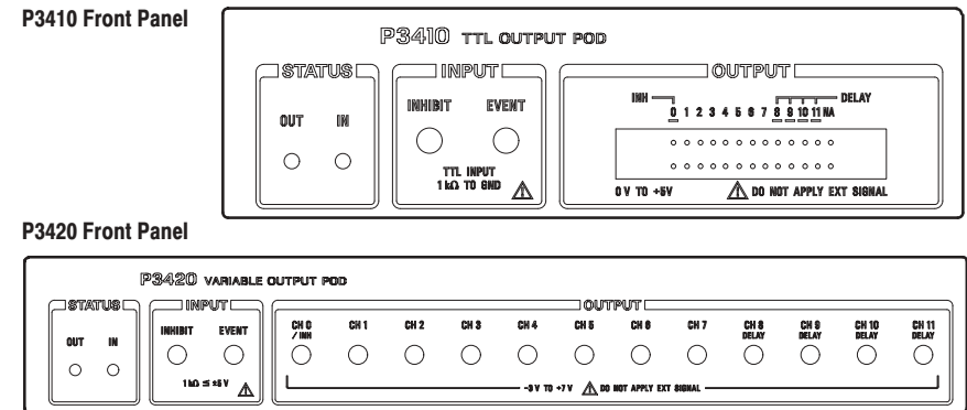
Figure 1: P3410 and P3420 front panels
