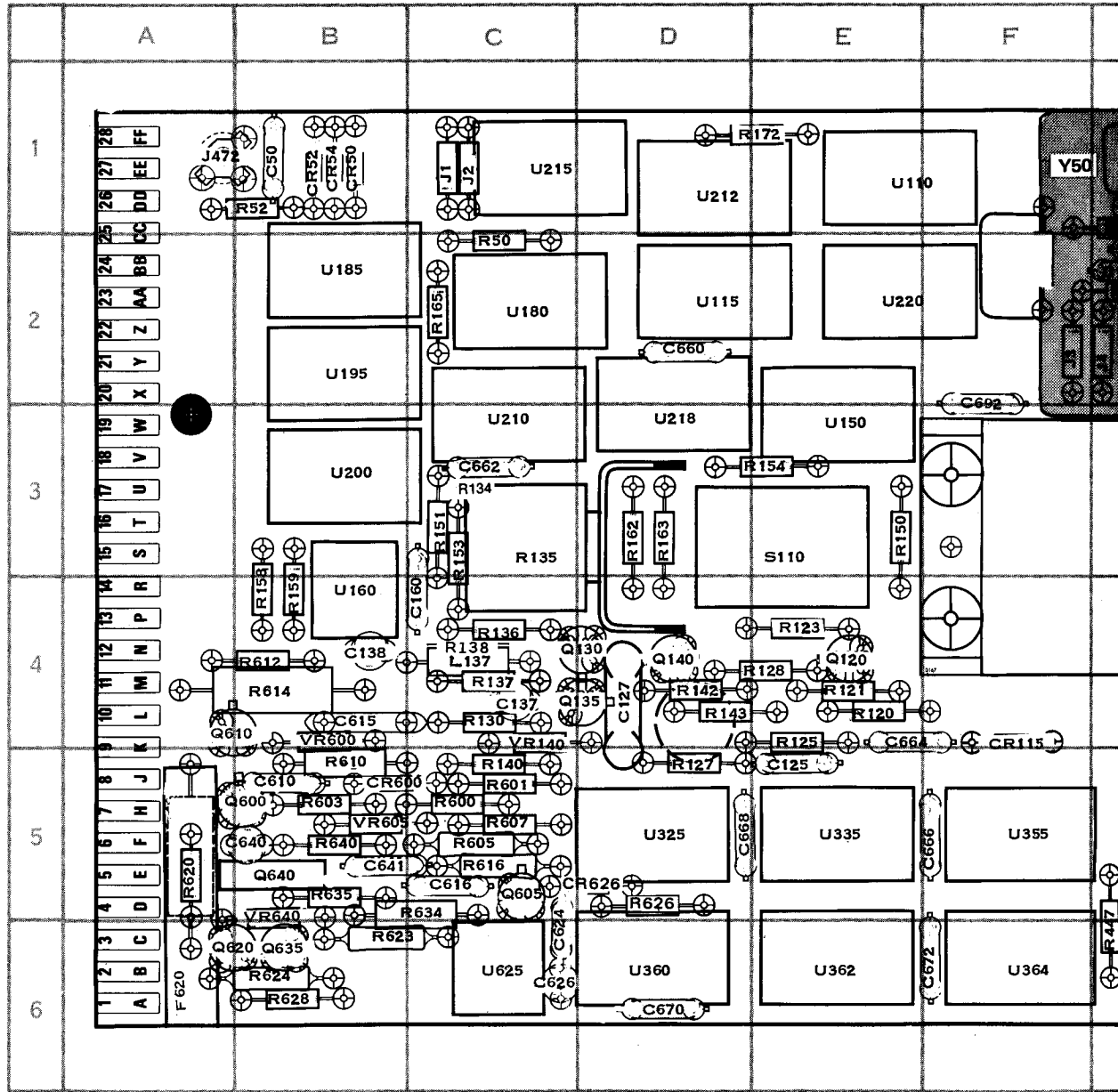
Fig. 8-3. A1—Main board
