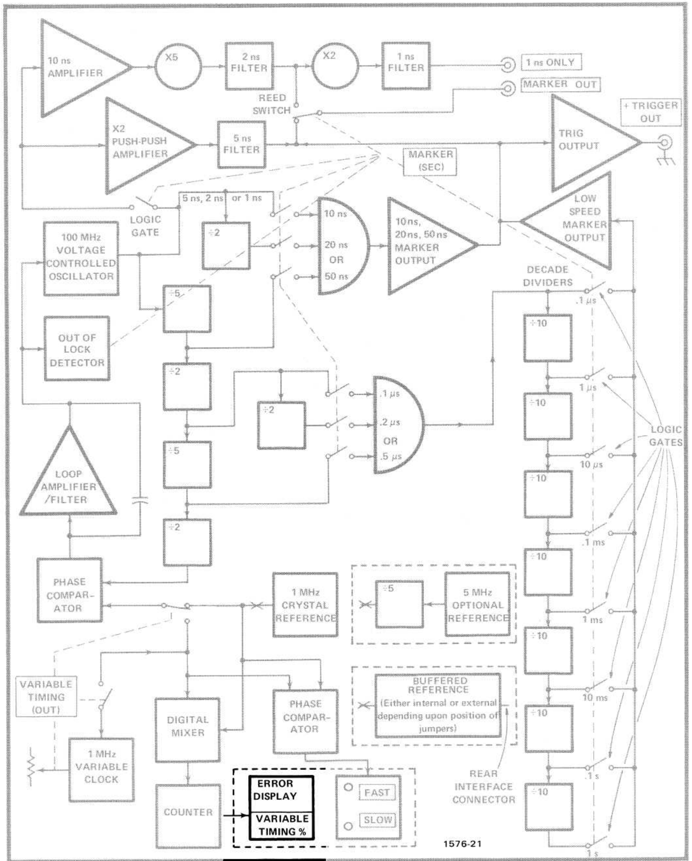
Fig. 3-4. Functional block diagram of schematic diagram 5 circuitry.
