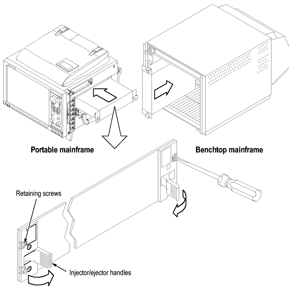
Figure 4: Installing modules
