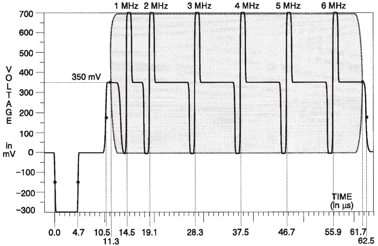
Fig. 3-235. Y Channel — 100% Sweep.
