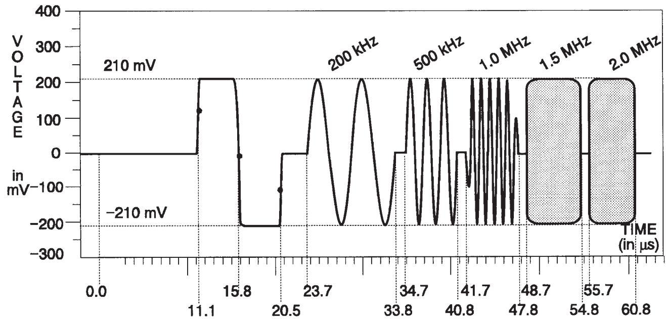
Fig. 3-200. B-Y & R-Y Channels — Narrow Multiburst.
