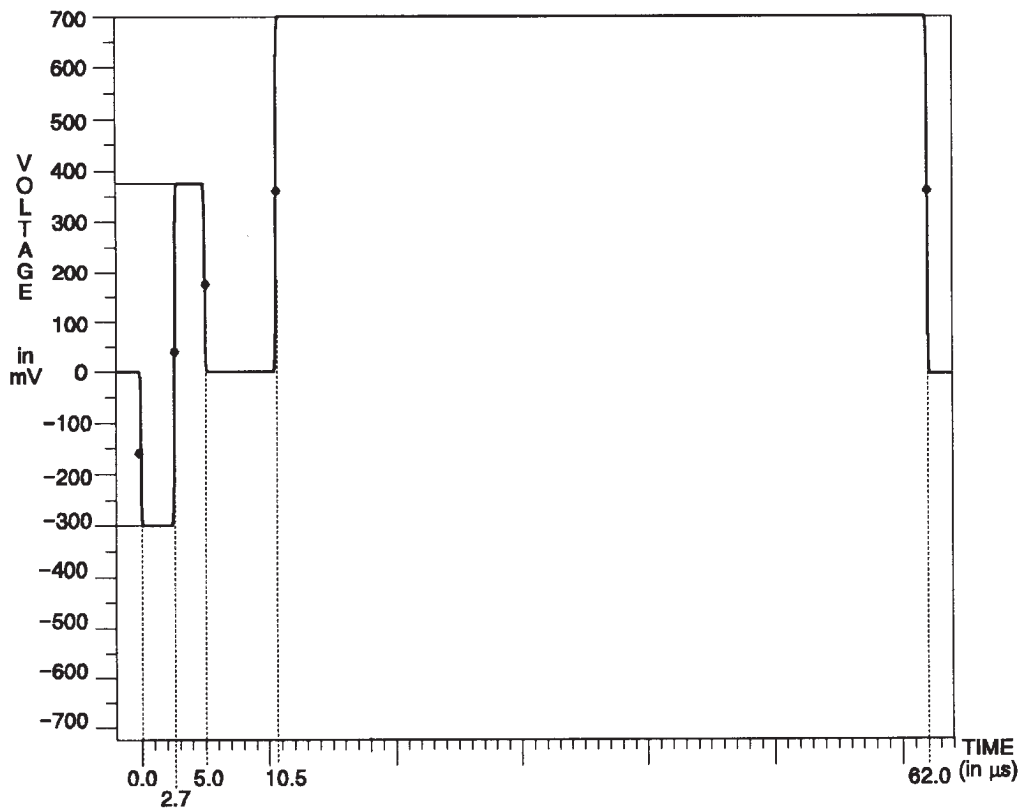
Fig. 3-110. Y Channel — 100% Flat Field.
