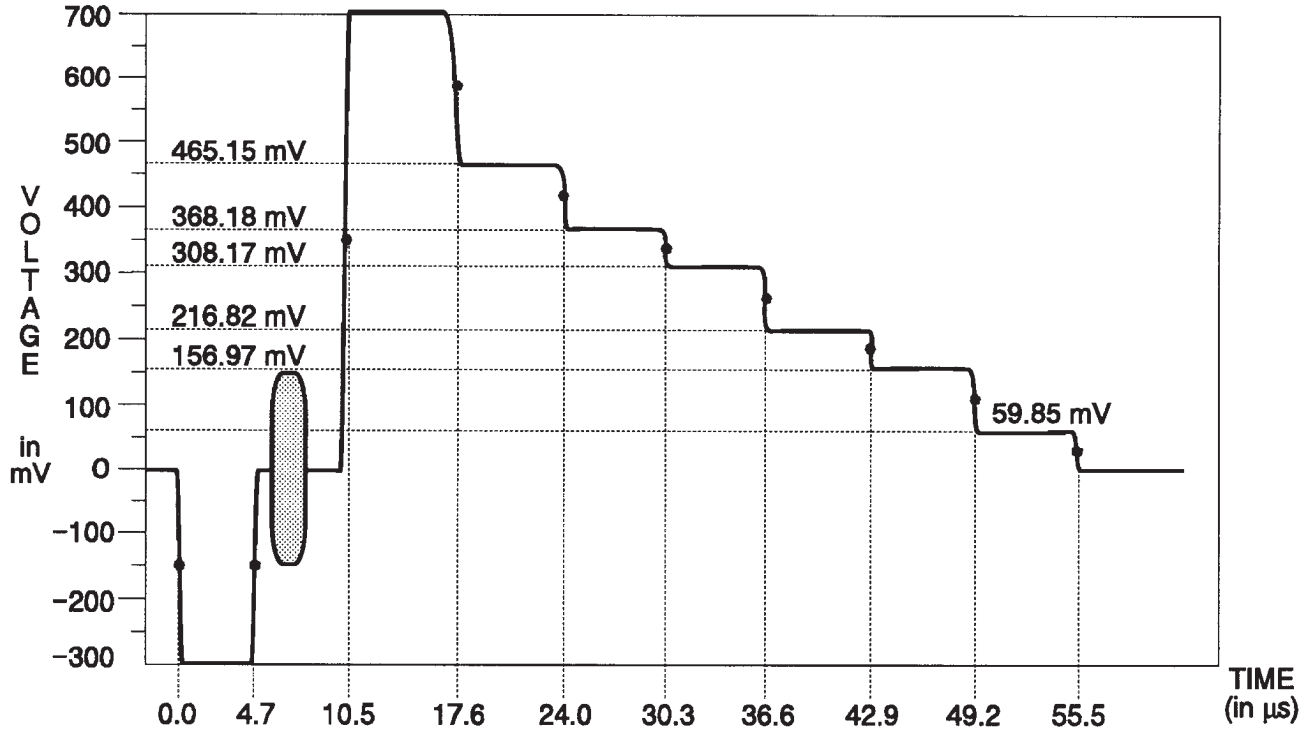
Fig. 3-141. Y Channel — 75% Color Bars.
