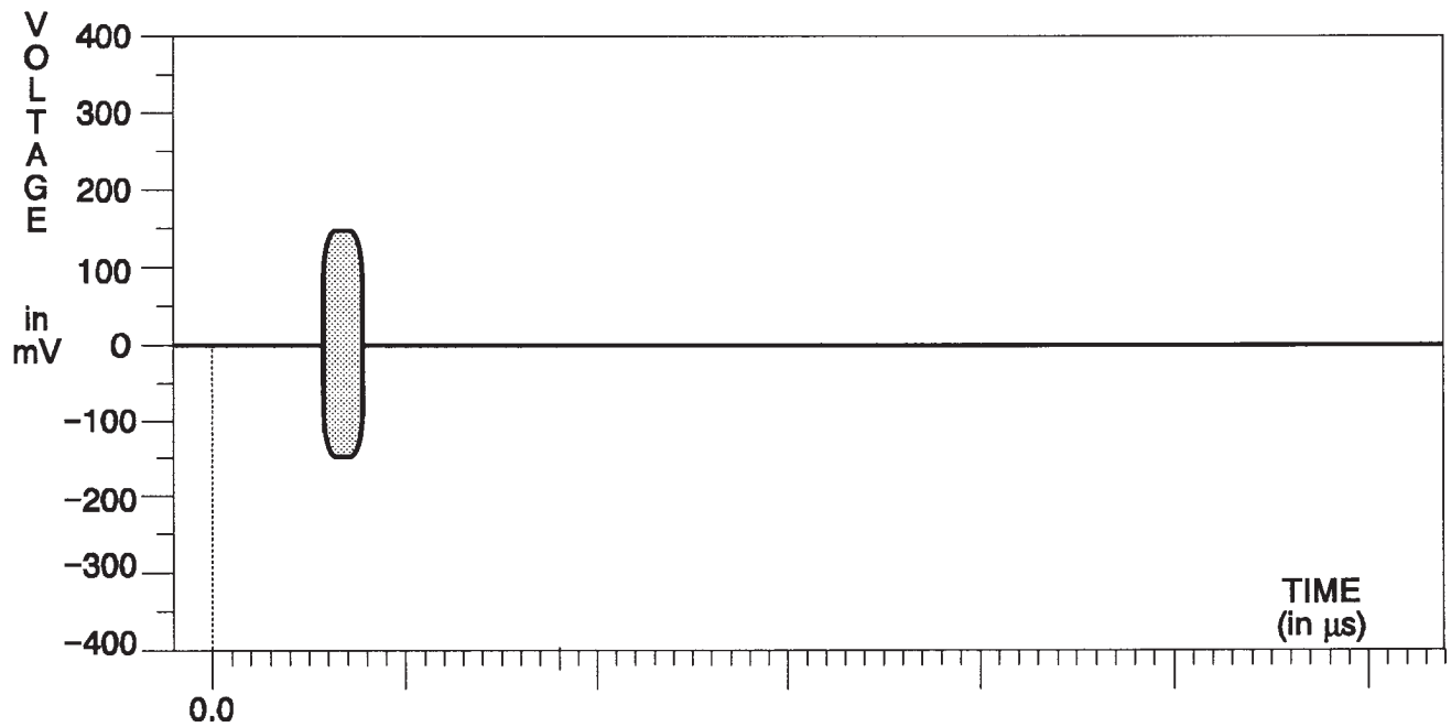
Fig. 3-41. C Channel — Pluge.
