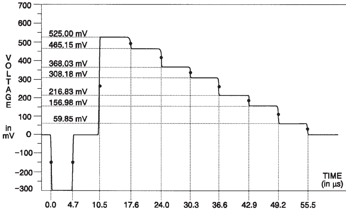
Fig. 3-221. Y Channel — 75% Bars.
