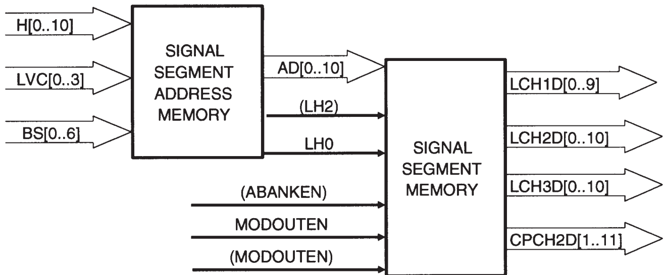
Fig. 3. Block diagram for <3>.
