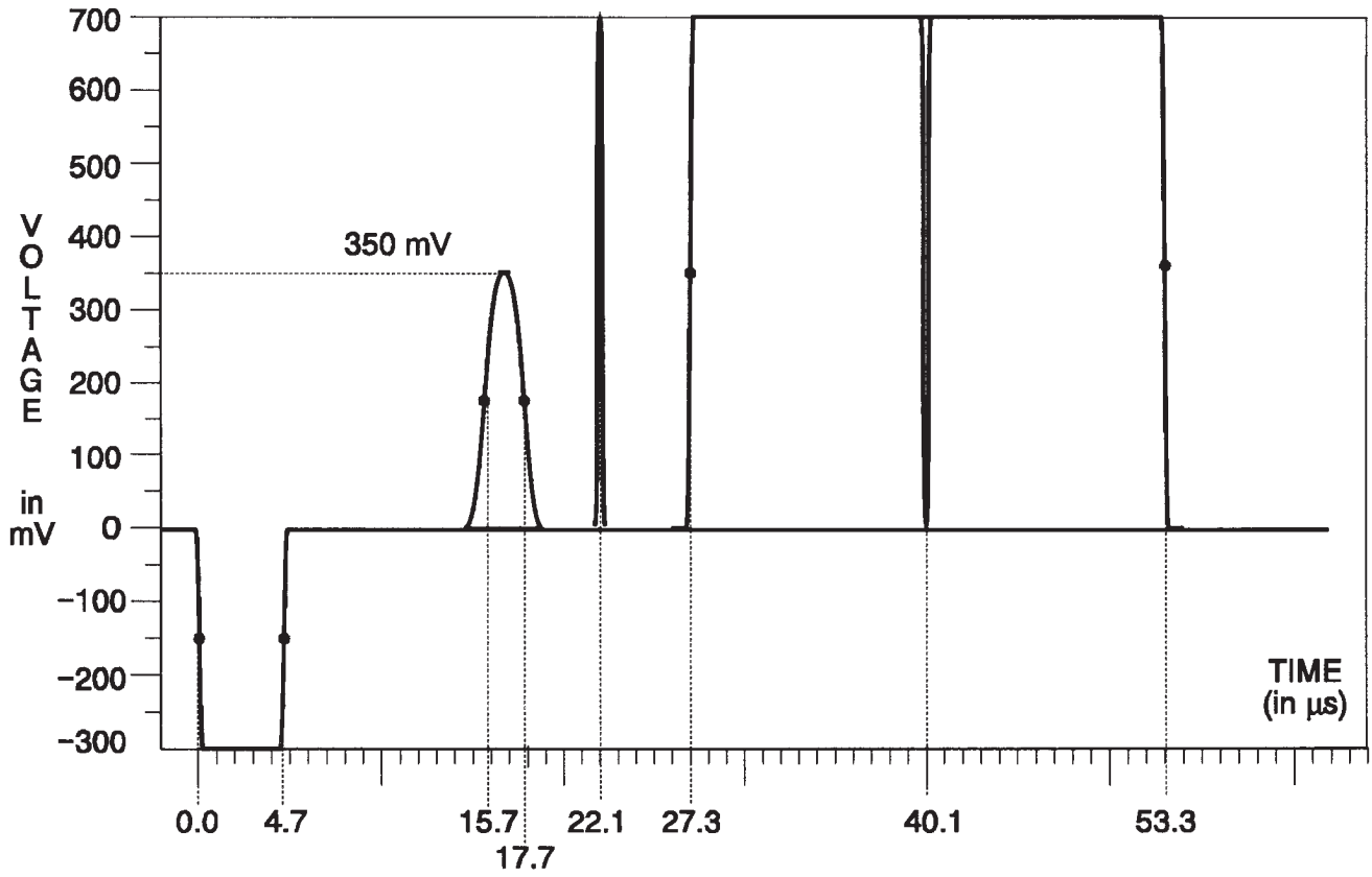
Fig. 3-54. Y Channel — Pulse & Bar with Window.
