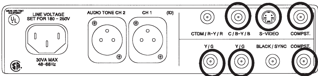
Fig. 2-5. Valid outputs in the PAL/YC mode.
