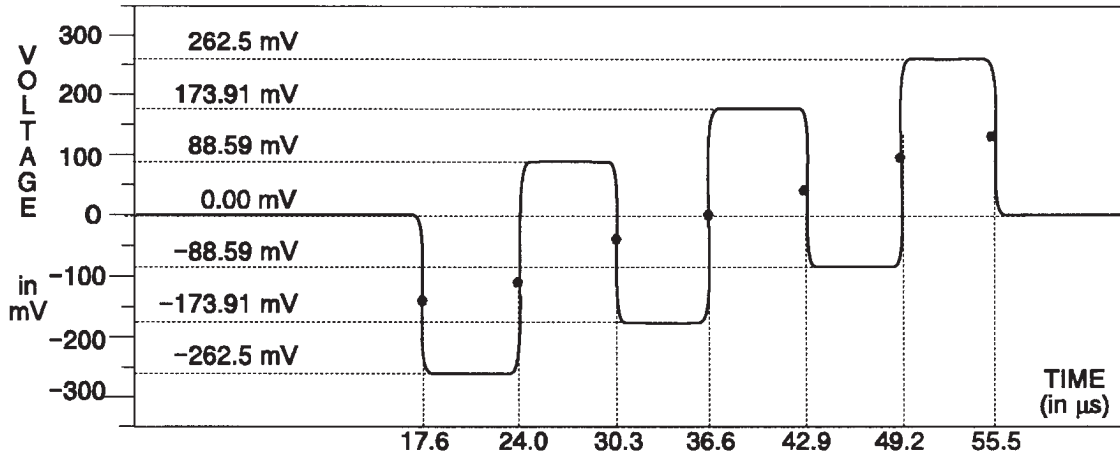
Fig. 3-222. B-Y Channel — 75% Bars.
