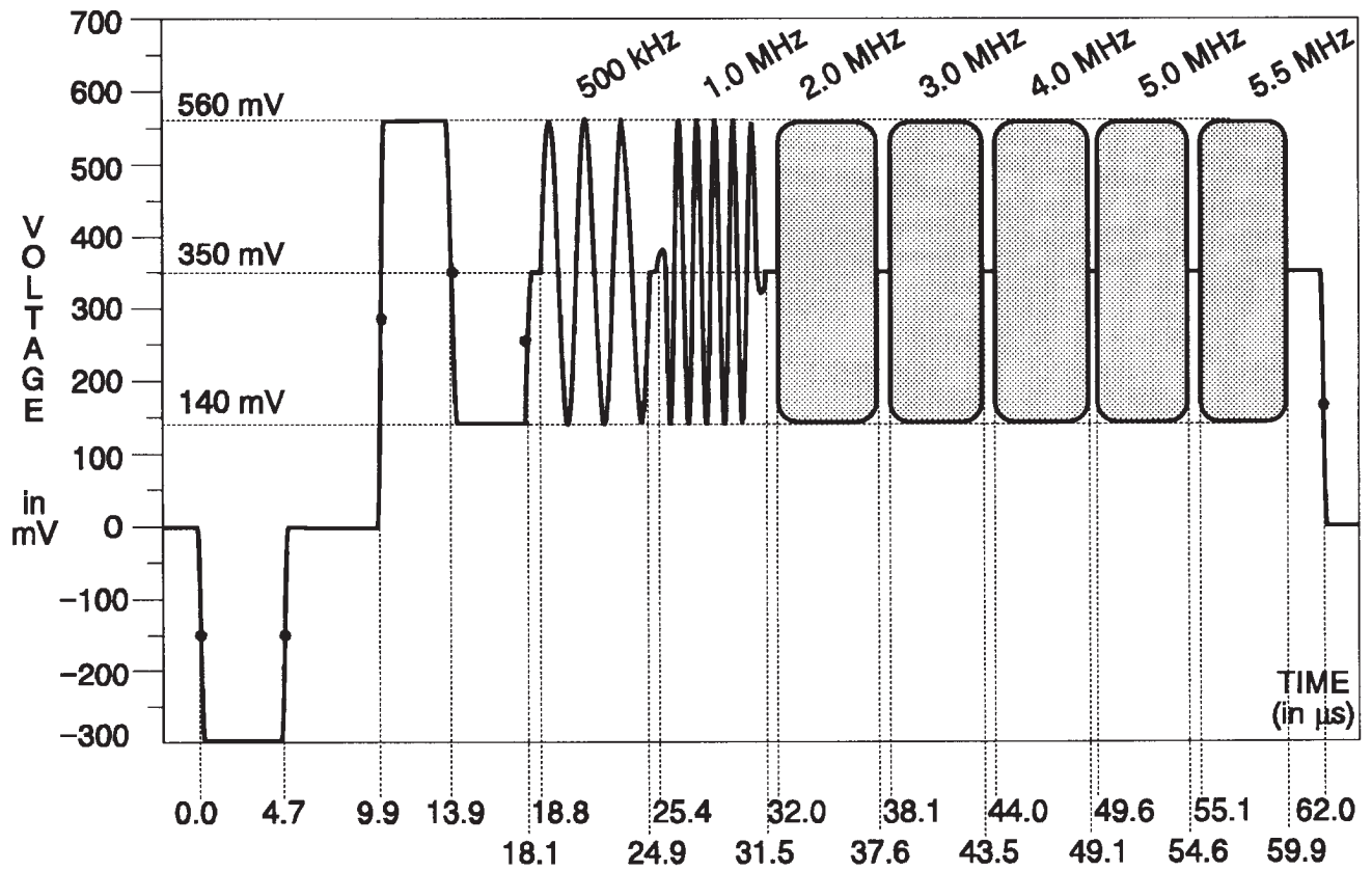
Fig. 3-201. Y Channel — 60% Wide Multiburst.
