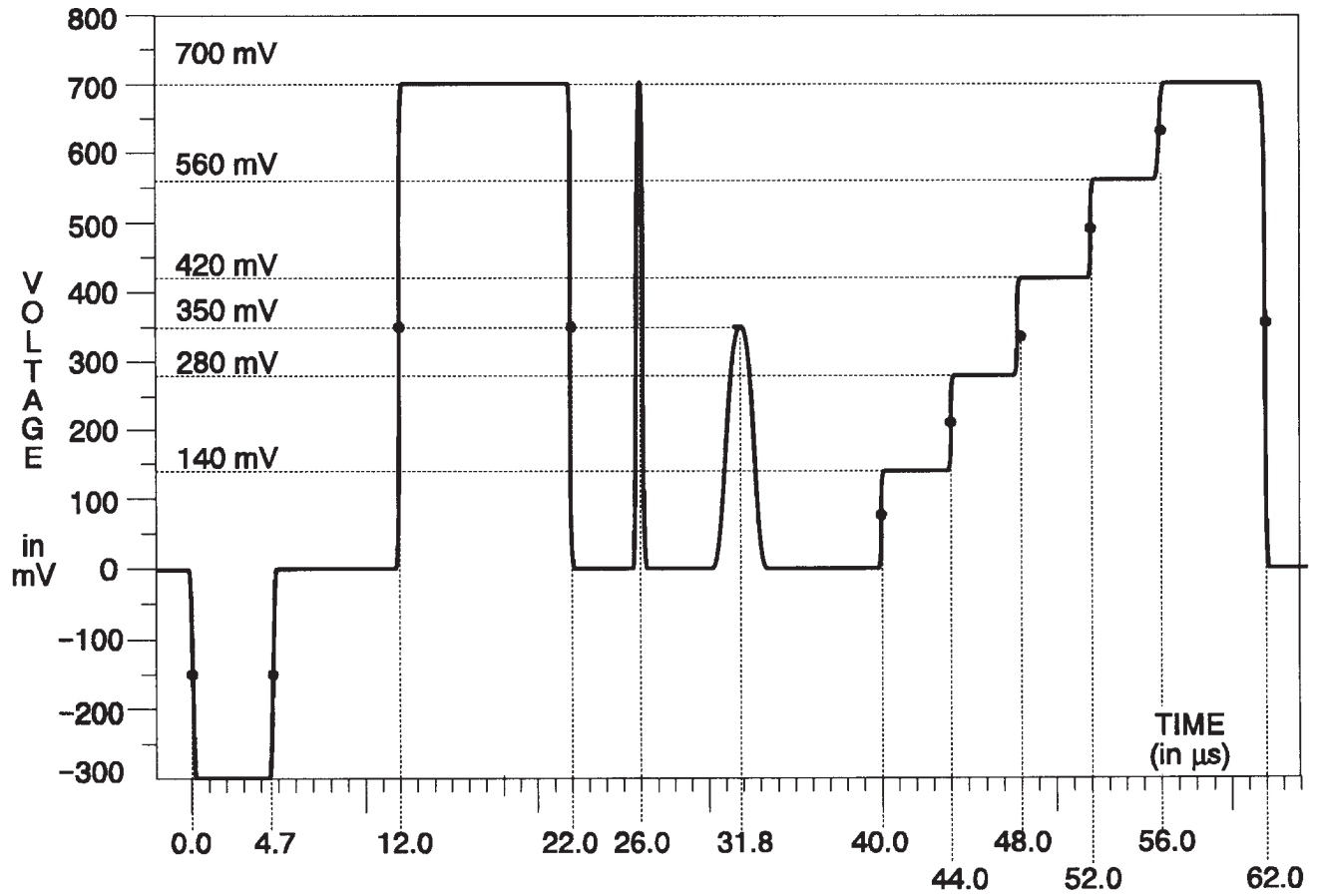
Fig. 3-197. Y Channel — Line 17.
