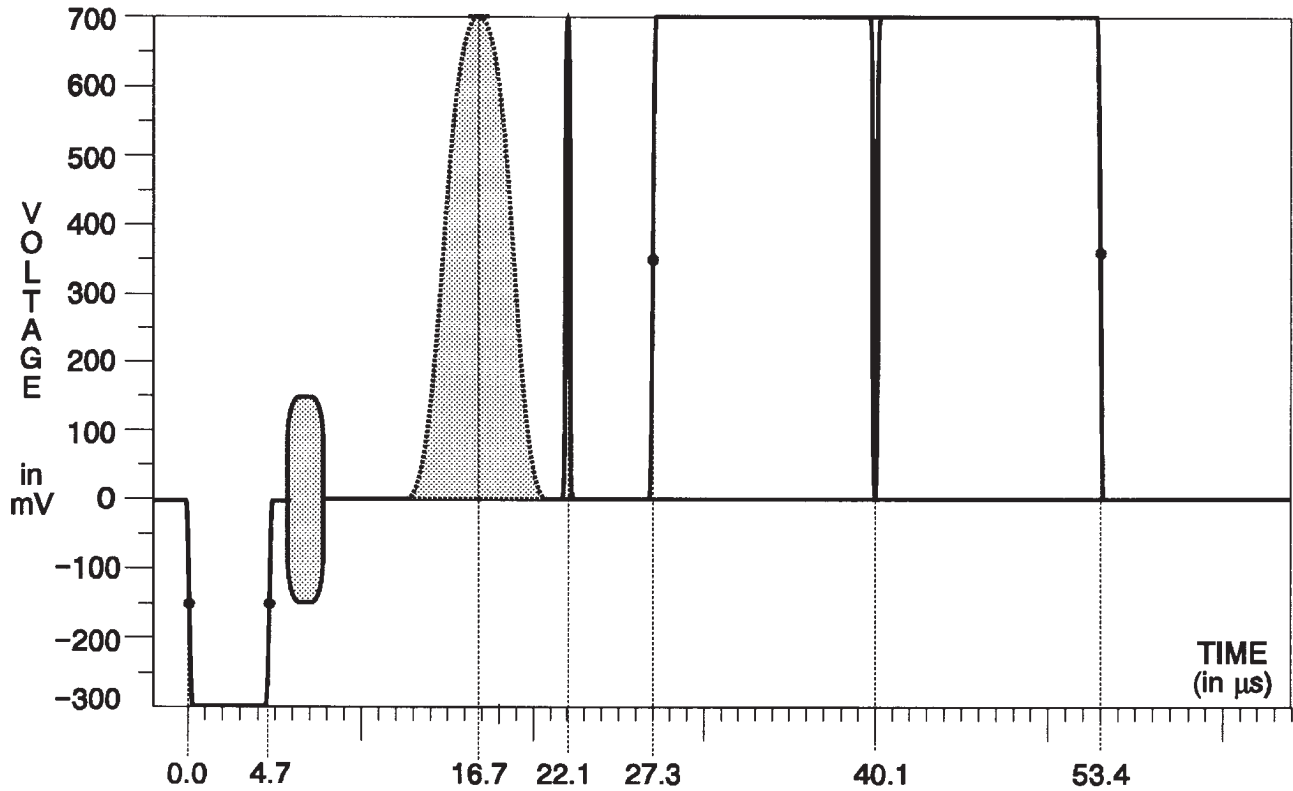
Fig. 3-18. Pulse & Bar with Window.
