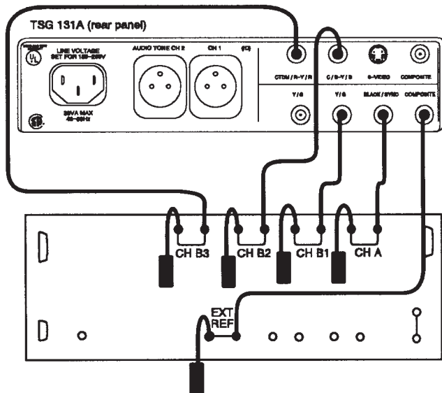
1781R WAVEFORM MONITOR/VECTORSCOPE (rear panel)
