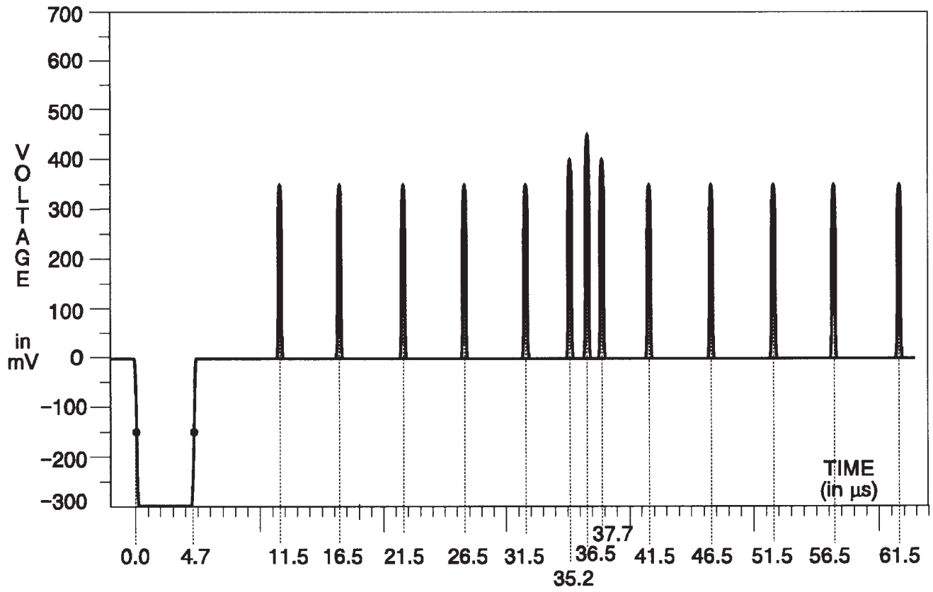
Fig. 3-241. Y Channel — 100% Bowtie Markers.
