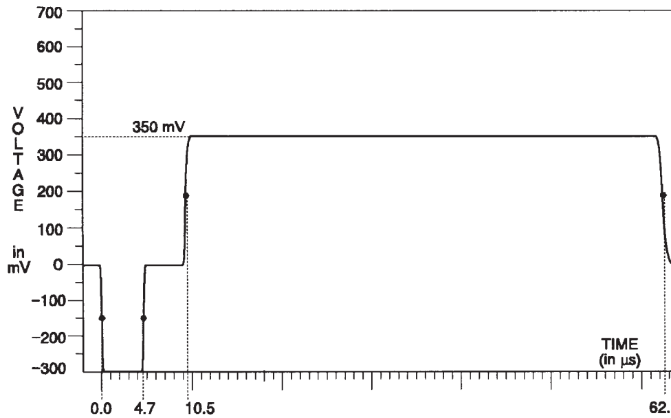
Fig. 3-84. Y Channel — 50% Flat Field.
