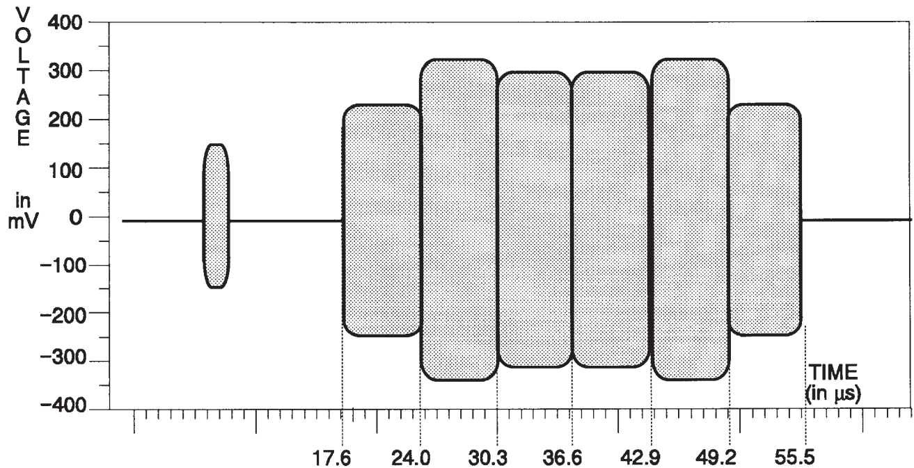
Fig. 3-33. C Channel — 75% Bars.
