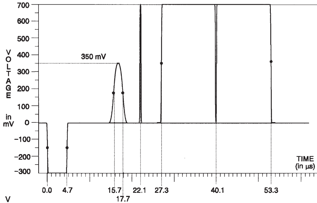
Fig. 3-226. Y Channel — Pulse & Bar.
