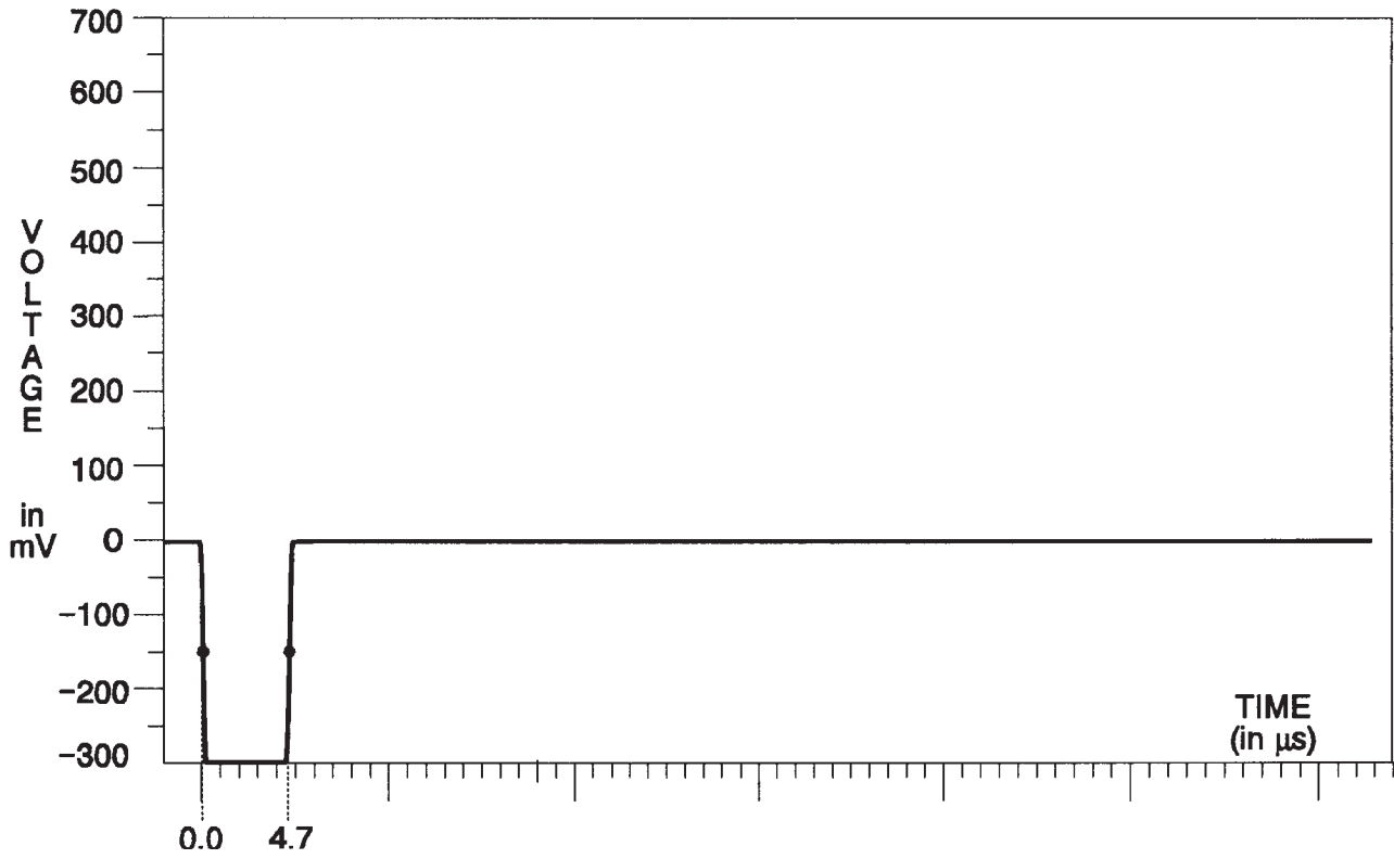
Fig. 3-46. Y Channel — 0% Flat Field.
