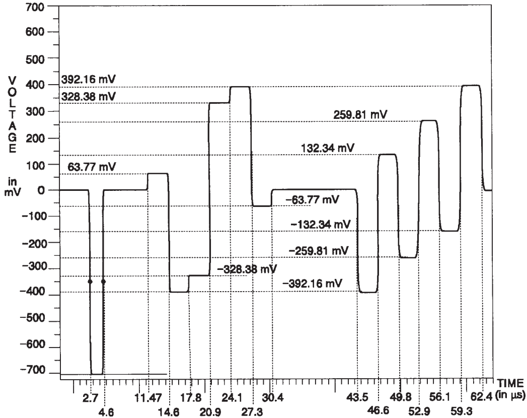
Fig. 3-106. C Channel — 100% Bars.
