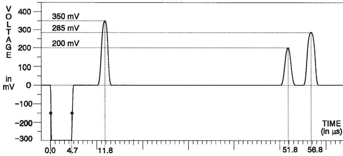
Fig. 3-208. Y Channel — 12T Pulses.
