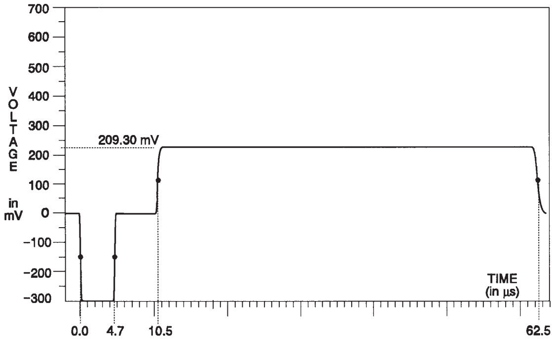
Fig. 3-80. Y Channel — 100% Red.
