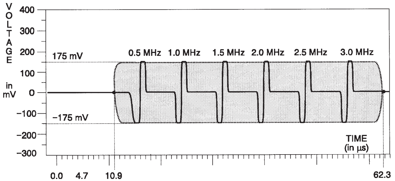
Fig. 3-97. B-Y & R-Y Channel — Reduced Line Sweep.
