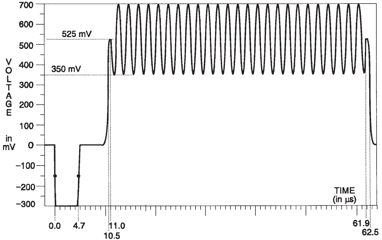
Fig. 3-137. Green Channel — Bowtie.
