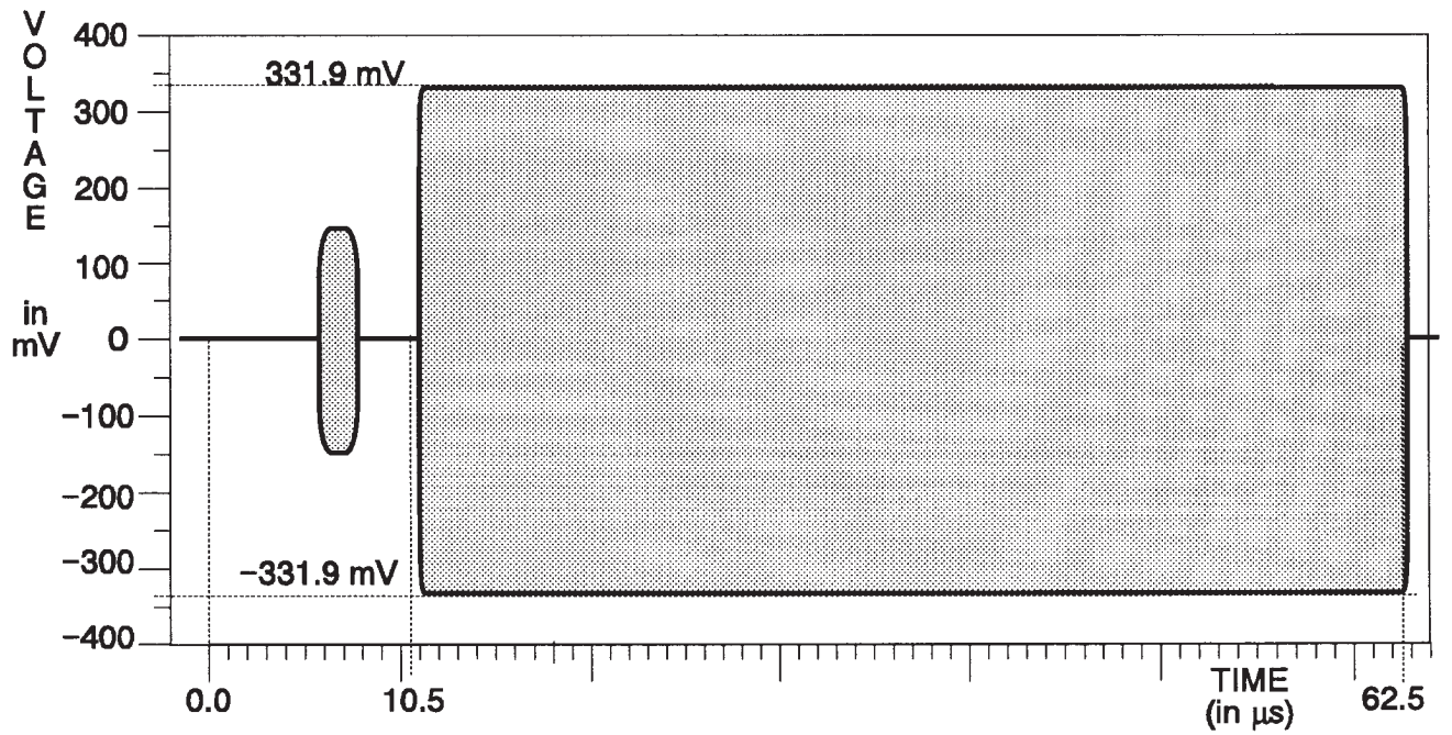
Fig. 3-35. C Channel — 75% Red (Same as Red Field)
