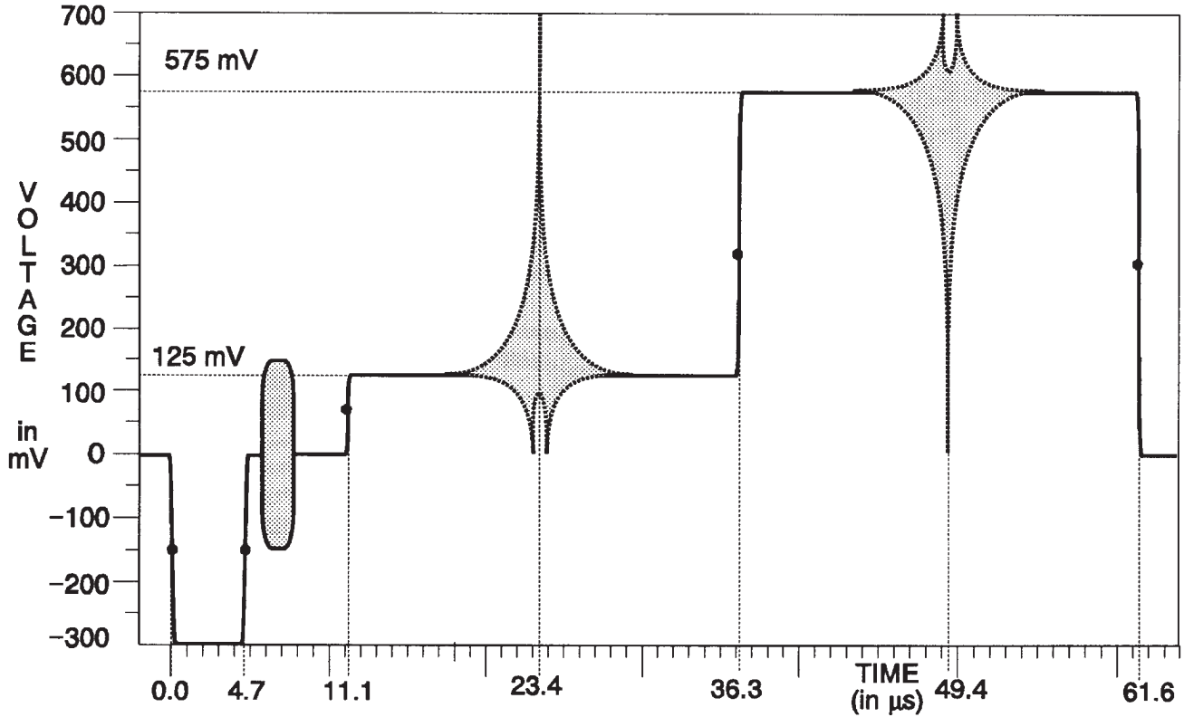
Fig. 3-28. Matrix Signal — \text{Sin}(x)/x .
