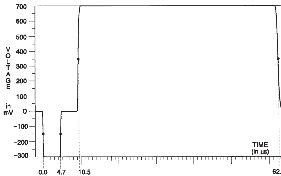
Fig. 3-85. Y Channel — 100% Flat Field.
