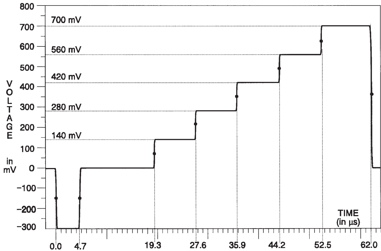
Fig. 3-190. Y Channel — 5-Step.
