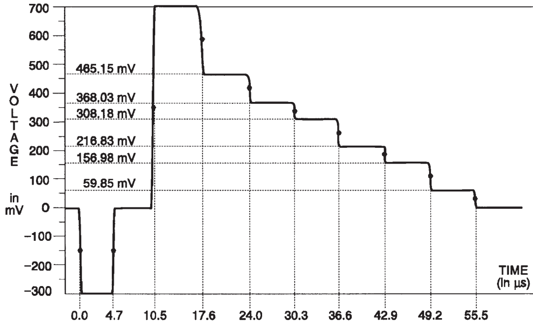
Fig. 3-71. Y Channel — 75% Bars.
