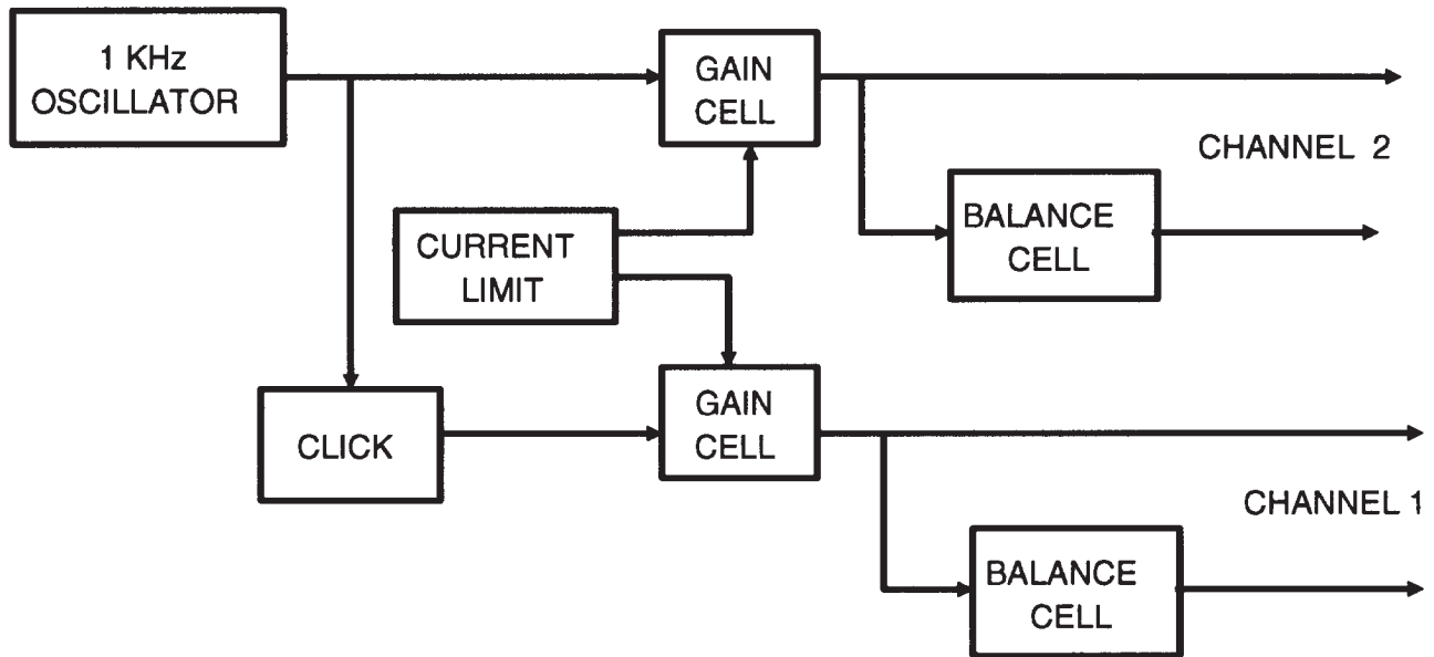
Fig. 7. Block diagram of the Audio circuitry.
