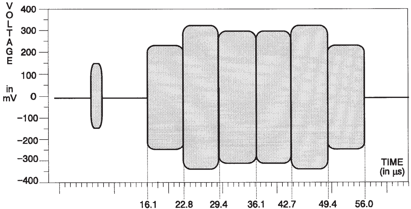
Fig. 3-150. C Channel — 75% Bars.
