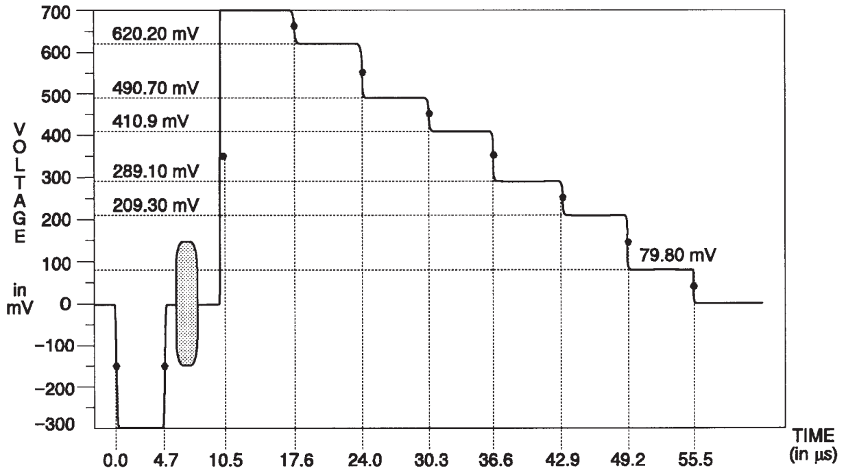
Fig. 3-242. Y Channel — 100% Bars.
