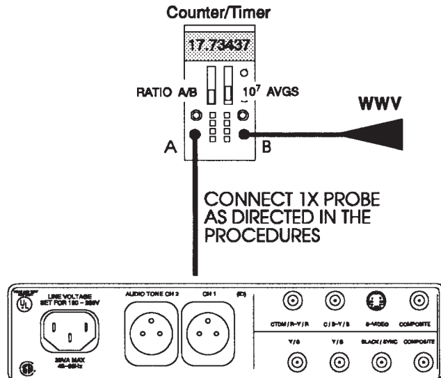
Fig. 4-1. Setup to check the crystal frequency.
