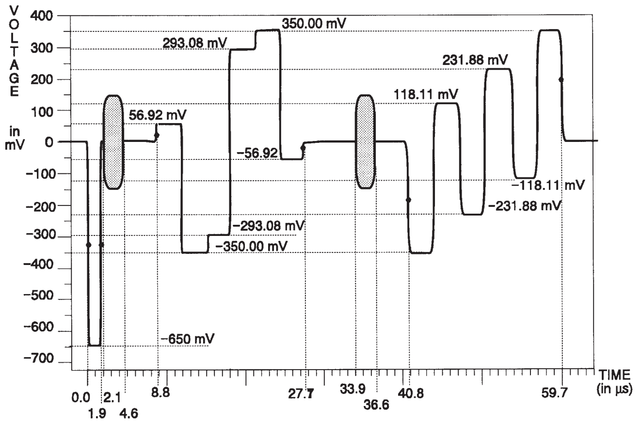
Fig. 3-243. C Channel — 100% Bars.
