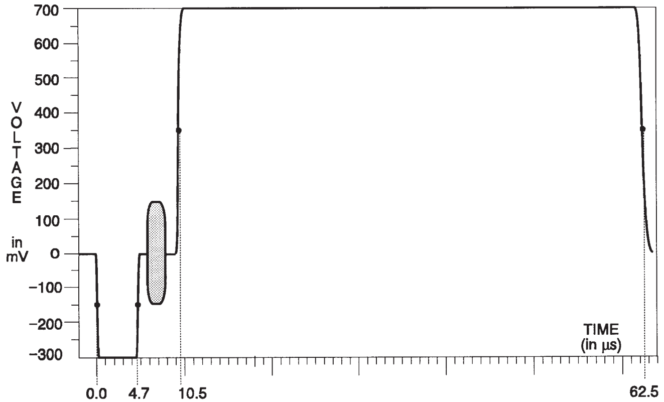
Fig. 3-148. Y Channel — 100% Flat Field.
