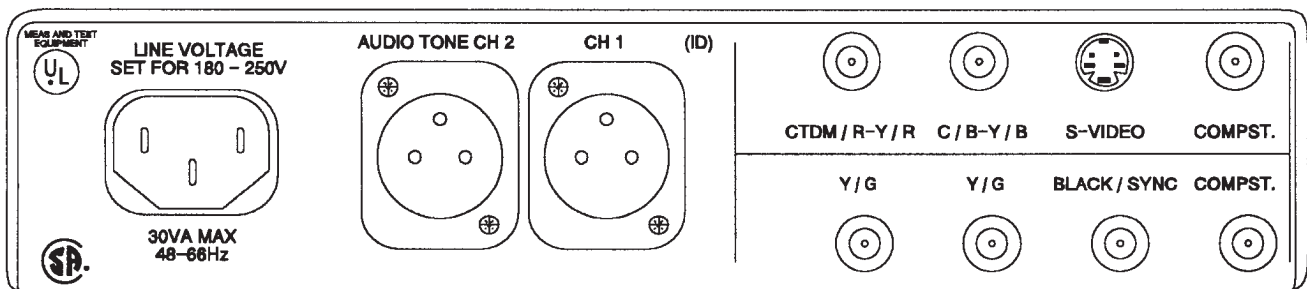
Fig. 1-2. Rear panel of the TSG 131A.
