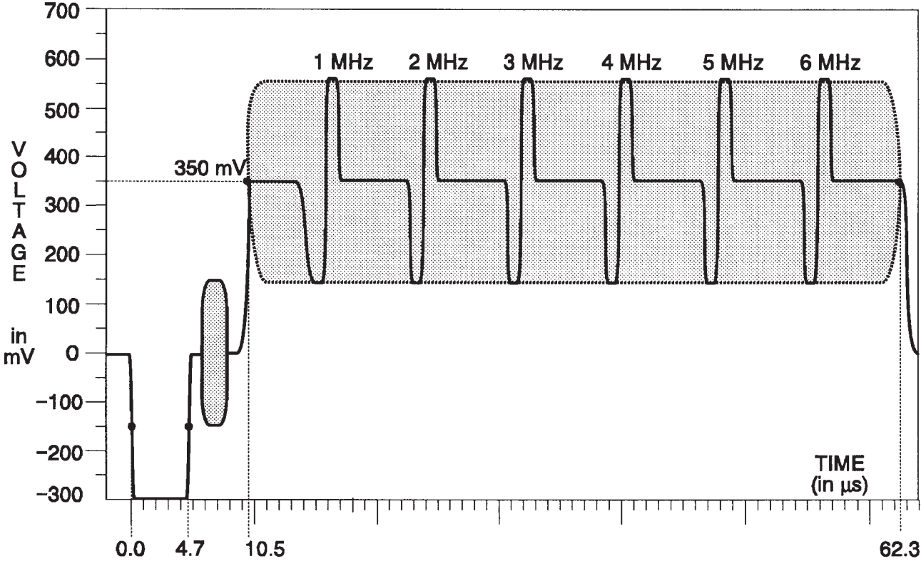
Fig. 3-21. Reduced Sweep.
