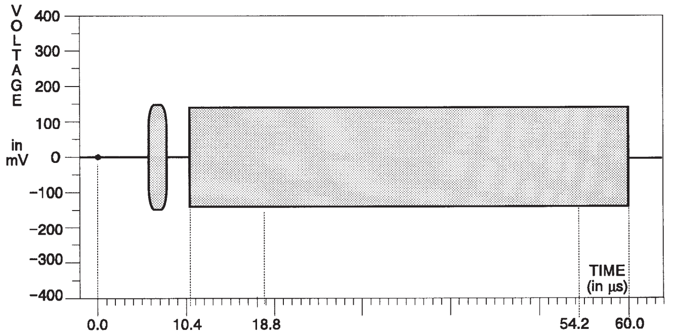
Fig. 3-61. C Channel — Modulated Ramp.
