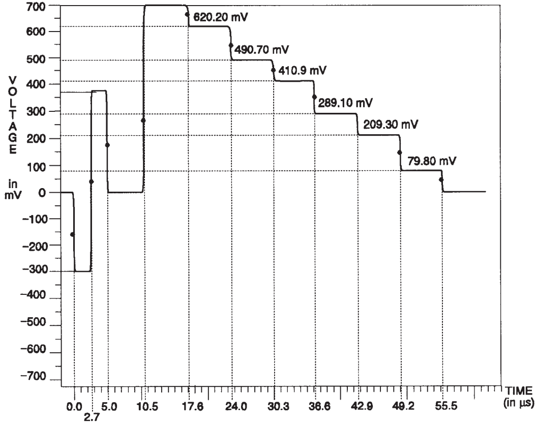
Fig. 3-105. Y Channel — 100% Bars.
