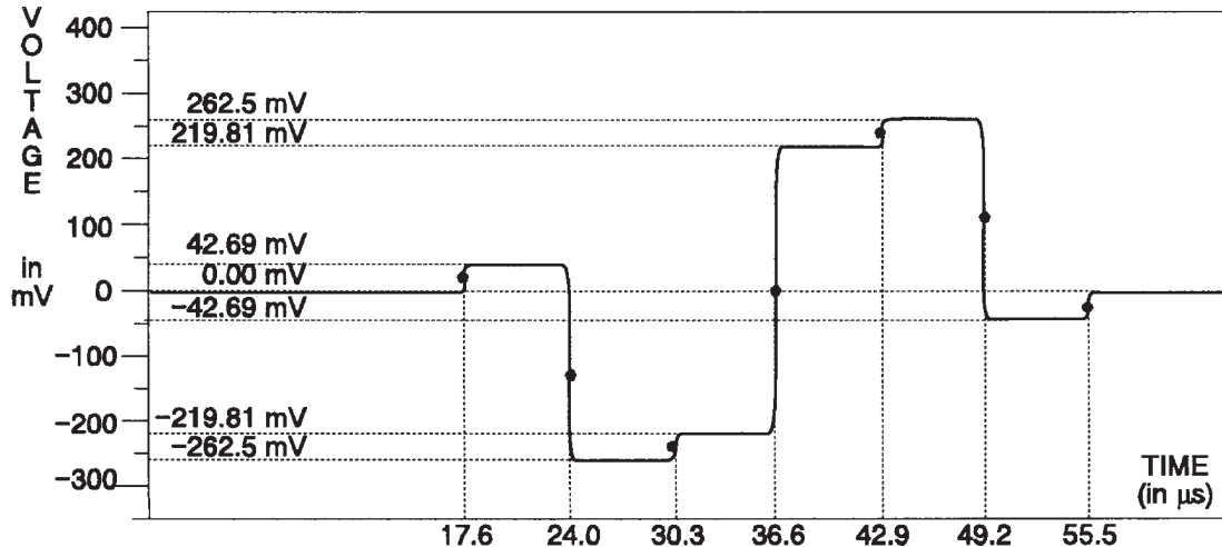
Fig. 3-223. R-Y Channel — 75% Bars.
