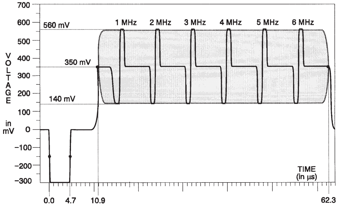
Fig. 3-94. Y Channel — Line Sweep.
