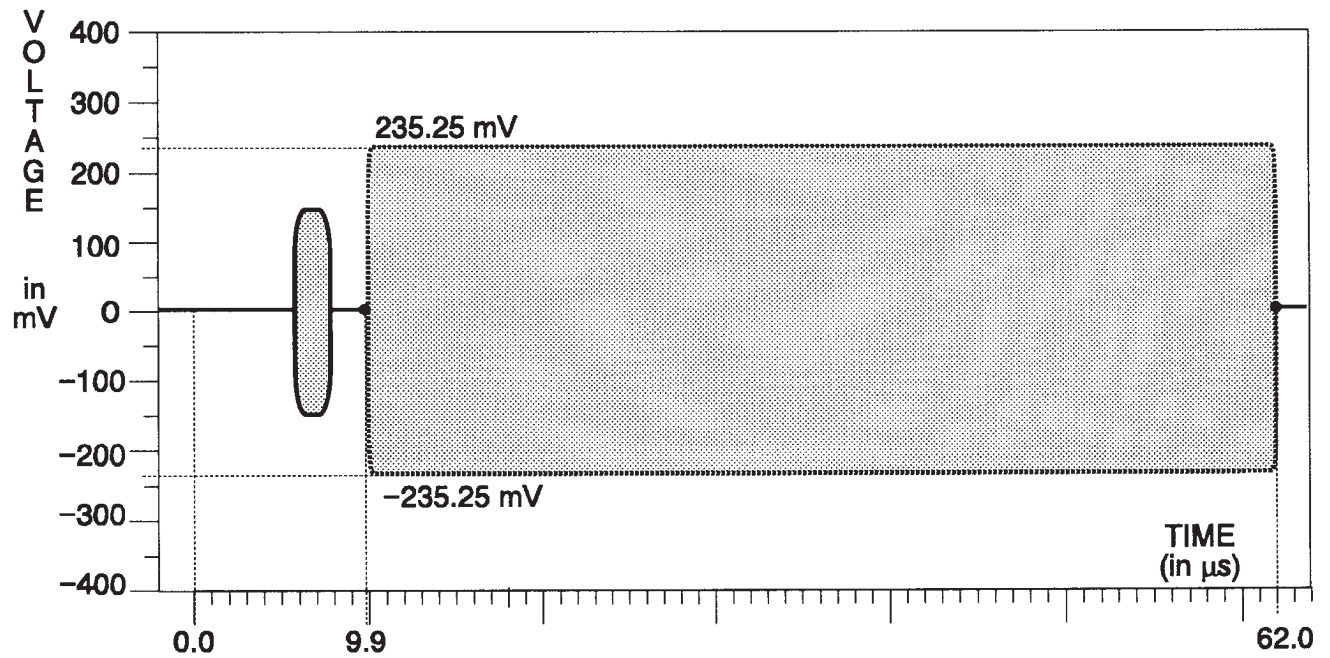
Fig. 3-158. C Channel — Blue Field.
