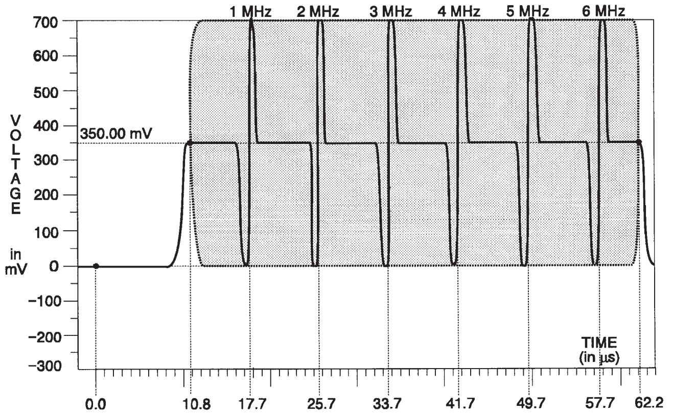
Fig. 3-136. Blue & Red Channels — Sweep.
