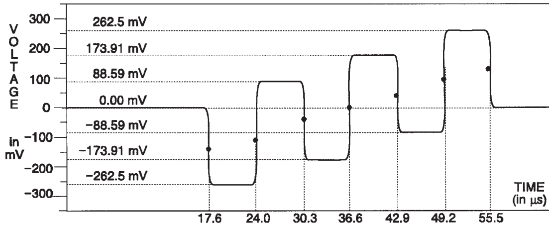
Fig. 3-72. B-Y Channel — 75% Bars.
