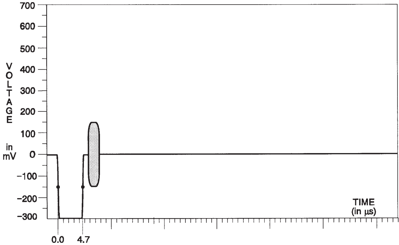
Fig. 3-1. Black Burst.
