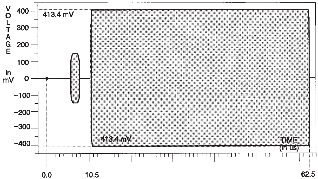
Fig. 3-39. C Channel — 100% Red.
