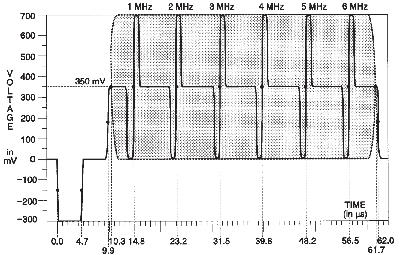
Fig. 3-169. Y Channel — Sweep.
