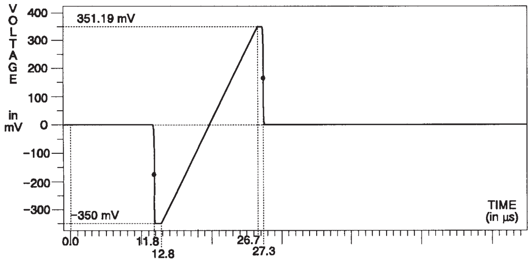
Fig. 3-193. B-Y Channel — Quad Phase.
