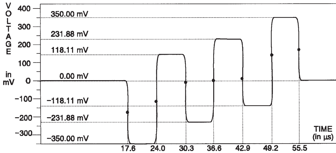
Fig. 3-75. B-Y Channel — 100% Bars.
