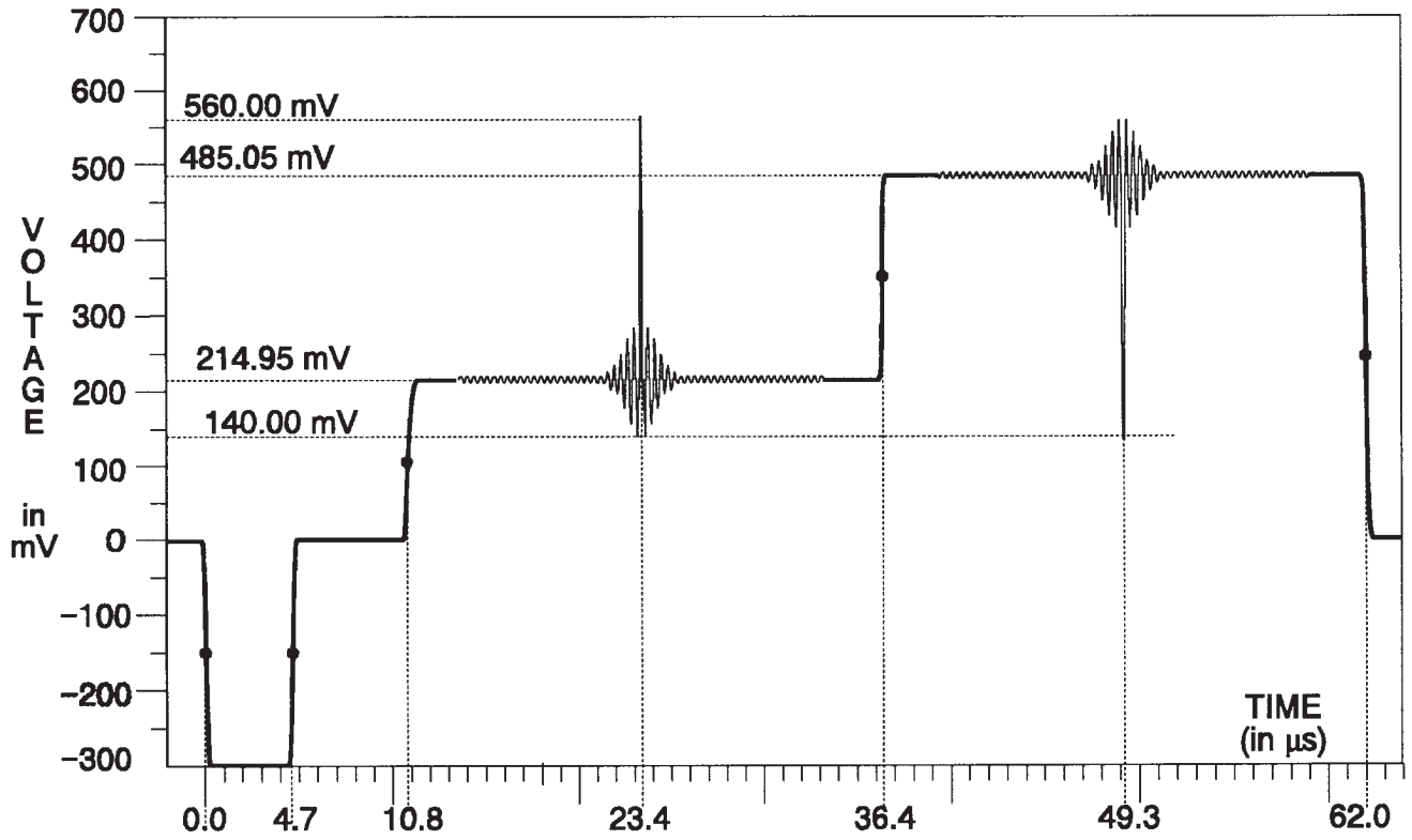
Fig. 3-188. Y Channel — Sin(x)/x.
