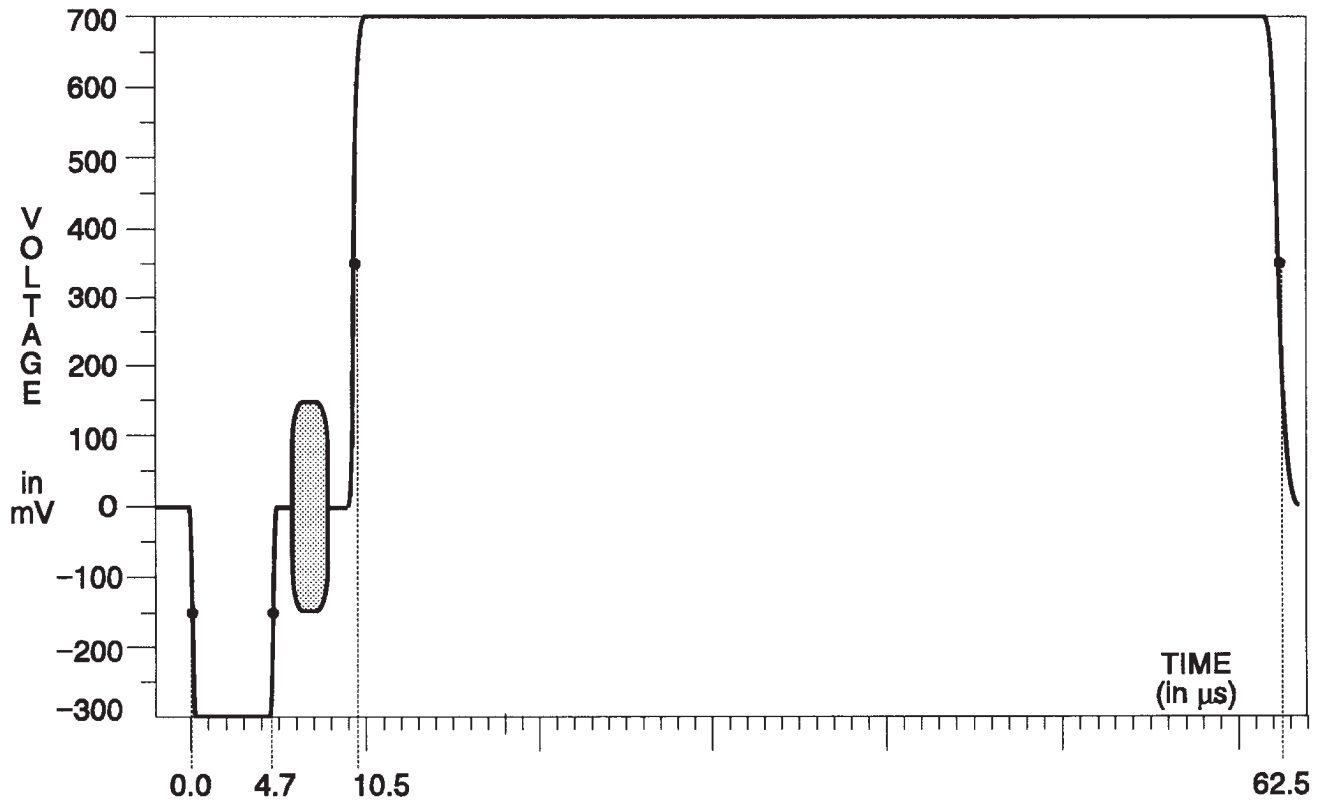
Fig. 3-145. Y Channel — 0% Flat Field.
