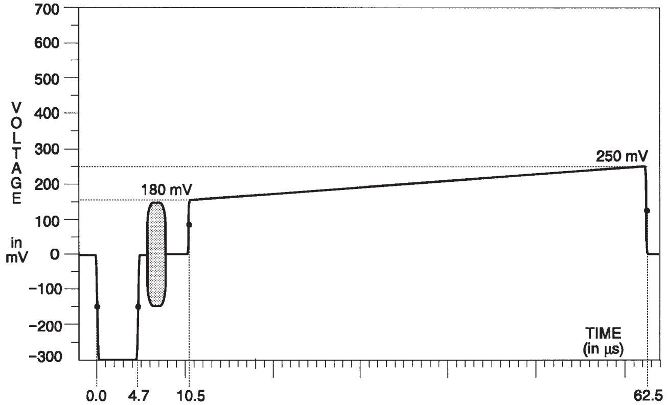
Fig. 3-30. Matrix Signal — Shallow Ramp.
