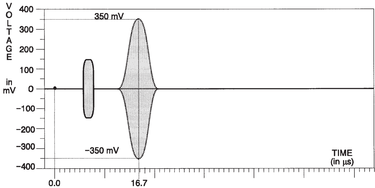
Fig. 3-55. C Channel — Pulse & Bar with Window.
