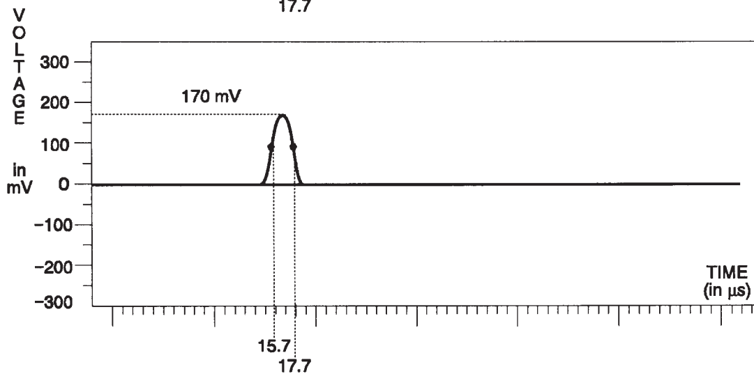
Fig. 3-90. B-Y Channel — Pulse & Bar with Window.
