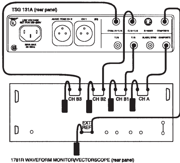
Fig. 4-2. Basic setup for the Performance Checks.
