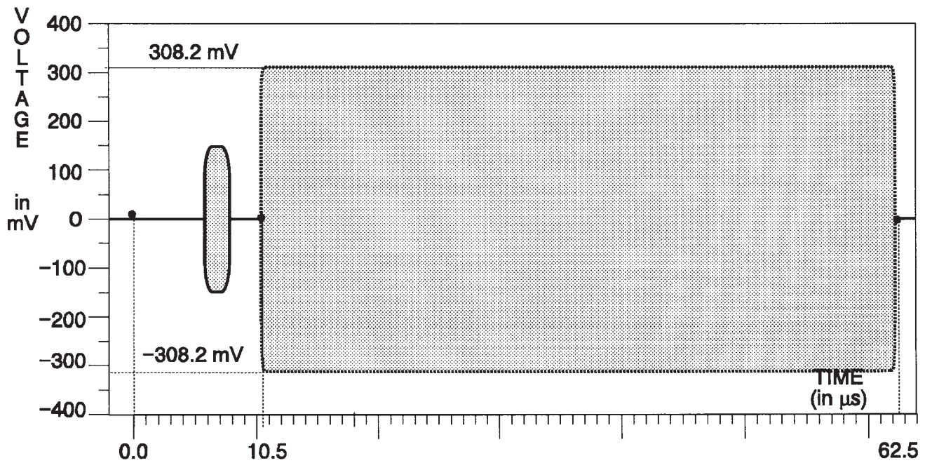
Fig. 3-45. C Channel — Green Field.
