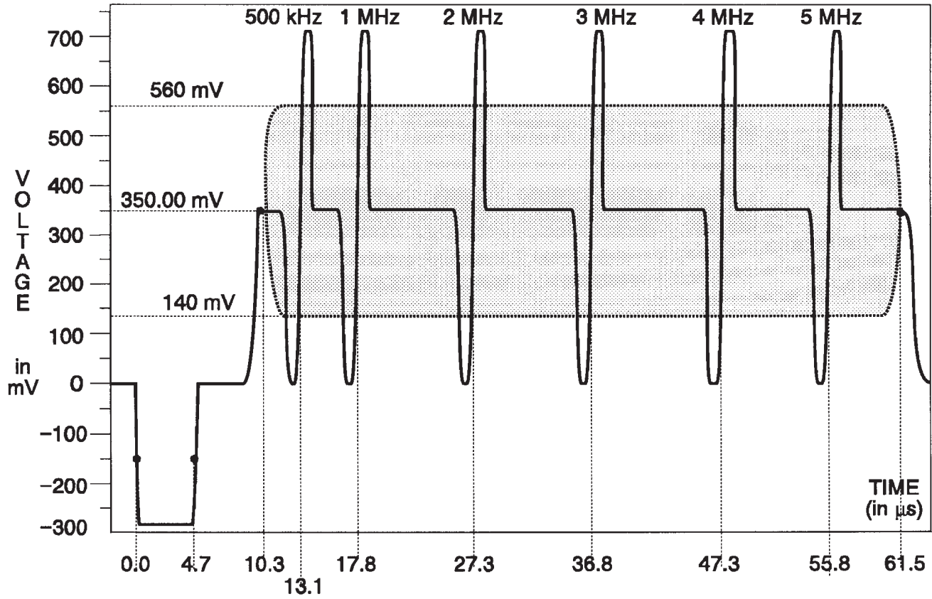
Fig. 3-203. Y Channel — 60% Narrow Sweep.
