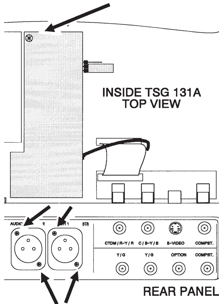
Fig. 5-1. Remove these 5 screws with a Pozidrive® screwdriver in order to take out the Audio board for adjustment of the Black Burst/Comp Sync output.
