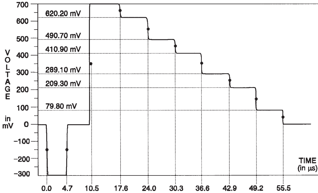
Fig. 3-74. Y Channel — 100% Bars.
