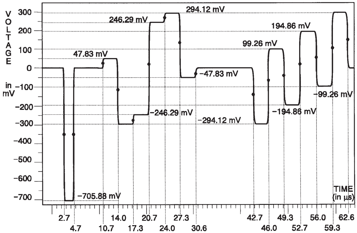
Fig. 3-212. C Channel — 75% Bars.
