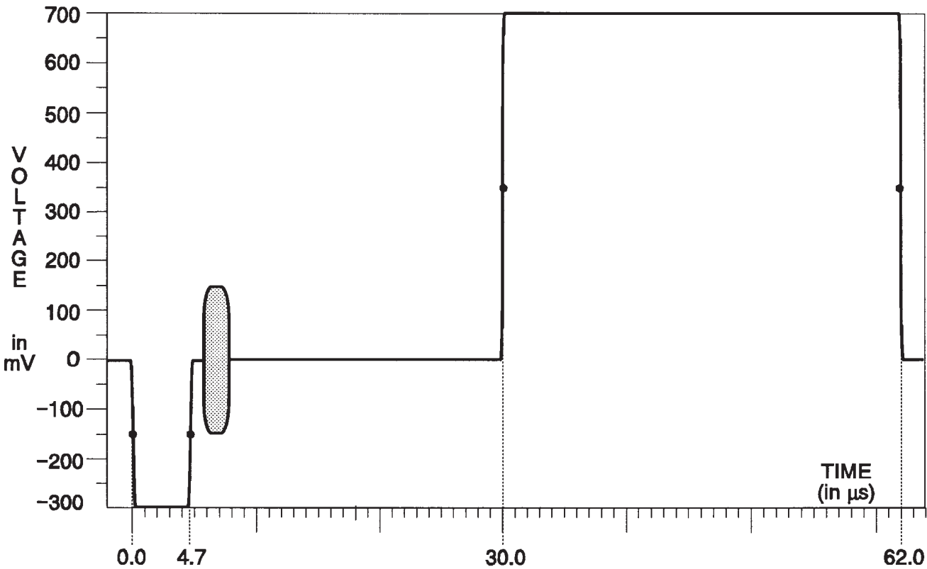
Fig. 3-29. Matrix Signal — 15 kHz Square Wave.
