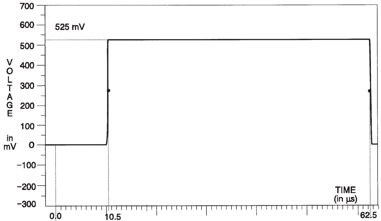
Fig. 3-126. Blue & Red Channels — Convergence (hor).
