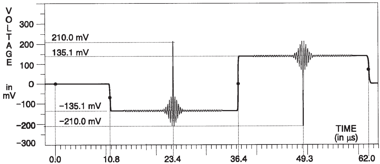
Fig. 3-189. B-Y & R-Y Channels — Sin(x)/x.
