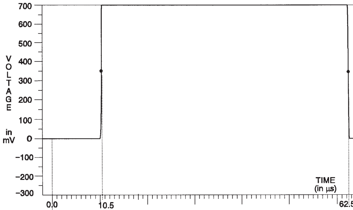
Fig. 3-121. Blue Channel — Blue Field.
