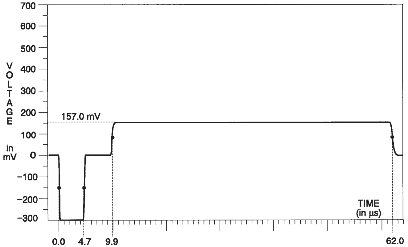
Fig. 3-151. Y Channel — 75% Red (same as Red Field).
