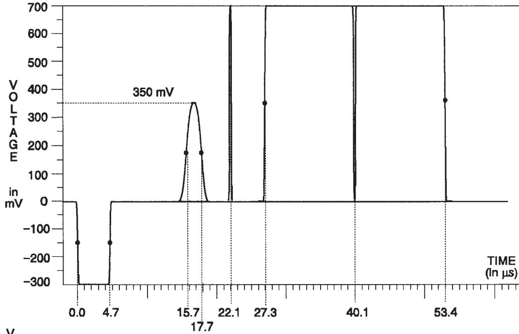
Fig. 3-89. Y Channel — Pulse & Bar with Window.
