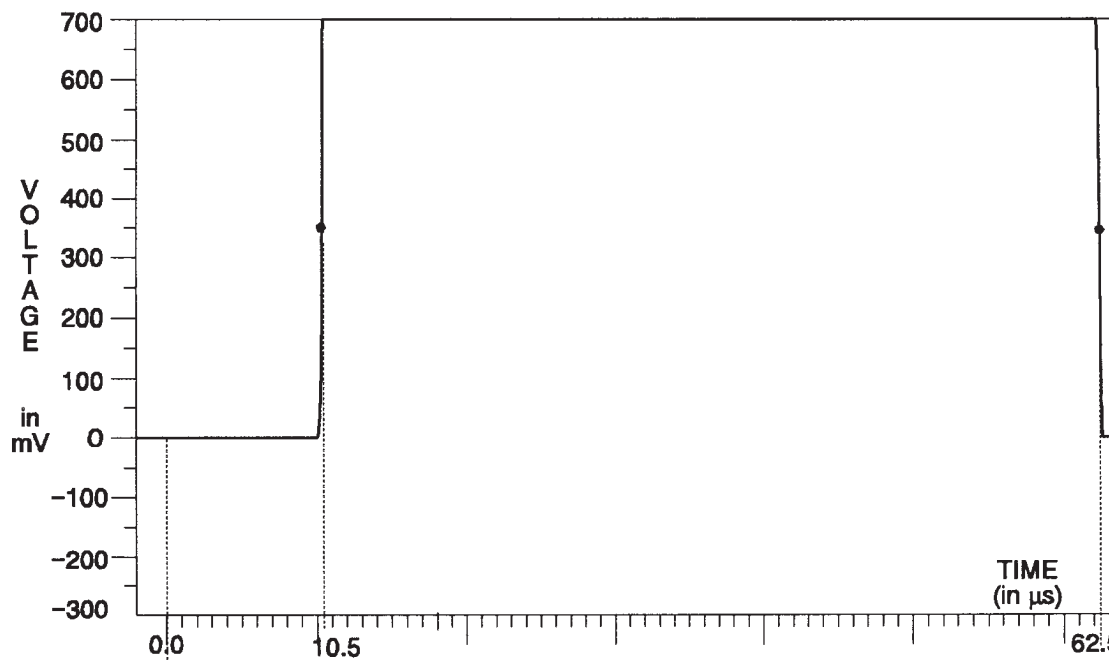
Fig. 3-119. Red Channel — Red Field.
