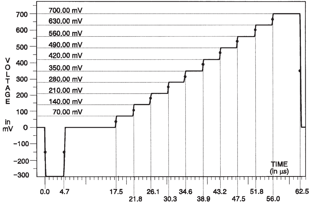
Fig. 3-129. Green Channel — 10-Step.
