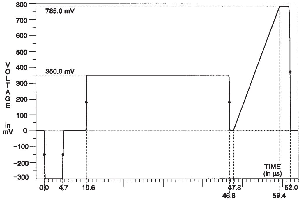
Fig. 3-192. Y Channel — Quad Phase.
