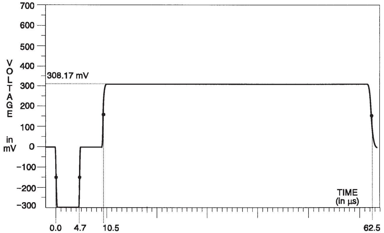
Fig. 3-44. Y Channel — Green Field.
