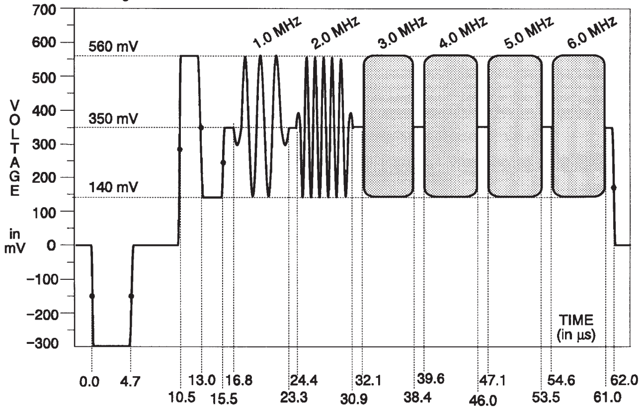
Fig. 3-133. Green Channel — Multiburst.
