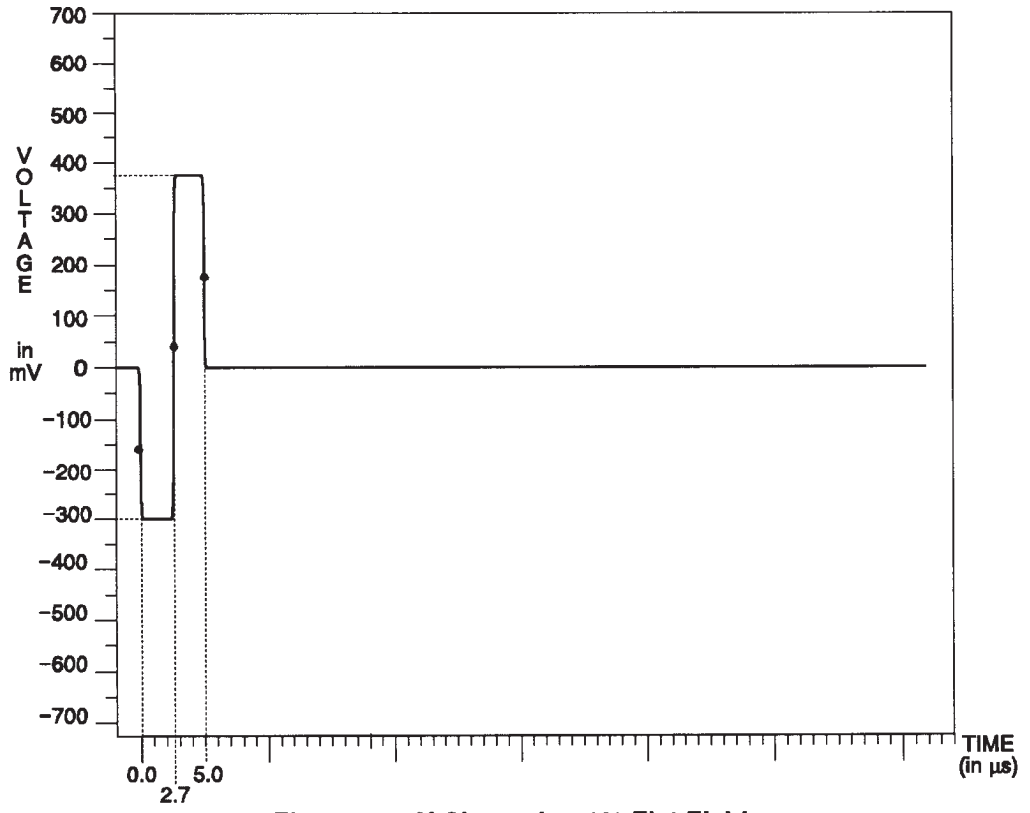
Fig. 3-108. Y Channel — 0% Flat Field.
