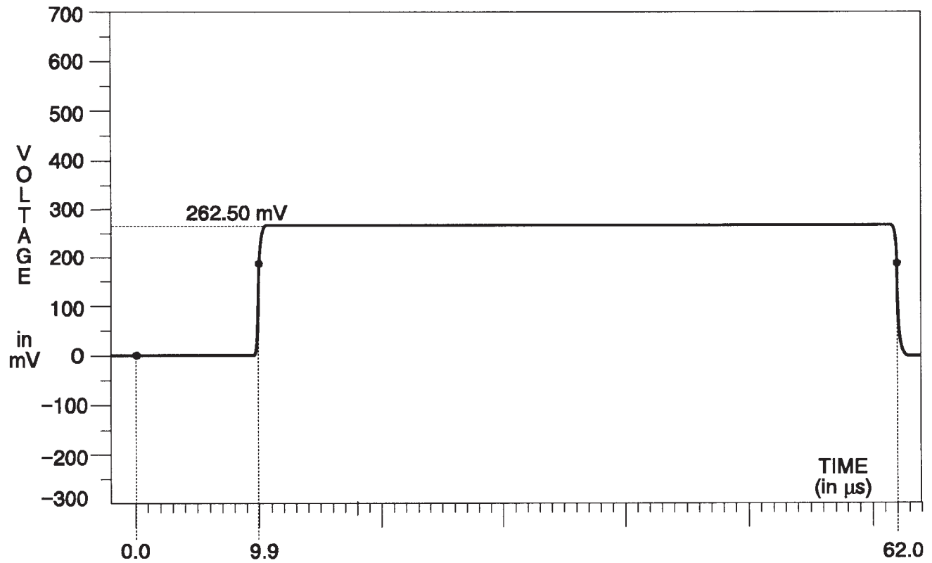
Fig. 3-187. B-Y & R-Y Channels — Flat Field.
