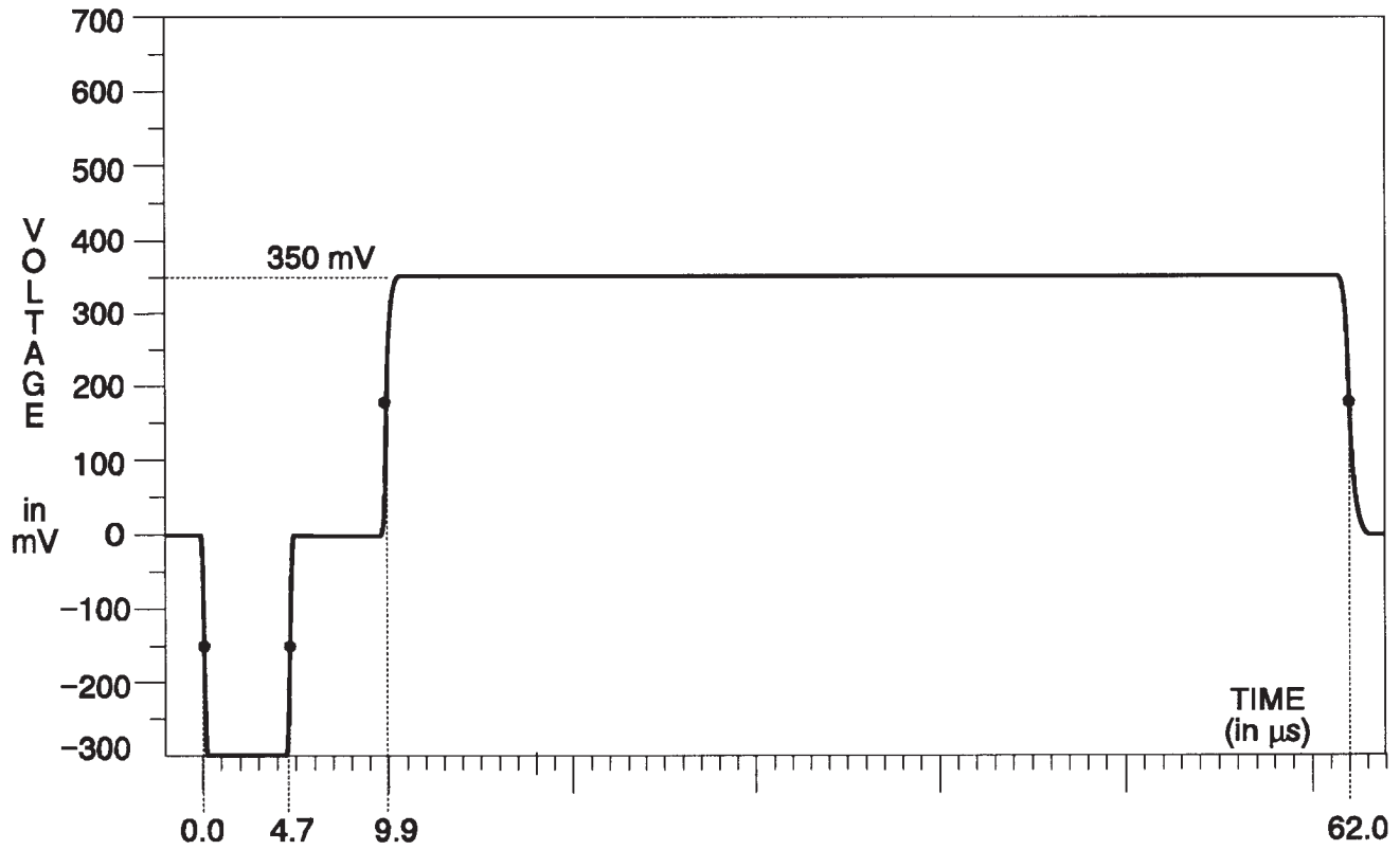
Fig. 3-163. Y Channel — Chroma Noise.
