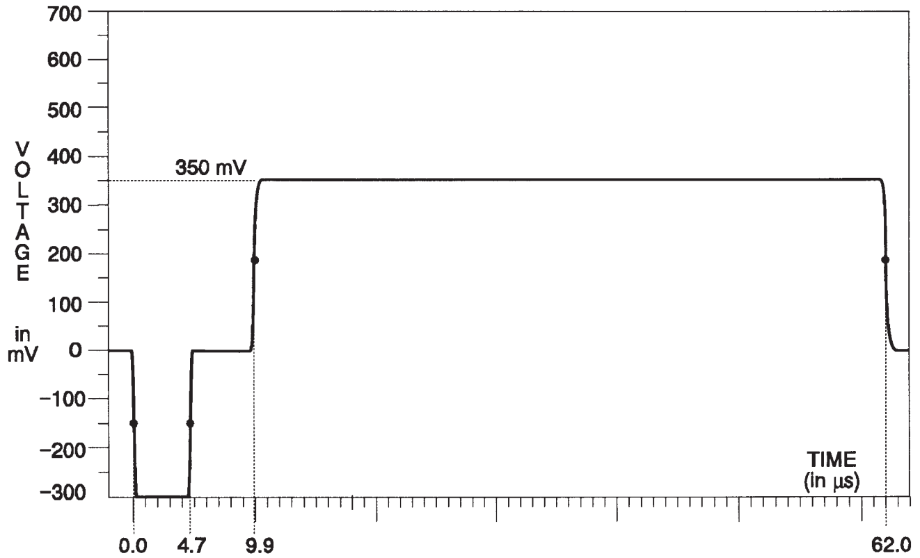
Fig. 3-186. Y Channel — Flat Field in all Channels.
