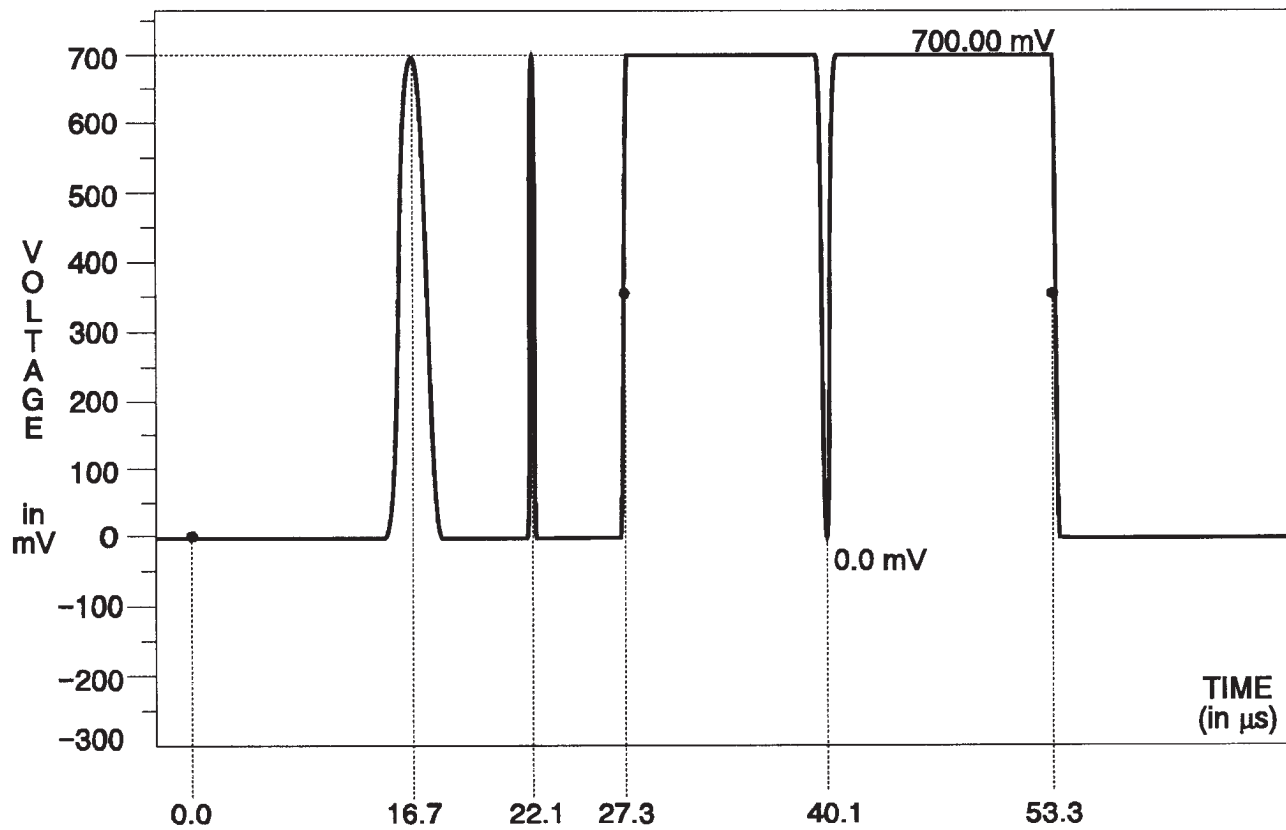
Fig. 3-132. Blue & Red Channels — Pulse & Bar.
