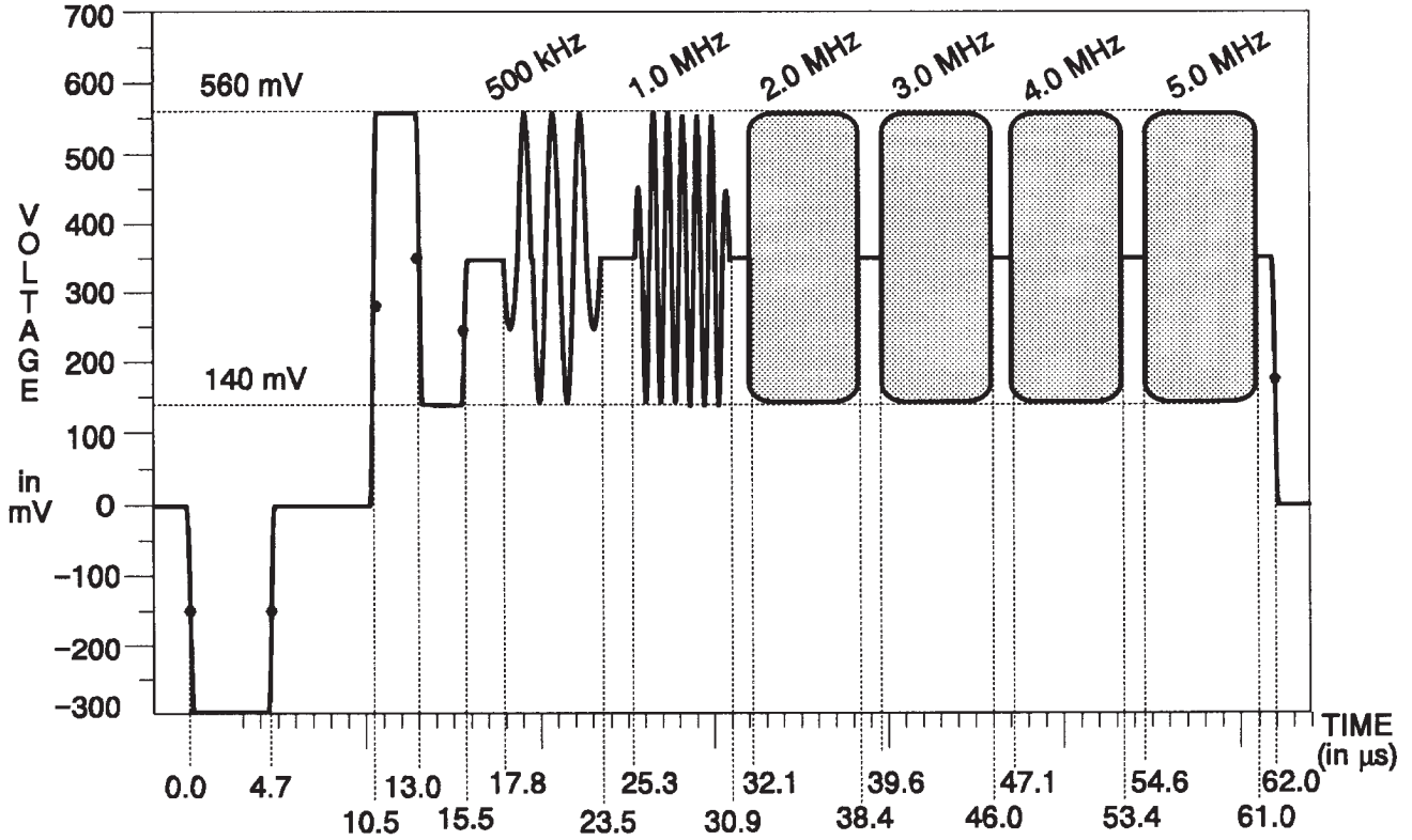
Fig. 3-101. Y Channel — Multiburst.
