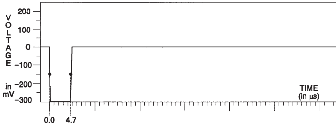
Fig. 3-117. Green Channel — Red Field.
