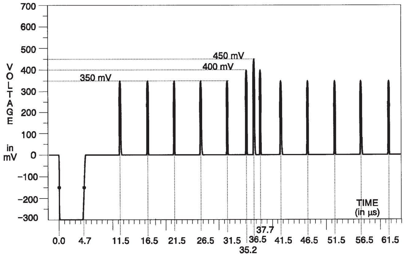
Fig. 3-139. Green Channel — Bowtie Markers.
