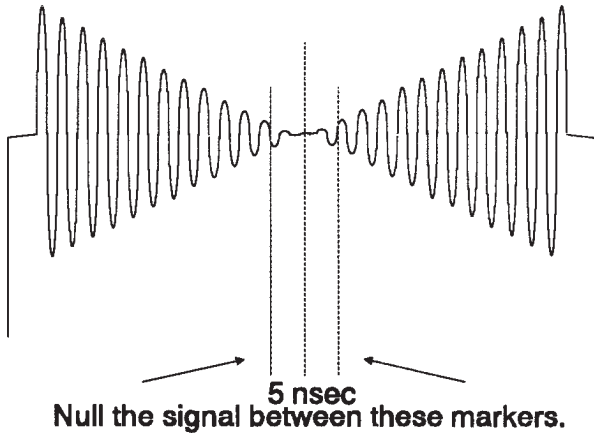
Fig. 4-13. Bowtie crossing.
