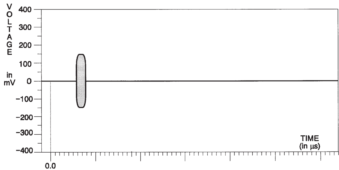
Fig. 3-49. C Channel — 50% Flat Field.
