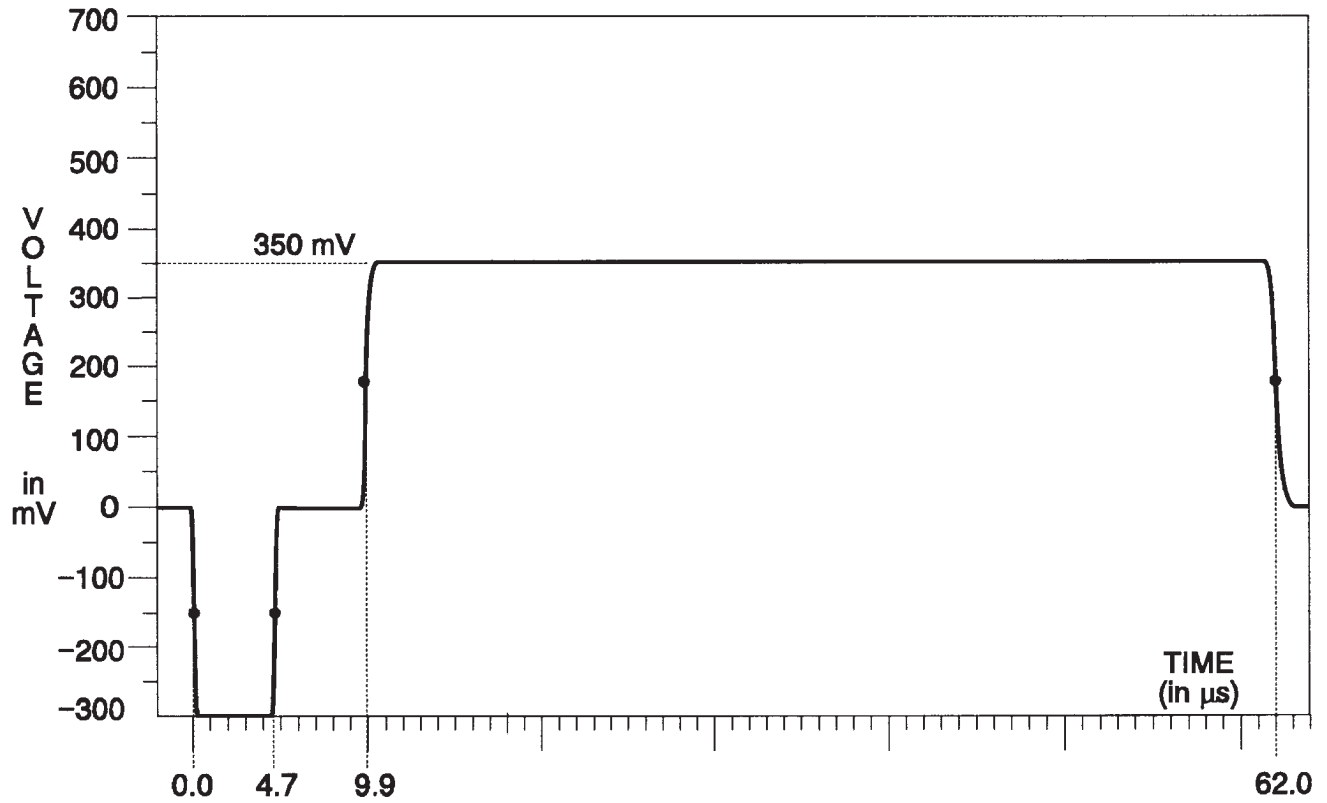
Fig. 3-161. Y Channel — 50% Flat Field.
