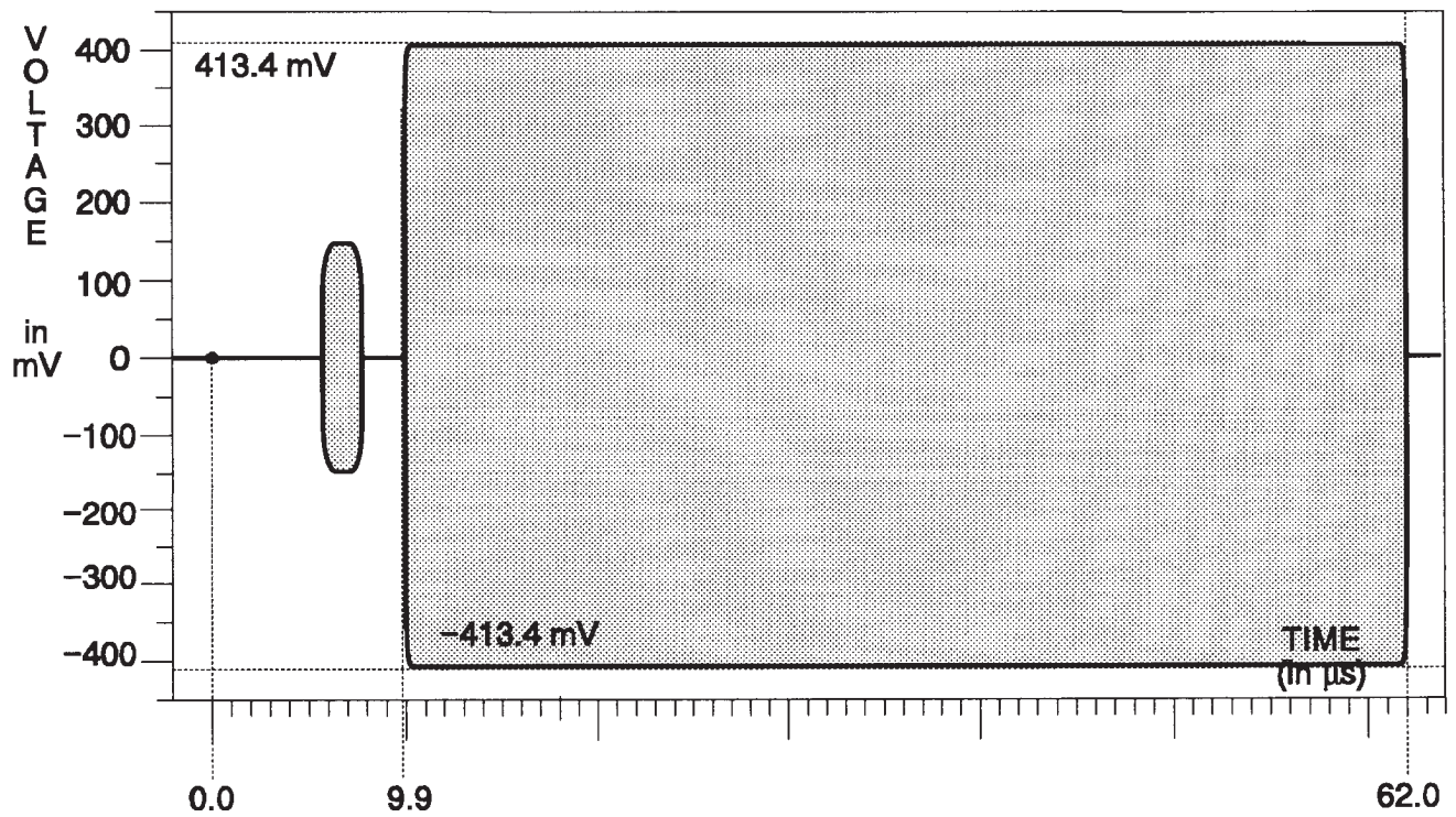
Fig. 3-156. C Channel — 100% Red.
