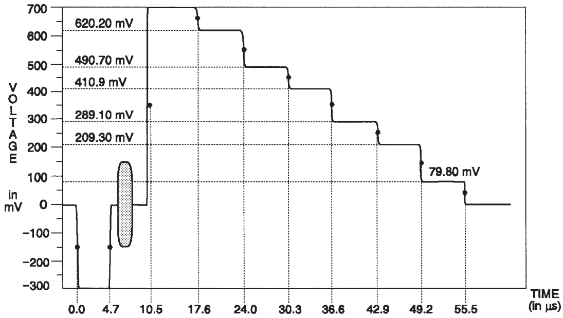
Fig. 3-143. Y Channel — 100% Color Bars.
