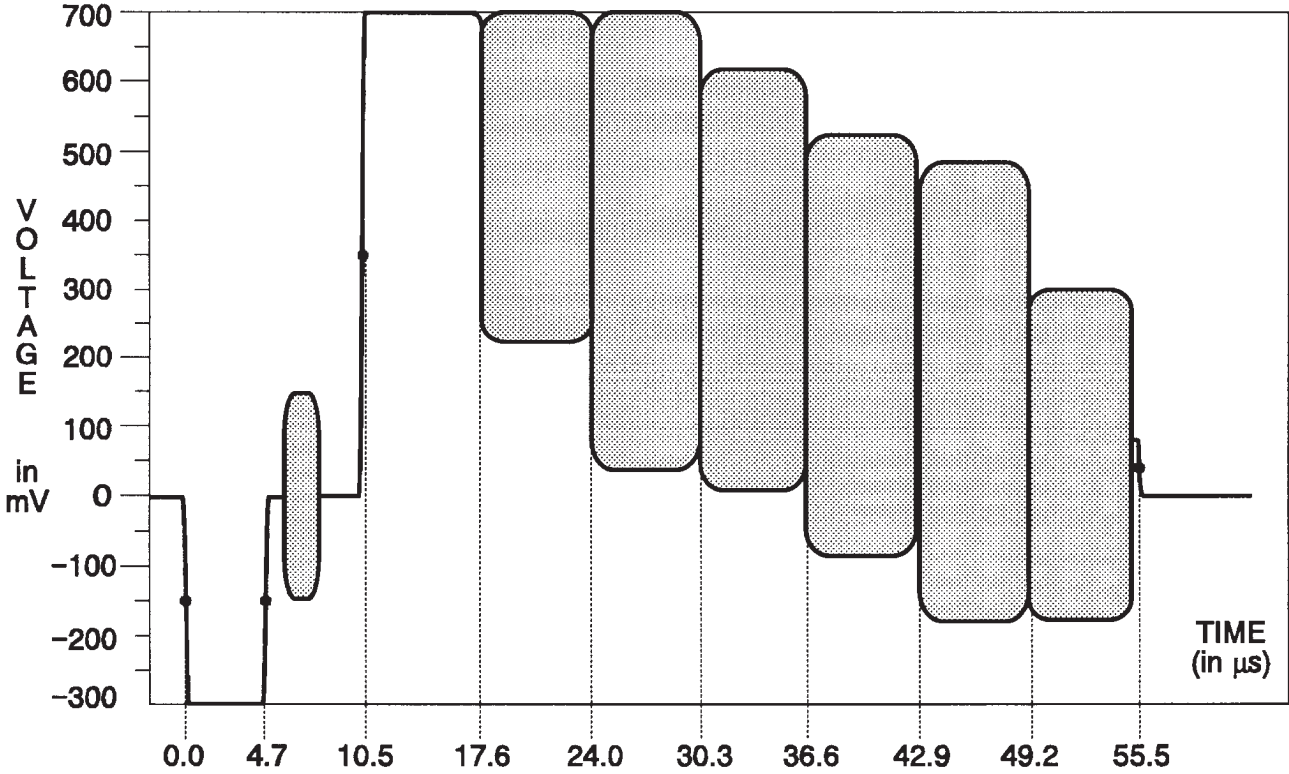
Fig. 3-2. 75% Color Bars.
