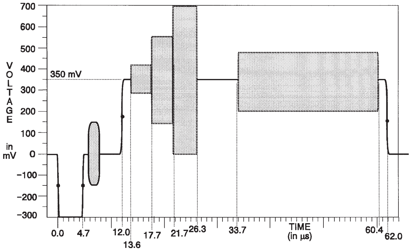
Fig. 3-27. Matrix Signal — CCIR Line 331.
