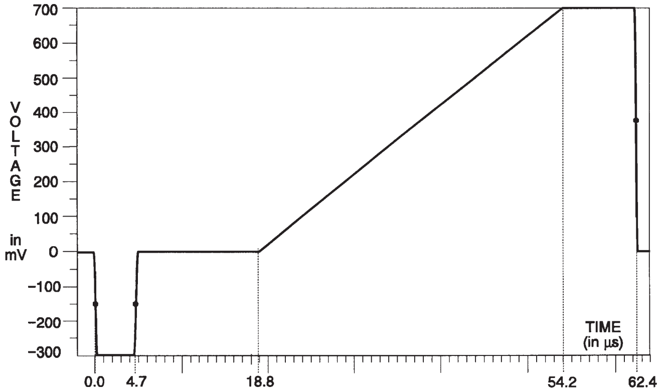
Fig. 3-60. Y Channel — Modulated Ramp.
