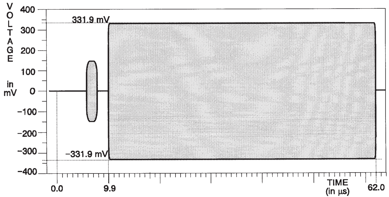
Fig. 3-152. C Channel — 75% red (same as Red Field).
