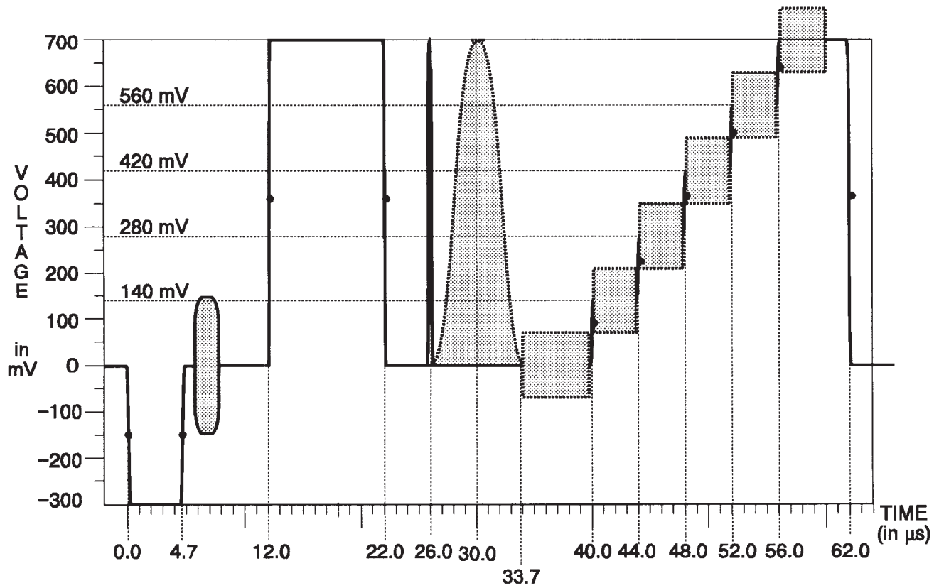
Fig. 3-31. Matrix Signal — UK ITS 1.
