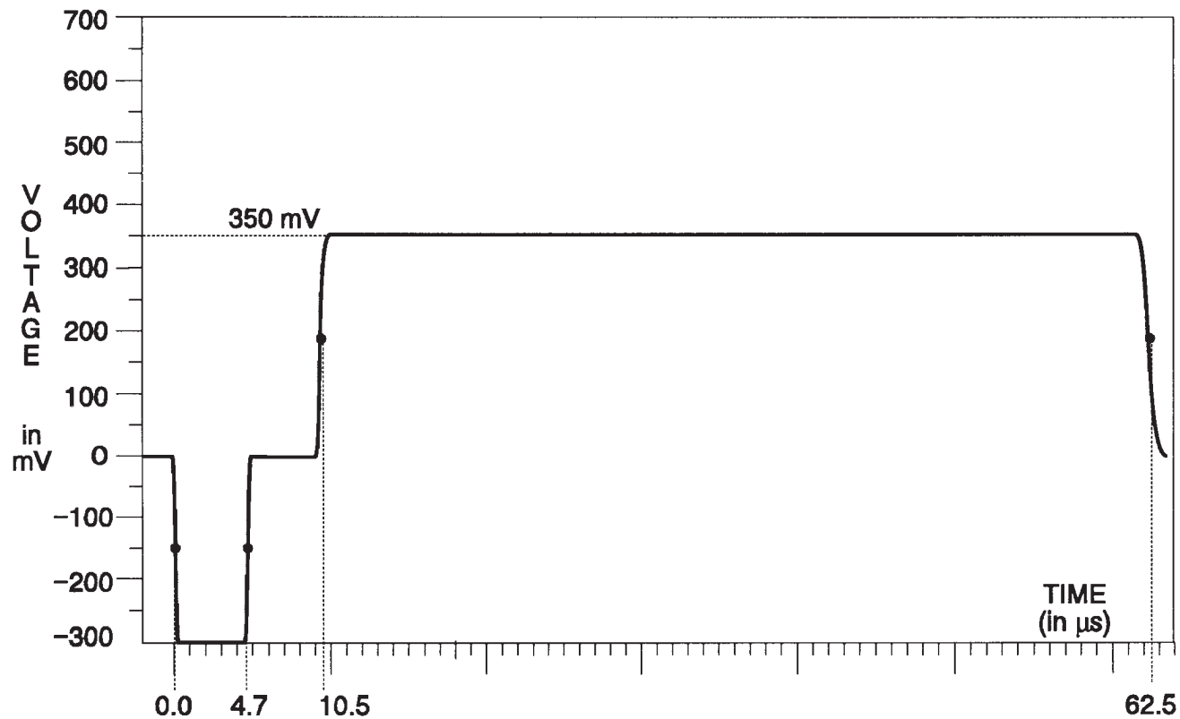
Fig. 3-48. Y Channel — 50% Flat Field.
