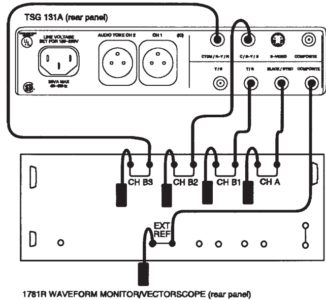
Fig. 4-14. Setup to calibrate the BLACK BURST output.
