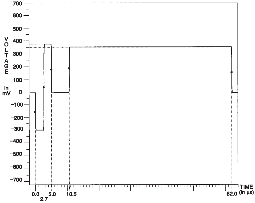
Fig. 3-109. Y Channel — 50% Flat Field.
