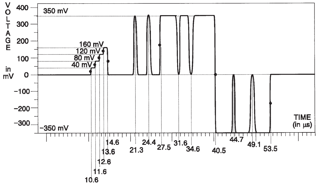
Fig. 3-93. B-Y Channel — T Pulses.
