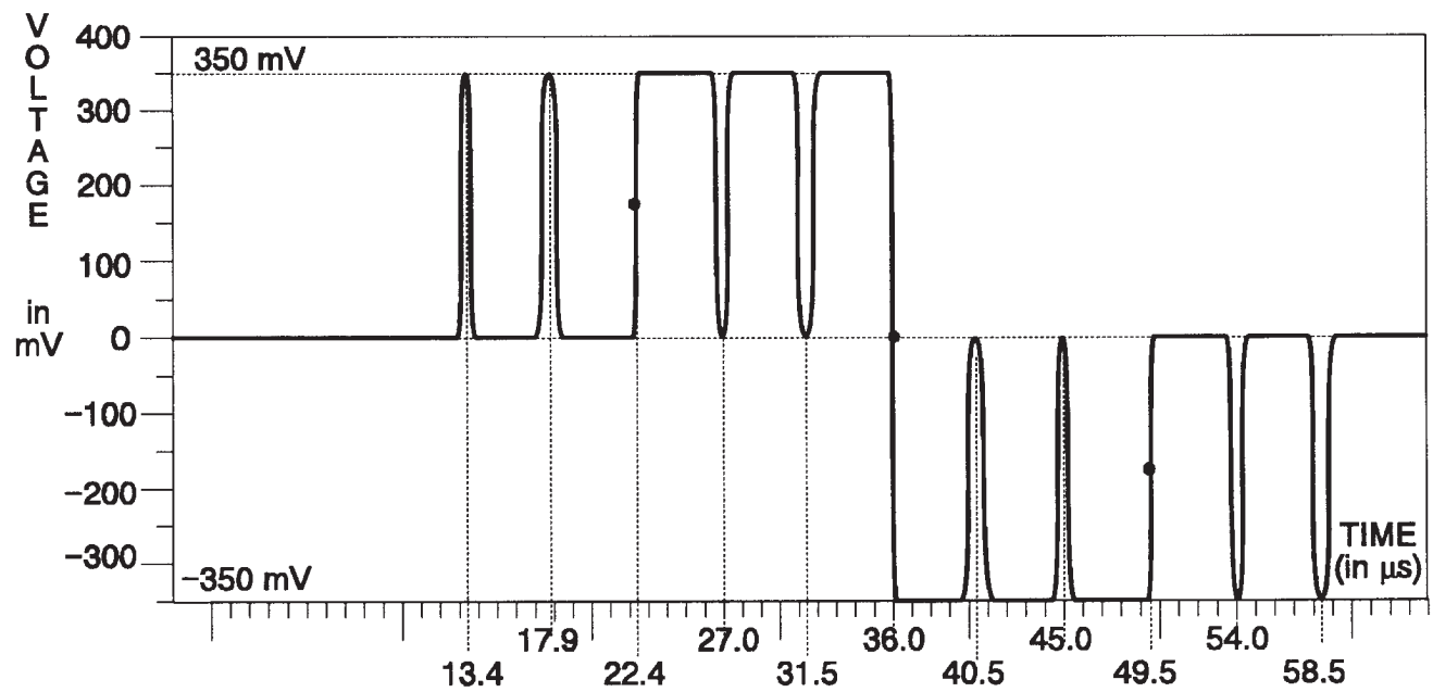
Fig. 3-196. B-Y Channel — T Pulses.
