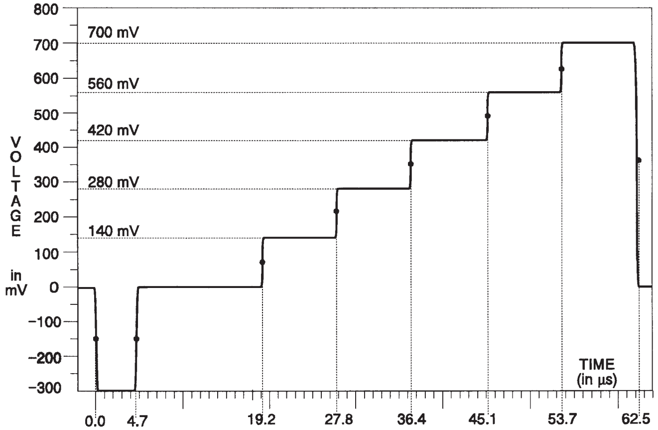
Fig. 3-231. Y Channel — 5-Step.
