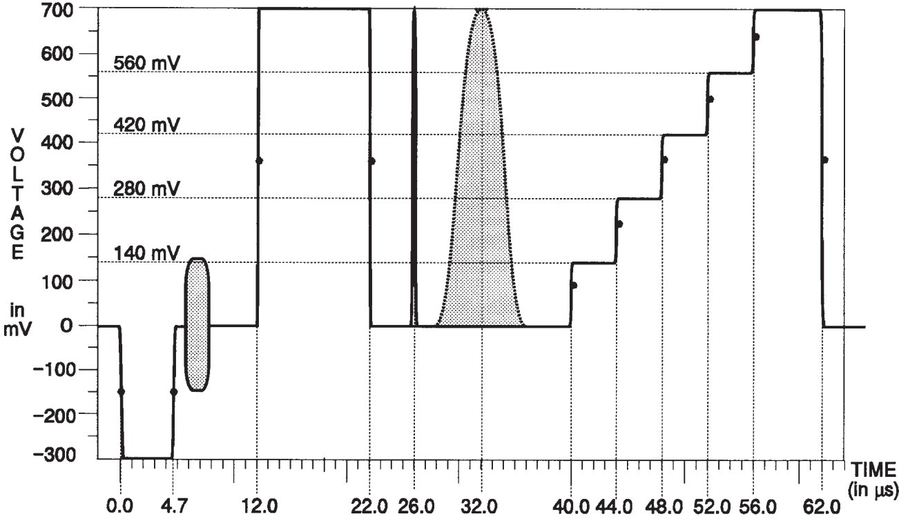
Fig. 3-24. Matrix Signal — CCIR Line 17.
