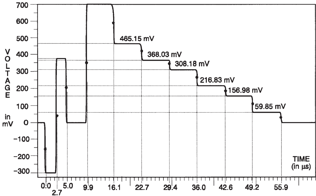
Fig. 3-211. Y Channel — 75% Bars.
