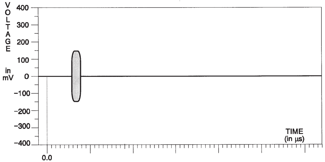
Fig. 3-51. C Channel — 100% Flat Field.
