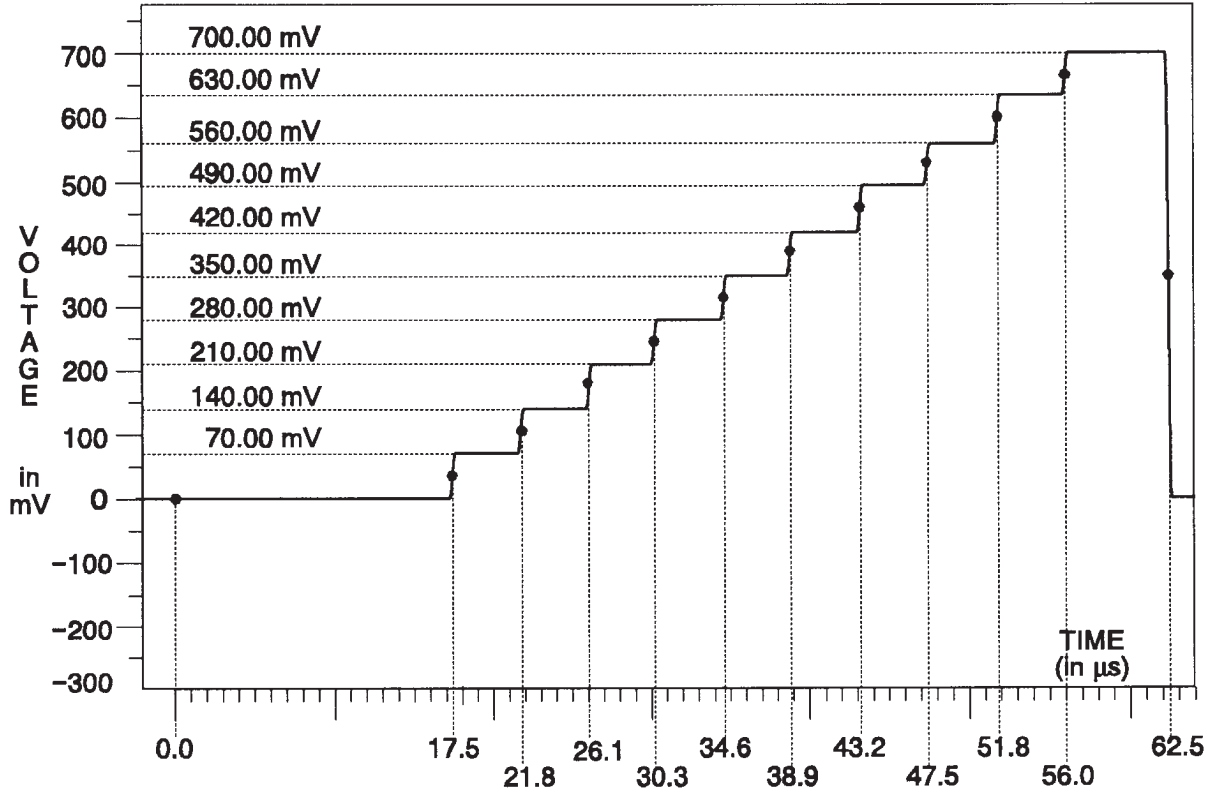
Fig. 3-130. Blue & Red Channels — 10-Step.
