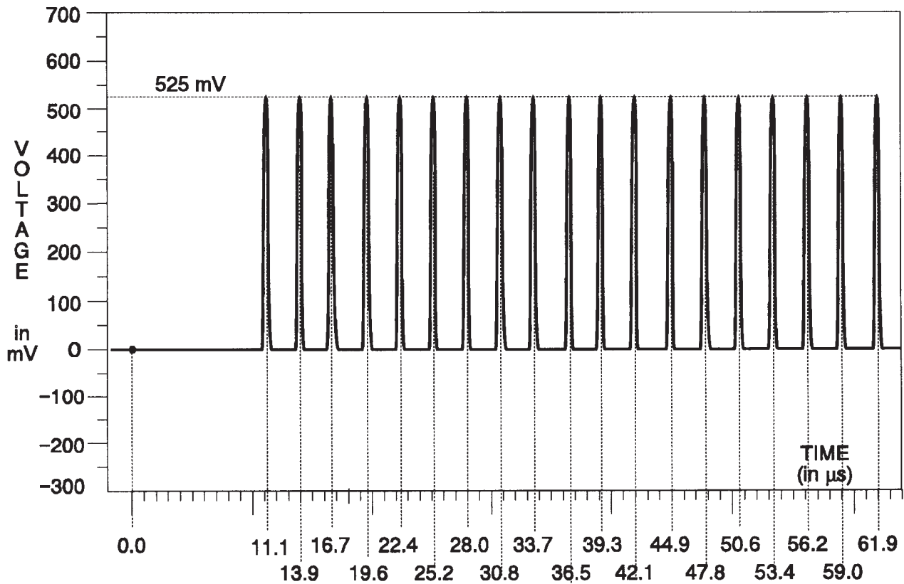
Fig. 3-128. Blue & Red Channels — Convergence (vrt).
