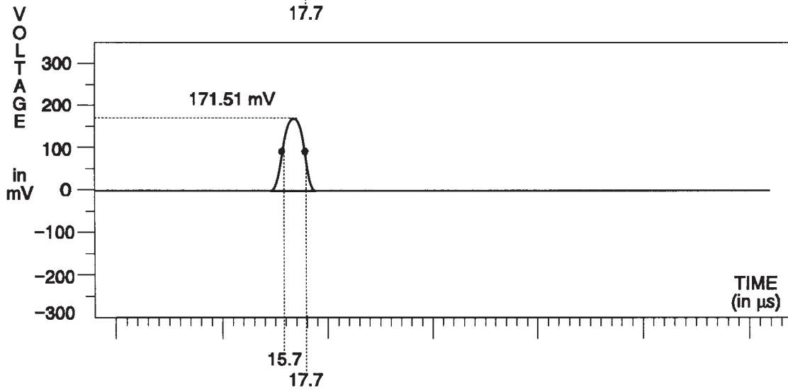
Fig. 3-227. B-Y Channel — Pulse & Bar.
