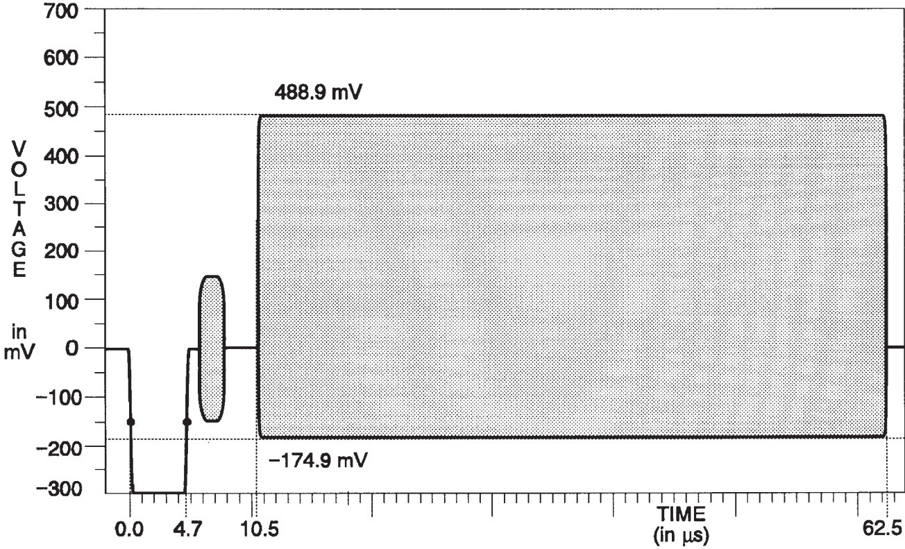
Fig. 3-3. 75% Red.
