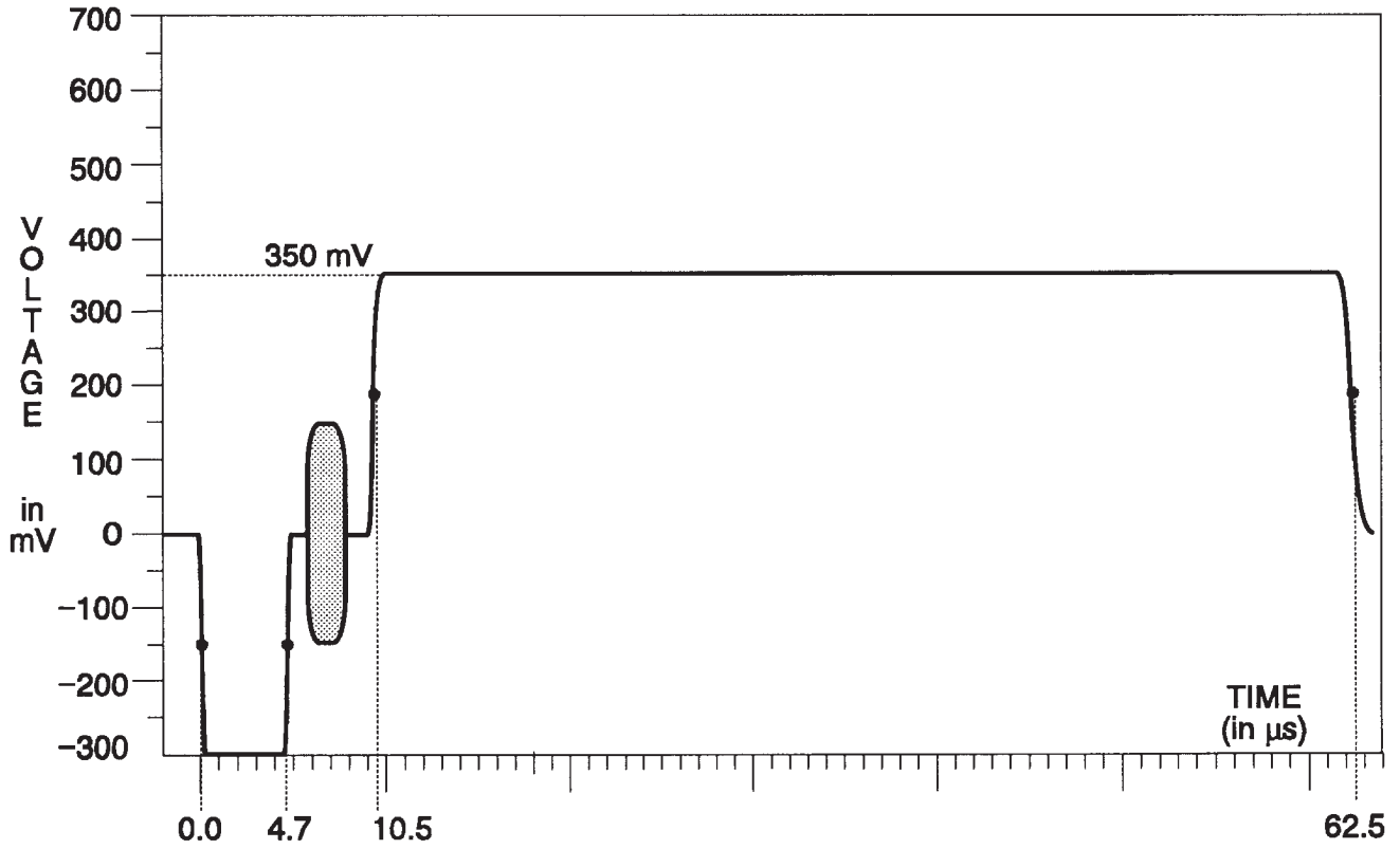
Fig. 3-147. Y Channel — 50% Flat Field.
