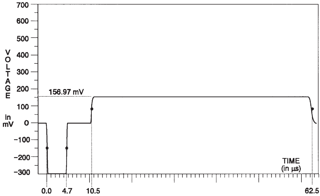
Fig. 3-77. Y Channel — 75% Red.
