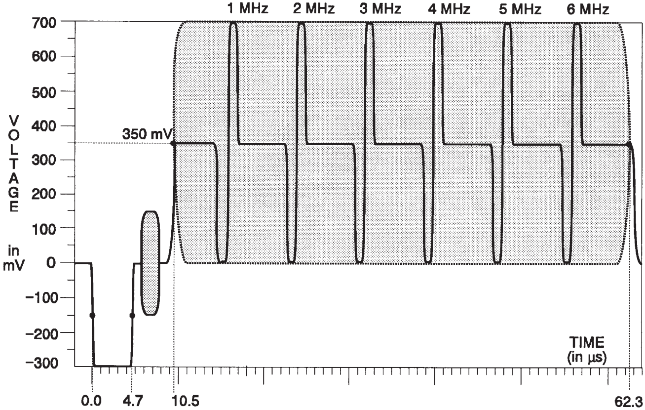
Fig. 3-20. Line Sweep.
