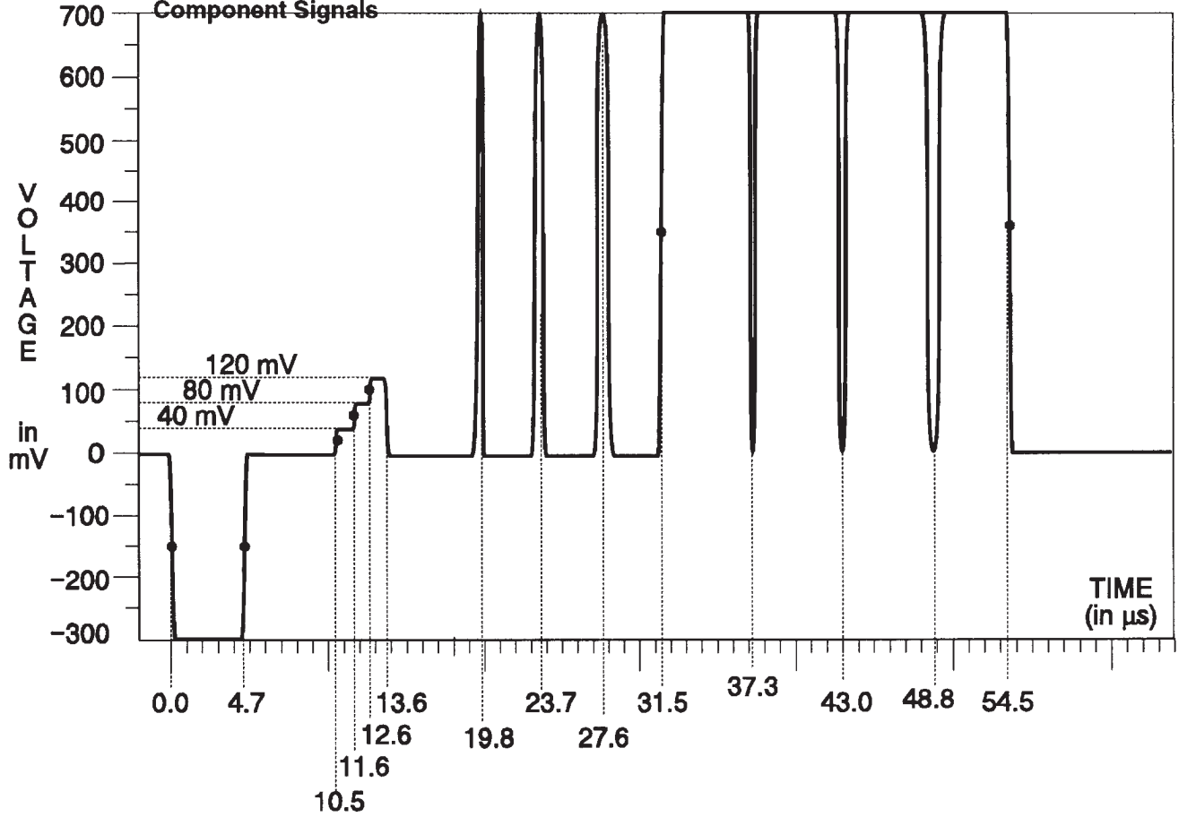
Fig. 3-92. Y Channel — T Pulses.
