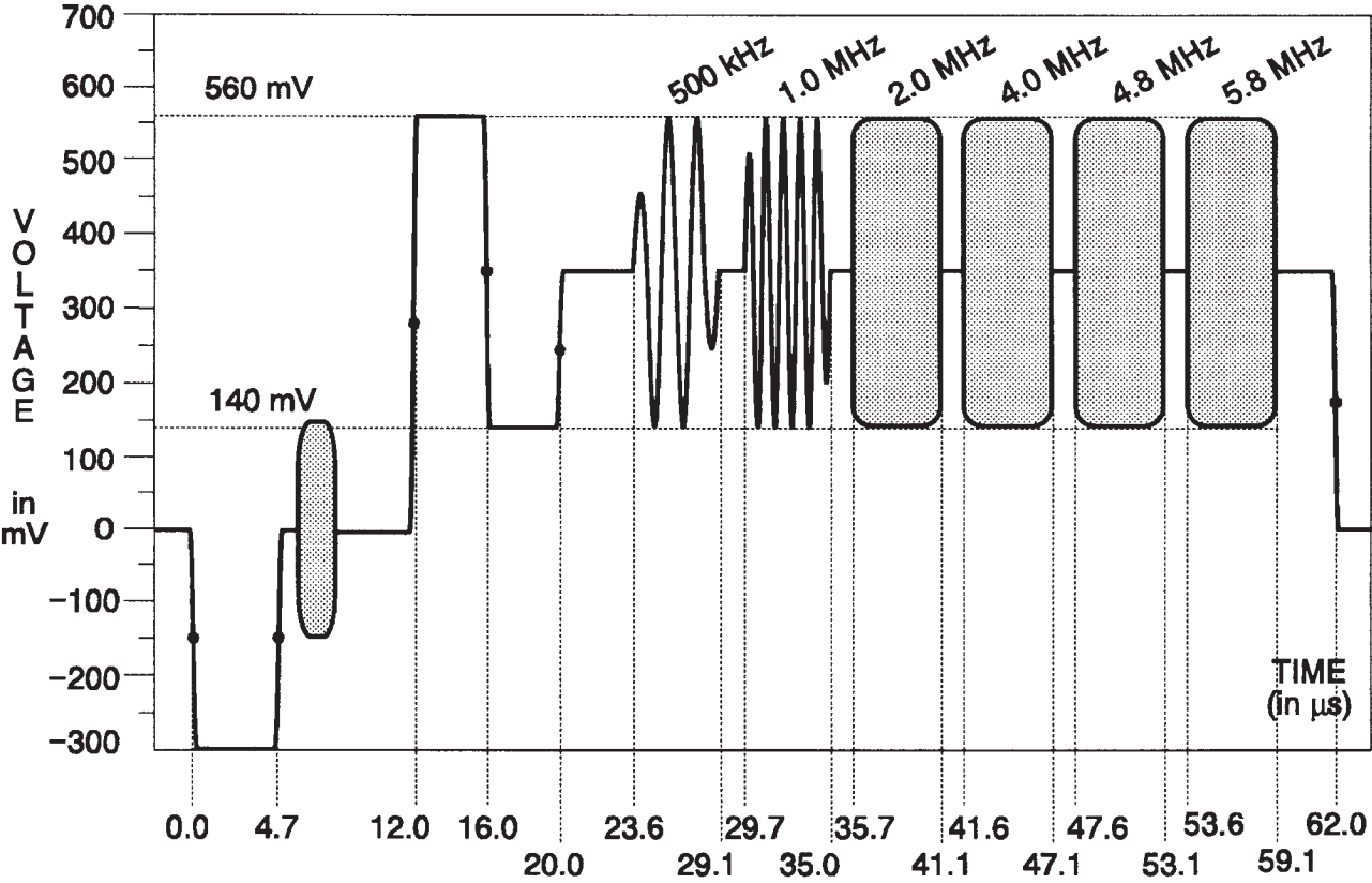
Fig. 3-25. Matrix Signal — CCIR Line 18.
