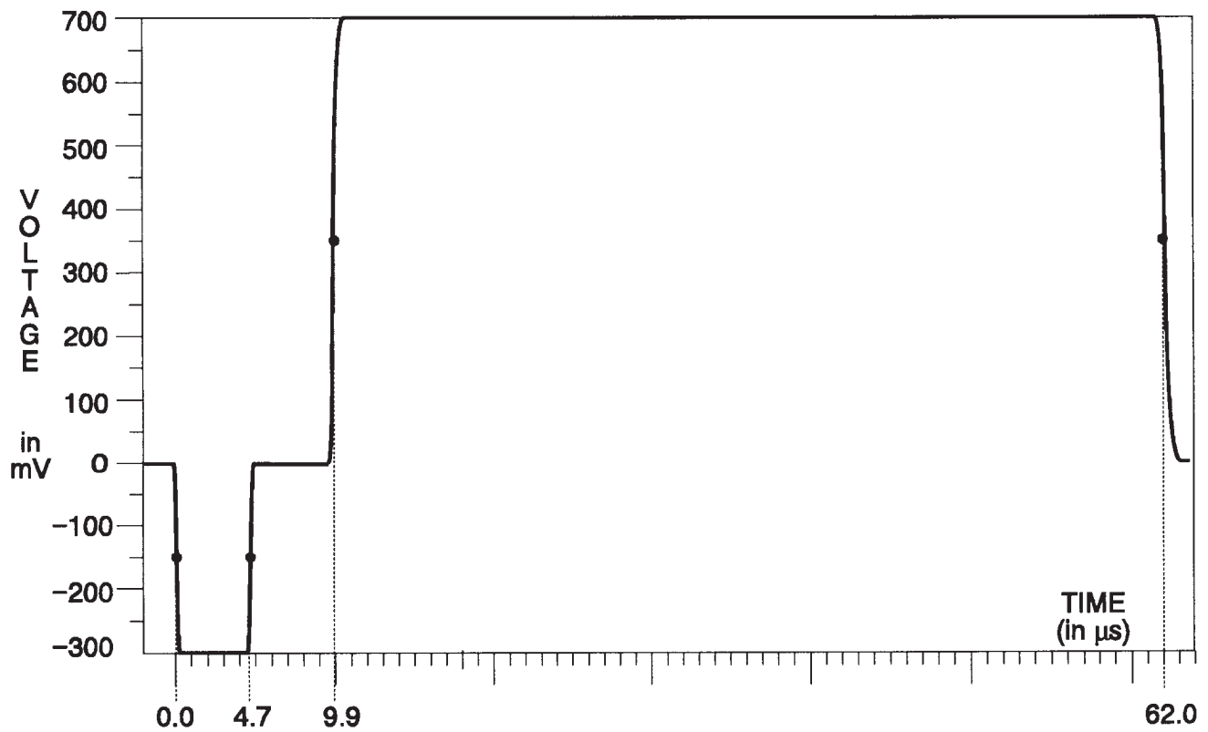
Fig. 3-162. Y Channel — 100% Flat Field.
