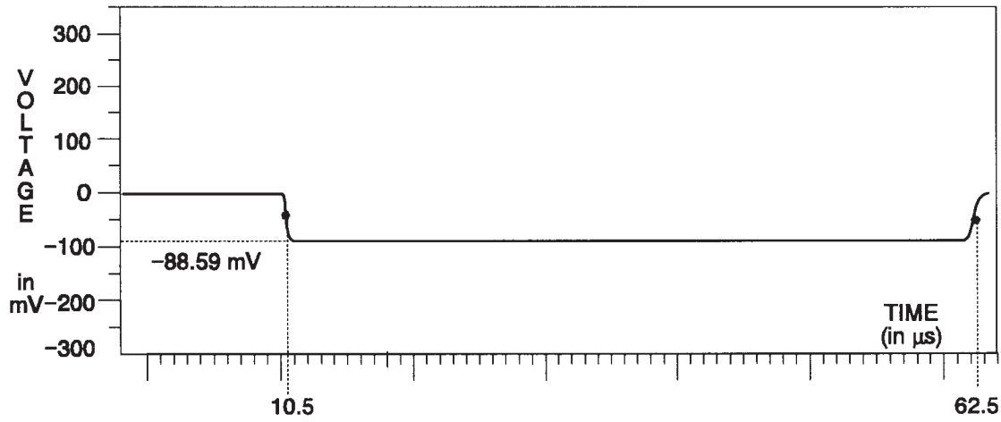
Fig. 3-78. B-Y Channel — 75% Red.
