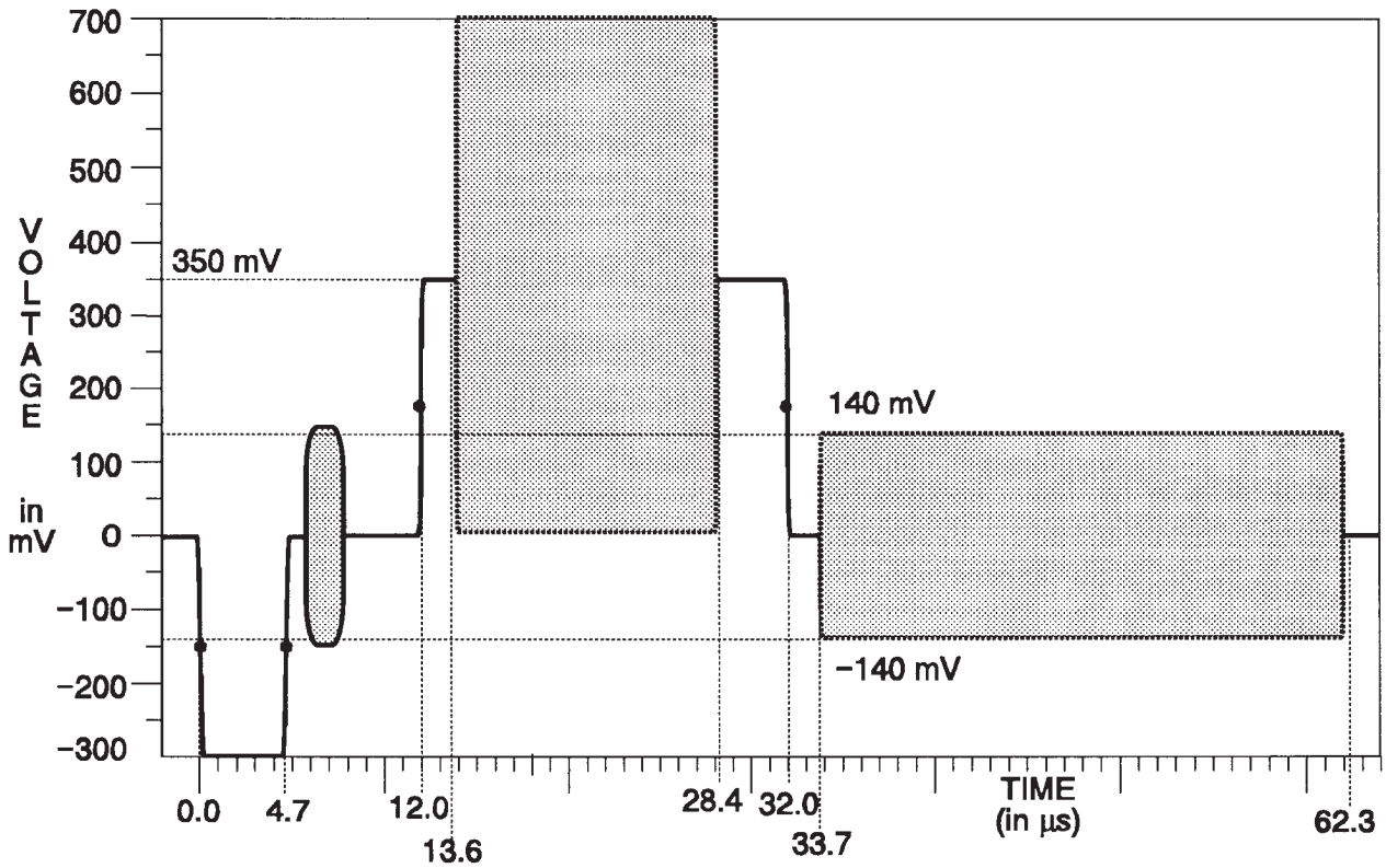
Fig. 3-23. Matrix Signal — UK ITS 2.
