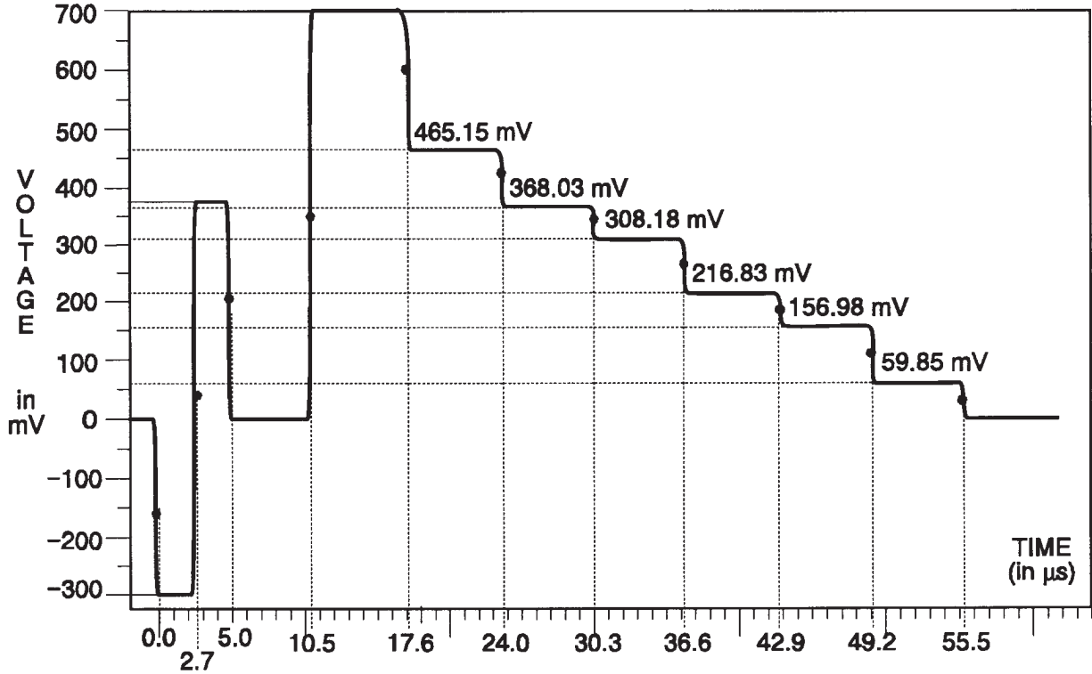
Fig. 3-103. Y Channel — 75% Bars.
