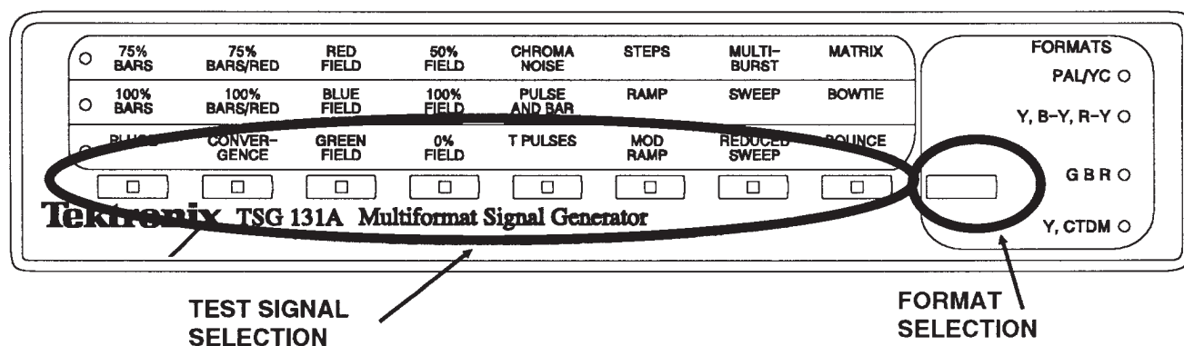
Fig. 2-1. Front panel of the TSG 131A.
