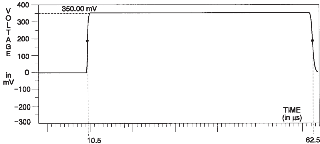
Fig. 3-82. R-Y Channel — 100% Red.
