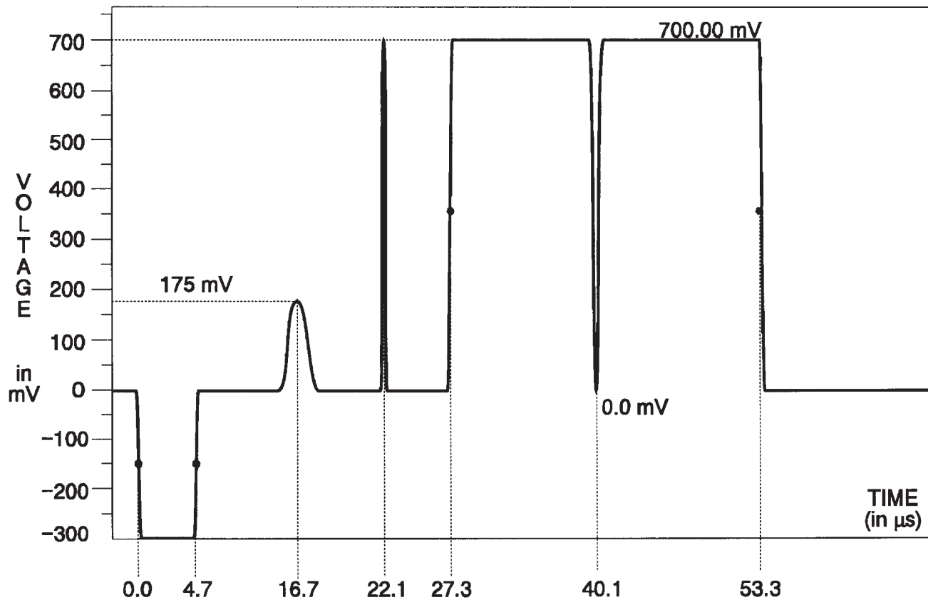
Fig. 3-131. Green Channel — Pulse & Bar.
