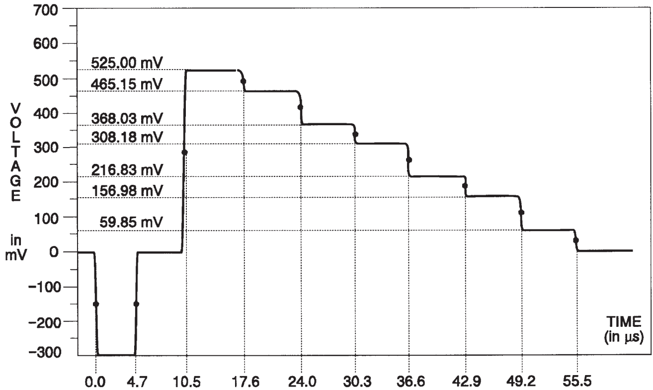
Fig. 3-213. Y Channel — 75% Color Bars.
