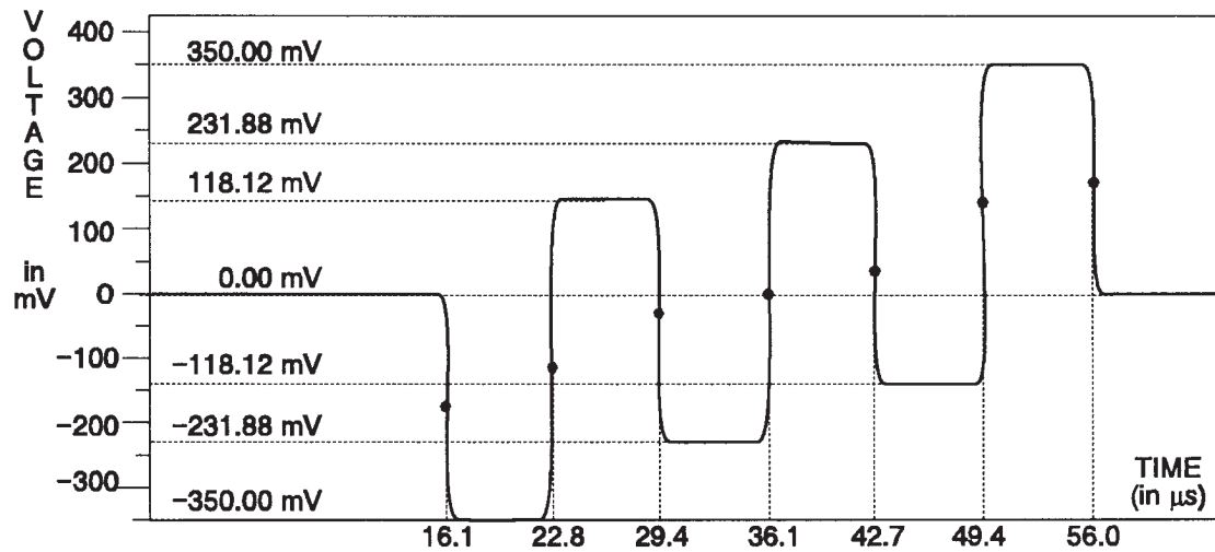
Fig. 3-179. B-Y Channel — 100% Color Bars.
