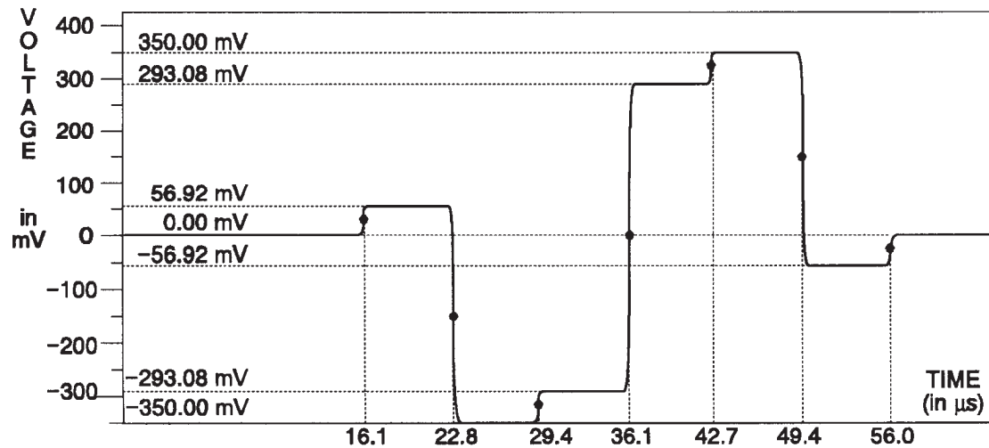
Fig. 3-180. R-Y Channel — 100% Color Bars.
