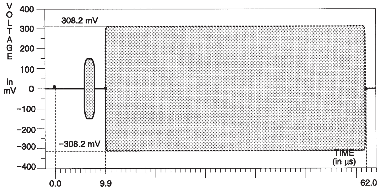
Fig. 3-160. C Channel — Green Field.
