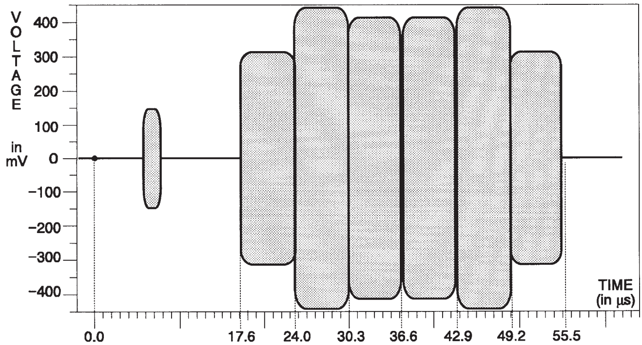
Fig. 3-37. C Channel — 100% Bars.
