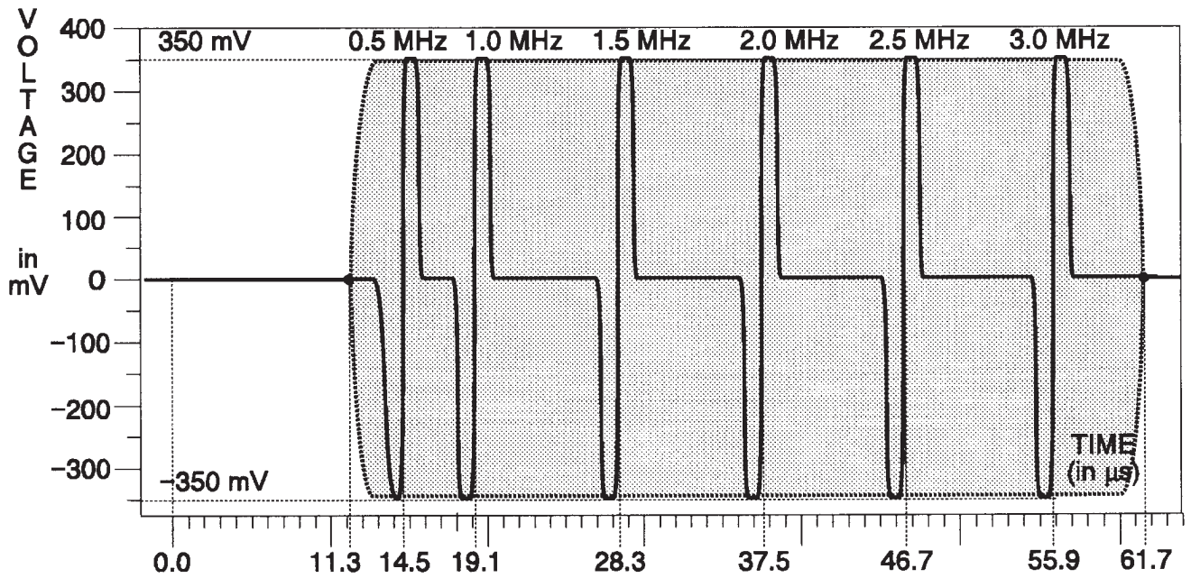
Fig. 3-236. B-Y & R-Y Channels — 100% Sweep.
