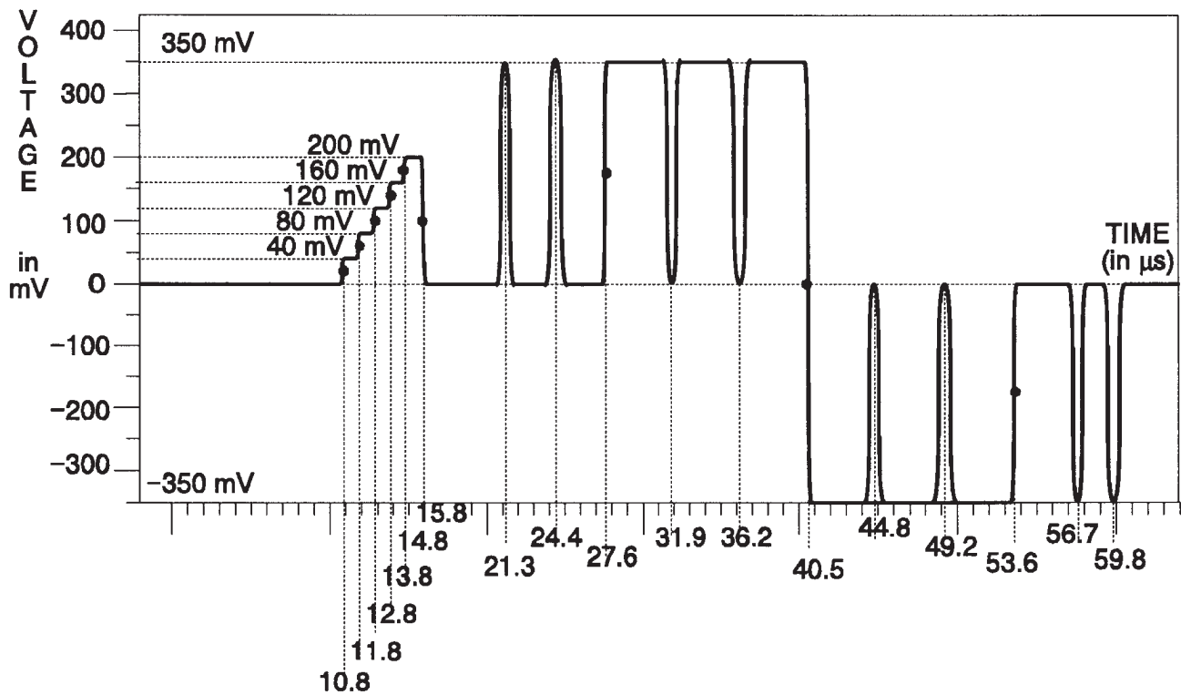
Fig. 3-230. B-Y & R-Y Channels — T Pulses.
