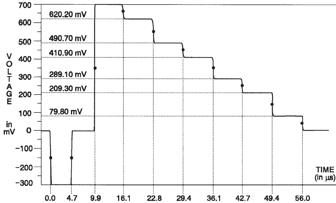
Fig. 3-178. Y Channel — 100% Color Bars.
