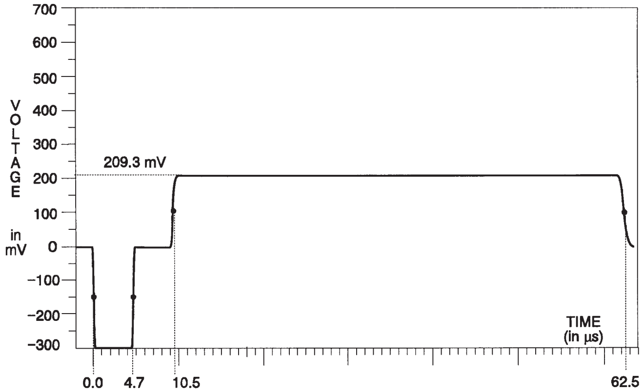
Fig. 3-38. Y Channel — 100% Red.
