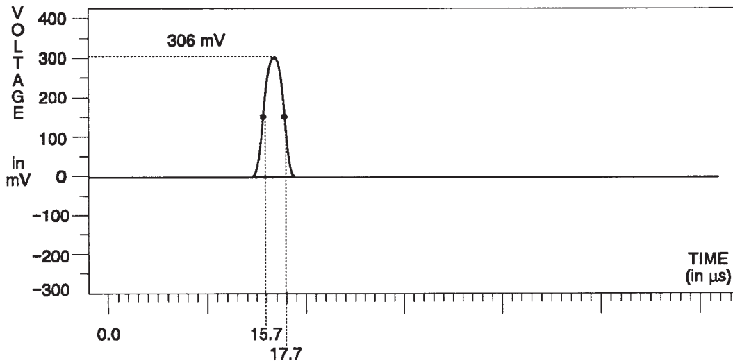
Fig. 3-91. R-Y Channel — Pulse & Bar with Window.
