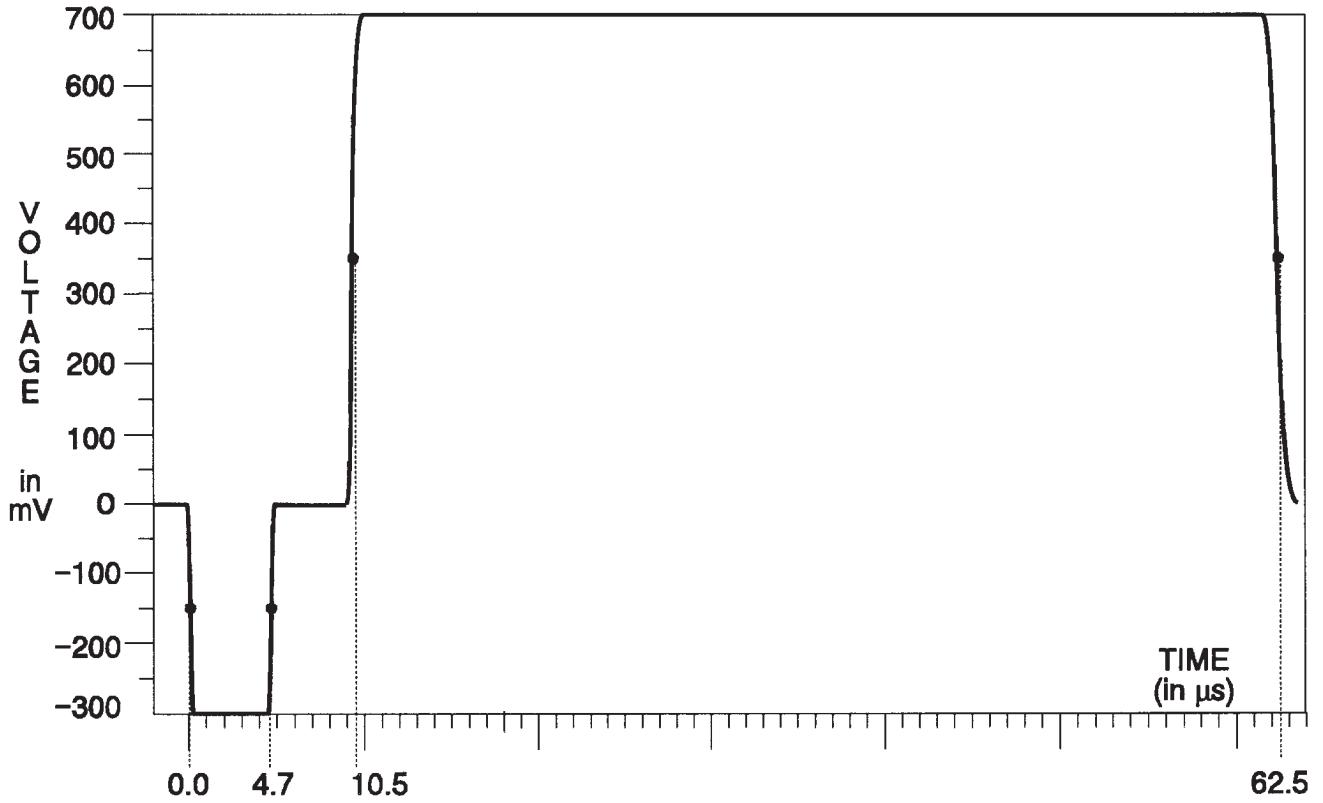
Fig. 3-50. Y Channel — 100% Flat Field.
