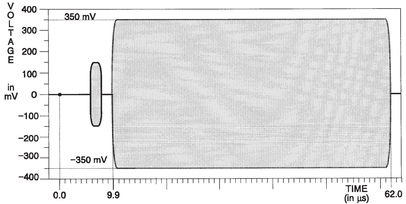
Fig. 3-164. C Channel — Chroma Noise.
