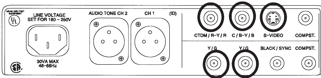
Fig. 2-9. Outputs available in the GBR format.
