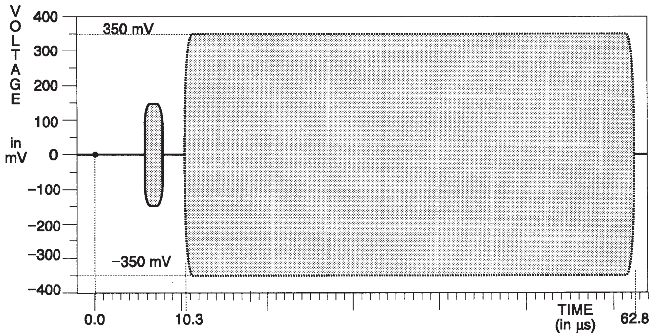
Fig. 3-53. C Channel — Chroma Noise.
