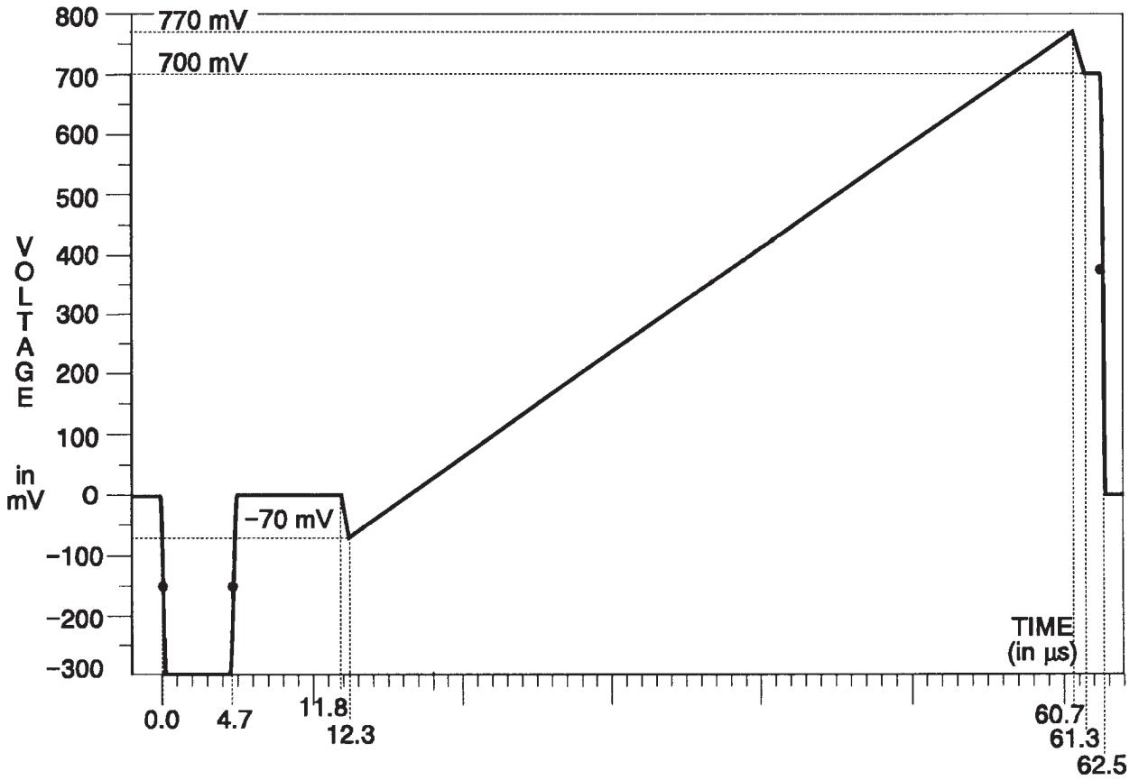
Fig. 3-237. Y Channel — Oversized ramp.
