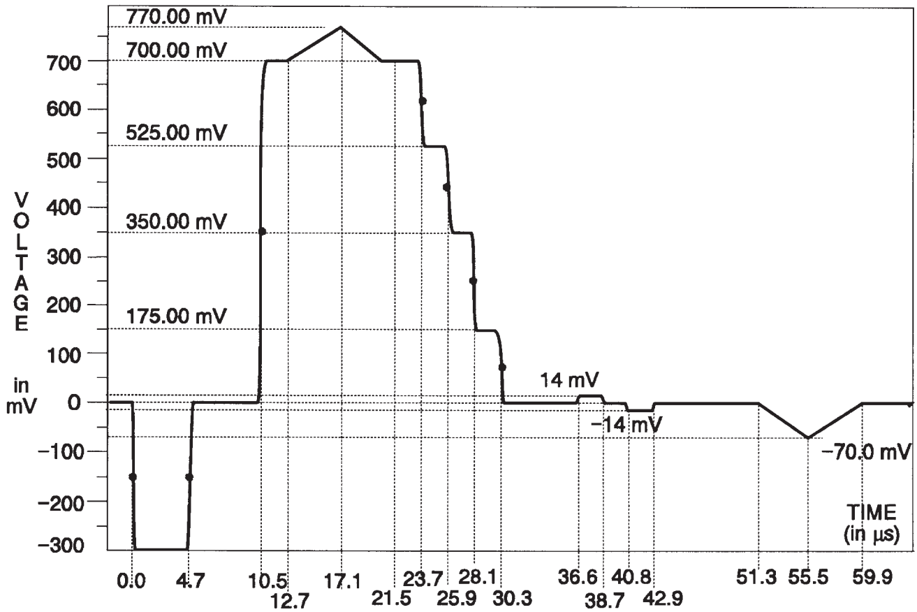
Fig. 3-224. Y Channel — Level Reference.
