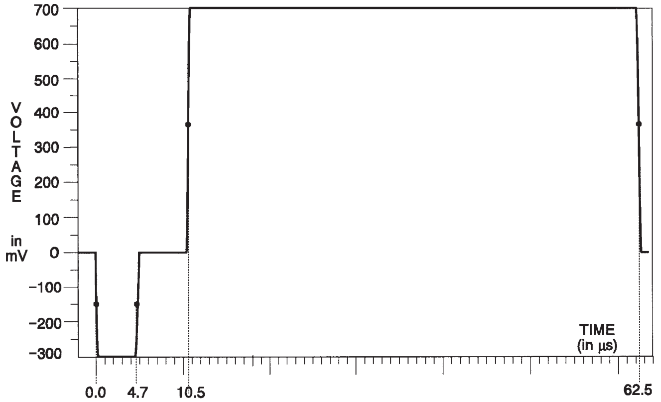
Fig. 3-123. Green Channel — Green Field.
