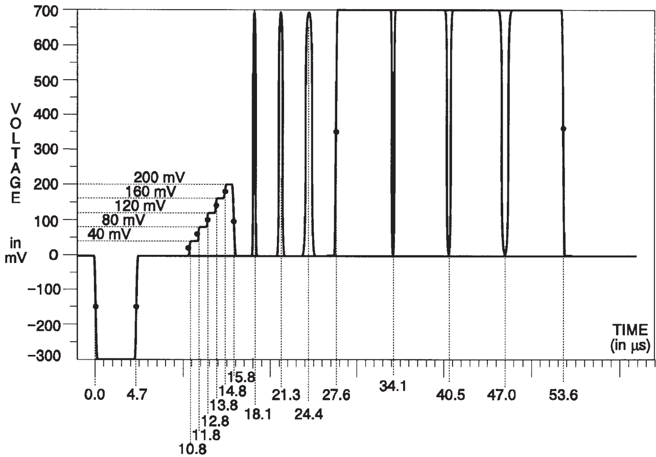
Fig. 3-229. Y Channel — T Pulses.
