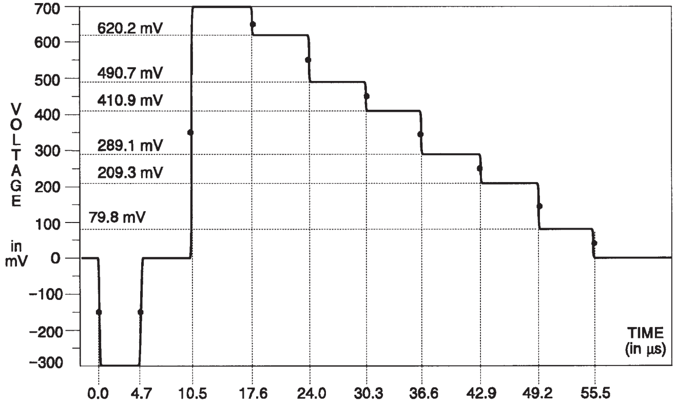
Fig. 3-36. Y Channel — 100% Bars.
