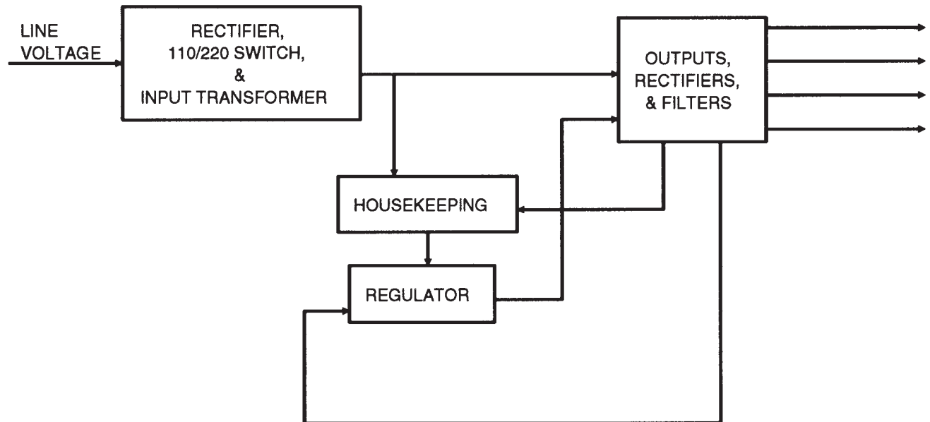
Fig. 8. Block diagram of the Power Supply circuitry.
