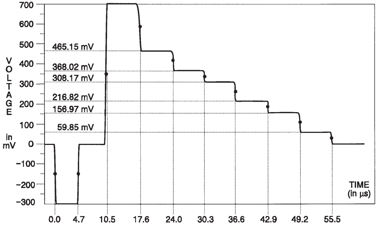
Fig. 3-32. Y Channel — 75% Bars.
