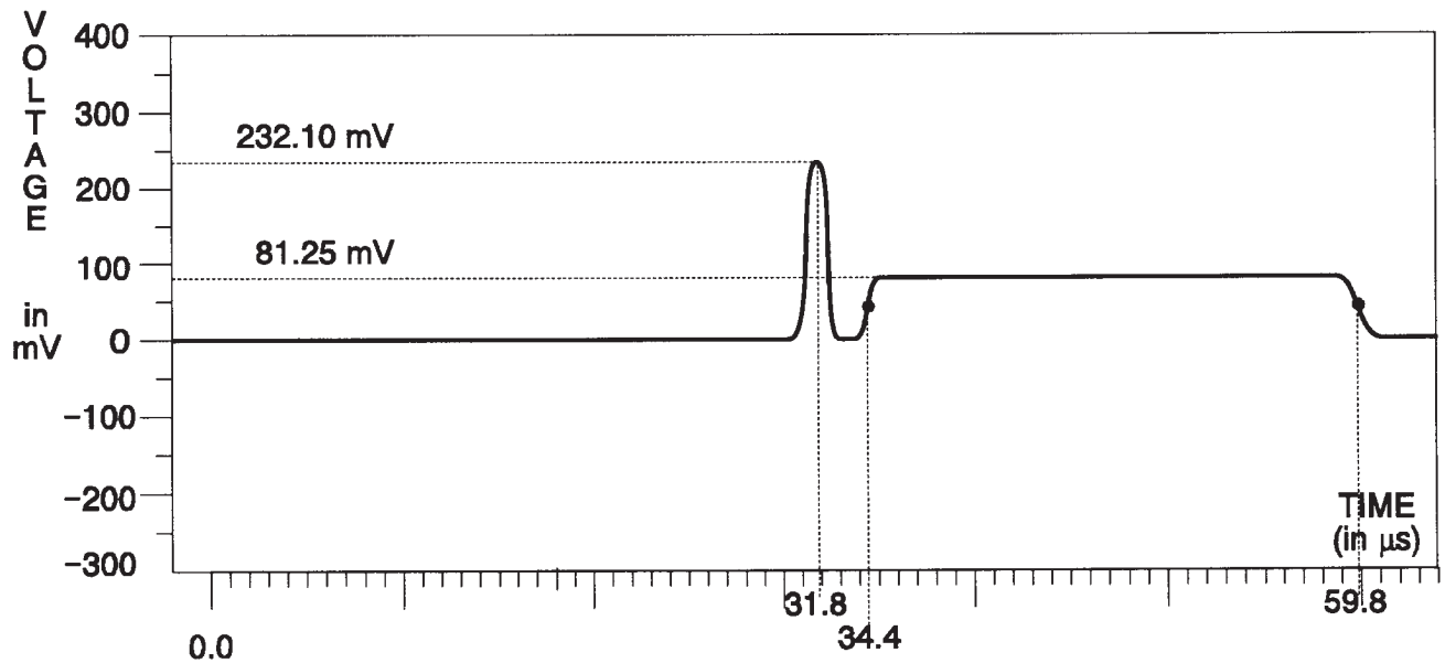
Fig. 3-198. B-Y & R-Y Channels — Line 17.
