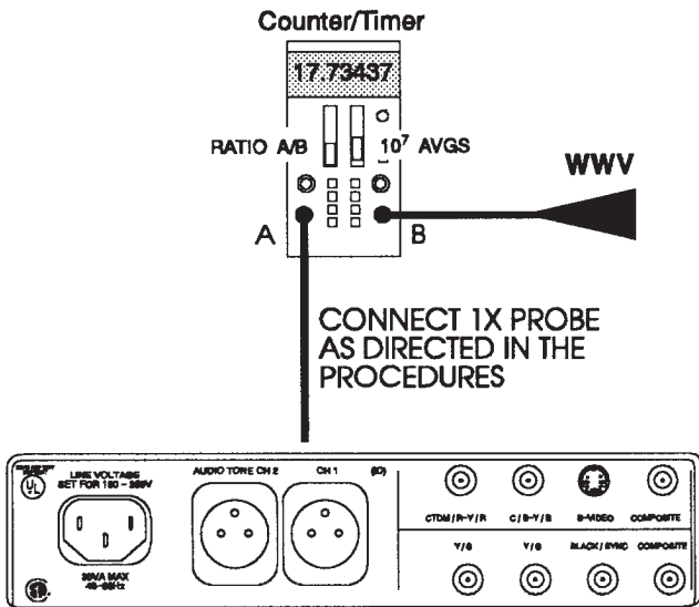
Fig. 4-8. Setup to adjust the oscillator frequency.
