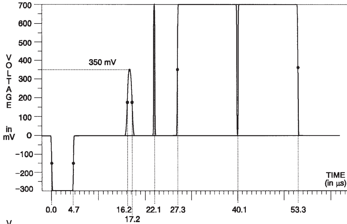
Fig. 3-181. Y Channel — Pulse & Bar.
