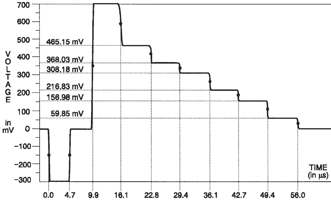
Fig. 3-175. Y Channel — 75% Color Bars.
