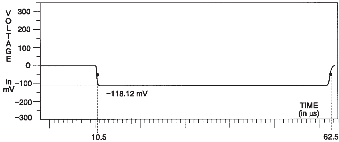
Fig. 3-81. B-Y Channel — 100% Red.
