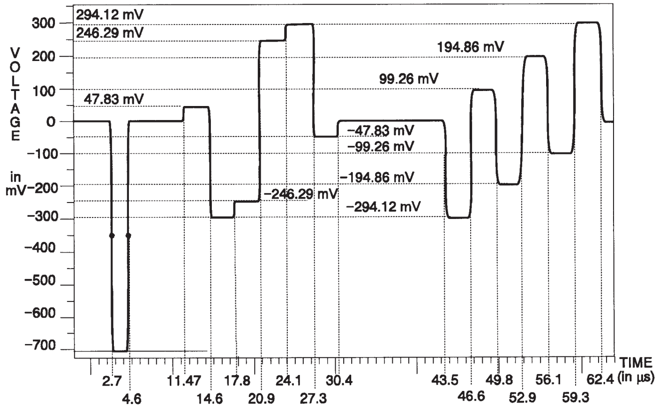
Fig. 3-104. C Channel — 75% Bars.
