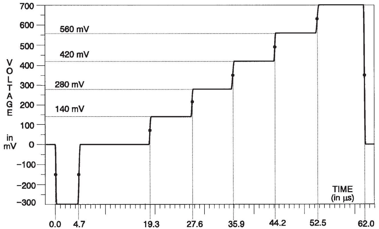
Fig. 3-165. Y Channel — 5-Step.
