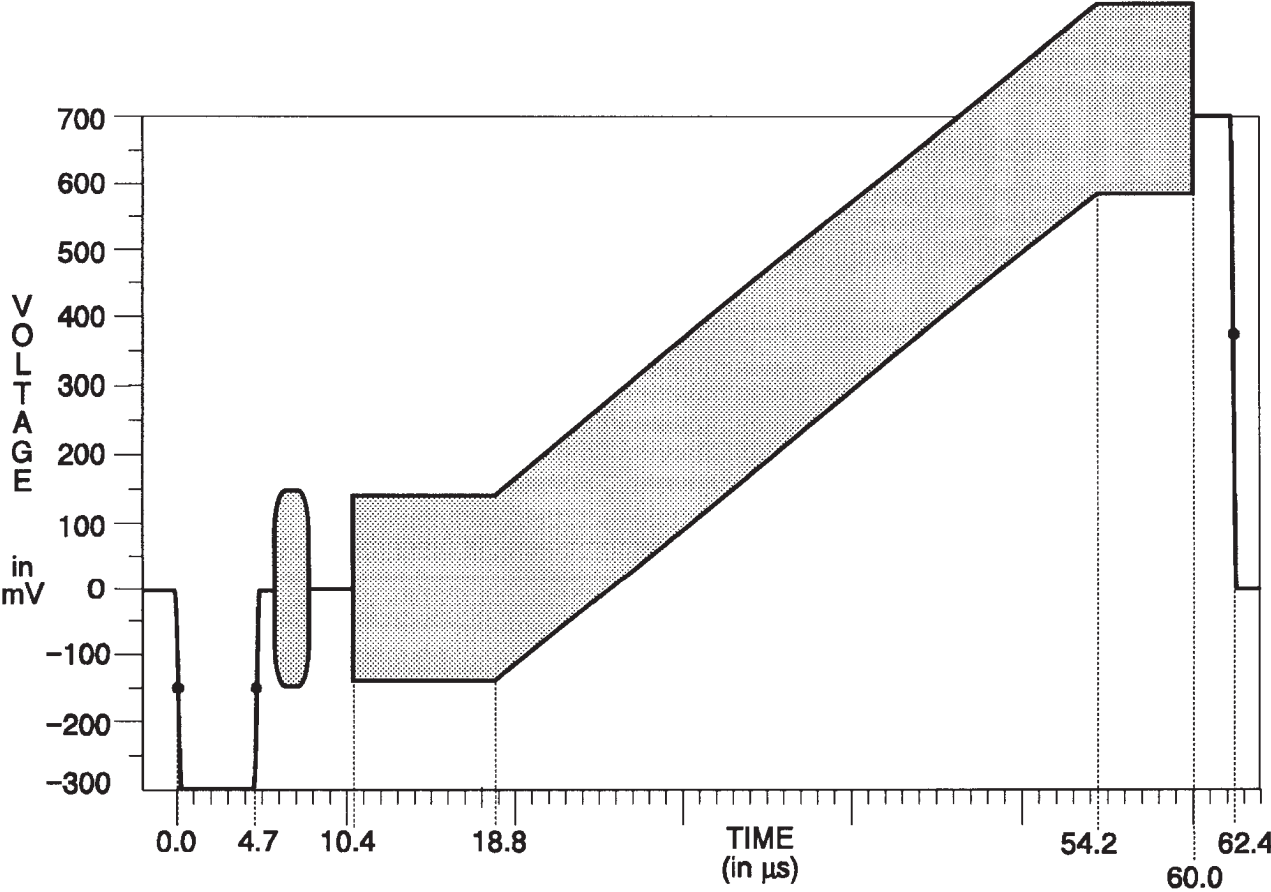
Fig. 3-17. Modulated Ramp.
