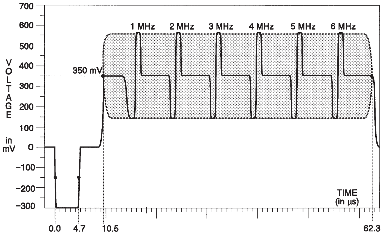
Fig. 3-66. Y Channel — Reduced Sweep.
