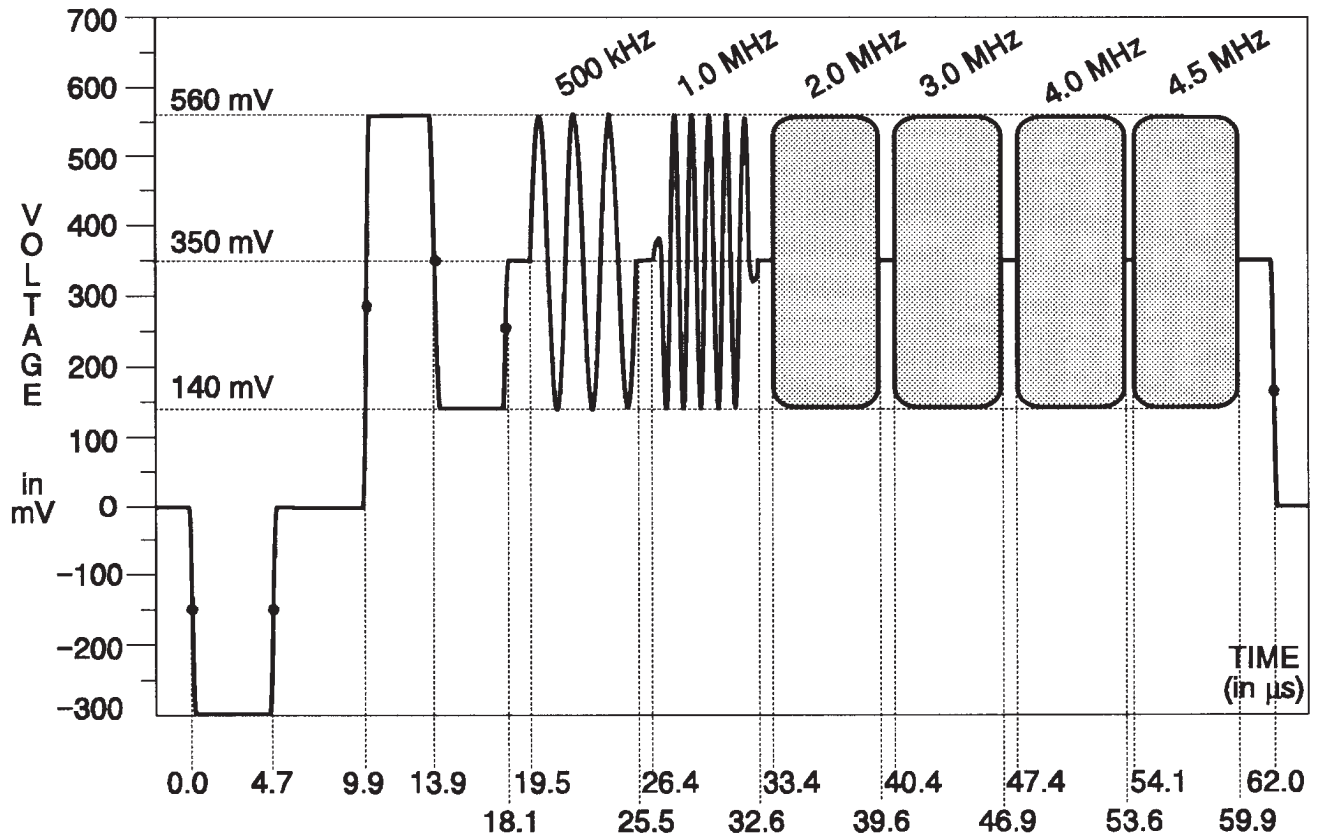
Fig. 3-199. Y Channel — 60% Narrow Multiburst.
