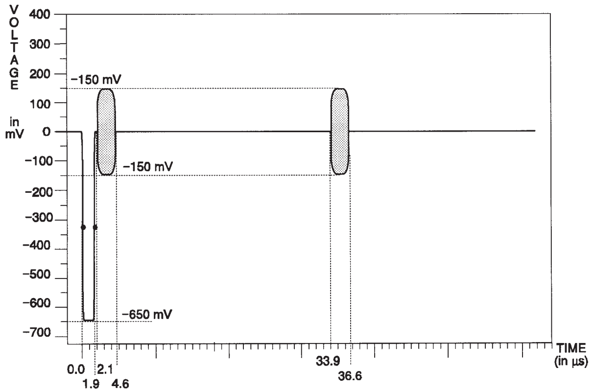
Fig. 3-146. C Channel — All Flat Field Signals.
