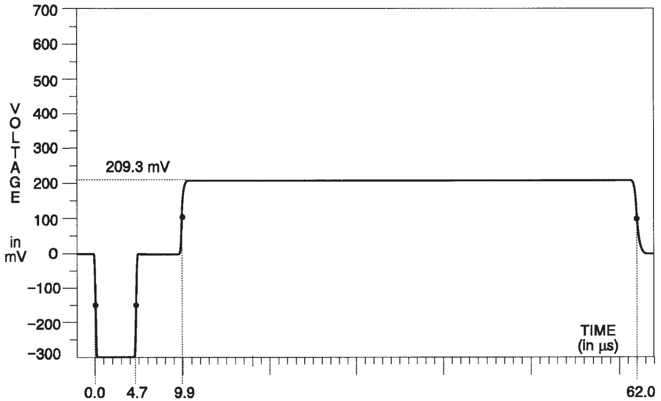
Fig. 3-155. Y Channel — 100% Red.
