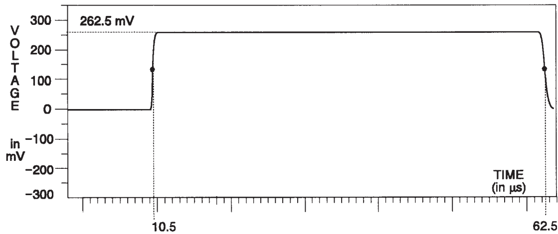
Fig. 3-79. R-Y Channel — 75% Red.
