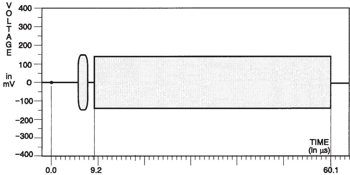
Fig. 3-168B C Channel — Modulated 5-Step.
