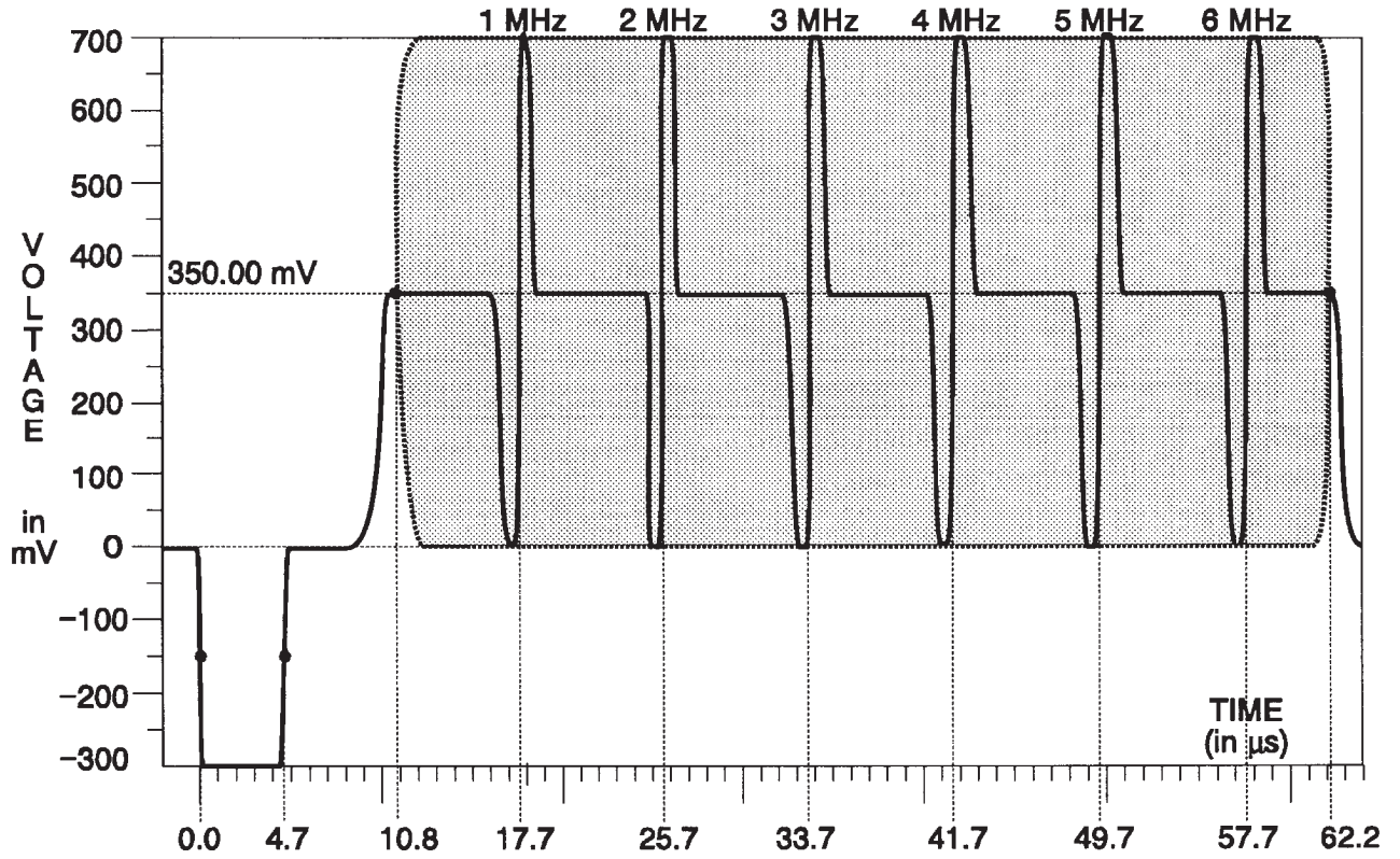
Fig. 3-135. Green Channel — Sweep.
