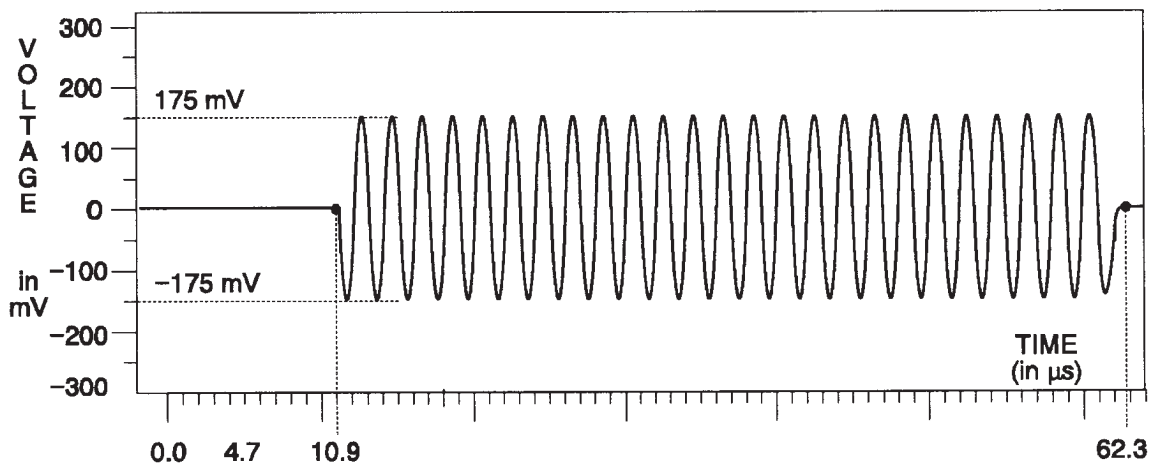
Fig. 3-100. B-Y & R-Y Channels — Bowtie.
