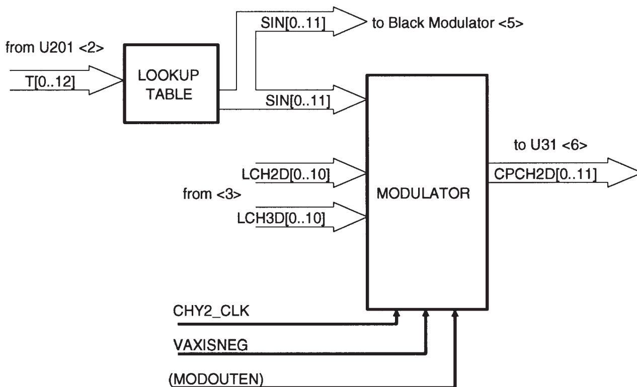
Fig. 4. Block diagram for <4>.
