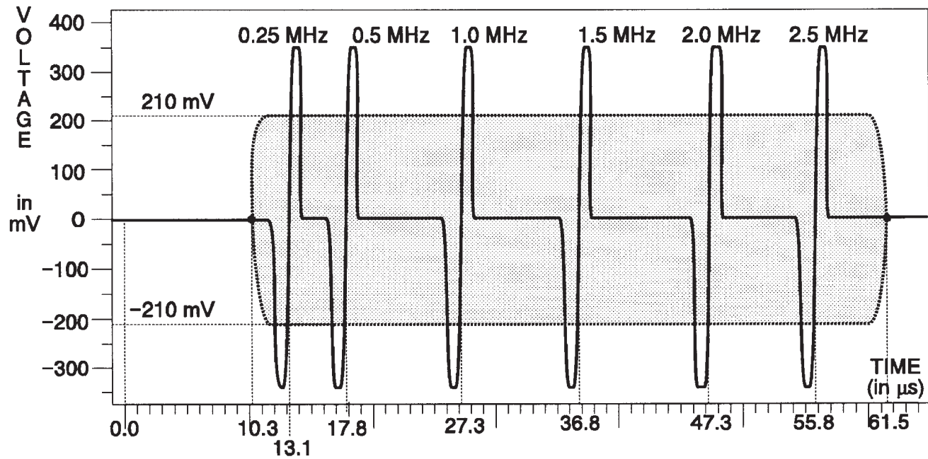
Fig. 3-204. B-Y & R-Y Channels — 60% Narrow Sweep.
