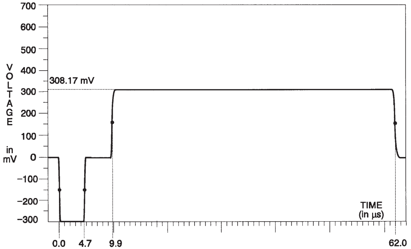
Fig. 3-159. Y Channel — Green Field.
