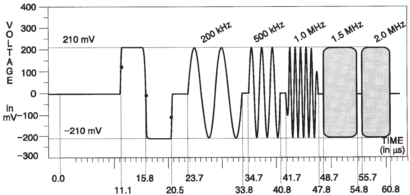
Fig. 3-202. B-Y & R-Y Channels — Wide Multiburst.
