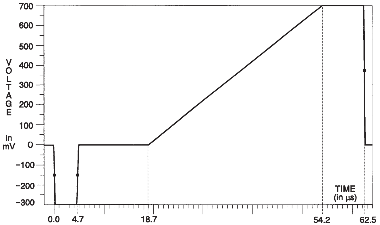
Fig. 3-219. Y Channel — Modulated Ramp.
