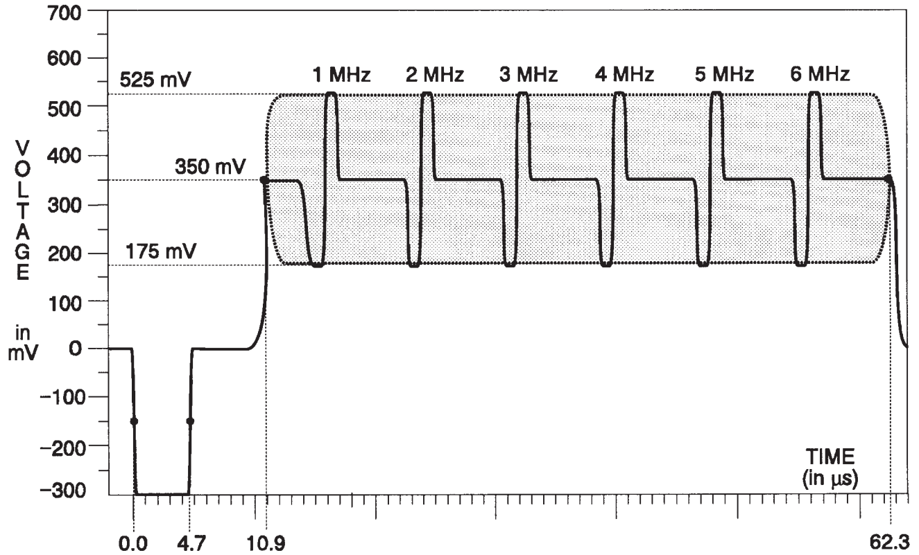
Fig. 3-96. Y Channel — Reduced Line Sweep.
