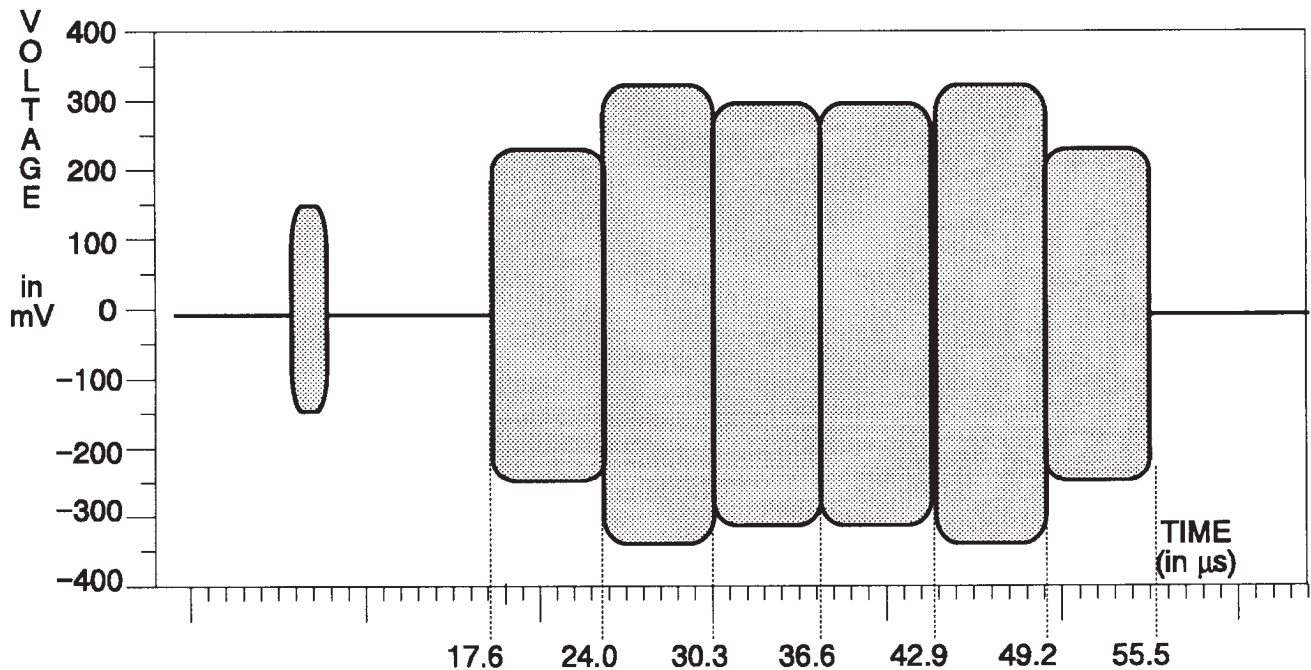
Fig. 3-214. C Channel — 75% Color Bars.
