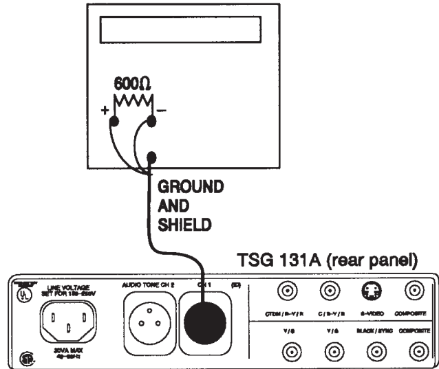
Fig. 4-9. Audio amplitude calibration setup.
