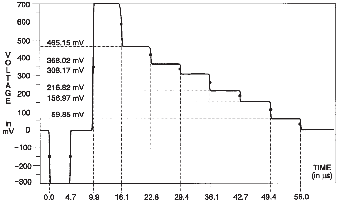
Fig. 3-149. Y Channel — 75% Bars.
