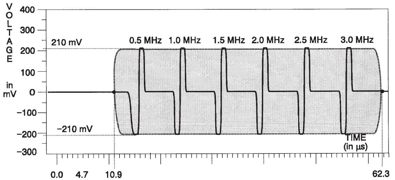
Fig. 3-95. B-Y & R-Y Channel — Line Sweep.
