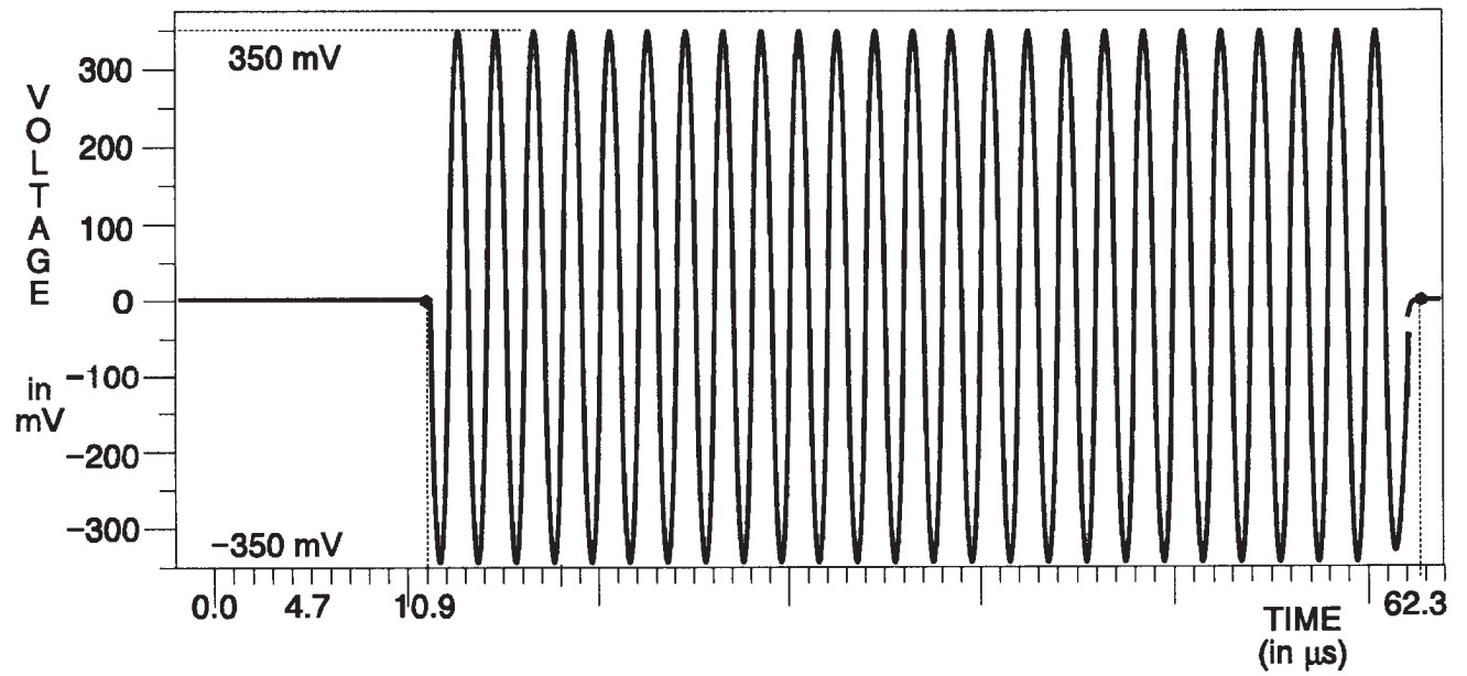
Fig. 3-240. B-Y & R-Y Channels — 100% Bowtie.
