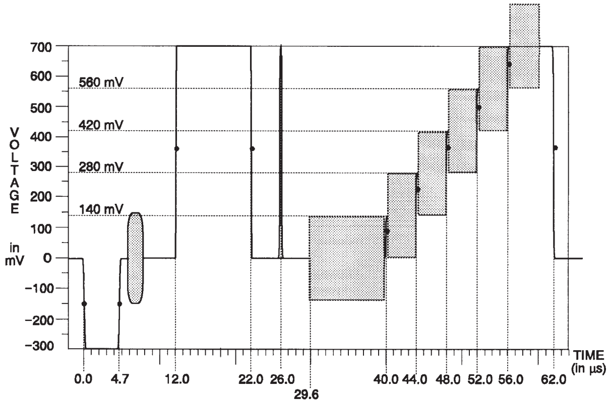
Fig. 3-26. Matrix Signal — CCIR Line 330.
