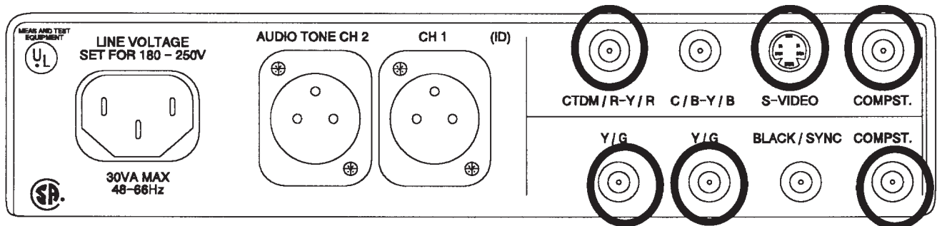
Fig. 2-11. Outputs available in the Y, CTDM format.
