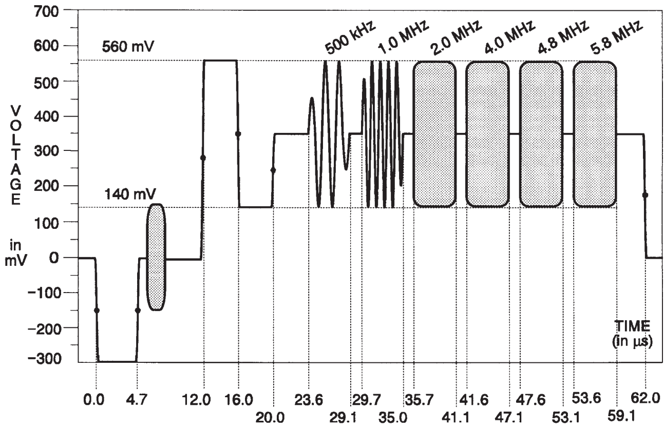
Fig. 3-19. Multiburst.
