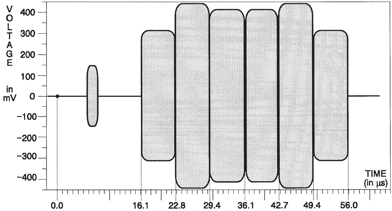
Fig. 3-154. C Channel — 100% Bars.
