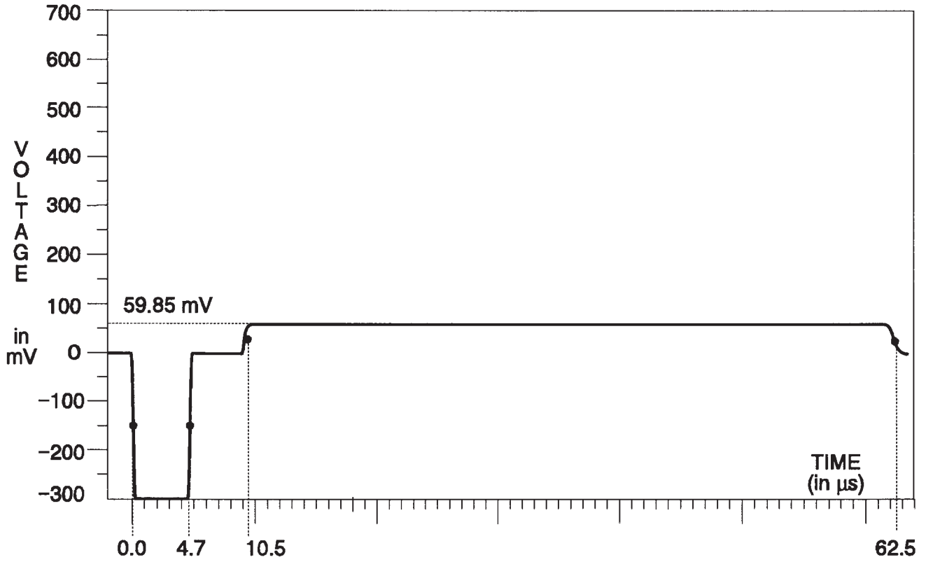
Fig. 3-42. Y Channel — Blue Field.
