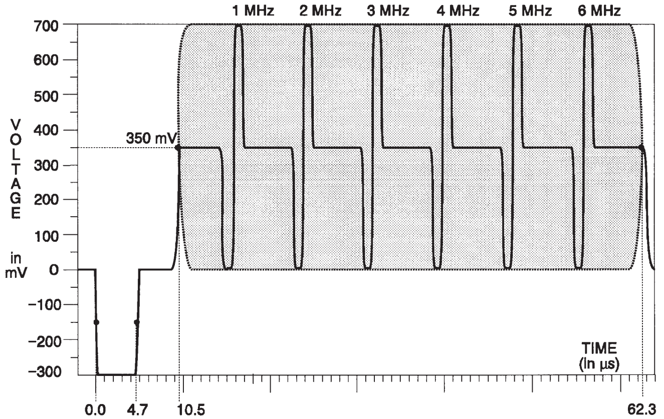
Fig. 3-64. Y Channel — Sweep.
