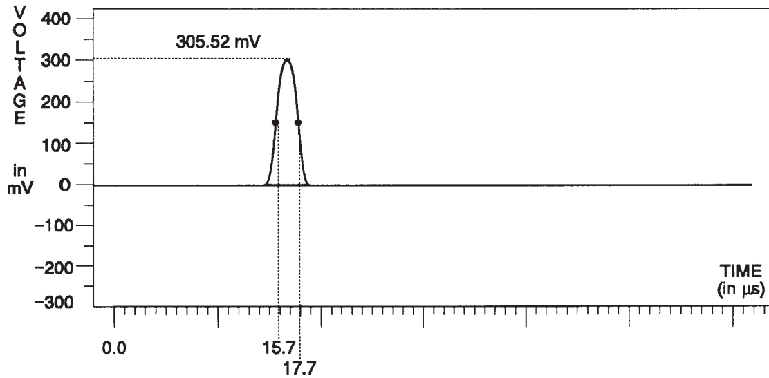
Fig. 3-228. R-Y Channel — Pulse & Bar.
