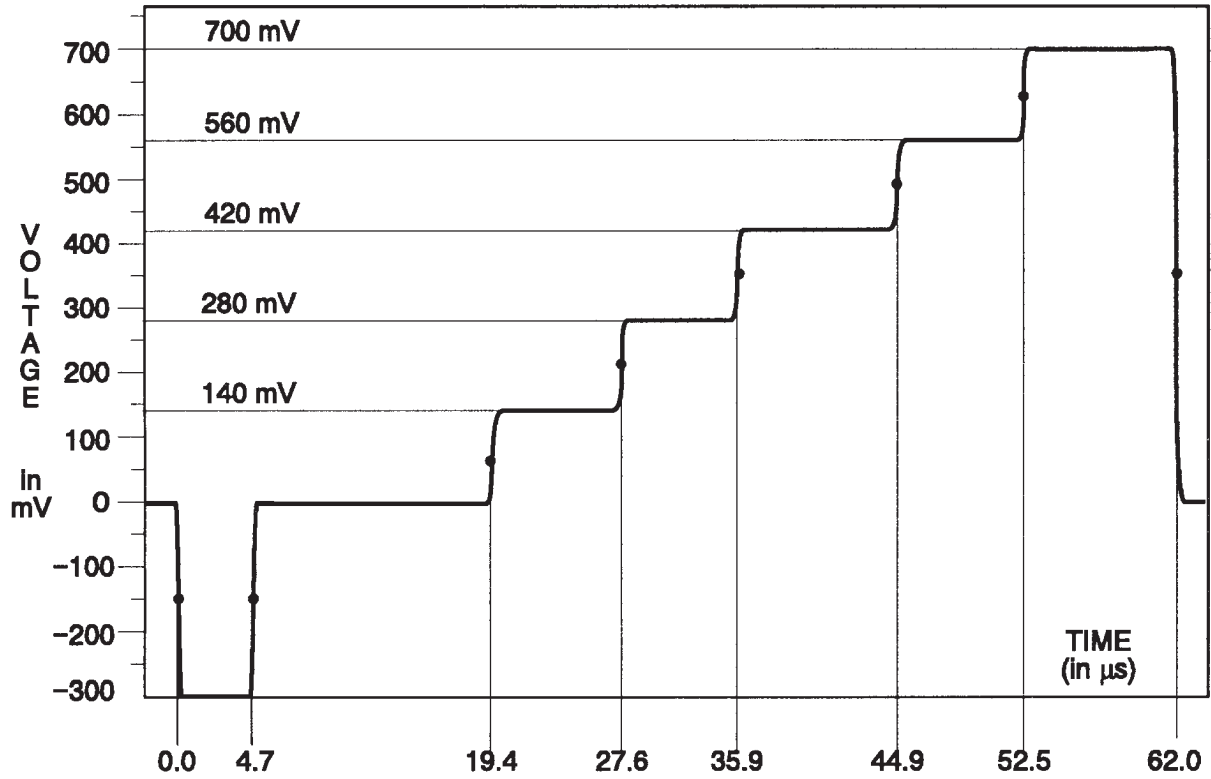
Fig. 3-168A Y Channel — Modulated 5-Step.
