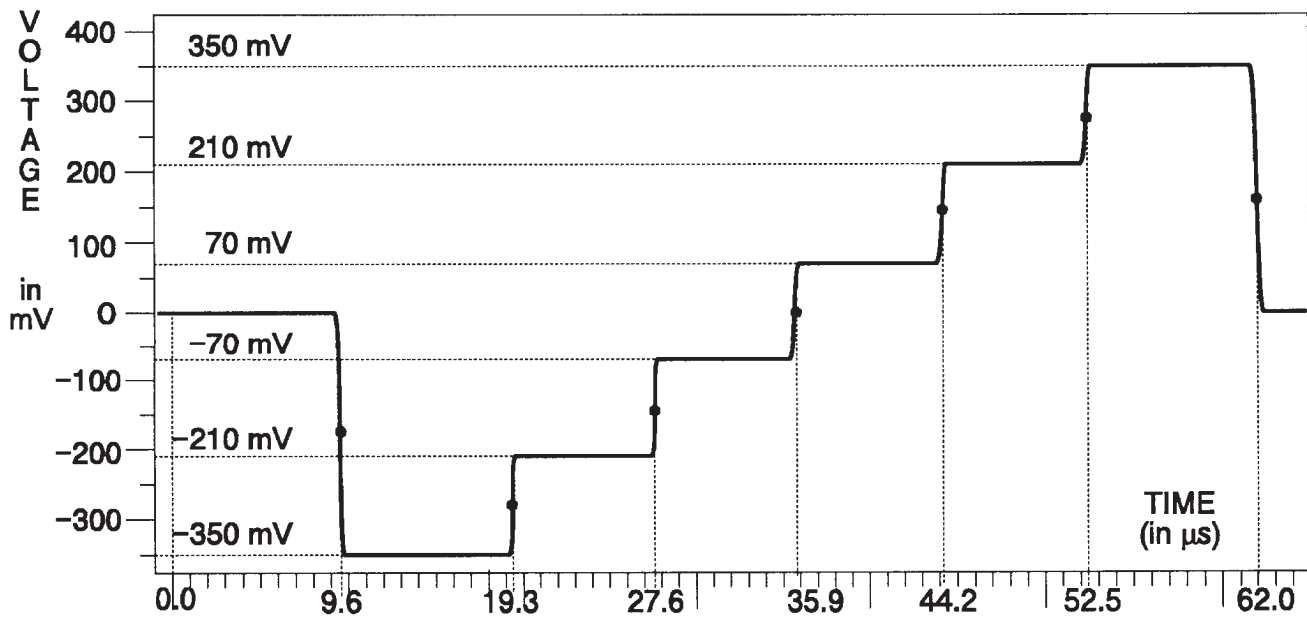
Fig. 3-191. B-Y & R-Y Channels — 5-Step.
