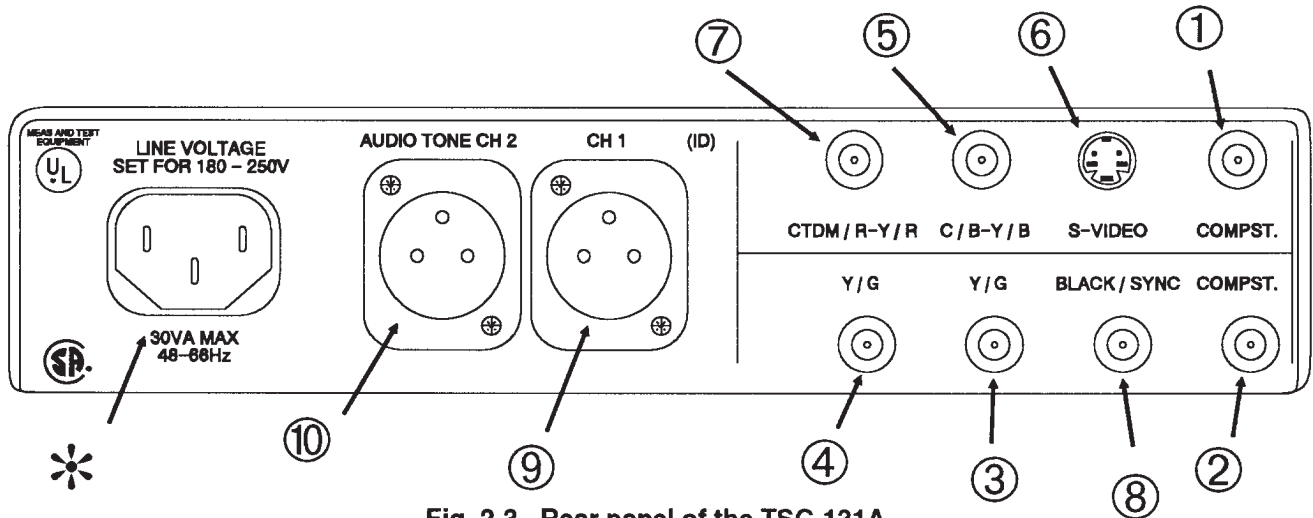
Fig. 2-3. Rear panel of the TSG 131A.
