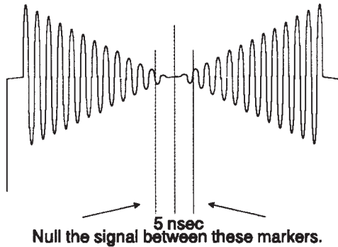
Fig. 4-4. Bowtie crossover.
