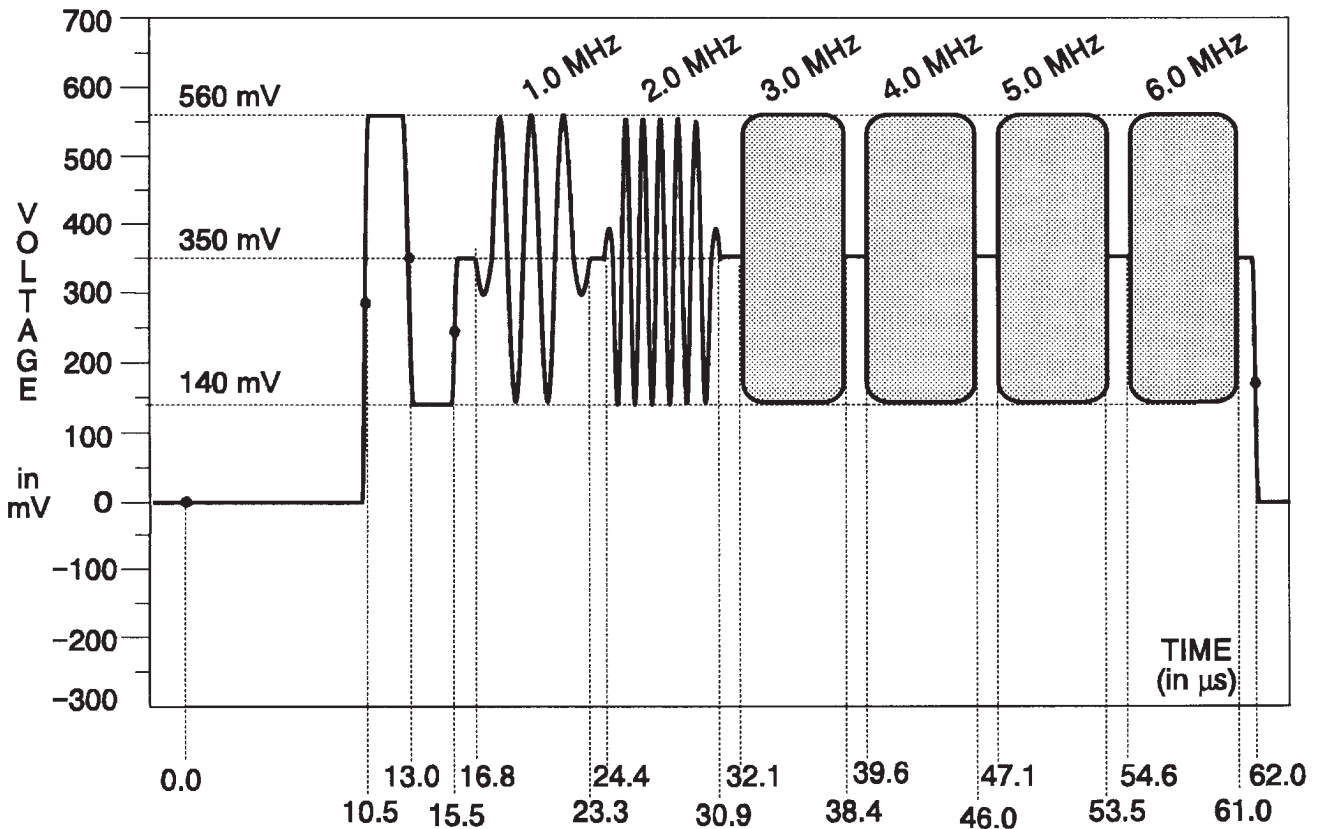
Fig. 3-134. Blue & Red Channels — Multiburst.
