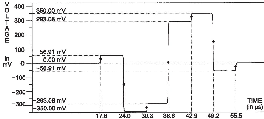
Fig. 3-76. R-Y Channel — 100% Bars.
