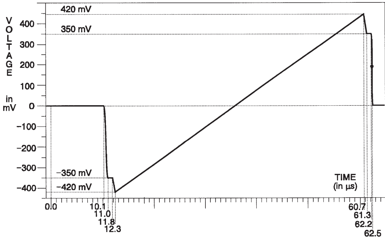
Fig. 3-238. B-Y & R-Y Channels — Oversized Ramp.
