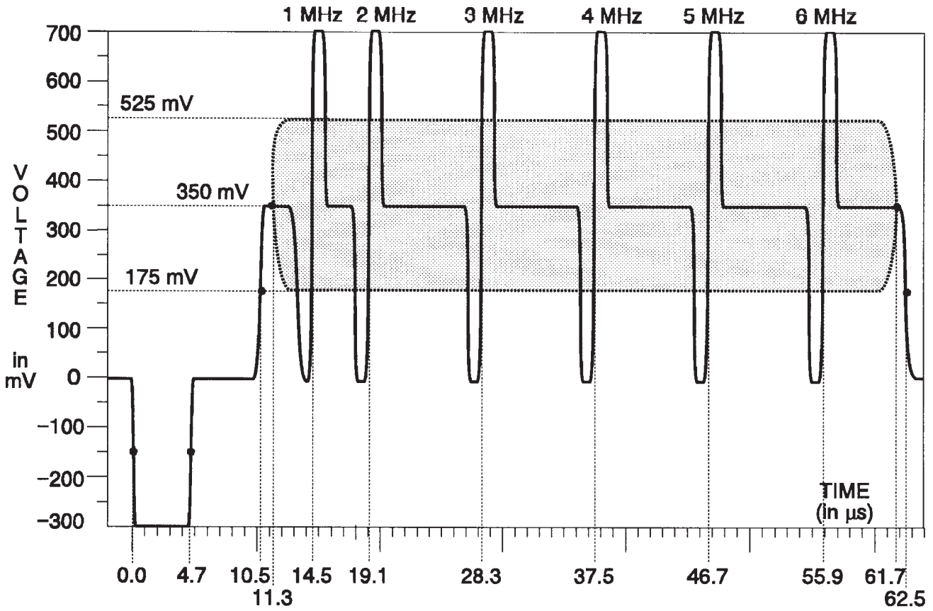
Fig. 3-233. Y Channel — 60% Sweep.
