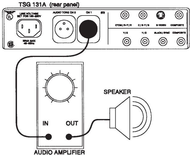
Fig. 4-10. Audio ID click frequency adjustment setup.
