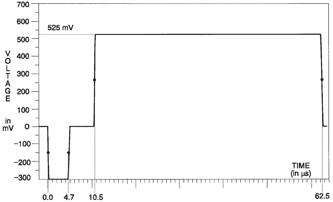
Fig. 3-125. Green Channel — Convergence (hor).
