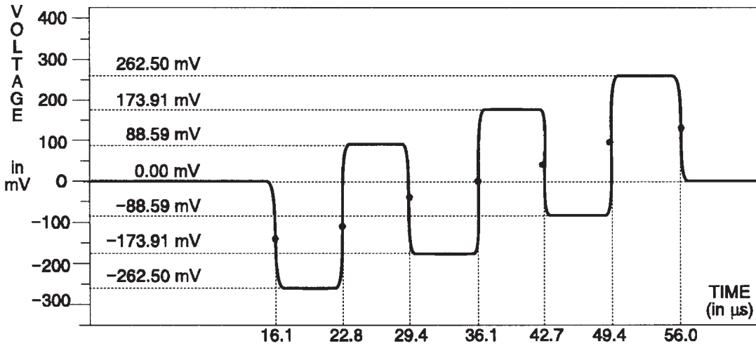
Fig. 3-176. B-Y Channel — 75% Color Bars.
