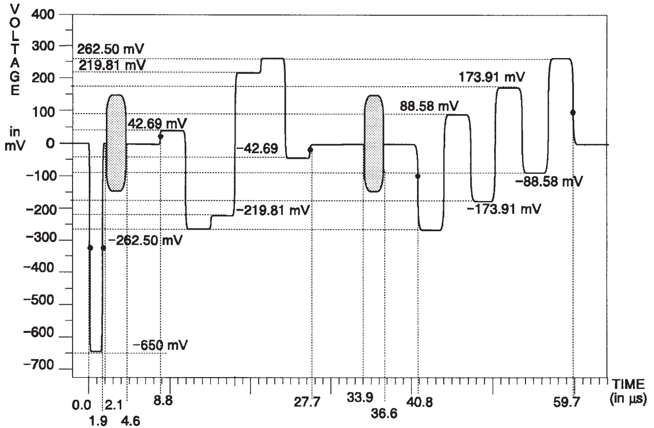
Fig. 3-142. C Channel — 75% Color Bars.
