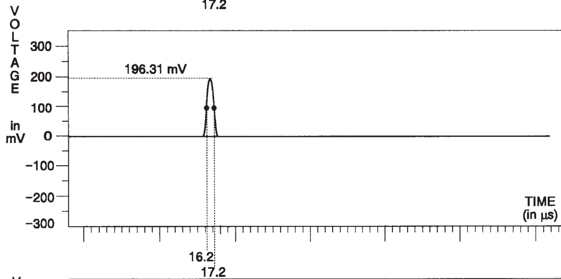
Fig. 3-182. B-Y Channel — Pulse & Bar.
