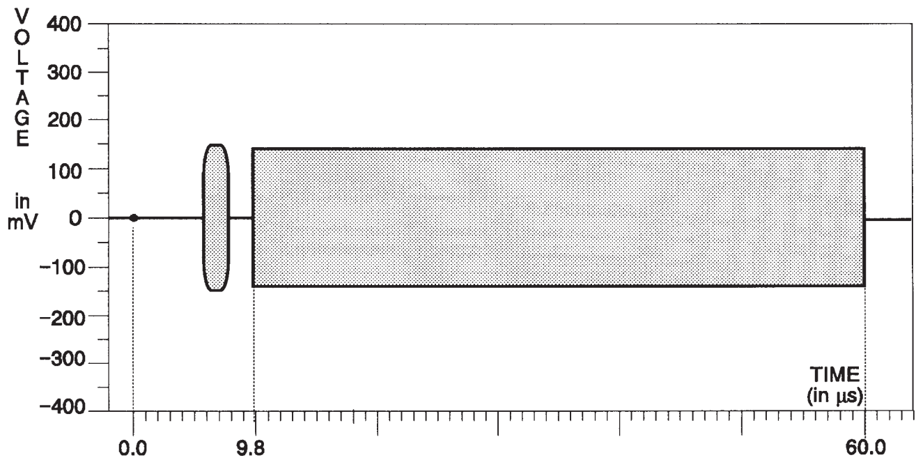
Fig. 3-220. C Channel — Modulated Ramp.
