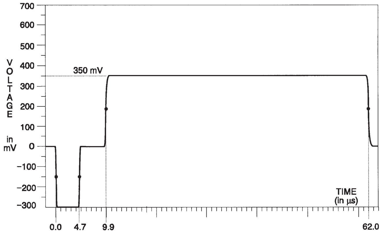
Fig. 3-184. Y Channel — 50% Flat Field.
