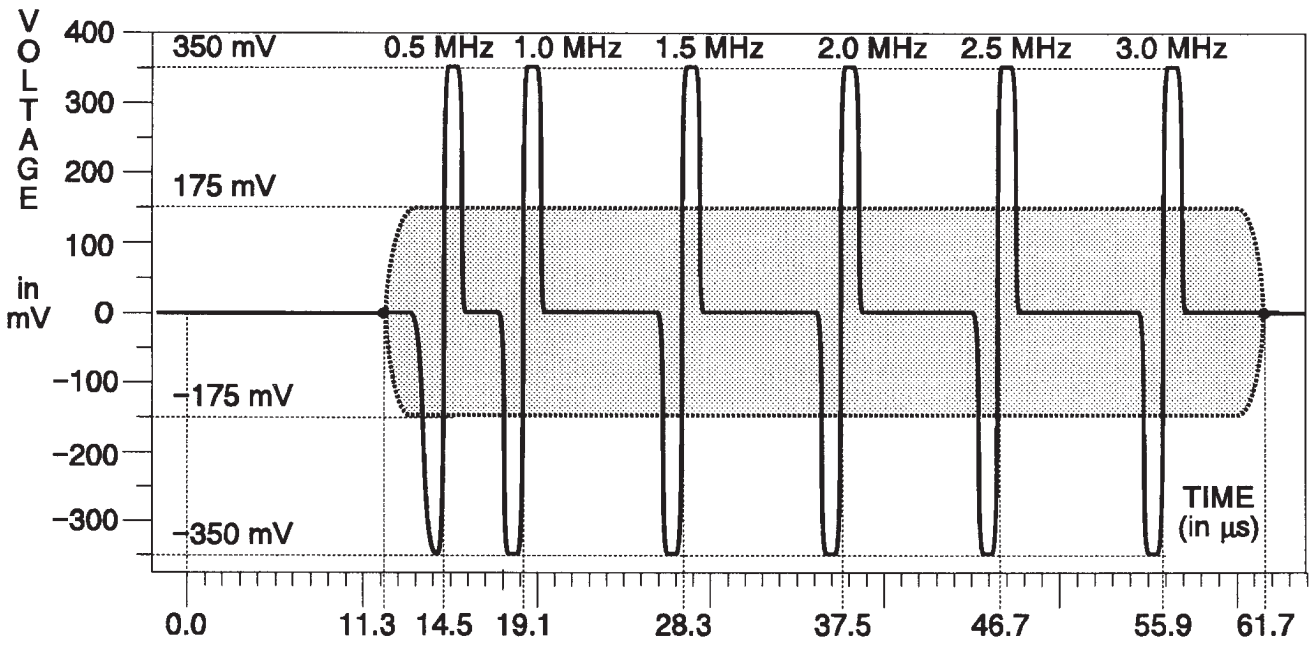
Fig. 3-234. B-Y & R-Y Channels — 60% Sweep.
