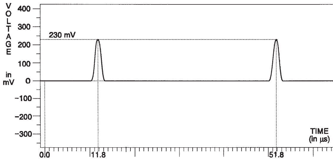
Fig. 3-209. B-Y Channel — 12T Pulses.
