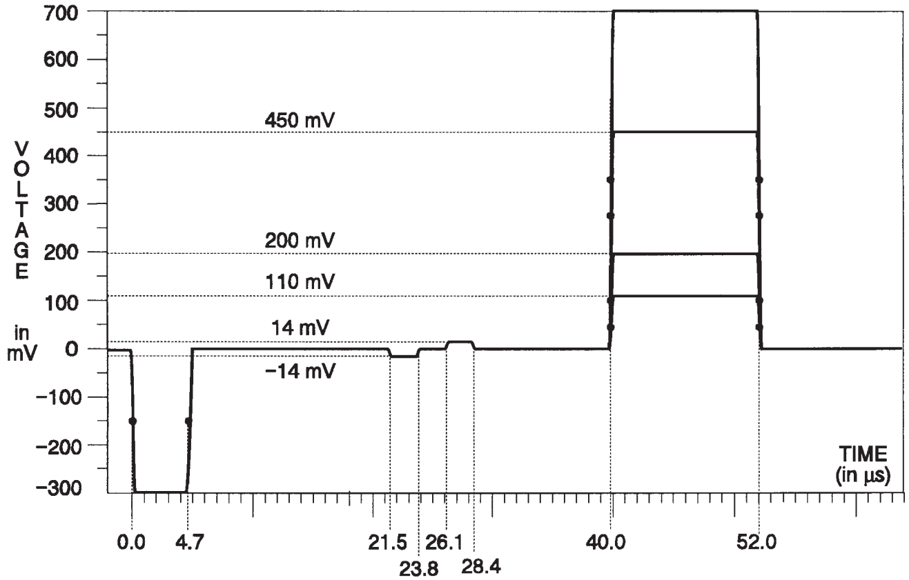
Fig. 3-40. Y Channel — Pluge.
