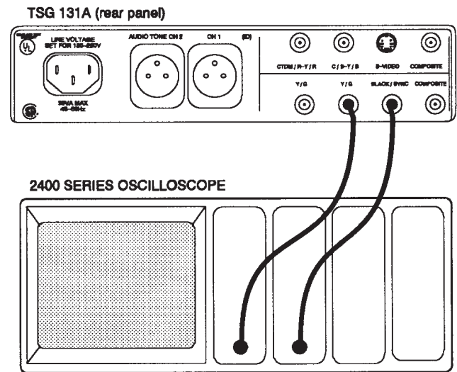
Fig. 4-7. Setup to check the pulse outputs for Options 02, 03, & 04.
