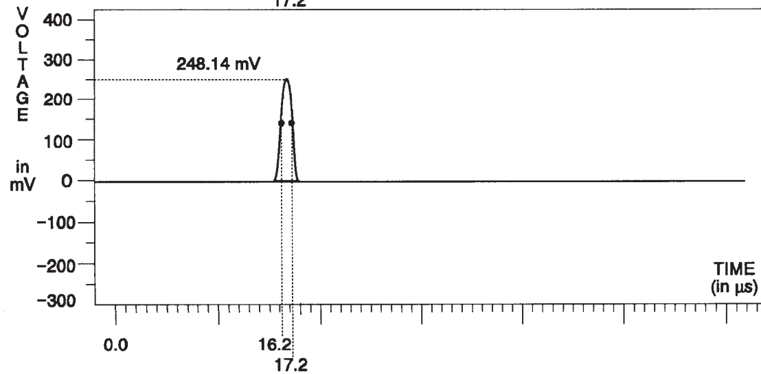
Fig. 3-183. R-Y Channel — Pulse & Bar.
