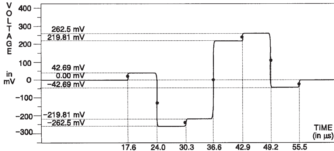
Fig. 3-73. R-Y Channel — 75% Bars.
