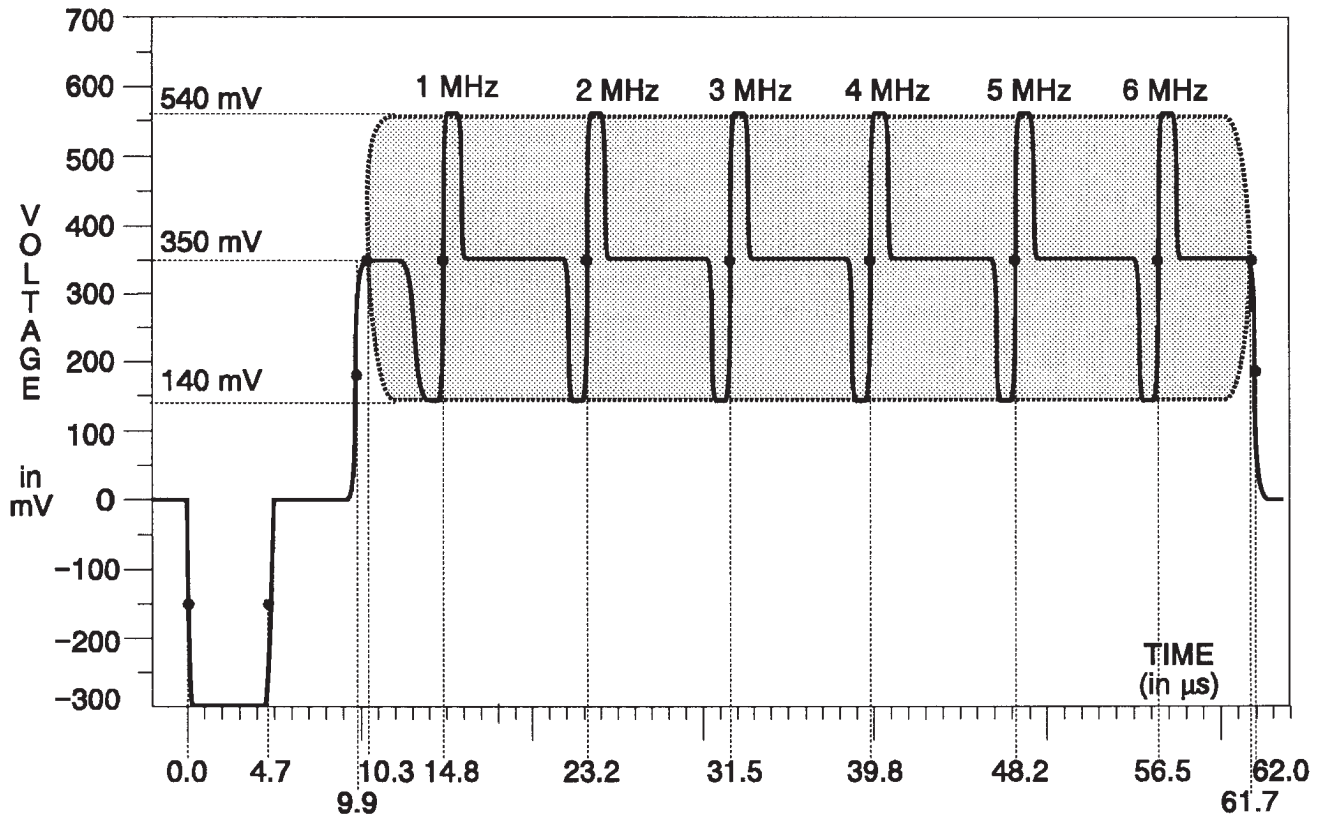
Fig. 3-171. Y Channel — Reduced Sweep.
