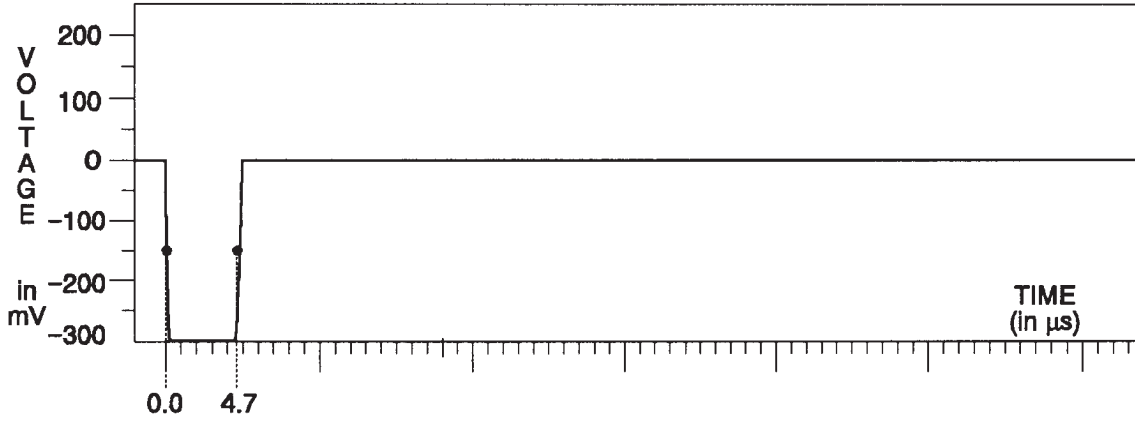
Fig. 3-120. Green Channel — Blue Field.
