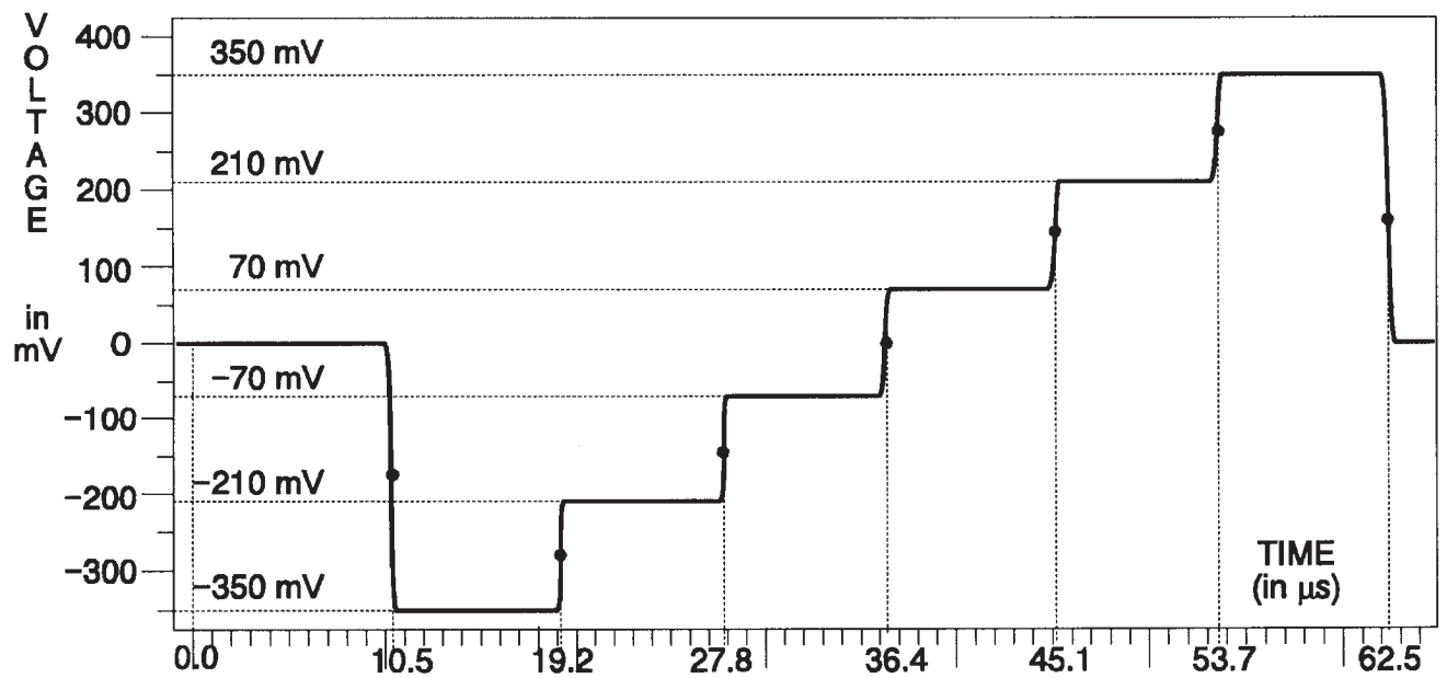
Fig. 3-232. B-Y & R-Y Channels — 5-Step.
