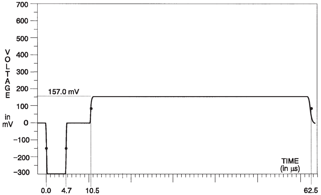
Fig. 3-34. Y Channel — 75% Red.(Same as Red Field)
