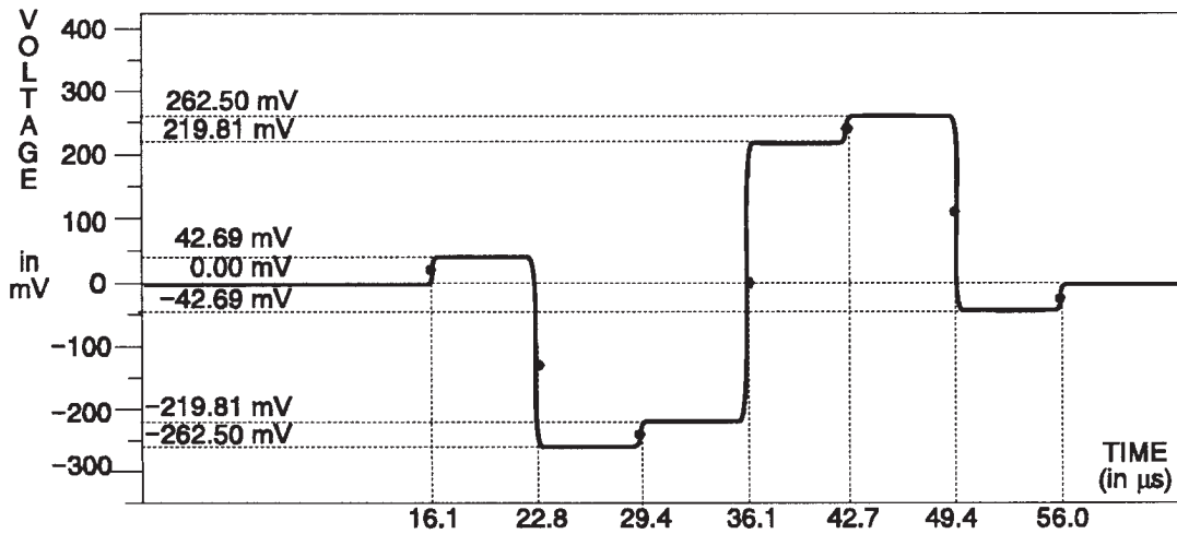
Fig. 3-177. R-Y Channel — 75% Color Bars.
