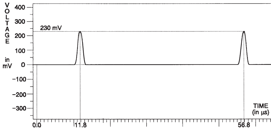
Fig. 3-210. R-Y Channel — 12T Pulses.
