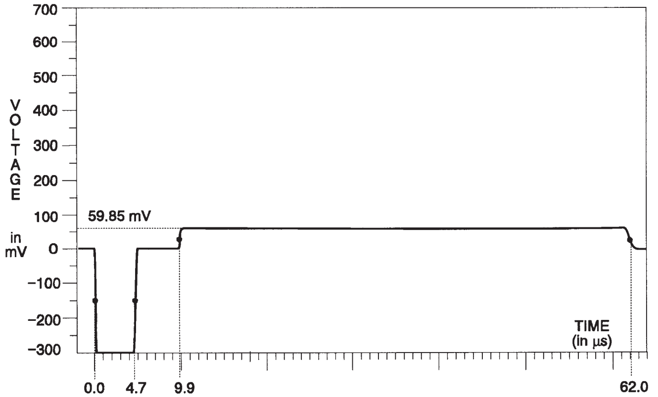
Fig. 3-157. Y Channel — Blue Field.
