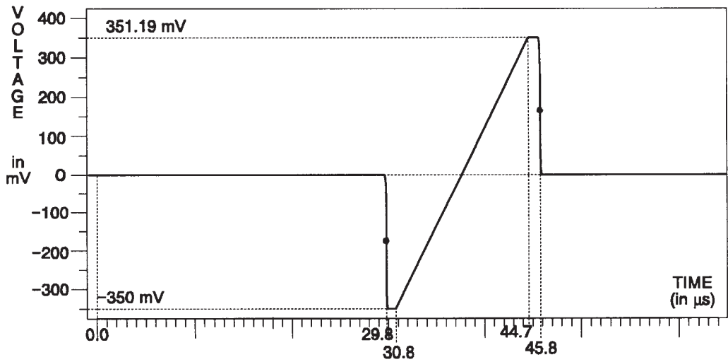
Fig. 3-194. R-Y Channel — Quad Phase.
