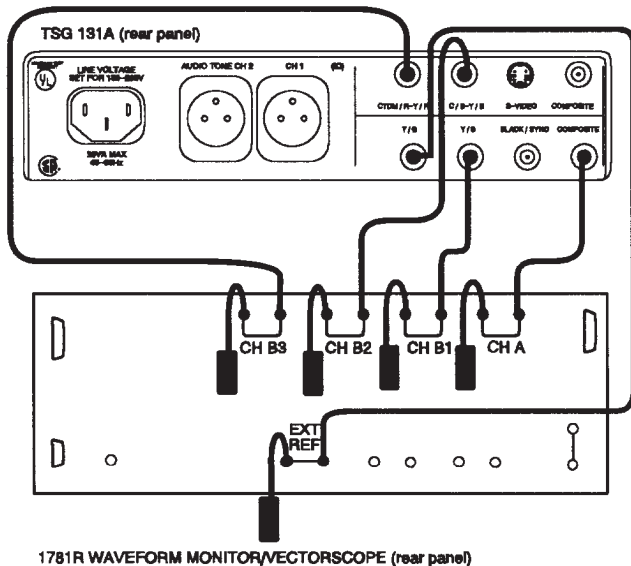
Fig. 4-12. Basic setup for the calibration procedures.
