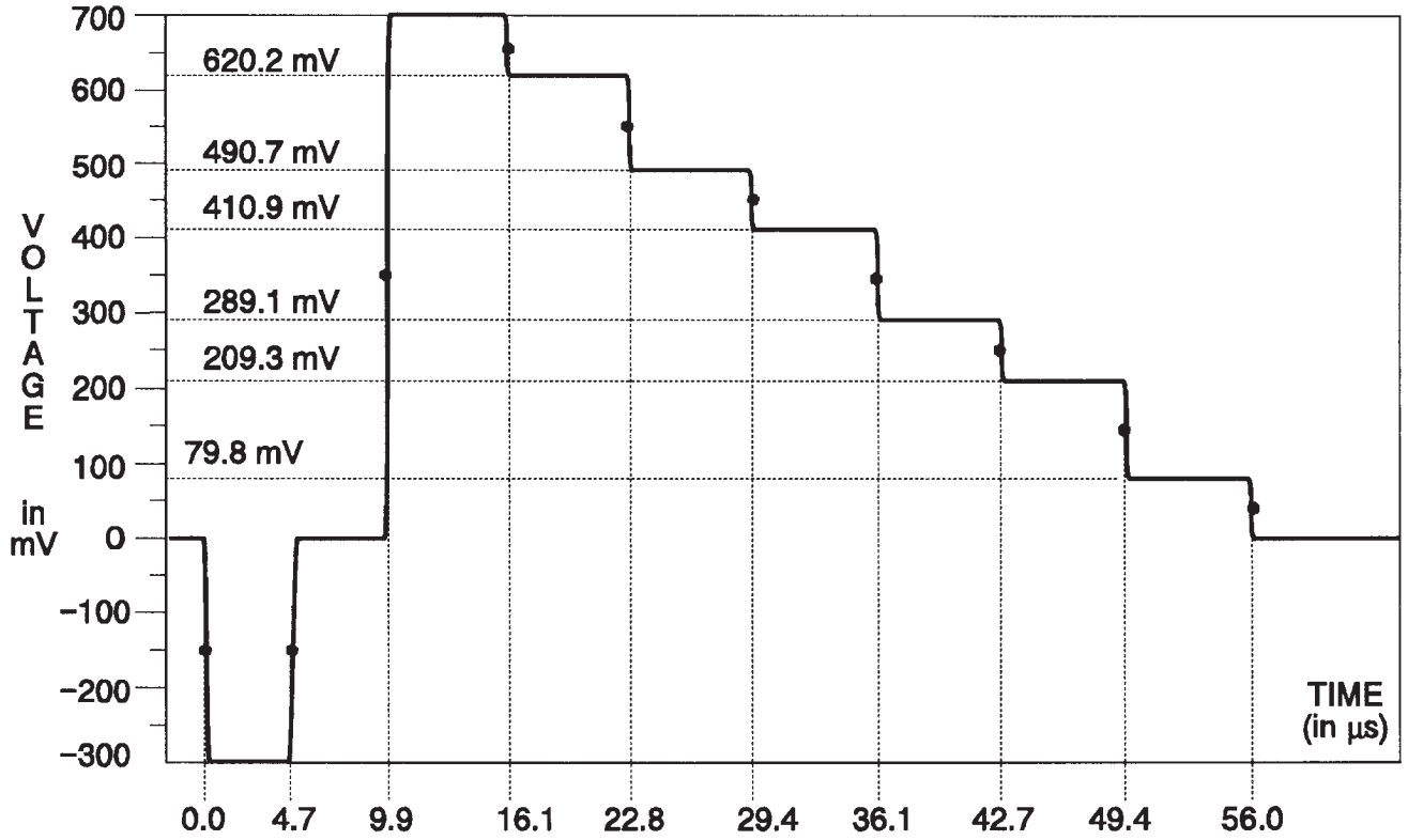
Fig. 3-153. Y Channel — 100% Bars.
