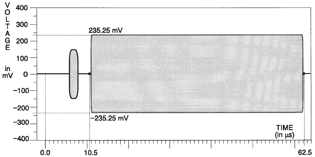
Fig. 3-43. C Channel — Blue Field.
