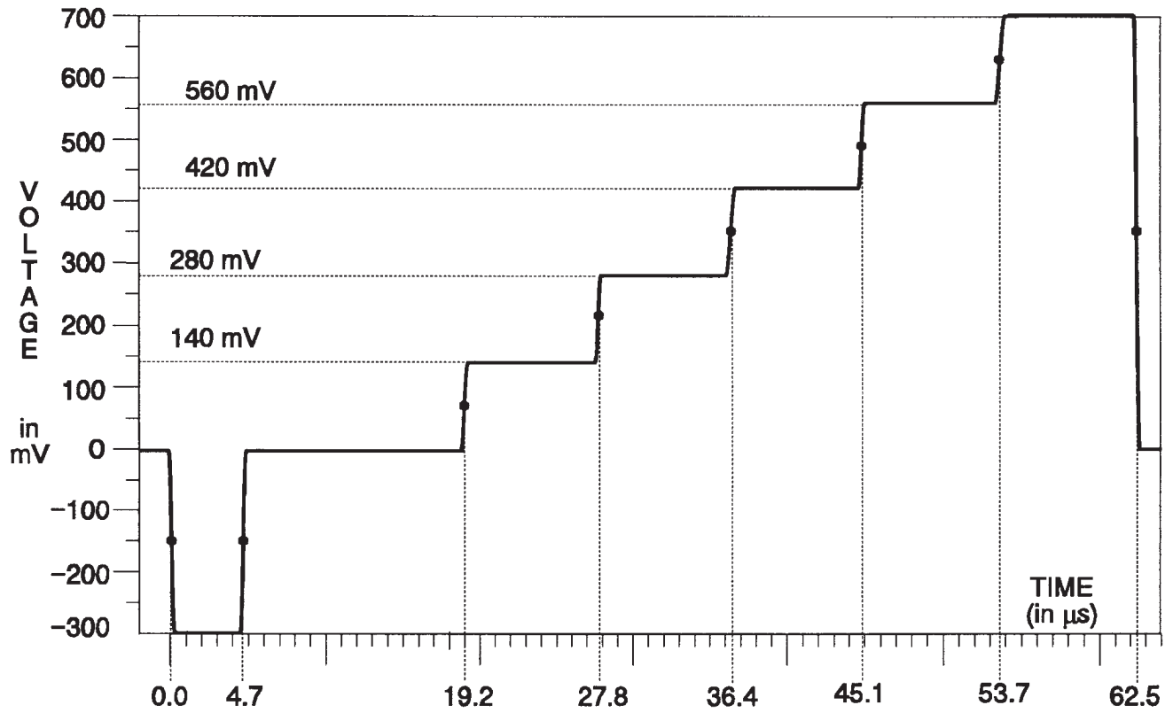
Fig. 3-56. Y Channel — 5-Step.
