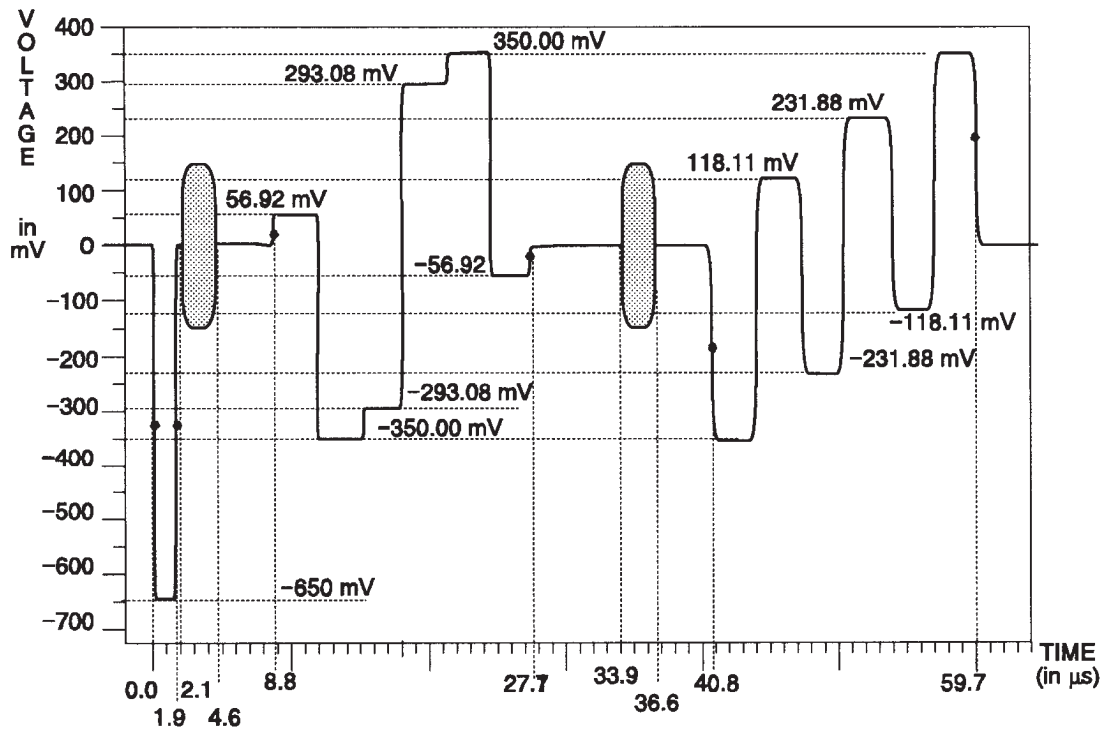
Fig. 3-144. C Channel — 100% Color Bars.
