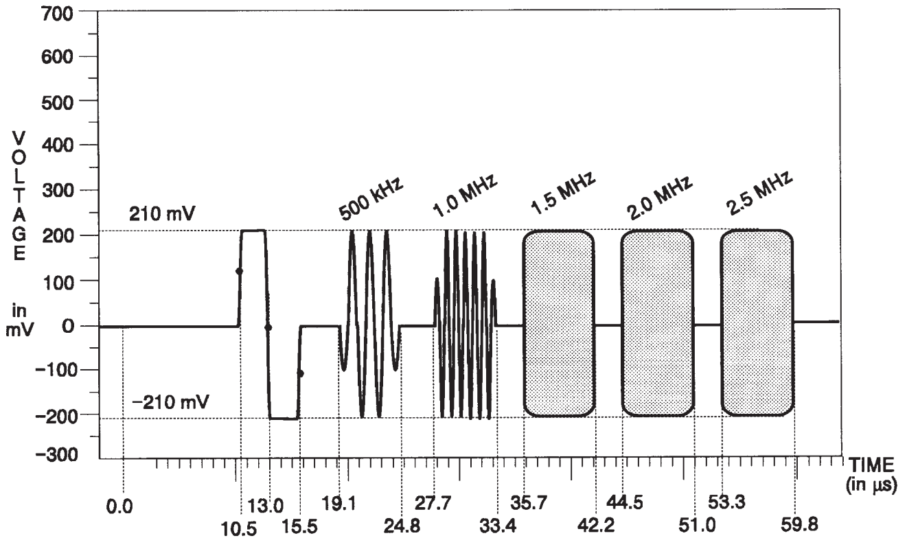
Fig. 3-102. B-Y & R-Y Channels — Multiburst.
